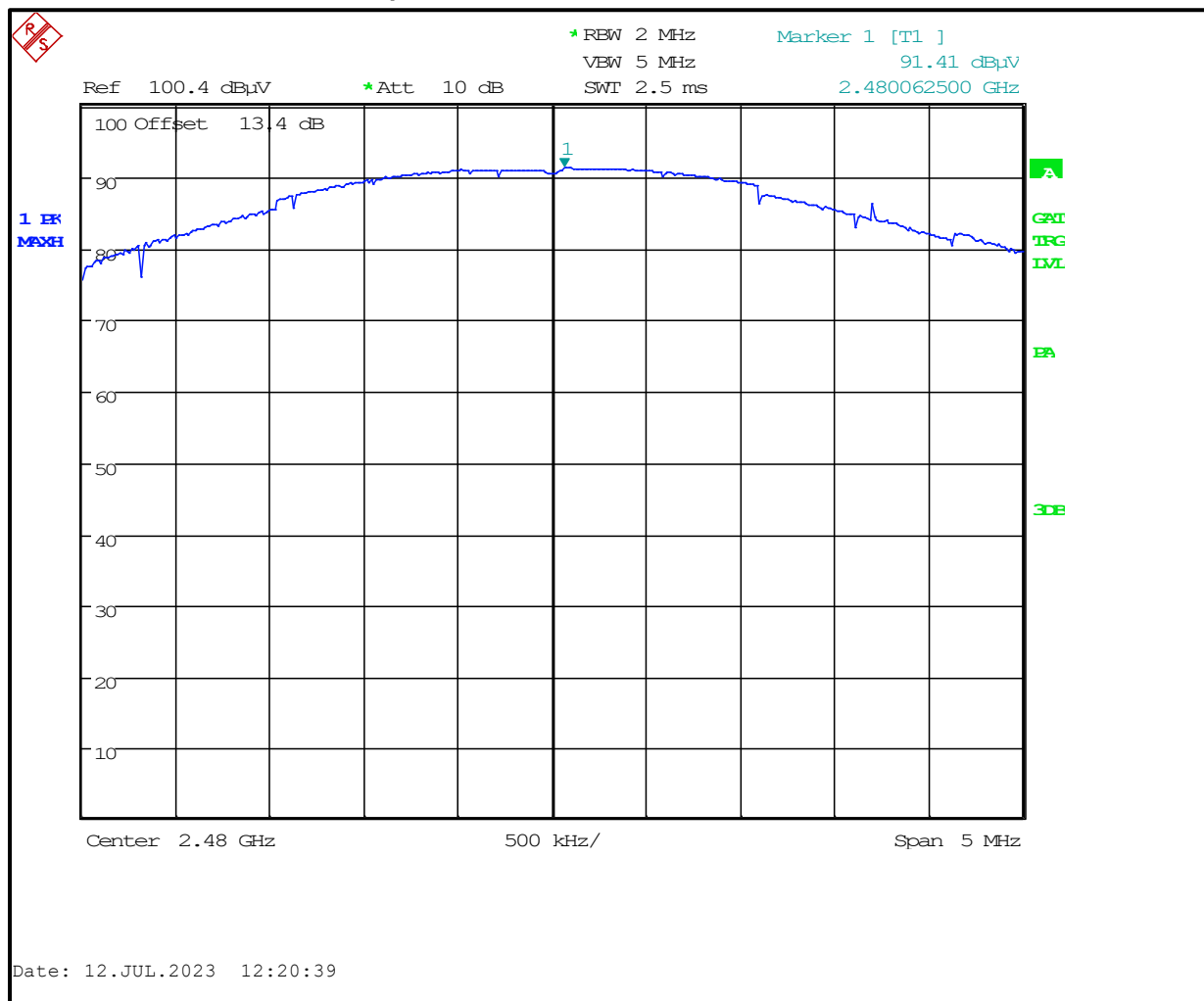
Plot 3-3: Peak Power Output – 2480 MHz
