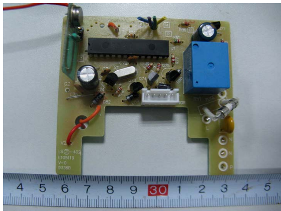
EUT- 433.92MHz Power Board Components View
