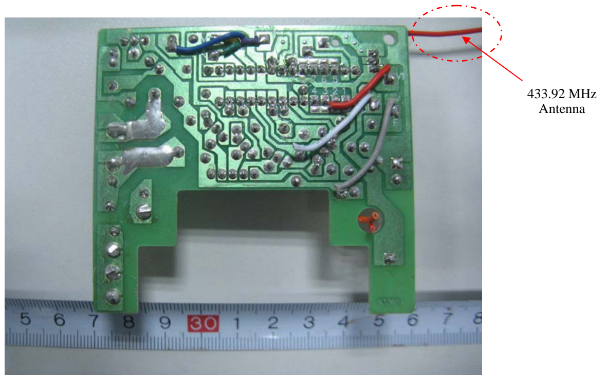
EUT- 433.92 MHz Power Board Circuit View
