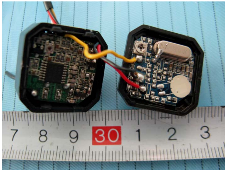
EUT- 2.4GHz Wireless Camera Mainboard1 Top View
