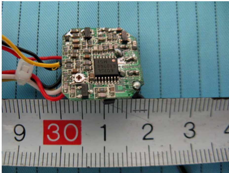
EUT- 2.4GHz Wireless Camera Mainboard1 Bottom View
