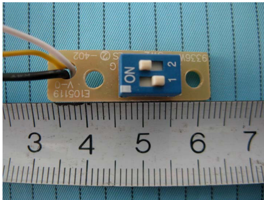
EUT- Channel Contrl Board Top View
