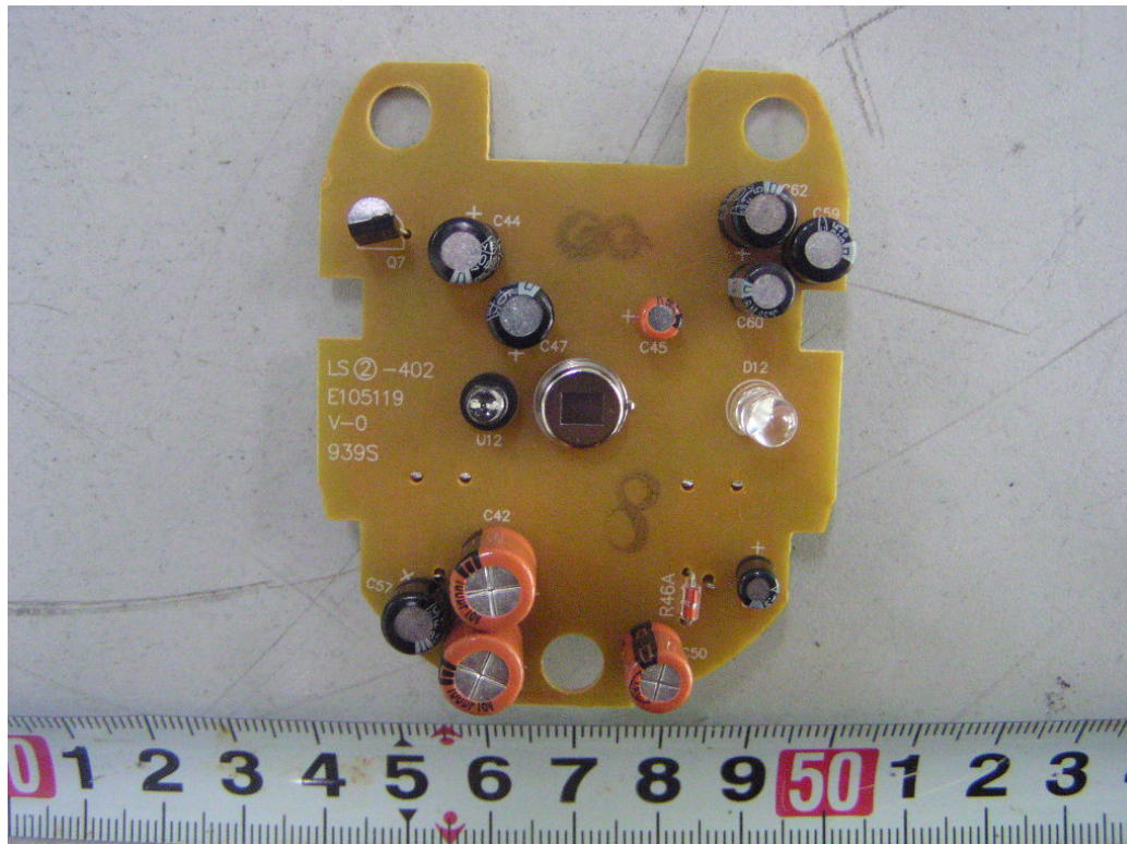
EUT – Sensor Board Top Components View
