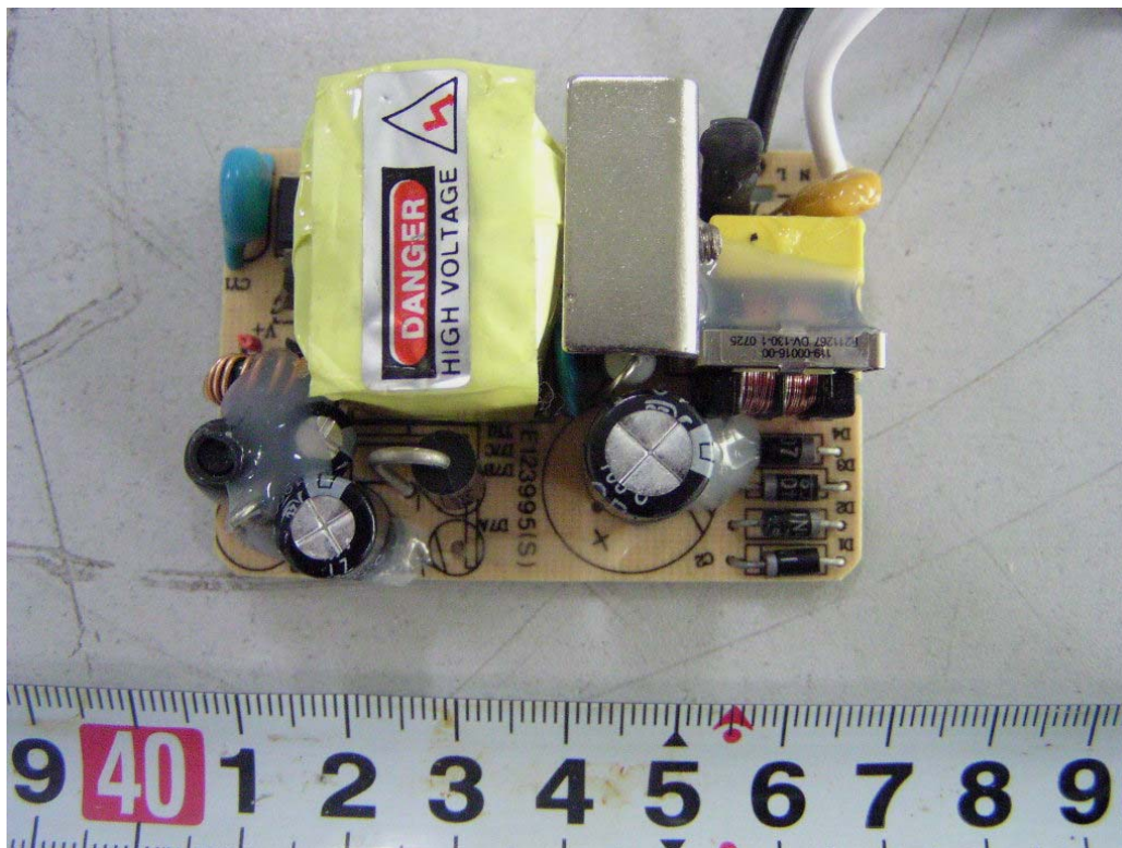
EUT – Power Supply Board Assembly Top Components View
