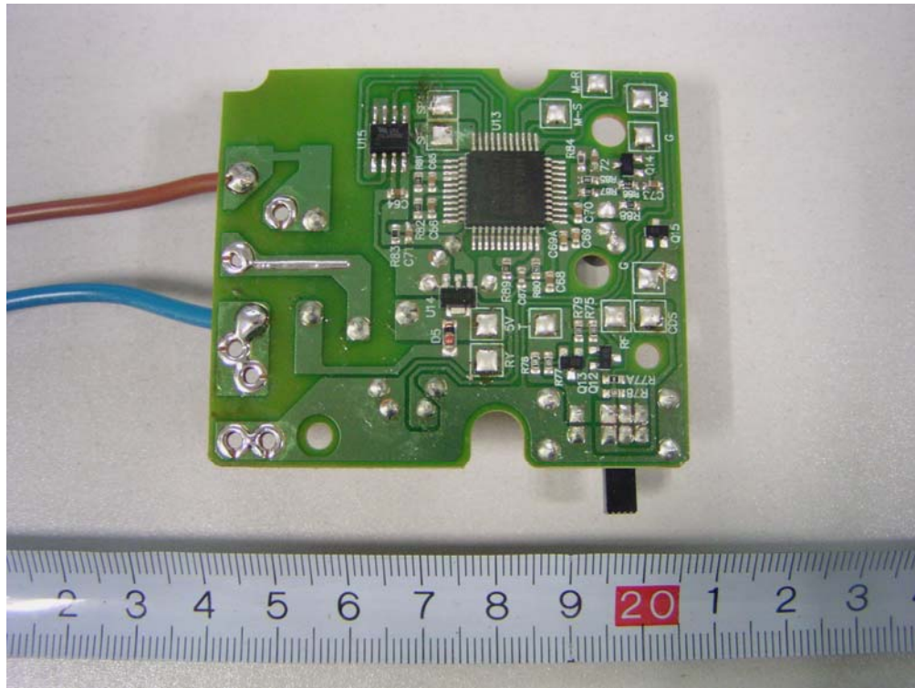
EUT – Switch Board Bottom Components View
