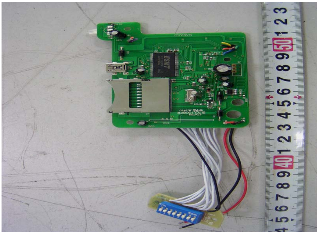
EUT – Main Board Top Components View
