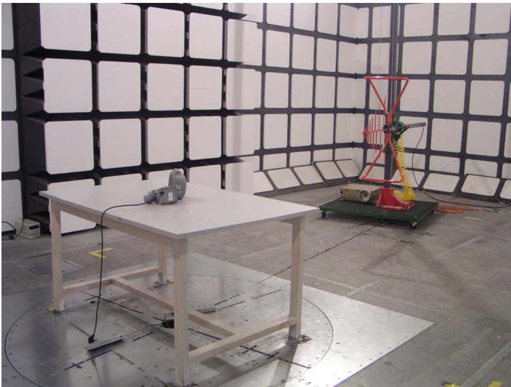
Radiated Emissions (30-1000MHz) - Rear View
