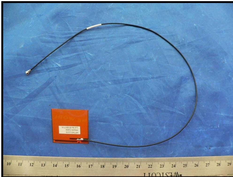
Antenna with Cable View
