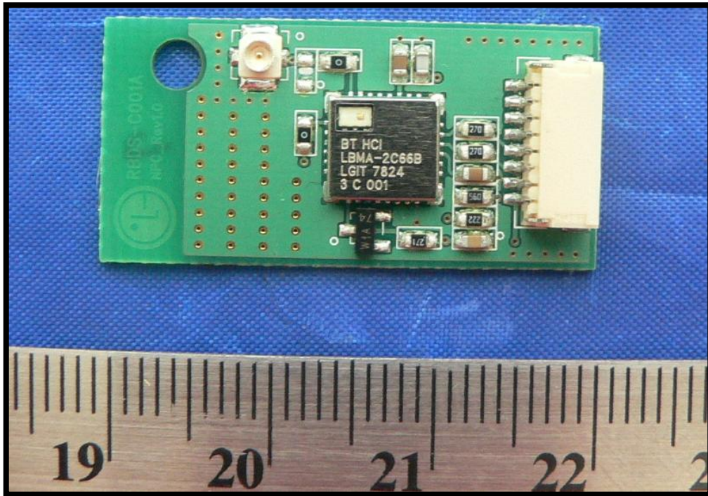
EUT without Shielding Component View
