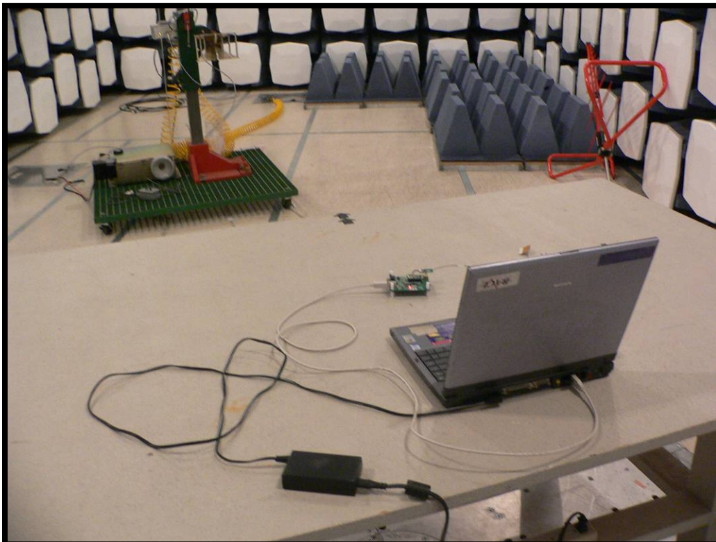
Transmitter Radiated Emissions – Rear View
