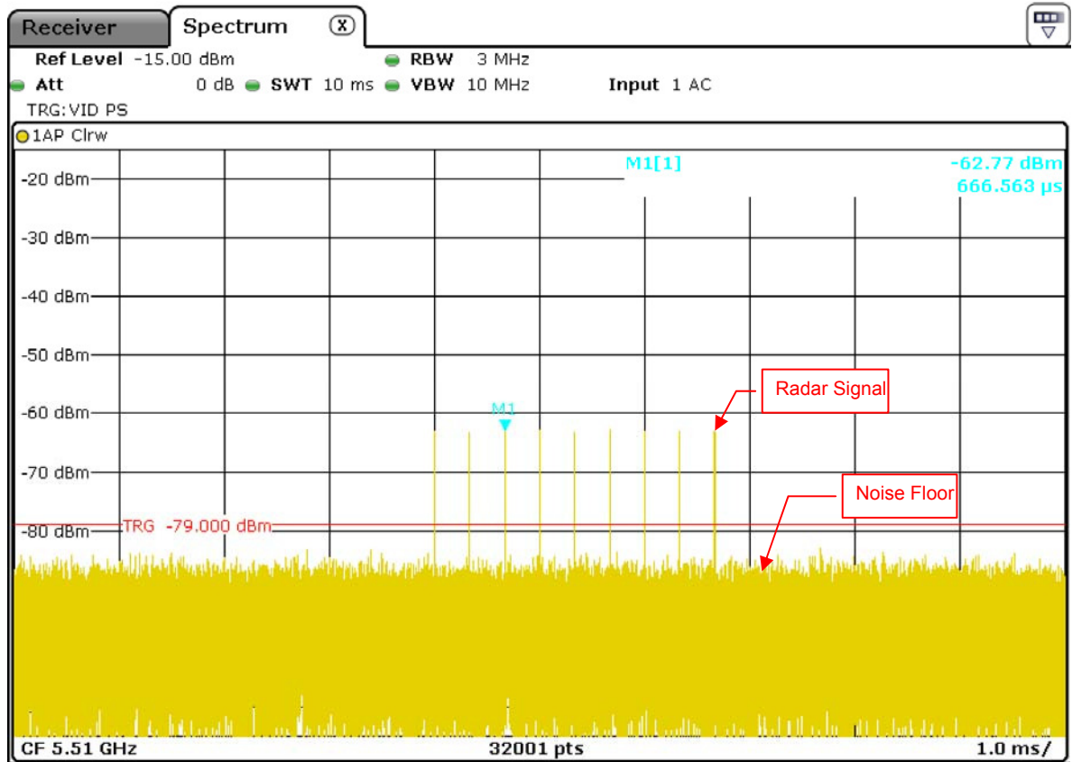
Radar Signal 6
