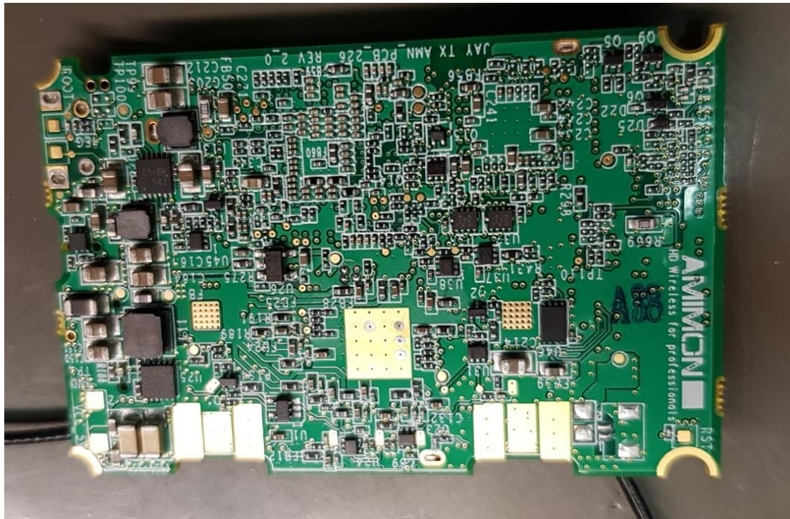
Figure 1 - VQSAMNPTTX01 Bottom View
