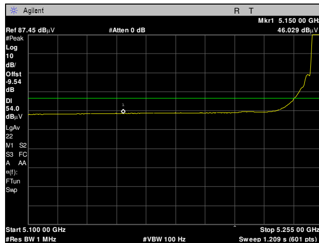
Plot 73. Radiated Band Edge, 5255 MHz, 10 MHz, Average
