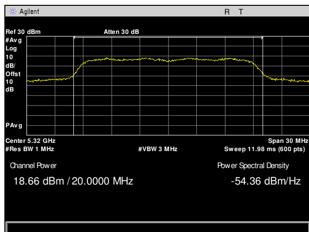
Plot 26. Maximum Conducted Output Power, 5320 MHz, 20 MHz, Channel 0
