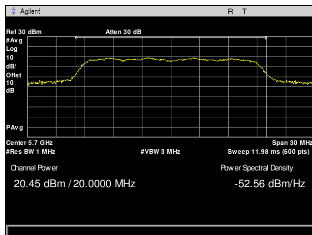
Plot 29. Maximum Conducted Output Power, 5700 MHz, 20 MHz, Channel 0
