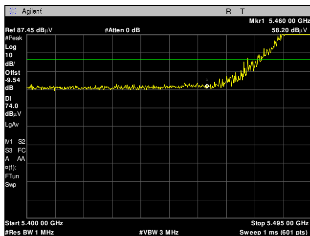
Plot 78. Radiated Band Edge, 5495 MHz, 10 MHz, Peak
