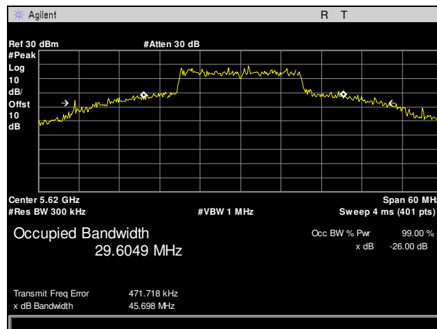
Plot 11. Occupied Bandwidth, 5620 MHz, 20 MHz, Channel 0
