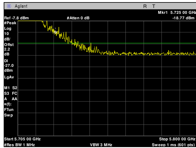
Plot 82. Radiated Band Edge, 5705 MHz, 10 MHz, Peak
