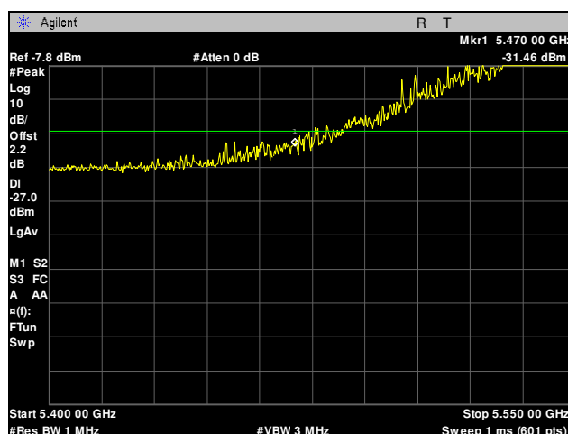
Plot 101. Radiated Band Edge, 5550 MHz, 40 MHz, Peak
