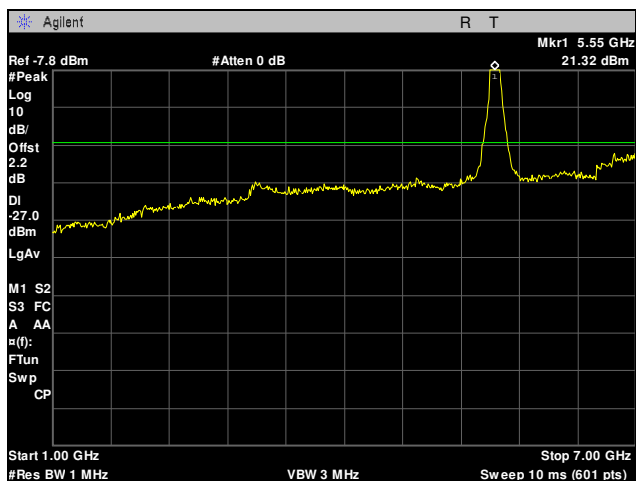
Plot 70. Radiated Spurious Emissions, 5550 MHz, 40 MHz, 1 GHz – 7 GHz
