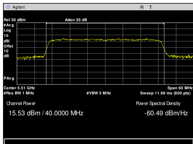
Plot 32. Maximum Conducted Output Power, 5510 MHz, 40 MHz, Channel 0
