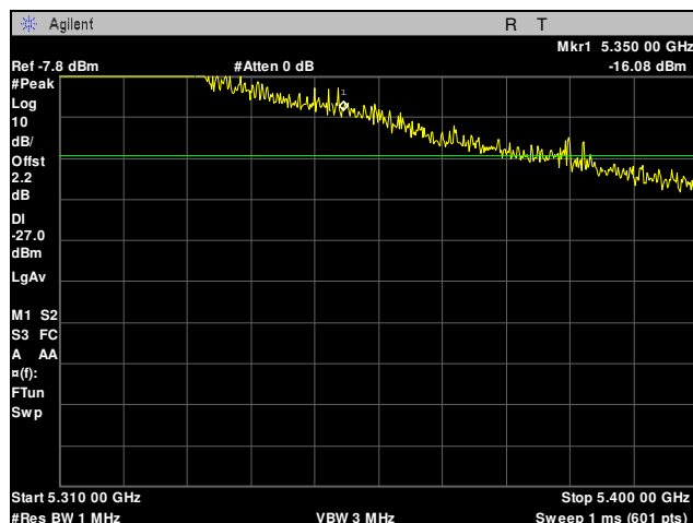
Plot 96. Radiated Band Edge, 5310 MHz, 40 MHz, Peak
