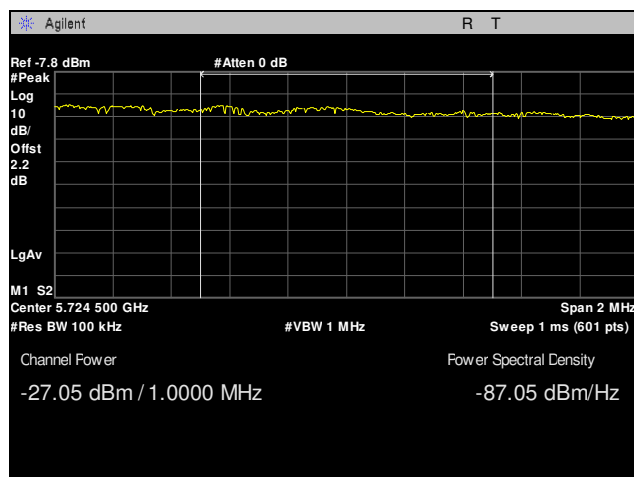
Plot 90. Radiated Band Edge, 5700 MHz, 20 MHz, Peak Integration
