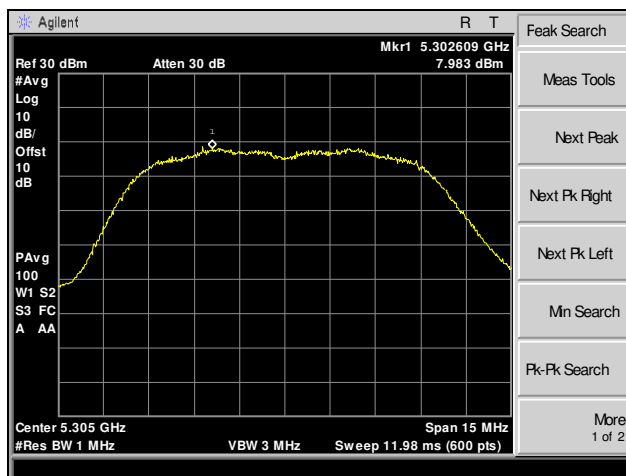
Plot 37. Maximum Power Spectral Density, 5305 MHz, 10 MHz, Channel 0
