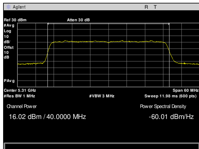
Plot 31. Maximum Conducted Output Power, 5310 MHz, 40 MHz, Channel 0
