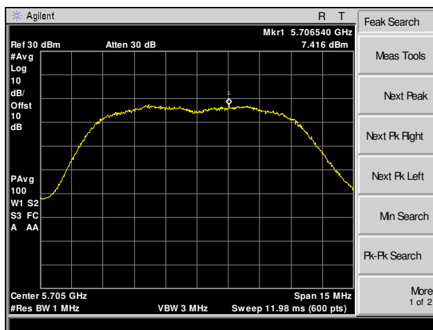
Plot 41. Maximum Power Spectral Density, 5705 MHz, 10 MHz, Channel 0
