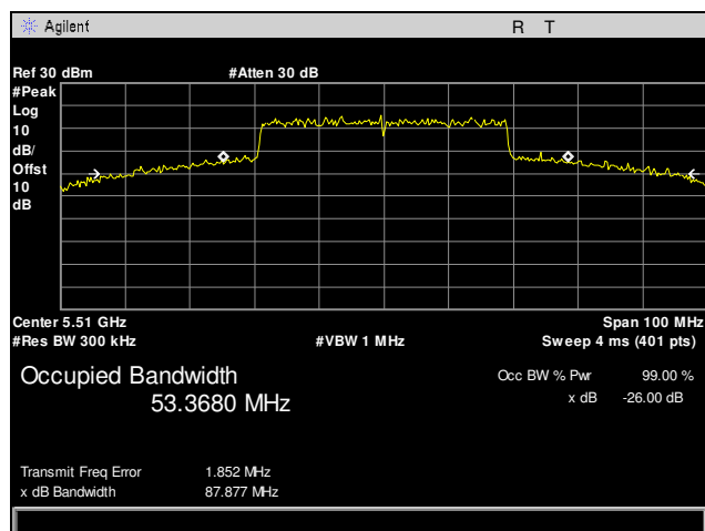
Plot 15. Occupied Bandwidth, 5510 MHz, 40 MHz, Channel 0
