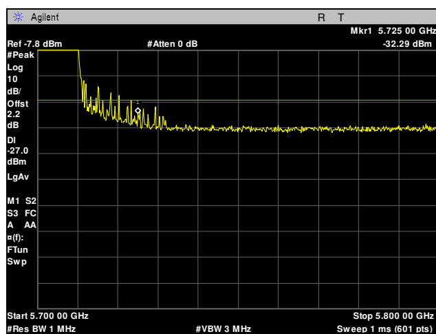
Plot 91. Radiated Band Edge, 5700 MHz, 20 MHz, Peak
