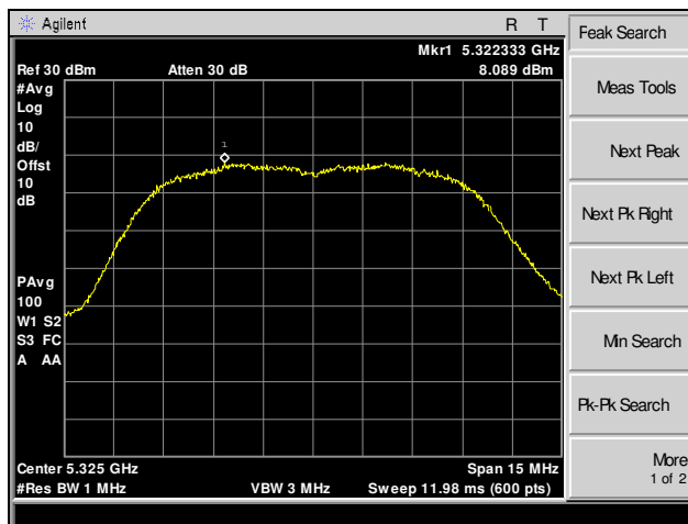
Plot 38. Maximum Power Spectral Density, 5325 MHz, 10 MHz, Channel 0
