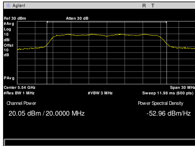
Plot 27. Maximum Conducted Output Power, 5540 MHz, 20 MHz, Channel 0
