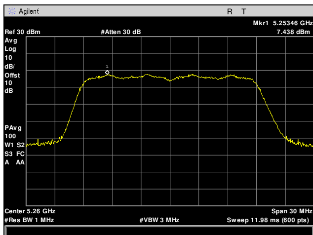
Plot 42. Maximum Power Spectral Density, 5260 MHz, 20 MHz, Channel 0
