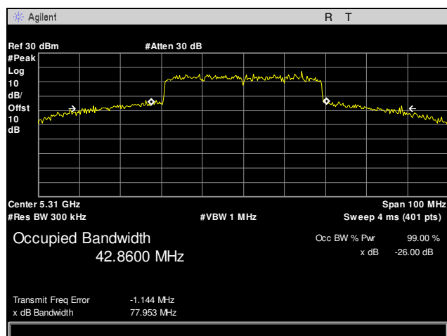
Plot 14. Occupied Bandwidth, 5310 MHz, 40 MHz, Channel 0
