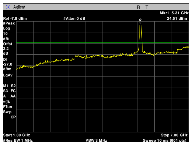
Plot 62. Radiated Spurious Emissions, 5320 MHz, 20 MHz, 1 GHz – 7 GHz
