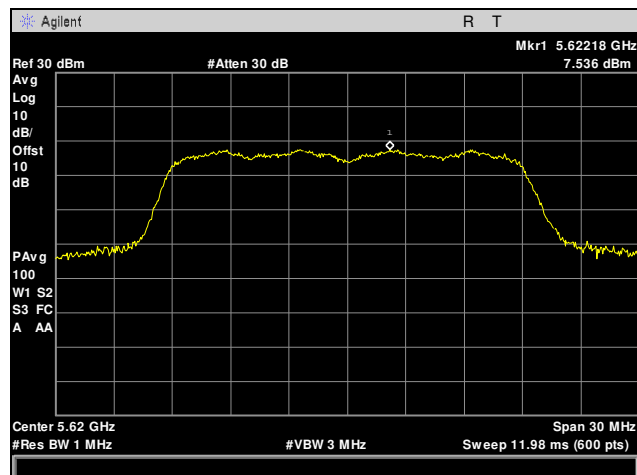
Plot 46. Maximum Power Spectral Density, 5620 MHz, 20 MHz, Channel 0
