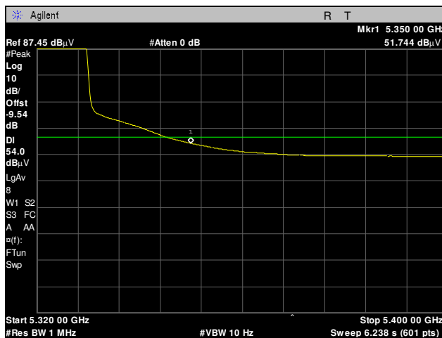
Plot 85. Radiated Band Edge, 5320 MHz, 20 MHz, Average
