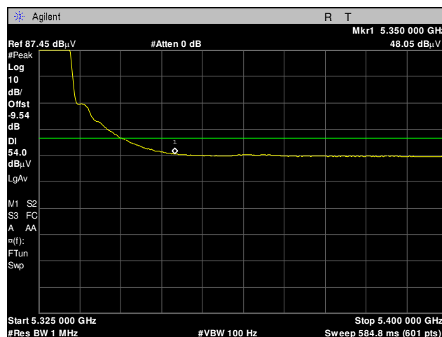
Plot 75. Radiated Band Edge, 5325 MHz, 10 MHz, Average
