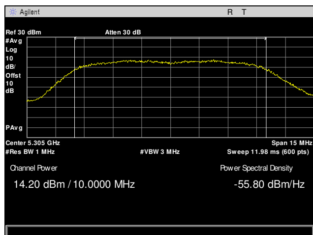
Plot 19. Maximum Conducted Output Power, 5305 MHz, 10 MHz, Channel 0
