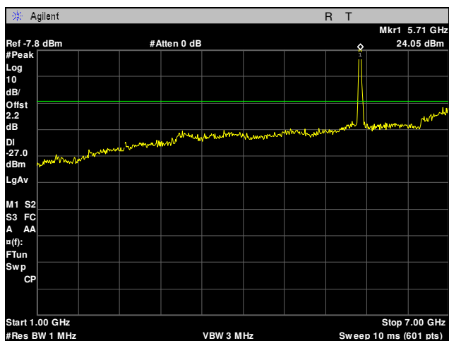
Plot 59. Radiated Spurious Emissions, 5705 MHz, 10 MHz, 1 GHz – 7 GHz
