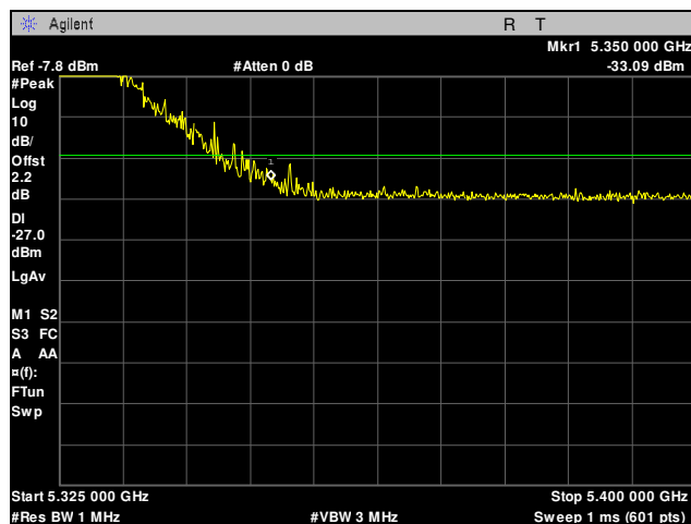
Plot 76. Radiated Band Edge, 5325 MHz, 10 MHz, Peak
