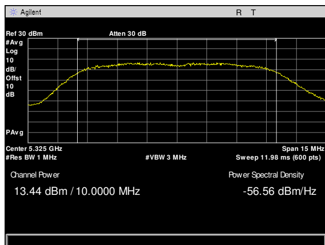
Plot 20. Maximum Conducted Output Power, 5325 MHz, 10 MHz, Channel 0
