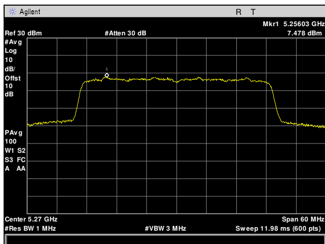
Plot 48. Maximum Power Spectral Density, 5270 MHz, 40 MHz, Channel 0
