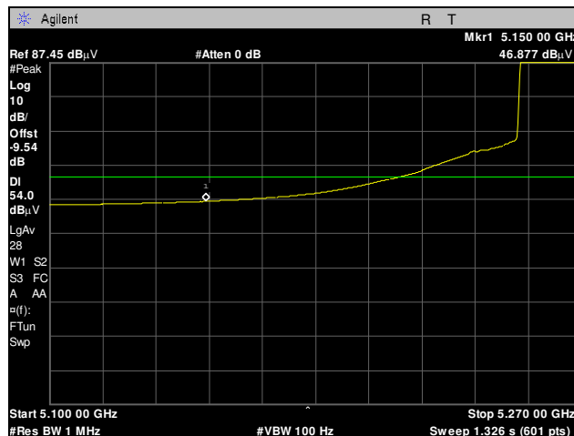
Plot 93. Radiated Band Edge, 5270 MHz, 40 MHz, Average
