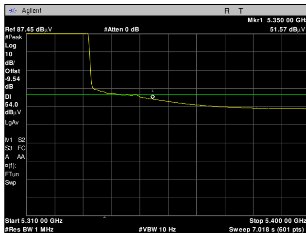
Plot 95. Radiated Band Edge, 5310 MHz, 40 MHz, Average
