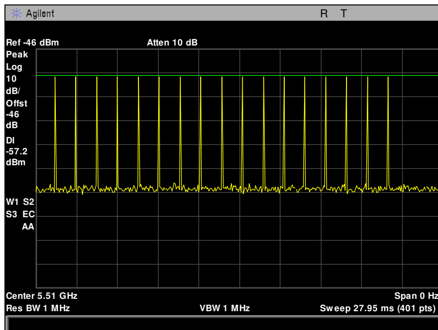
Plot 107. Radar Waveform Calibration, Type 0, 5510 MHz, 10 dBm
