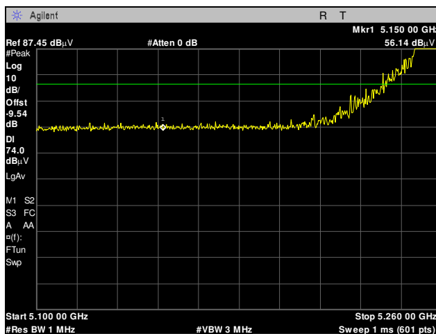
Plot 84. Radiated Band Edge, 5260 MHz, 20 MHz, Peak
