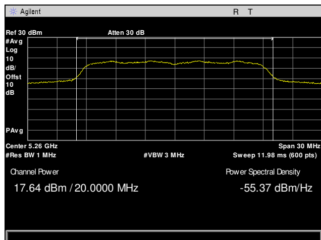
Plot 24. Maximum Conducted Output Power, 5260 MHz, 20 MHz, Channel 0
