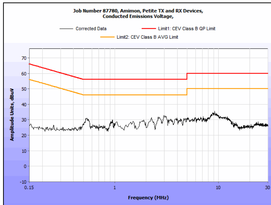
Plot 105. Conducted Emission, Neutral Line Plot
