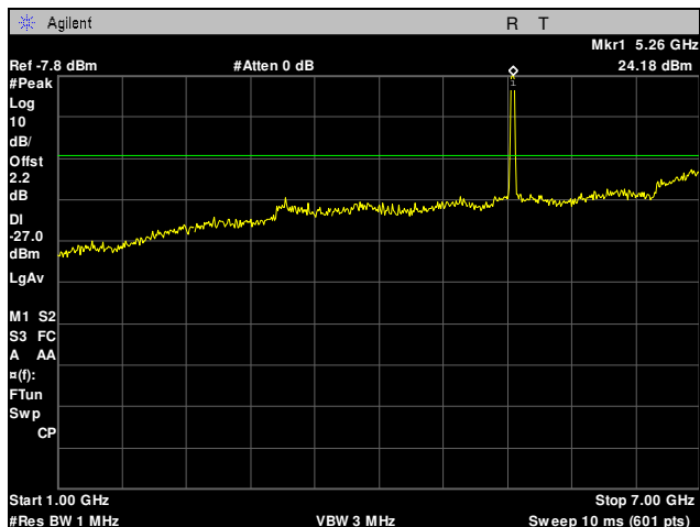
Plot 54. Radiated Spurious Emissions, 5255 MHz, 10 MHz, 1 GHz – 7 GHz
