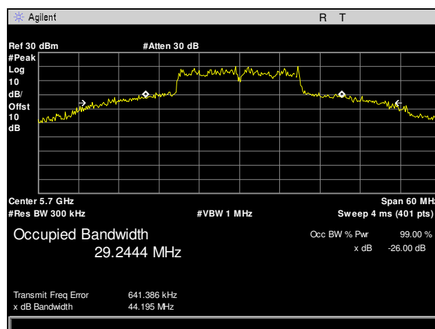
Plot 12. Occupied Bandwidth, 5700 MHz, 20 MHz, Channel 0
