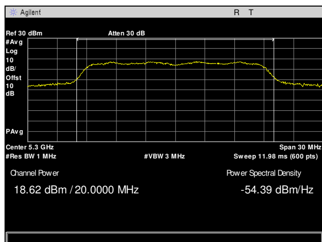
Plot 25. Maximum Conducted Output Power, 5300 MHz, 20 MHz, Channel 0
