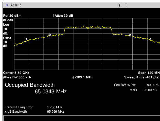
Plot 16. Occupied Bandwidth, 5590 MHz, 40 MHz, Channel 0
