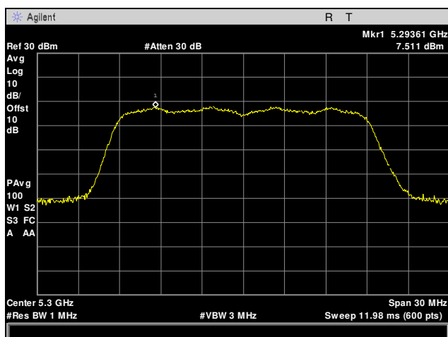
Plot 43. Maximum Power Spectral Density, 5300 MHz, 20 MHz, Channel 0
