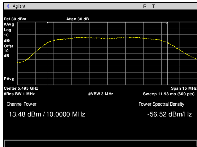
Plot 21. Maximum Conducted Output Power, 5495 MHz, 10 MHz, Channel 0
