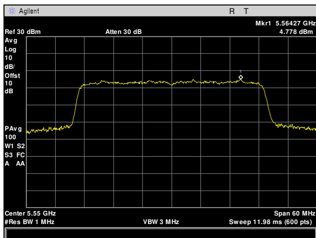
Plot 51. Maximum Power Spectral Density, 5550 MHz, 40 MHz, Channel 0
