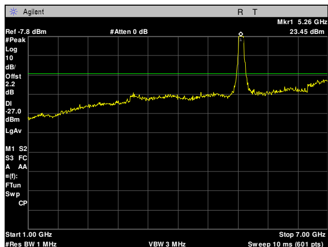
Plot 67. Radiated Spurious Emissions, 5270 MHz, 40 MHz, 1 GHz – 7 GHz
