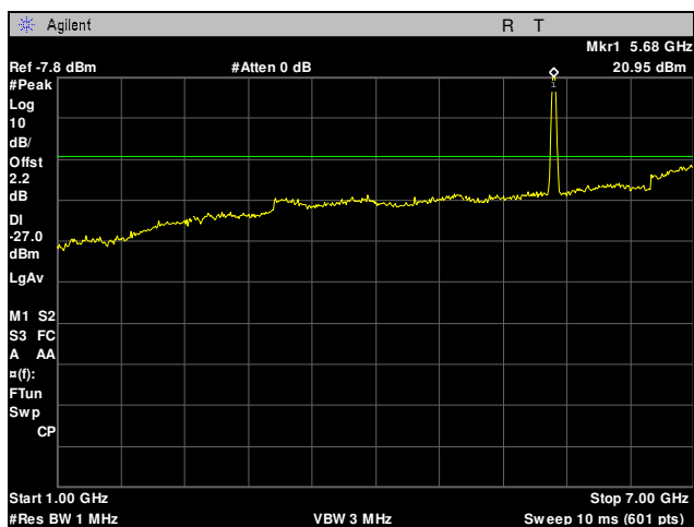
Plot 65. Radiated Spurious Emissions, 5680 MHz, 20 MHz, 1 GHz – 7 GHz
