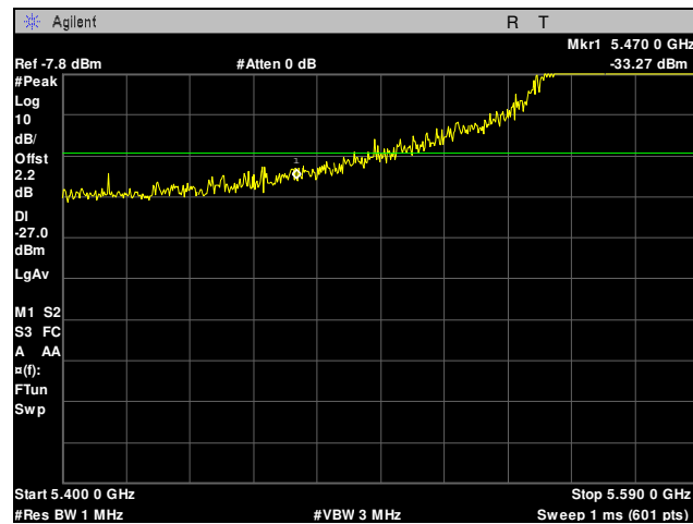
Plot 102. Radiated Band Edge, 5590 MHz, 40 MHz, Peak
