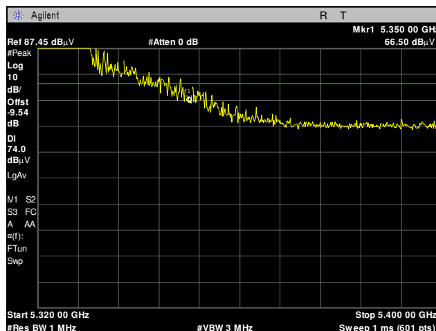
Plot 86. Radiated Band Edge, 5320 MHz, 20 MHz, Peak
