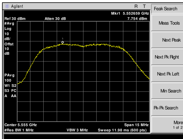
Plot 40. Maximum Power Spectral Density, 5555 MHz, 10 MHz, Channel 0
