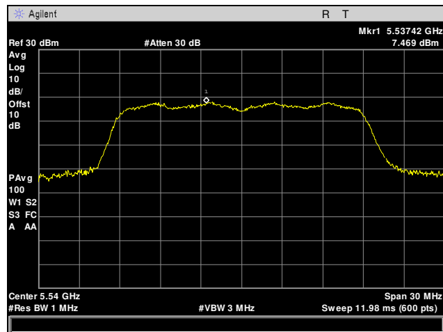
Plot 45. Maximum Power Spectral Density, 5540 MHz, 20 MHz, Channel 0
