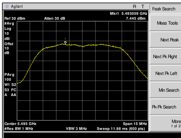
Plot 39. Maximum Power Spectral Density, 5495 MHz, 10 MHz, Channel 0
