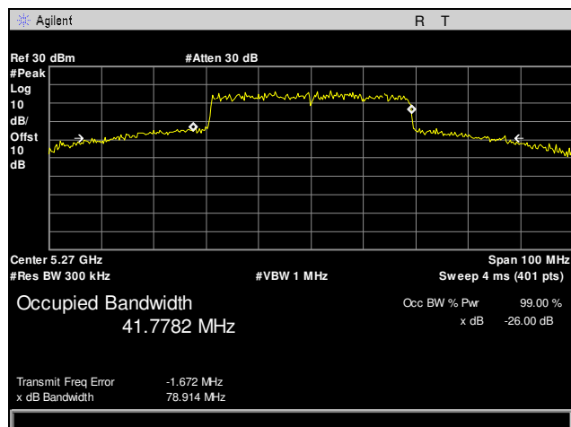
Plot 13. Occupied Bandwidth, 5270 MHz, 40 MHz, Channel 0
