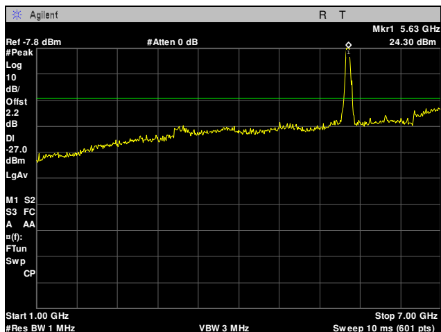
Plot 64. Radiated Spurious Emissions, 5620 MHz, 20 MHz, 1 GHz – 7 GHz
