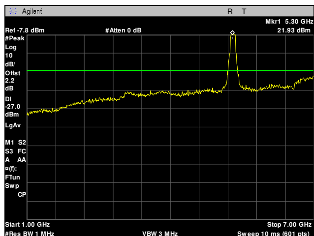
Plot 68. Radiated Spurious Emissions, 5310 MHz, 40 MHz, 1 GHz – 7 GHz
