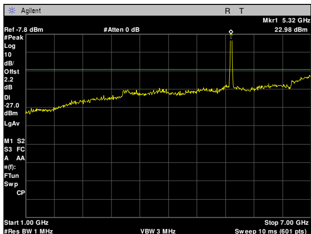
Plot 56. Radiated Spurious Emissions, 5325 MHz, 10 MHz, 1 GHz – 7 GHz
