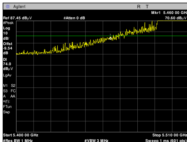
Plot 99. Radiated Band Edge, 5510 MHz, 40 MHz, Peak
