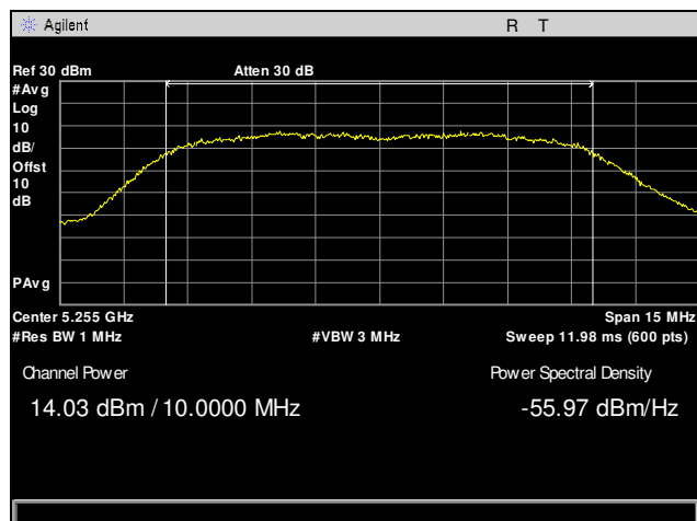
Plot 18. Maximum Conducted Output Power, 5255 MHz, 10 MHz, Channel 0
