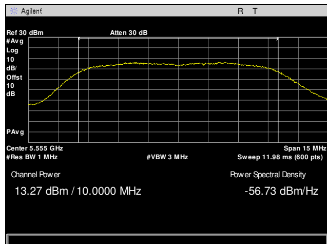
Plot 22. Maximum Conducted Output Power, 5555 MHz, 10 MHz, Channel 0
