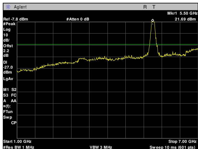
Plot 69. Radiated Spurious Emissions, 5510 MHz, 40 MHz, 1 GHz – 7 GHz
