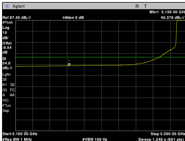
Plot 83. Radiated Band Edge, 5260 MHz, 20 MHz, Average
