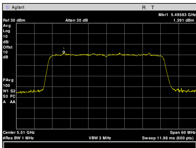
Plot 50. Maximum Power Spectral Density, 5510 MHz, 40 MHz, Channel 0
