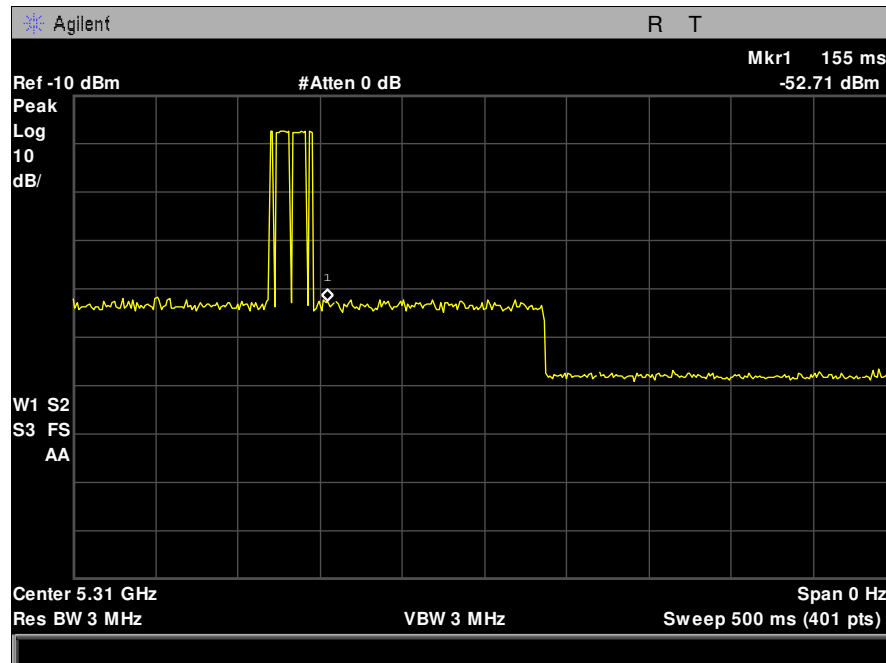
Plot 109. Channel Close Time, 40 MHz
