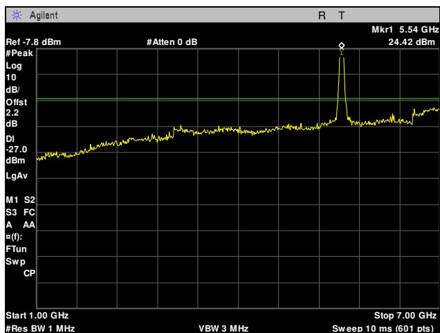
Plot 63. Radiated Spurious Emissions, 5540 MHz, 20 MHz, 1 GHz – 7 GHz
