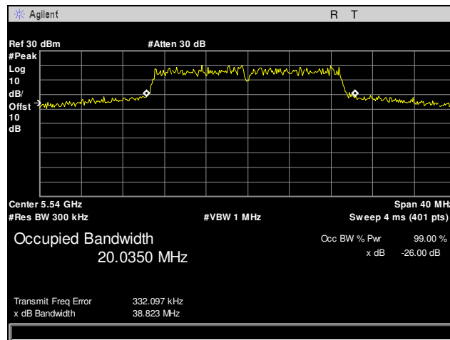
Plot 10. Occupied Bandwidth, 5540 MHz, 20 MHz, Channel 0
