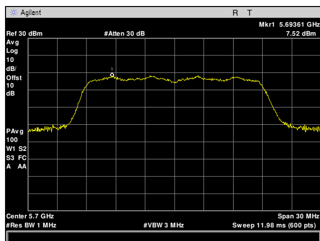
Plot 47. Maximum Power Spectral Density, 5700 MHz, 20 MHz, Channel 0
