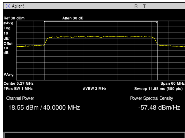
Plot 30. Maximum Conducted Output Power, 5270 MHz, 40 MHz, Channel 0
