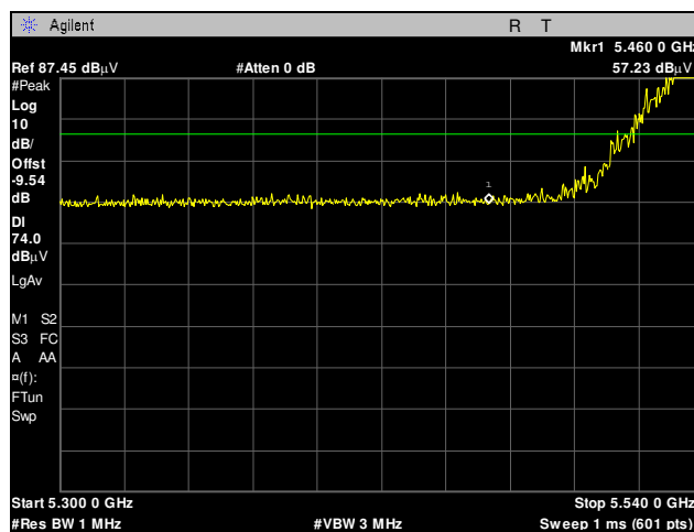
Plot 88. Radiated Band Edge, 5540 MHz, 20 MHz, Peak
