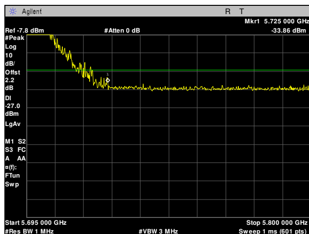
Plot 80. Radiated Band Edge, 5695 MHz, 10 MHz, Peak
