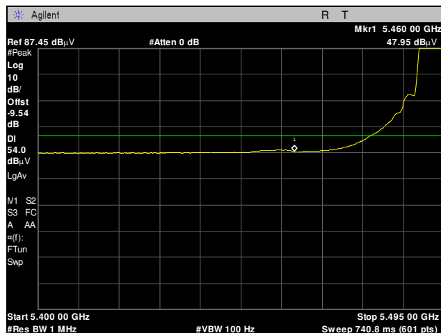
Plot 77. Radiated Band Edge, 5495 MHz, 10 MHz, Average
