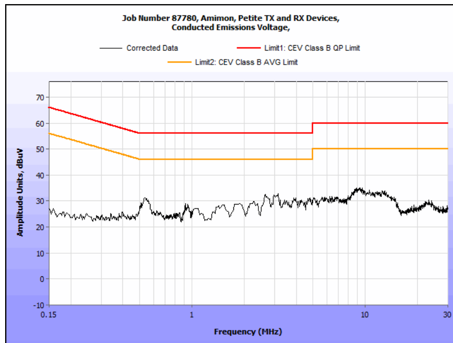
Plot 104. Conducted Emission, Phase Line Plot
