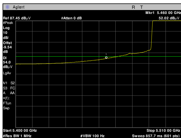
Plot 98. Radiated Band Edge, 5510 MHz, 40 MHz, Average
