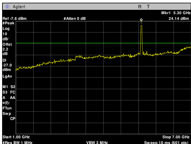
Plot 55. Radiated Spurious Emissions, 5305 MHz, 10 MHz, 1 GHz – 7 GHz
