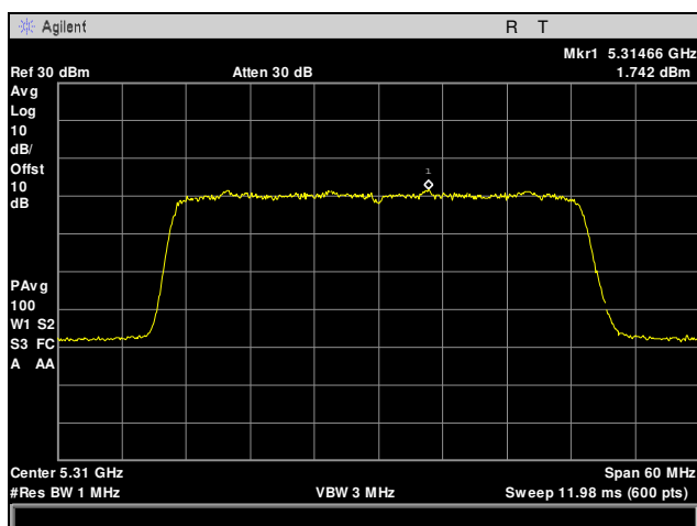
Plot 49. Maximum Power Spectral Density, 5310 MHz, 40 MHz, Channel 0
