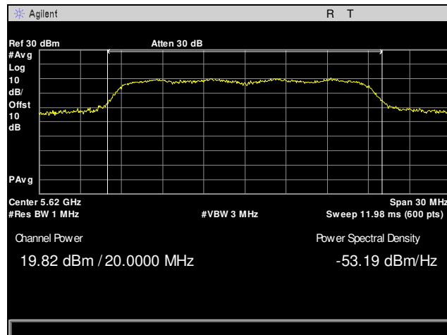
Plot 28. Maximum Conducted Output Power, 5620 MHz, 20 MHz, Channel 0
