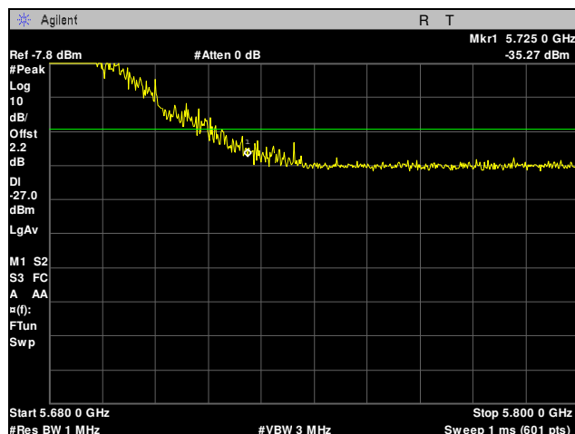
Plot 89. Radiated Band Edge, 5680 MHz, 20 MHz, Peak
