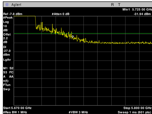
Plot 103. Radiated Band Edge, 5670MHz, 40 MHz, Peak
