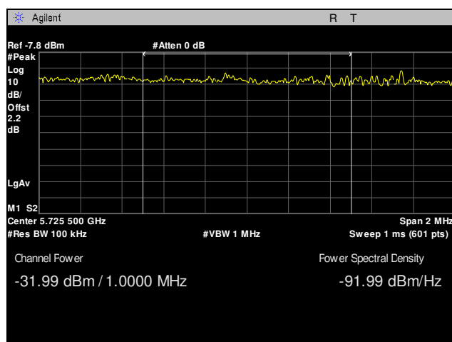
Plot 81. Radiated Band Edge, 5705 MHz, 10 MHz, Peak Integration
