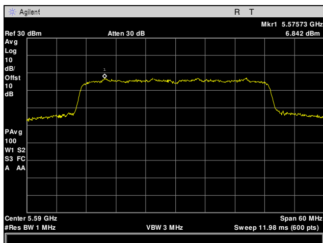
Plot 52. Maximum Power Spectral Density, 5590 MHz, 40 MHz, Channel 0
