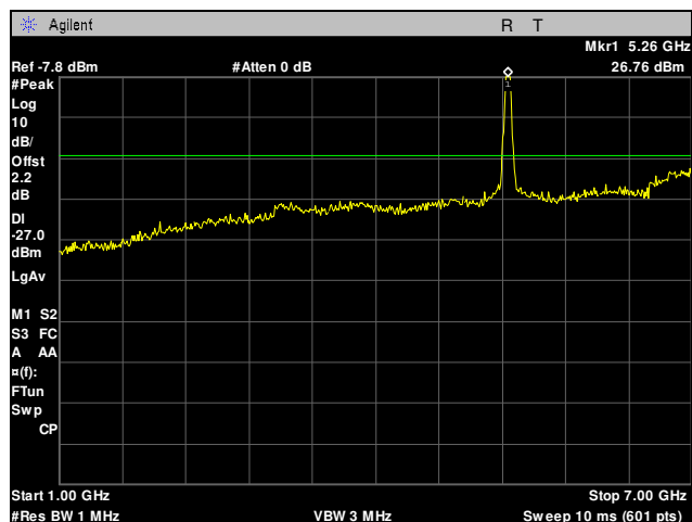
Plot 60. Radiated Spurious Emissions, 5260 MHz, 20 MHz, 1 GHz – 7 GHz
