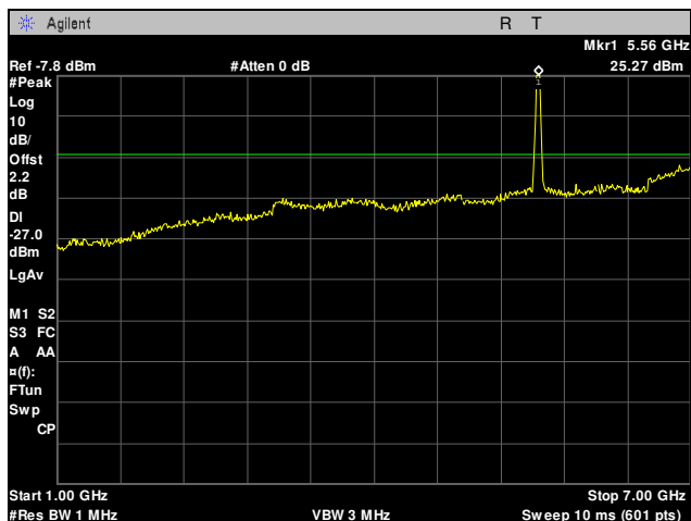
Plot 58. Radiated Spurious Emissions, 5555 MHz, 10 MHz, 1 GHz – 7 GHz
