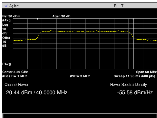
Plot 34. Maximum Conducted Output Power, 5590 MHz, 40 MHz, Channel 0
