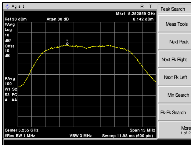
Plot 36. Maximum Power Spectral Density, 5255 MHz, 10 MHz, Channel 0
