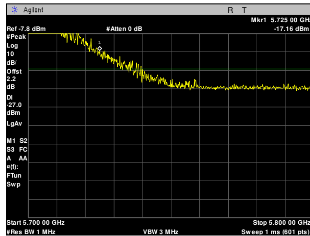
Plot 92. Radiated Band Edge, 5700 MHz, 20 MHz, -27 Peak
