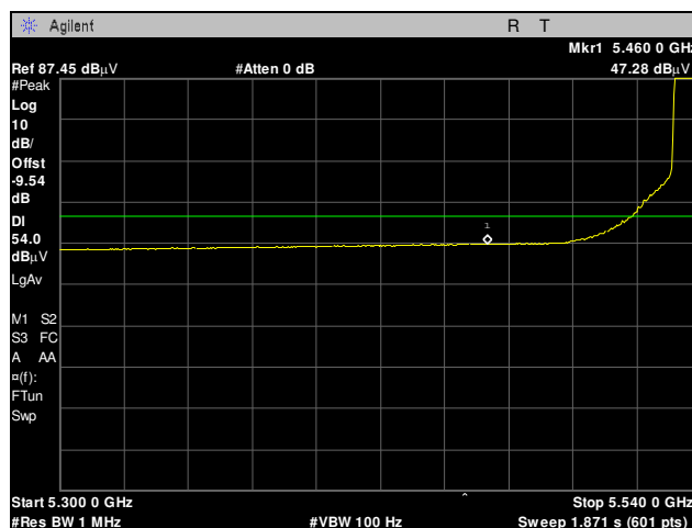
Plot 87. Radiated Band Edge, 5540 MHz, 20 MHz, Average
