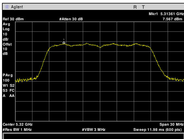
Plot 44. Maximum Power Spectral Density, 5320 MHz, 20 MHz, Channel 0
