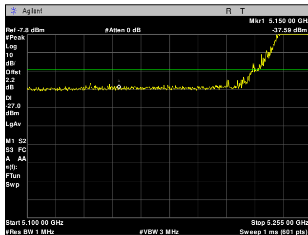
Plot 74. Radiated Band Edge, 5255 MHz, 10 MHz, Peak
