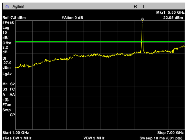
Plot 57. Radiated Spurious Emissions, 5495 MHz, 10 MHz, 1 GHz – 7 GHz
