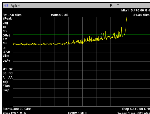
Plot 100. Radiated Band Edge, 5510 MHz, 40 MHz, -27 Peak
