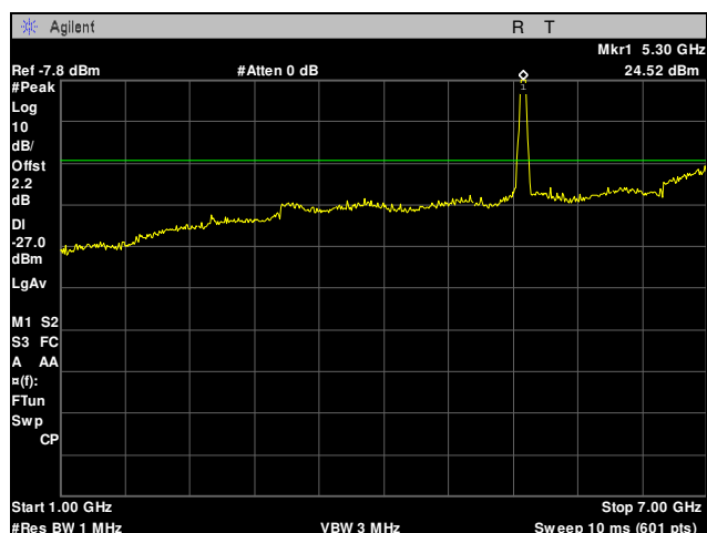
Plot 61. Radiated Spurious Emissions, 5300 MHz, 20 MHz, 1 GHz – 7 GHz
