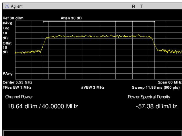
Plot 33. Maximum Conducted Output Power, 5550 MHz, 40 MHz, Channel 0
