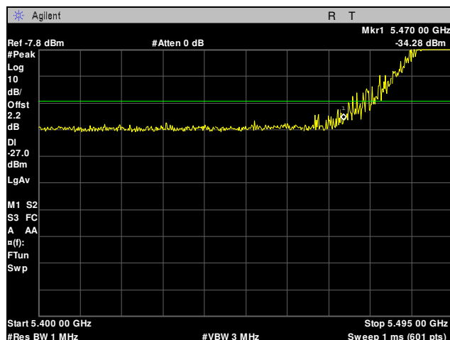
Plot 79. Radiated Band Edge, 5495 MHz, 10 MHz, -27 Peak
