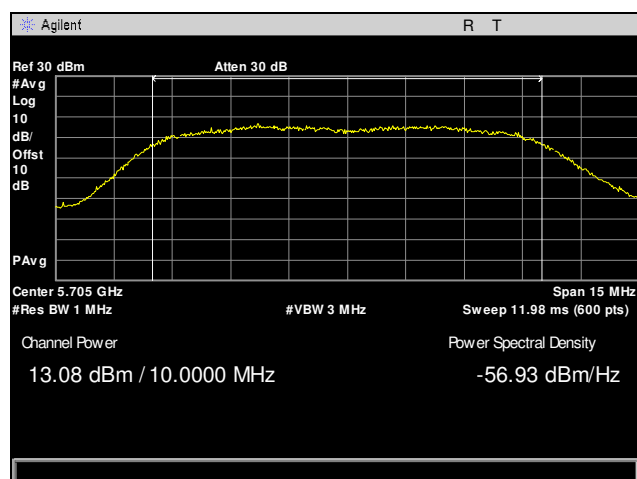
Plot 23. Maximum Conducted Output Power, 5705 MHz, 10 MHz, Channel 0
