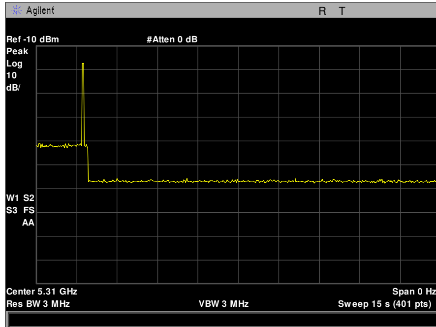
Plot 108. Channel Move Time, 40 MHz
