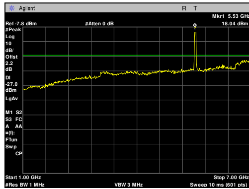
Plot 61. Radiated Spurious Emissions, 5540 MHz, 20 MHz, 1 GHz – 7 GHz
