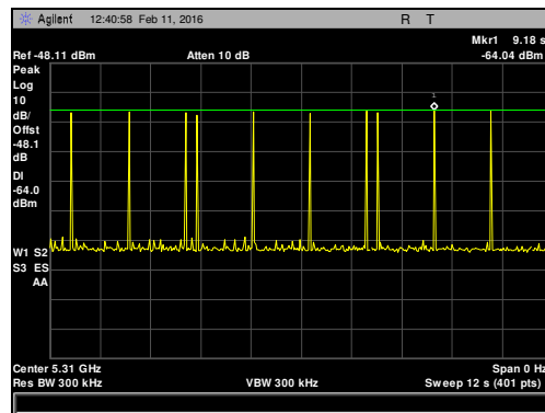
Plot 106. Radar Waveform Calibration, Type 5, 5310 MHz, -13 dBm
