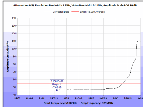
Plot 71. Radiated Band Edge, 5255 MHz, 10 MHz, Average
