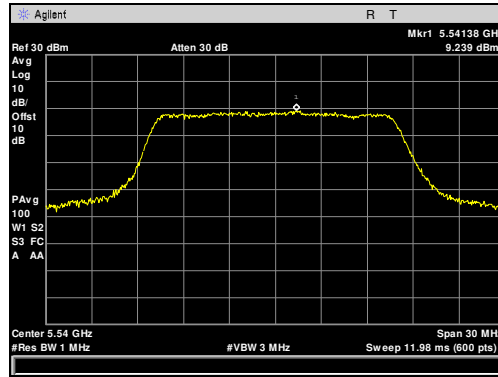
Plot 44. Maximum Power Spectral Density, 5540 MHz, 20 MHz
