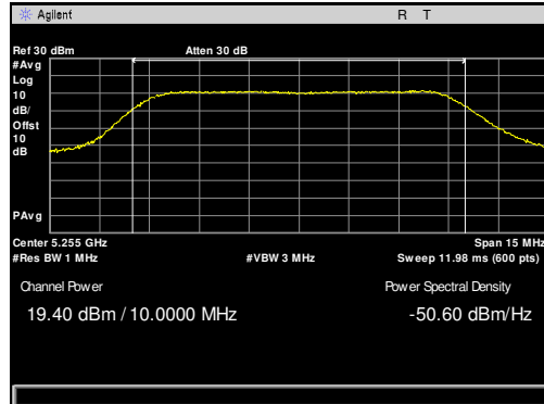
Plot 18. Maximum Conducted Output Power, 5255 MHz, 10 MHz
