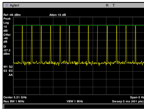
Plot 112. Radar Waveform Calibration, Type 4, 5510 MHz, 4.5 dBm
