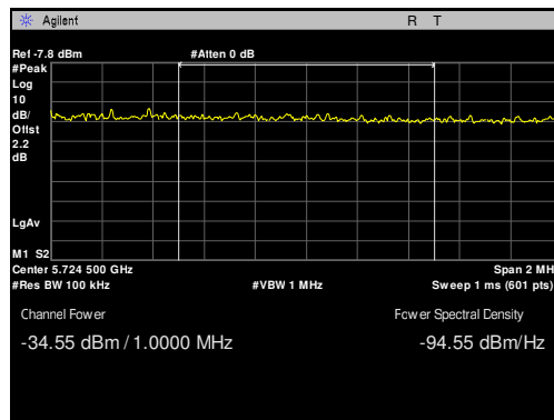
Plot 87. Radiated Band Edge, 5700 MHz, 20 MHz, Peak Integration
