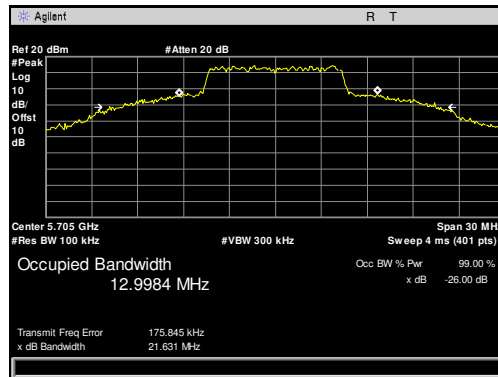
Plot 6. Occupied Bandwidth, 5705 MHz, 10 MHz
