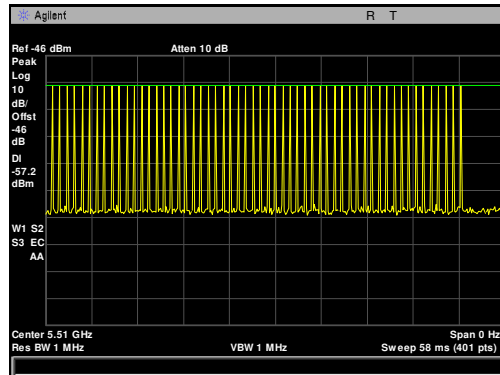
Plot 109. Radar Waveform Calibration, Type 1, 5510 MHz, 6.5 dBm
