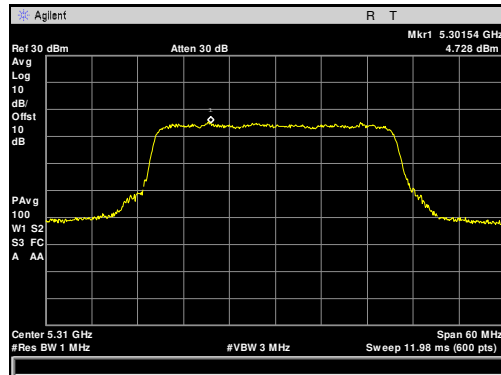
Plot 48. Maximum Power Spectral Density, 5310 MHz, 40 MHz
