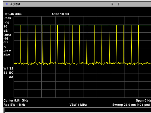
Plot 108. Radar Waveform Calibration, Type 0, 5510 MHz, 6.5 dBm
