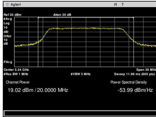
Plot 27. Maximum Conducted Output Power, 5540 MHz, 20 MHz
