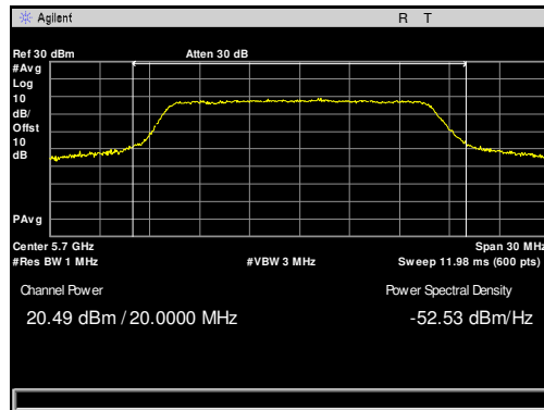
Plot 29. Maximum Conducted Output Power, 5700 MHz, 20 MHz
