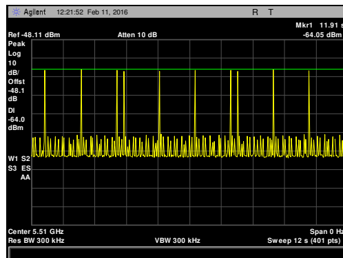
Plot 113. Radar Waveform Calibration, Type 5, 5510 MHz, -11 dBm
