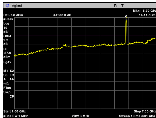
Plot 63. Radiated Spurious Emissions, 5700 MHz, 20 MHz, 1 GHz – 7 GHz
