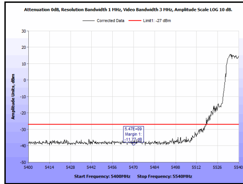
Plot 86. Radiated Band Edge, 5540 MHz, 20 MHz, -27 Peak
