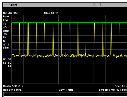
Plot 105. Radar Waveform Calibration, Type 4, 5310 MHz, 4.5 dBm
