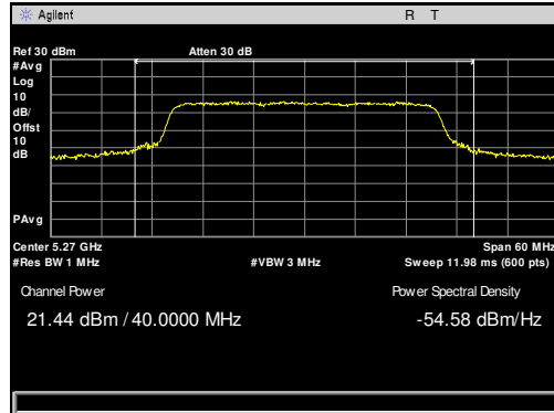
Plot 30. Maximum Conducted Output Power, 5270 MHz, 40 MHz
