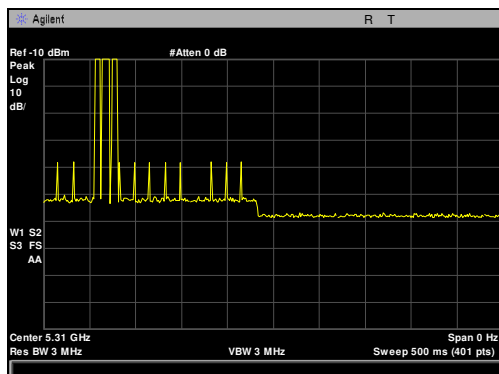
Plot 119. Channel Close Time, 40 MHz
