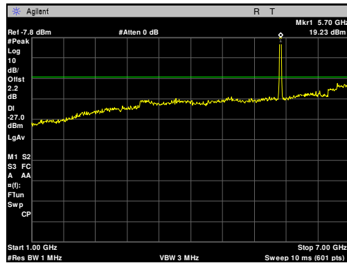
Plot 56. Radiated Spurious Emissions, 5695 MHz, 10 MHz, 1 GHz – 7 GHz
