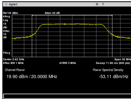
Plot 28. Maximum Conducted Output Power, 5620 MHz, 20 MHz
