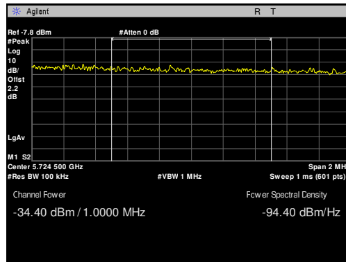
Plot 78. Radiated Band Edge, 5705 MHz, 10 MHz, Peak Integration
