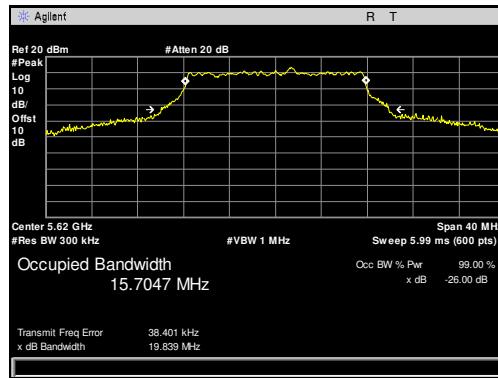
Plot 11. Occupied Bandwidth, 5620 MHz, 20 MHz
