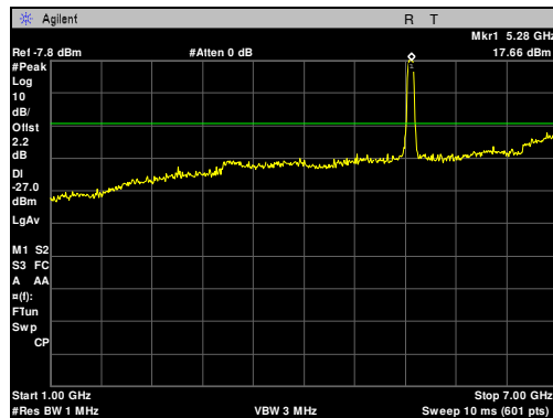
Plot 65. Radiated Spurious Emissions, 5270 MHz, 40 MHz, 1 GHz – 7 GHz
