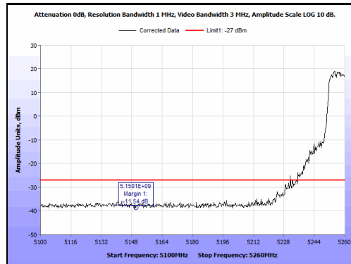
Plot 81. Radiated Band Edge, 5260 MHz, 20 MHz, Peak
