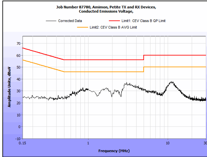
Plot 100. Conducted Emission, Neutral Line Plot
