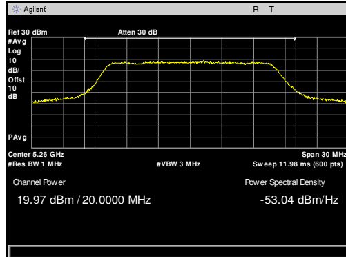
Plot 24. Maximum Conducted Output Power, 5260 MHz, 20 MHz
