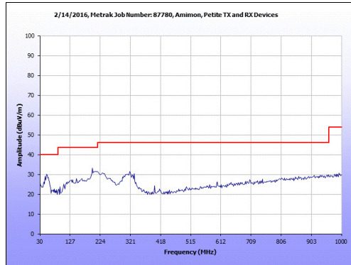
Plot 64. Radiated Spurious Emissions, Low Channel, 40 MHz, 30 MHz – 1 GHz
