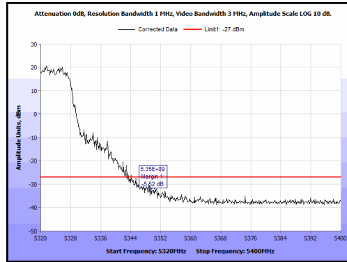
Plot 83. Radiated Band Edge, 5350 MHz, 20 MHz, Peak
