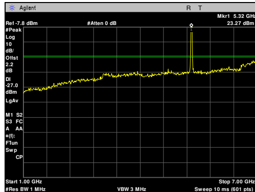
Plot 54. Radiated Spurious Emissions, 5325 MHz, 10 MHz, 1 GHz – 7 GHz
