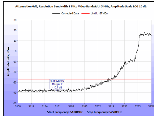
Plot 90. Radiated Band Edge, 5270 MHz, 40 MHz, Peak
