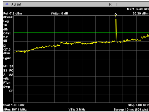
Plot 55. Radiated Spurious Emissions, 5495 MHz, 10 MHz, 1 GHz – 7 GHz
