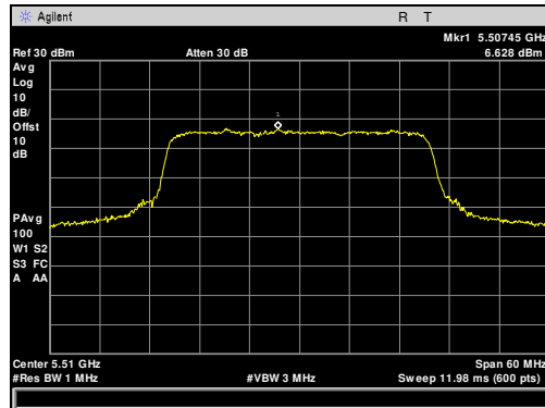
Plot 49. Maximum Power Spectral Density, 5510 MHz, 40 MHz
