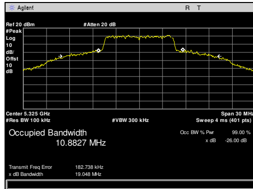
Plot 3. Occupied Bandwidth, 5325 MHz, 10 MHz
