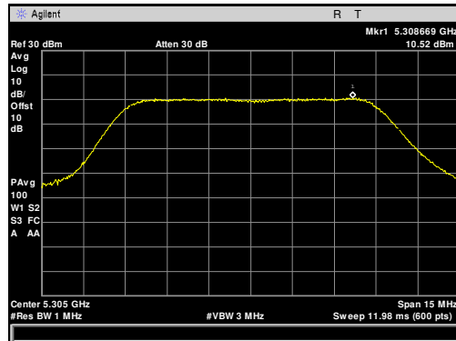
Plot 36. Maximum Power Spectral Density, 5305 MHz, 10 MHz
