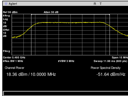
Plot 21. Maximum Conducted Output Power, 5495 MHz, 10 MHz
