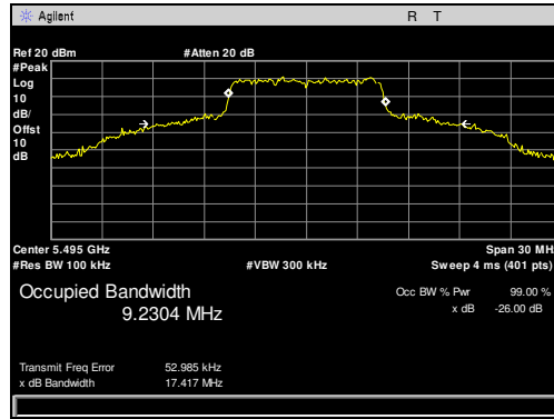
Plot 4. Occupied Bandwidth, 5495 MHz, 10 MHz
