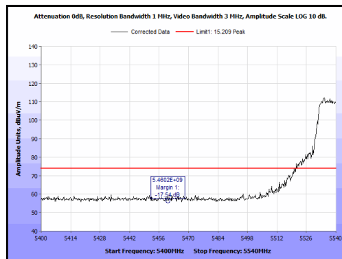
Plot 85. Radiated Band Edge, 5540 MHz, 20 MHz, Peak
