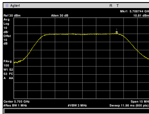
Plot 40. Maximum Power Spectral Density, 5705 MHz, 10 MHz
