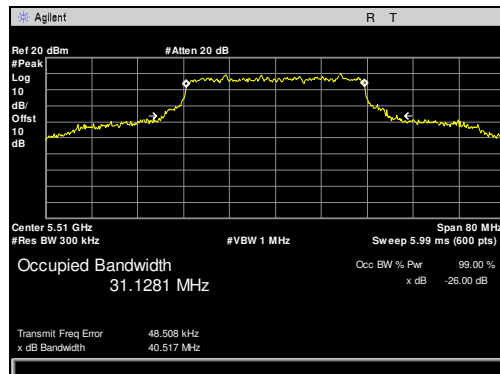
Plot 15. Occupied Bandwidth, 5510 MHz, 40 MHz
