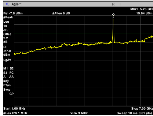
Plot 58. Radiated Spurious Emissions, 5260 MHz, 20 MHz, 1 GHz – 7 GHz
