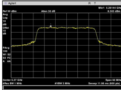
Plot 47. Maximum Power Spectral Density, 5270 MHz, 40 MHz
