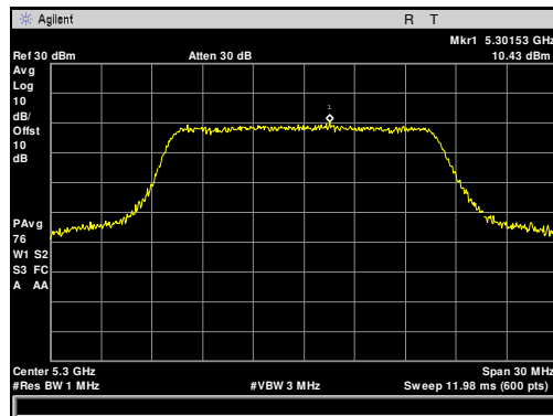
Plot 42. Maximum Power Spectral Density, 5300 MHz, 20 MHz
