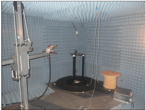
Photograph 2. Radiated Emissions, Test Setup Above 1GHz
