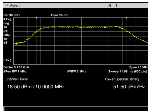
Plot 23. Maximum Conducted Output Power, 5705 MHz, 10 MHz
