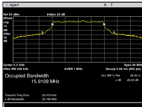
Plot 8. Occupied Bandwidth, 5300 MHz, 20 MHz
