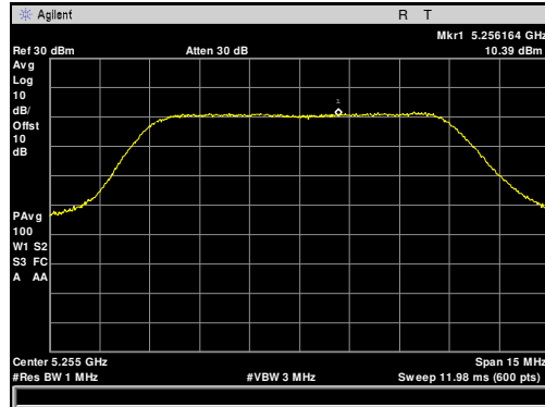
Plot 35. Maximum Power Spectral Density, 5255 MHz, 10 MHz
