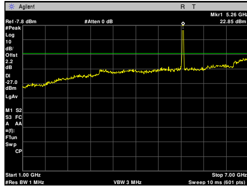
Plot 52. Radiated Spurious Emissions, 5255 MHz, 10 MHz, 1 GHz – 7 GHz
