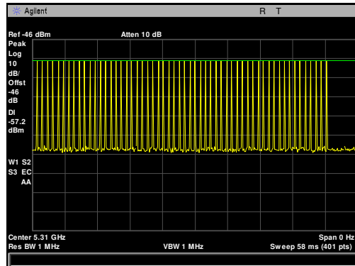
Plot 102. Radar Waveform Calibration, Type 1, 5310 MHz, 6.5 dBm
