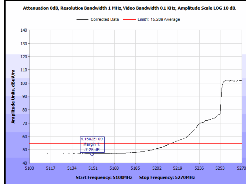
Plot 89. Radiated Band Edge, 5270 MHz, 40 MHz, Average
