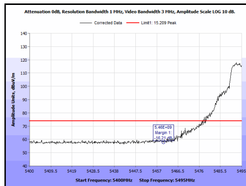
Plot 76. Radiated Band Edge, 5495 MHz, 10 MHz, Peak
