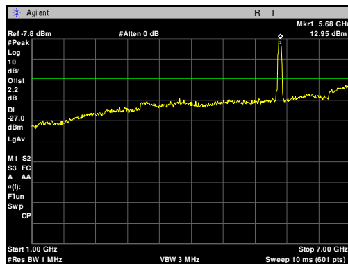
Plot 69. Radiated Spurious Emissions, 5760 MHz, 40 MHz, 1 GHz – 7 GHz
