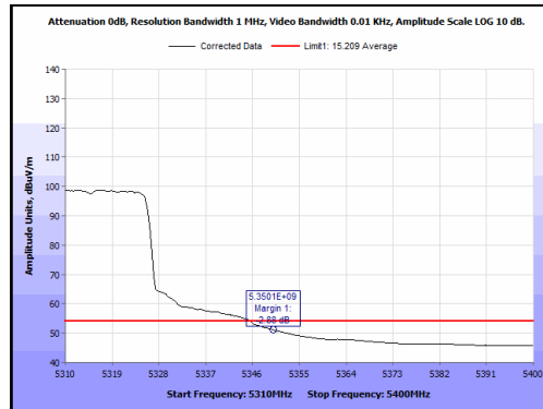
Plot 91. Radiated Band Edge, 5310 MHz, 40 MHz, Average
