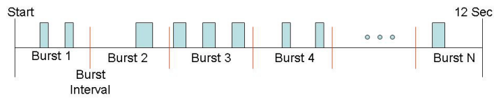
Figure 1. Long Pulse Radar Test Signal Waveform
