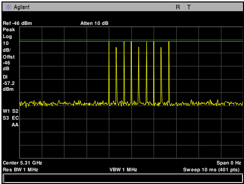
Plot 107. Radar Waveform Calibration, Type 6, 5310 MHz, 6 dBm
