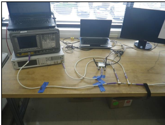
Photograph 4. DFS, Test Setup
