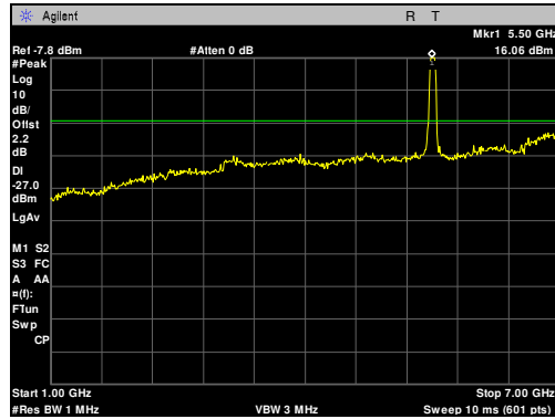
Plot 67. Radiated Spurious Emissions, 5510 MHz, 40 MHz, 1 GHz – 7 GHz
