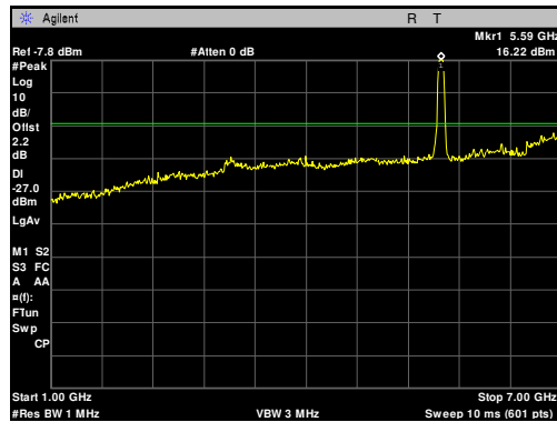
Plot 68. Radiated Spurious Emissions, 5590 MHz, 40 MHz, 1 GHz – 7 GHz
