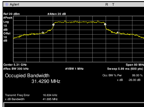
Plot 14. Occupied Bandwidth, 5310 MHz, 40 MHz
