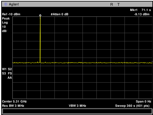
Plot 117. Radar Burst at the End of Channel Availability Check Time, 40 MHz
