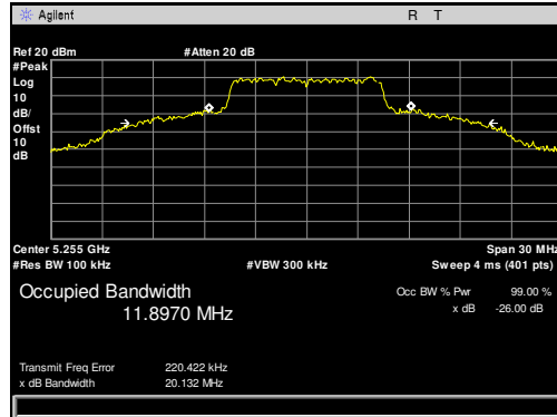
Plot 1. Occupied Bandwidth, 5255 MHz, 10 MHz
