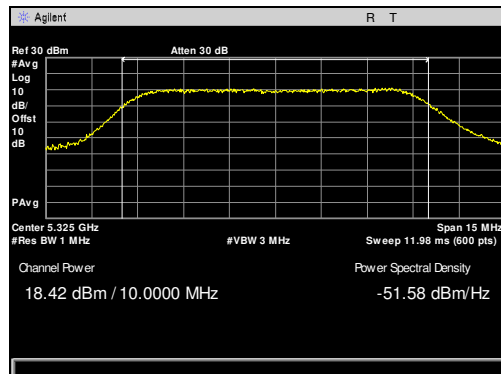
Plot 20. Maximum Conducted Output Power, 5325 MHz, 10 MHz
