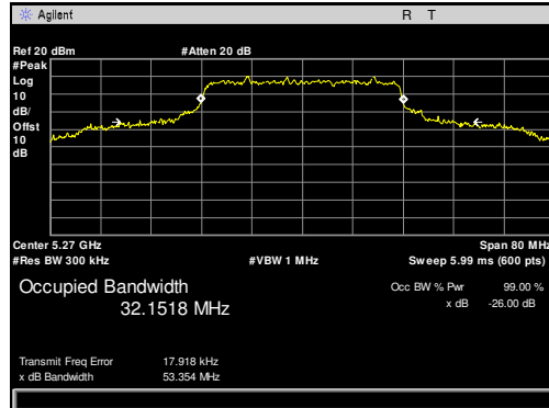
Plot 13. Occupied Bandwidth, 5270 MHz, 40 MHz
