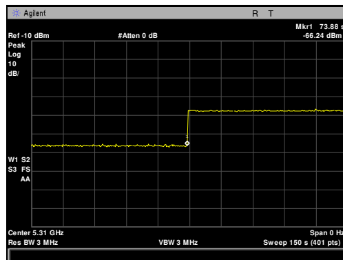
Plot 115. Channel Availability Check Time, 40 MHz
