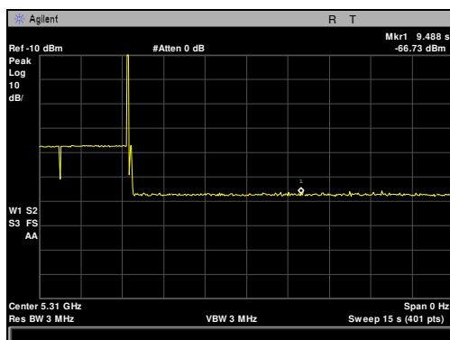
Plot 118. Channel Move Time, 40 MHz
