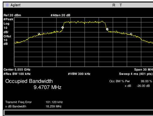
Plot 5. Occupied Bandwidth, 5555 MHz, 10 MHz
