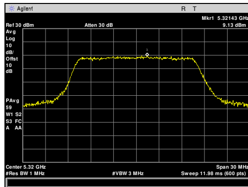
Plot 43. Maximum Power Spectral Density, 5320 MHz, 20 MHz
