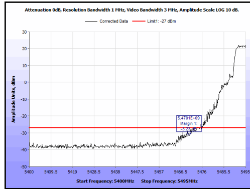
Plot 77. Radiated Band Edge, 5495 MHz, 10 MHz, -27 Peak
