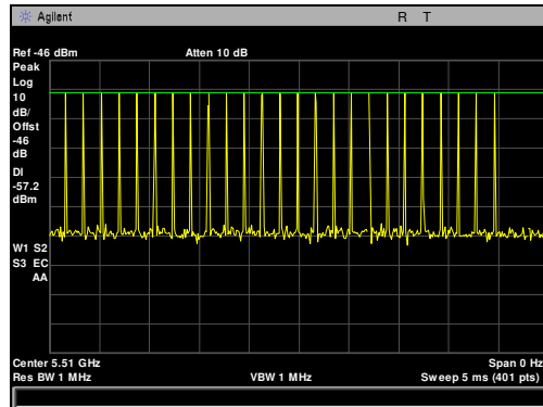
Plot 110. Radar Waveform Calibration, Type 2, 5510 MHz, 4.5 dBm
