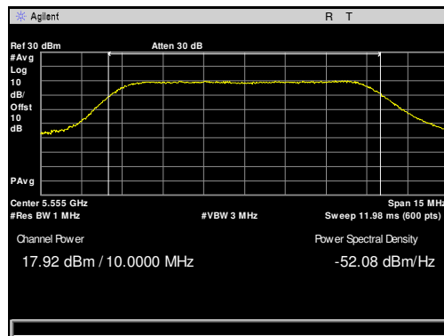
Plot 22. Maximum Conducted Output Power, 5555 MHz, 10 MHz
