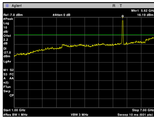
Plot 62. Radiated Spurious Emissions, 5620 MHz, 20 MHz, 1 GHz – 7 GHz
