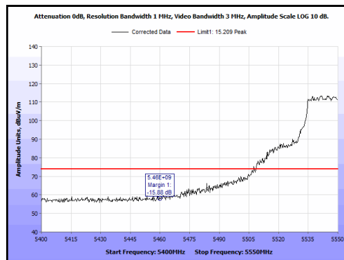
Plot 97. Radiated Band Edge, 5550 MHz, 40 MHz, Peak
