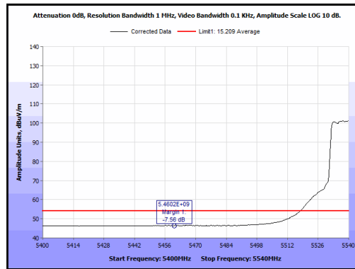
Plot 84. Radiated Band Edge, 5540 MHz, 20 MHz, Average
