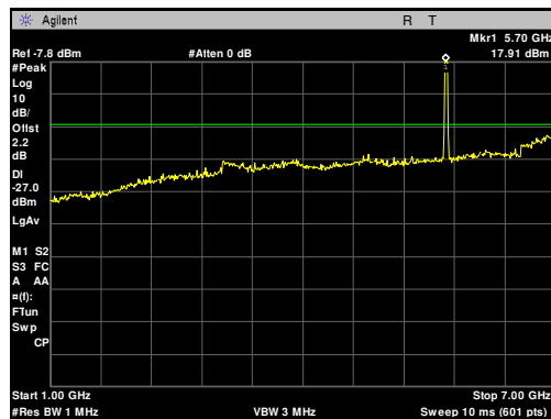
Plot 57. Radiated Spurious Emissions, 5705 MHz, 10 MHz, 1 GHz – 7 GHz
