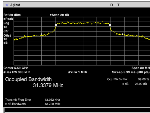
Plot 16. Occupied Bandwidth, 5590 MHz, 40 MHz
