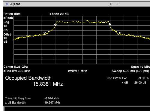
Plot 7. Occupied Bandwidth, 5260 MHz, 20 MHz
