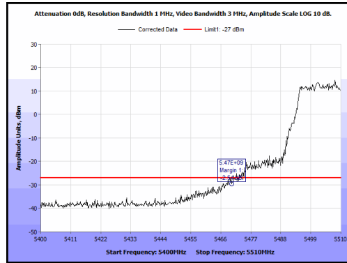
Plot 95. Radiated Band Edge, 5510 MHz, 40 MHz, -27 Peak
