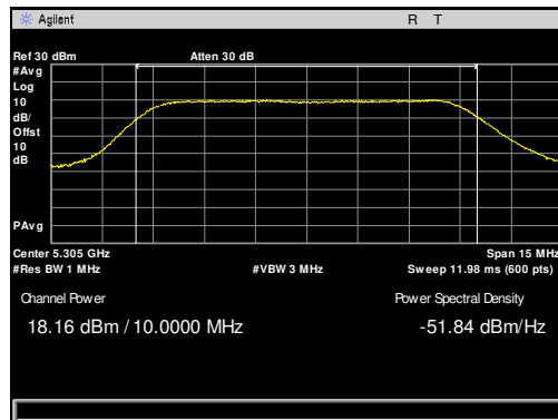
Plot 19. Maximum Conducted Output Power, 5305 MHz, 10 MHz
