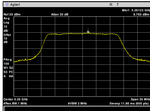
Plot 41. Maximum Power Spectral Density, 5260 MHz, 20 MHz
