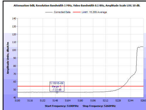
Plot 80. Radiated Band Edge, 5260 MHz, 20 MHz, Average
