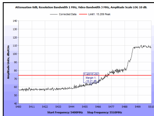
Plot 94. Radiated Band Edge, 5510 MHz, 40 MHz, Peak
