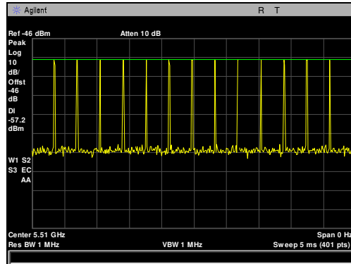
Plot 111. Radar Waveform Calibration, Type 3, 5510 MHz, 4.5 dBm
