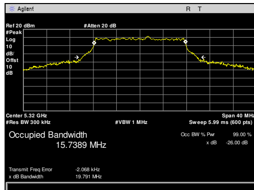
Plot 9. Occupied Bandwidth, 5320 MHz, 20 MHz
