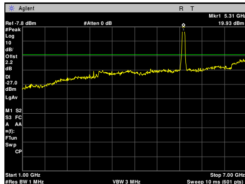
Plot 66. Radiated Spurious Emissions, 5310 MHz, 40 MHz, 1 GHz – 7 GHz
