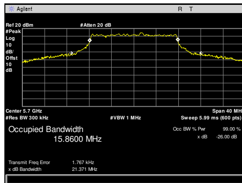
Plot 12. Occupied Bandwidth, 5700 MHz, 20 MHz
