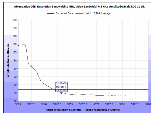
Plot 73. Radiated Band Edge, 5325 MHz, 10 MHz, Average
