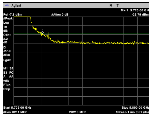
Plot 79. Radiated Band Edge, 5705 MHz, 10 MHz, Peak
