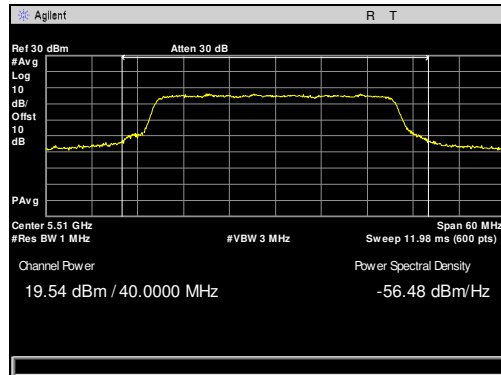
Plot 32. Maximum Conducted Output Power, 5510 MHz, 40 MHz
