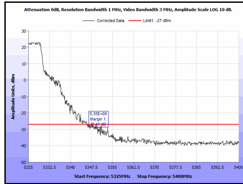
Plot 74. Radiated Band Edge, 5325 MHz, 10 MHz, Peak
