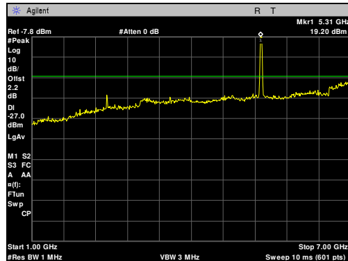
Plot 60. Radiated Spurious Emissions, 5320 MHz, 20 MHz, 1 GHz – 7 GHz
