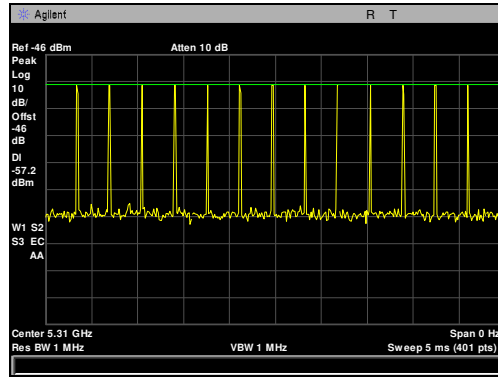
Plot 104. Radar Waveform Calibration, Type 3, 5310 MHz, 4.5 dBm
