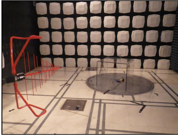
Photograph 1. Radiated Emissions, Test Setup Below 1GHz
