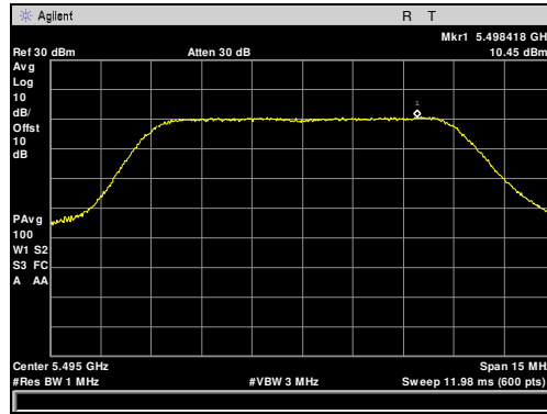
Plot 38. Maximum Power Spectral Density, 5495 MHz, 10 MHz
