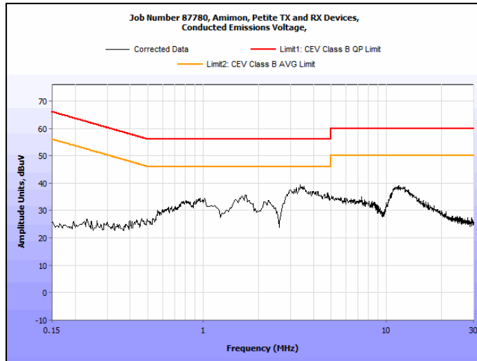
Plot 99. Conducted Emission, Phase Line Plot
