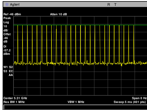
Plot 103. Radar Waveform Calibration, Type 2, 5310 MHz, 5 dBm
