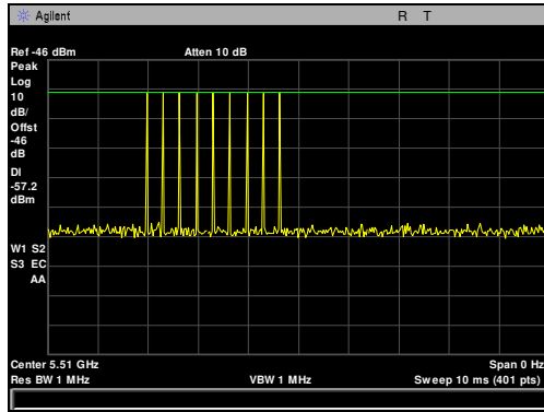
Plot 114. Radar Waveform Calibration, Type 6, 5510 MHz, 6 dBm
