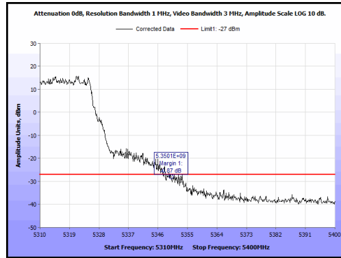
Plot 92. Radiated Band Edge, 5310 MHz, 40 MHz, Peak
