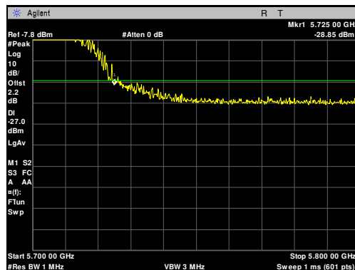
Plot 88. Radiated Band Edge, 5700 MHz, 20 MHz, Peak
