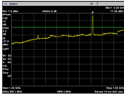
Plot 59. Radiated Spurious Emissions, 5300 MHz, 20 MHz, 1 GHz – 7 GHz
