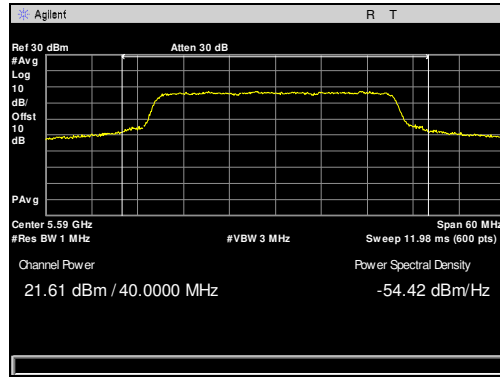
Plot 33. Maximum Conducted Output Power, 5590 MHz, 40 MHz
