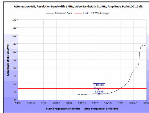
Plot 75. Radiated Band Edge, 5495 MHz, 10 MHz, Average
