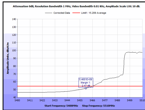
Plot 93. Radiated Band Edge, 5510 MHz, 40 MHz, Average
