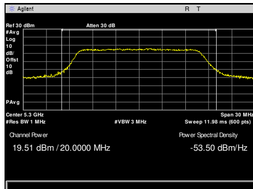
Plot 25. Maximum Conducted Output Power, 5300 MHz, 20 MHz
