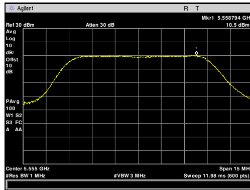
Plot 39. Maximum Power Spectral Density, 5555 MHz, 10 MHz
