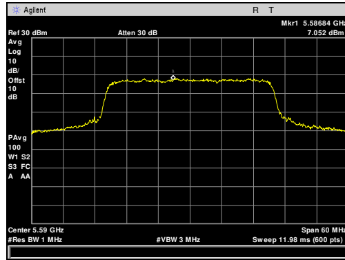
Plot 50. Maximum Power Spectral Density, 5590 MHz, 40 MHz
