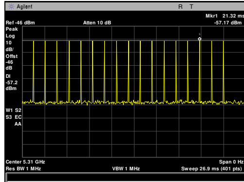
Plot 101. Radar Waveform Calibration, Type 0, 5310 MHz, 6.5 dBm
