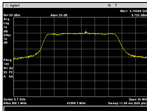
Plot 46. Maximum Power Spectral Density, 5700 MHz, 20 MHz
