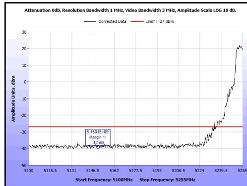
Plot 72. Radiated Band Edge, 5255 MHz, 10 MHz, Peak
