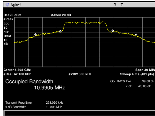
Plot 2. Occupied Bandwidth, 5305 MHz, 10 MHz
