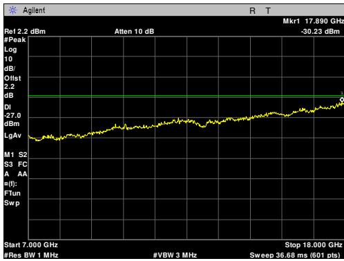
Plot 70. Radiated Spurious Emissions, Low Channel, 40 MHz, 7 GHz – 18 GHz
