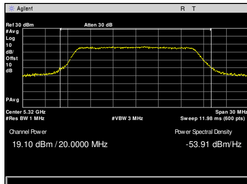
Plot 26. Maximum Conducted Output Power, 5320 MHz, 20 MHz
