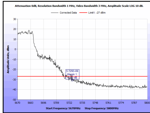
Plot 98. Radiated Band Edge, 5670MHz, 40 MHz, Peak
