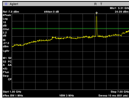
Plot 53. Radiated Spurious Emissions, 5305 MHz, 10 MHz, 1 GHz – 7 GHz
