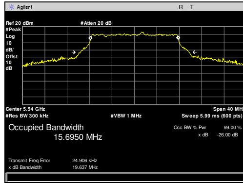
Plot 10. Occupied Bandwidth, 5540 MHz, 20 MHz
