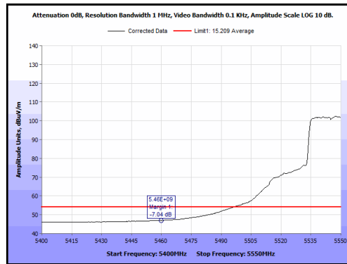
Plot 96. Radiated Band Edge, 5550 MHz, 40 MHz, Average
