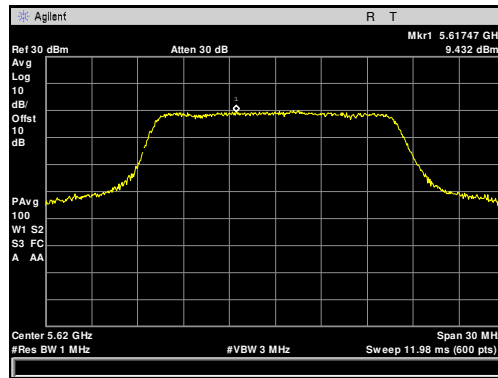
Plot 45. Maximum Power Spectral Density, 5620 MHz, 20 MHz
