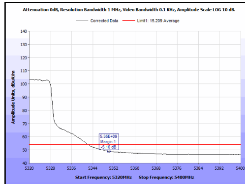
Plot 82. Radiated Band Edge, 5350 MHz, 20 MHz, Average
