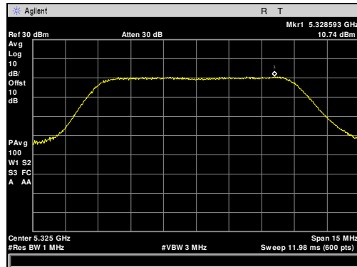
Plot 37. Maximum Power Spectral Density, 5325 MHz, 10 MHz
