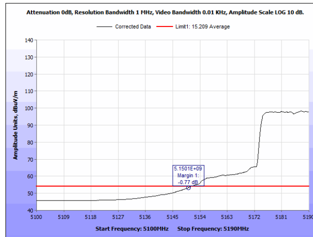
Plot 43. Radiated Band Edge, Low Channel, 40 MHz, Average
