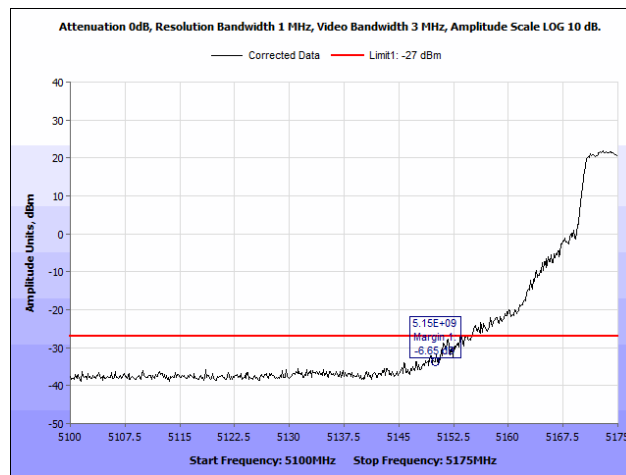
Plot 36. Radiated Band Edge, Low Channel, 10 MHz, Peak
