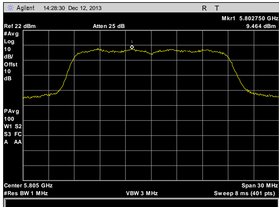
Plot 41. Power Spectral Density, 5805 MHz, 20 MHz, Channel 1
