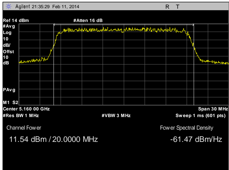
Plot 27. RF Power Output, 5160 MHz, 20 MHz, Channel 1
