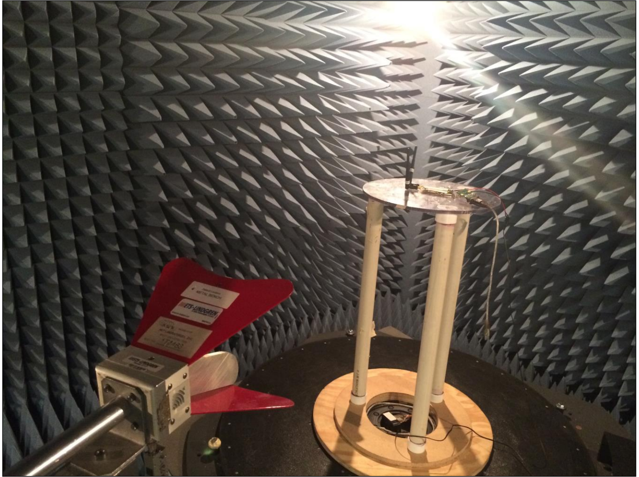
Photograph 4. Radiated Spurious Emissions, Test Setup Above 1 GHz
