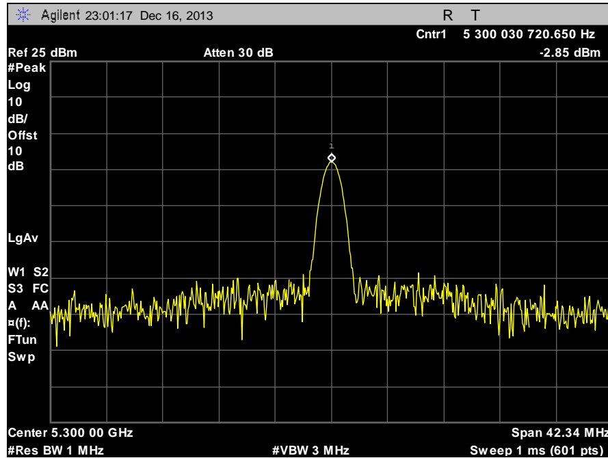
Plot 90. Frequency Stability, 5300 MHz, -20°C, 120 V
