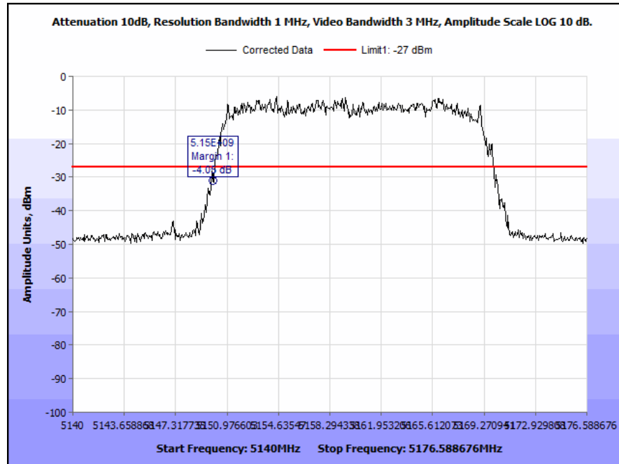
Plot 74. Radiated Restricted Band, 5160 MHz, 20 MHz
