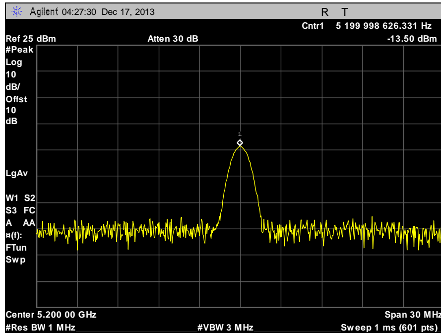
Plot 88. Frequency Stability, 5200 MHz, 50°C, 120 V
