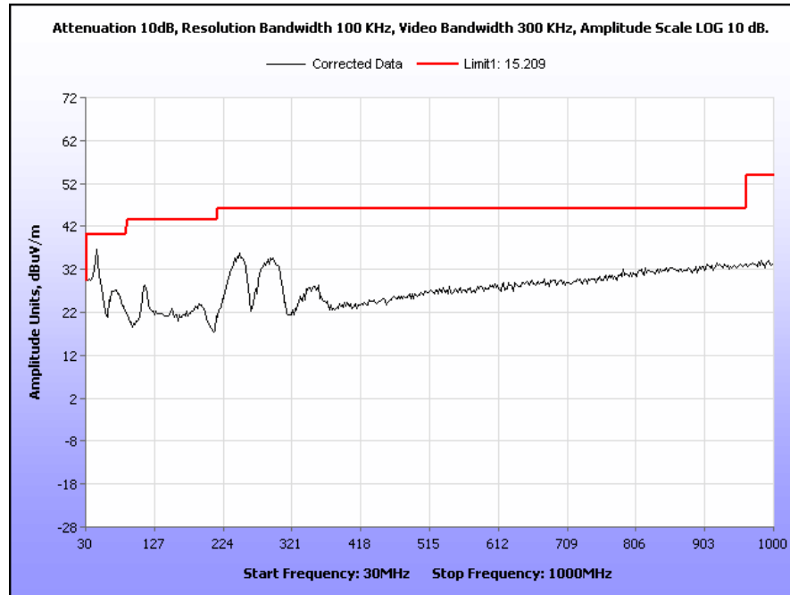
Plot 59. Radiated Spurious Emissions, 5240 MHz, 20 MHz Channel, 30 MHz – 1 GHz
