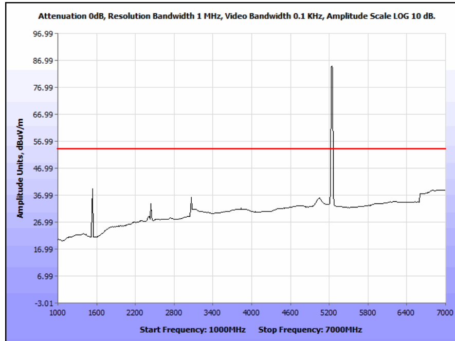
Plot 61. Radiated Spurious Emissions, 5240 MHz, 20 MHz Channel, 1 GHz – 7 GHz, Average
