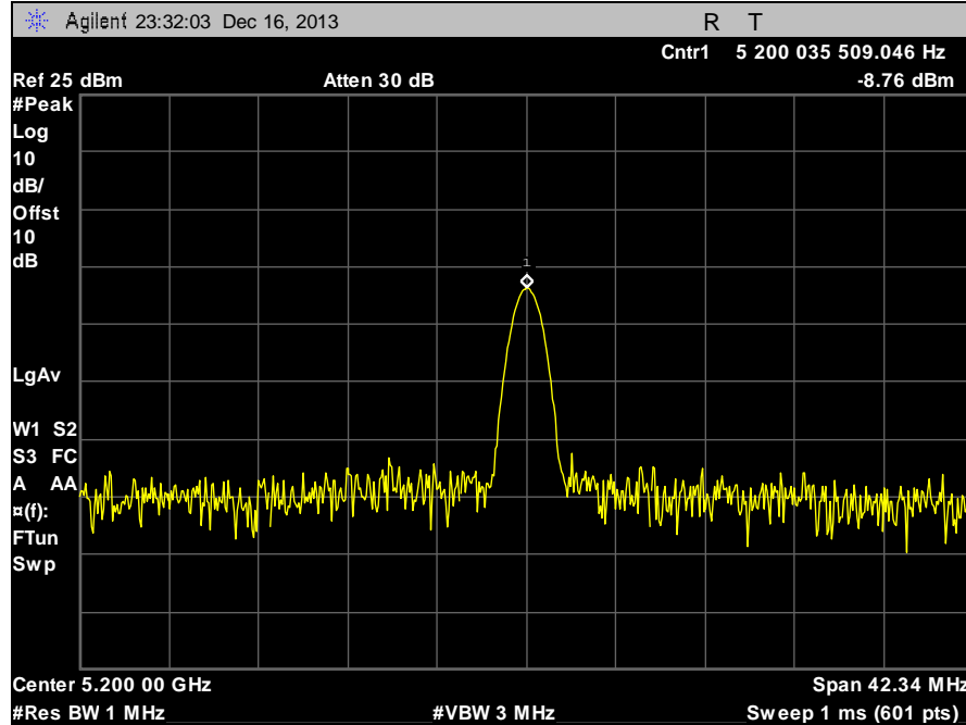
Plot 80. Frequency Stability, 5200 MHz, -10°C, 120 V
