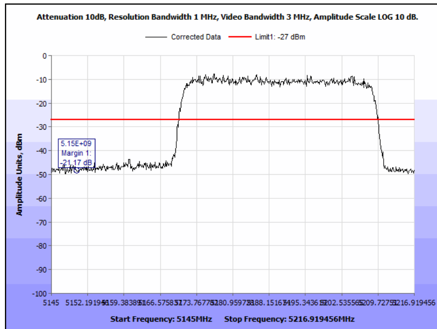
Plot 75. Radiated Restricted Band, 5190 MHz, 40 MHz
