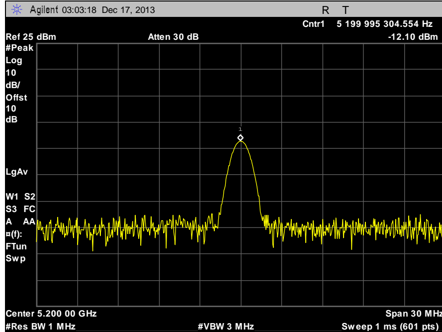
Plot 86. Frequency Stability, 5200 MHz, 30°C, 120 V
