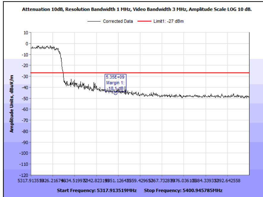
Plot 76. Radiated Restricted Band, 5310 MHz, 40 MHz
