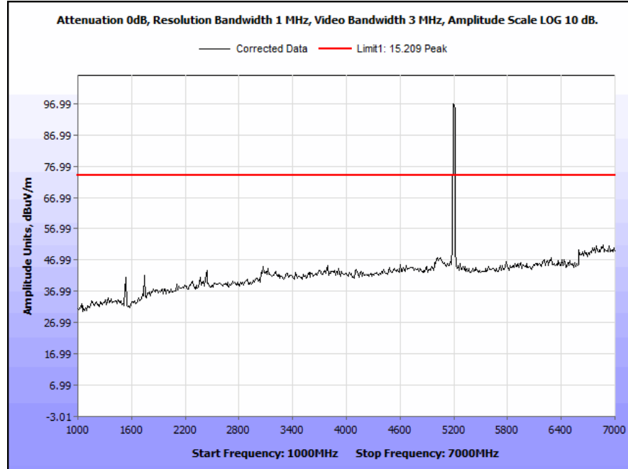
Plot 60. Radiated Spurious Emissions, 5240 MHz, 20 MHz Channel, 1 GHz – 7 GHz, Peak
