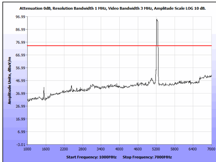
Plot 70. Radiated Spurious Emissions, 5230 MHz, 40 MHz Channel, 1 GHz – 7 GHz, Peak
