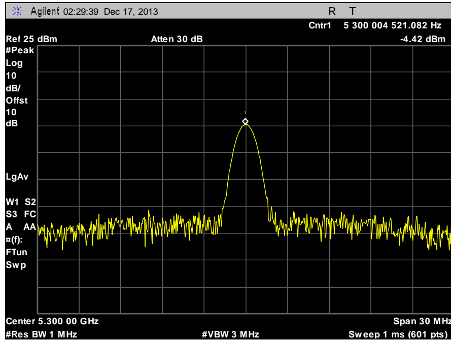
Plot 94. Frequency Stability, 5300 MHz, 20°C, 108V
