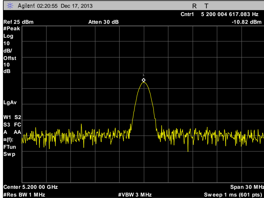
Plot 84. Frequency Stability, 5200 MHz, 20°C, 120 V
