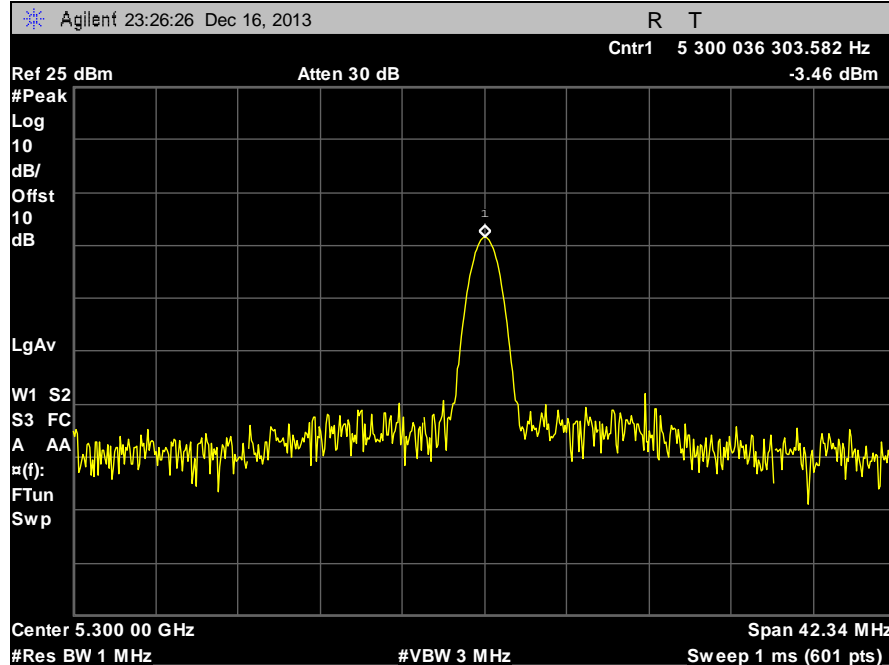
Plot 91. Frequency Stability, 5300 MHz, -10°C, 120 V
