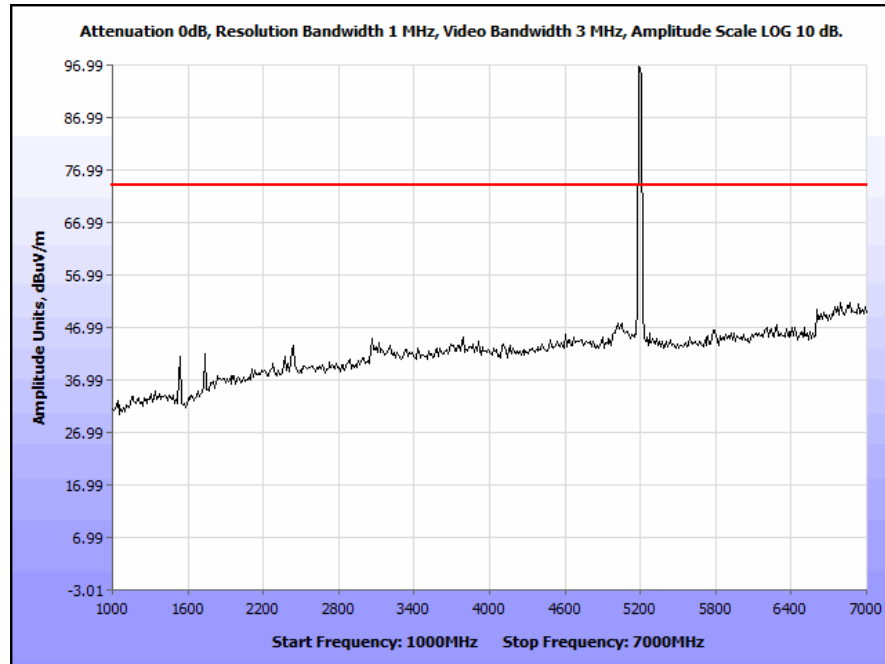
Plot 49. Radiated Spurious Emissions, 5160 MHz, 20 MHz Channel, 1 GHz – 7 GHz, Peak
