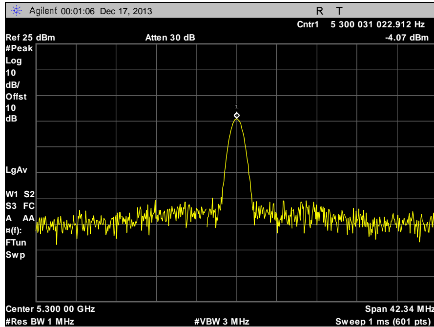
Plot 92. Frequency Stability, 5300 MHz, 0°C, 120 V
