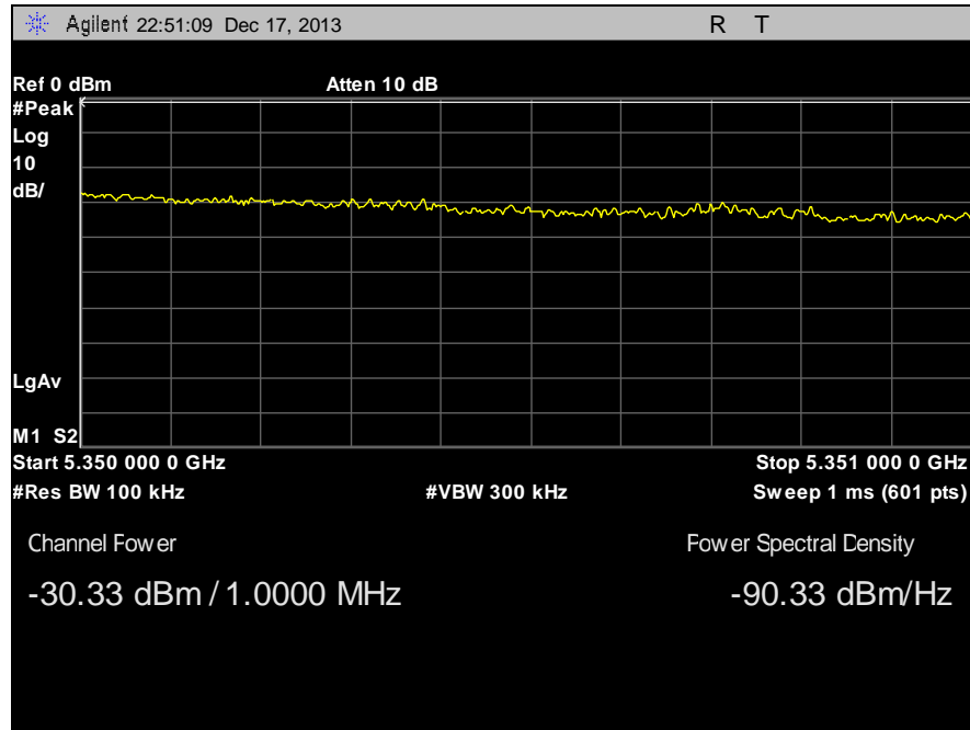
Plot 78. Radiated Restricted Band, 5340 MHz, 20 MHz
