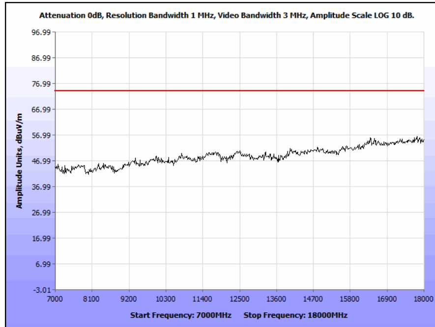
Plot 51. Radiated Spurious Emissions, 5160 MHz, 20 MHz Channel, 7 GHz – 18 GHz, Peak
