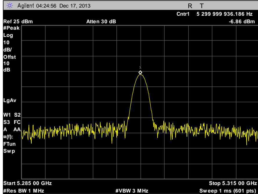
Plot 99. Frequency Stability, 5300 MHz, 50°C, 120 V
