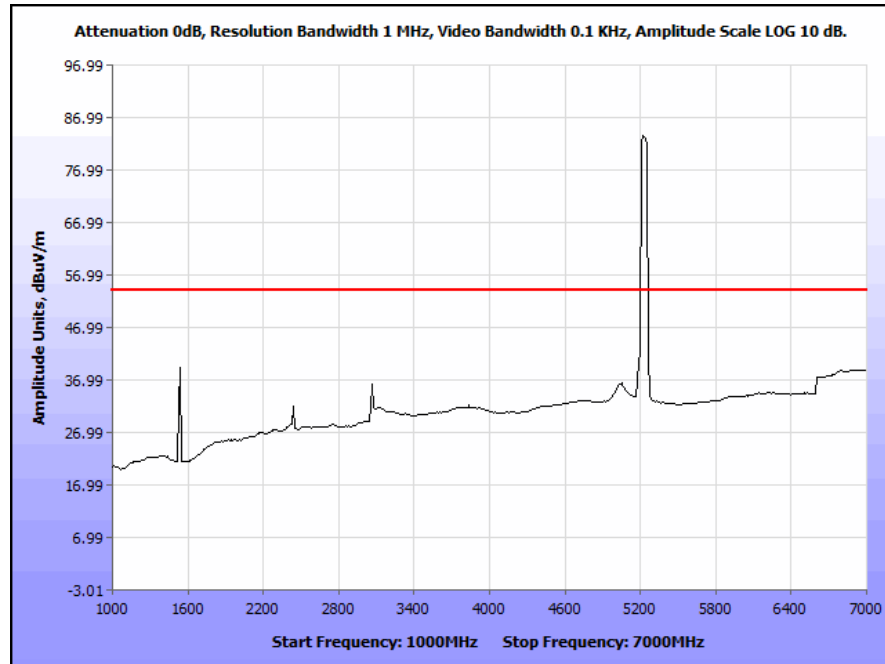
Plot 71. Radiated Spurious Emissions, 5230 MHz, 40 MHz Channel, 1 GHz – 7 GHz, Average
