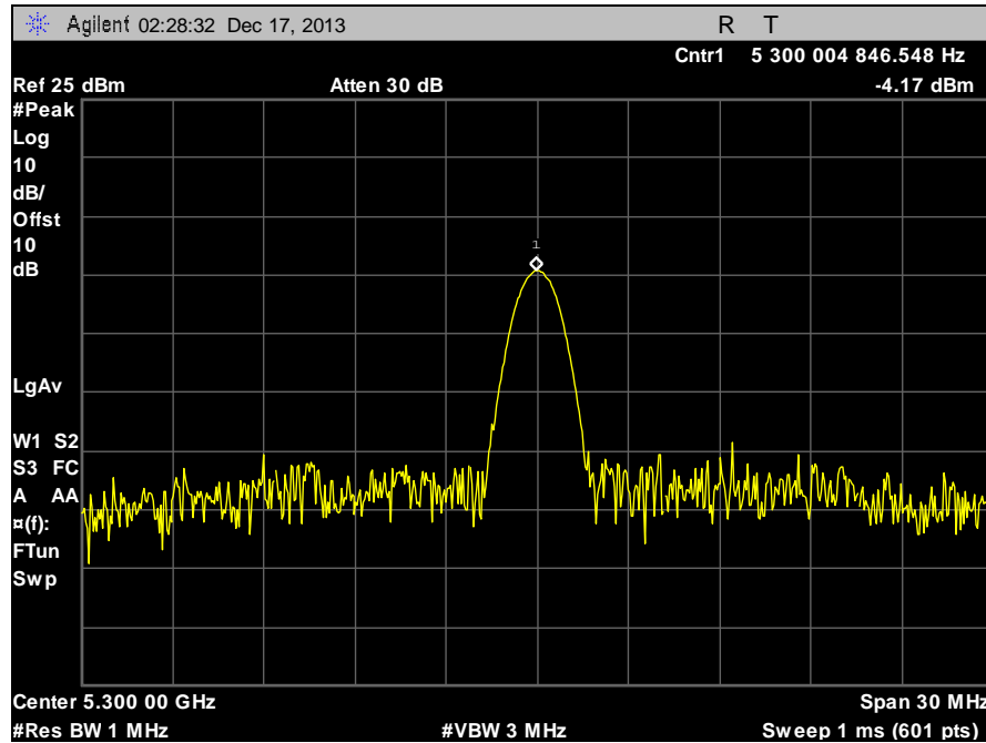
Plot 96. Frequency Stability, 5300 MHz, 20°C, 132 V
