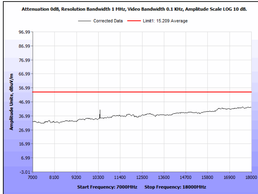
Plot 73. Radiated Spurious Emissions, 5230 MHz, 40 MHz Channel, 7 GHz – 18 GHz, Average
