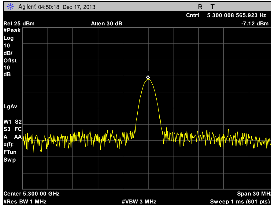
Plot 100. Frequency Stability, 5300 MHz, 55°C, 132 V
