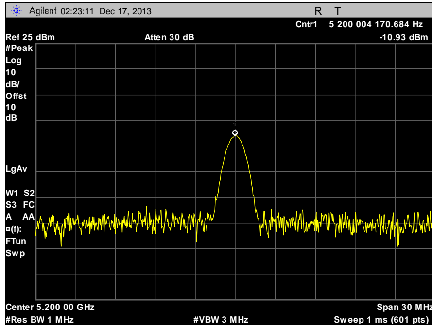
Plot 83. Frequency Stability, 5200 MHz, 20°C, 108V
