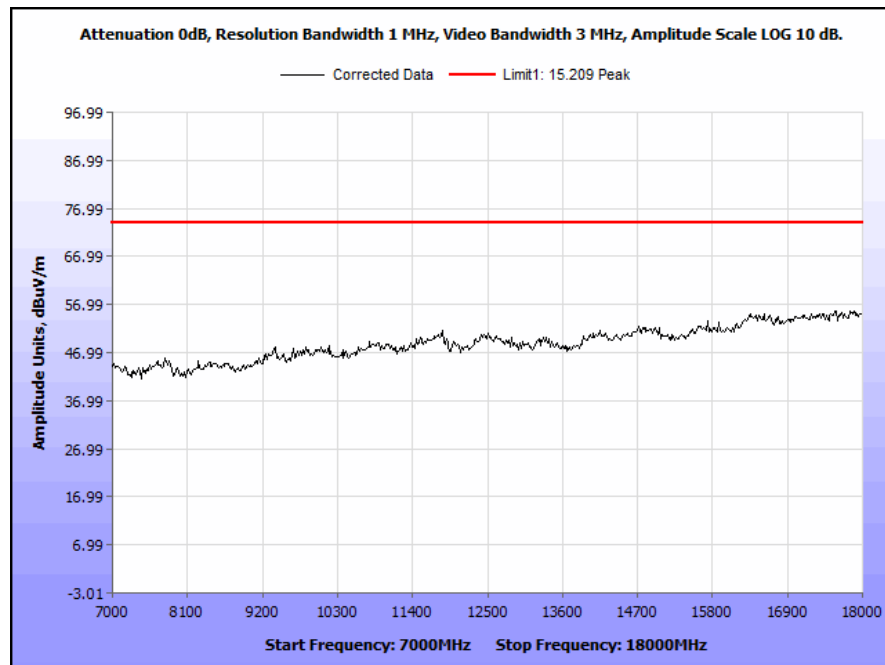
Plot 62. Radiated Spurious Emissions, 5240 MHz, 20 MHz Channel, 7 GHz – 18 GHz, Peak
