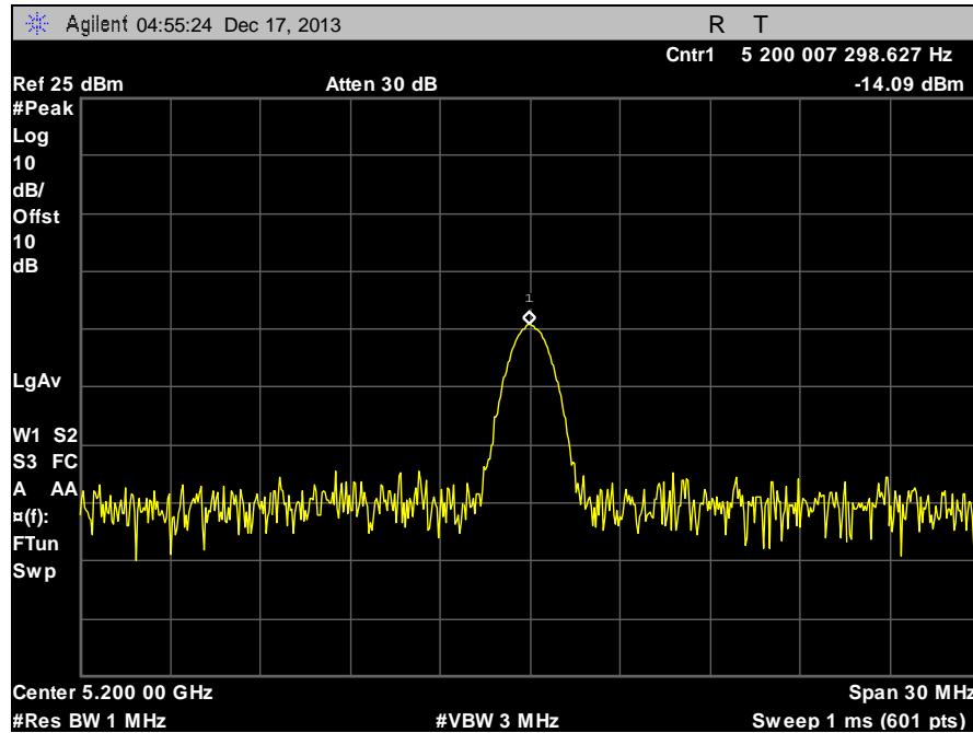
Plot 89. Frequency Stability, 5200 MHz, 55°C, 132 V
