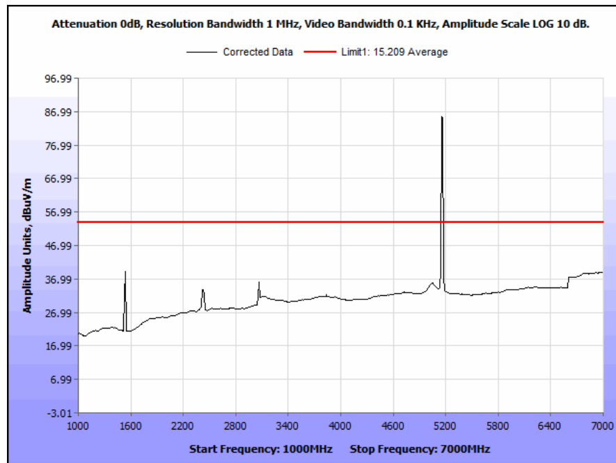
Plot 50. Radiated Spurious Emissions, 5160 MHz, 20 MHz Channel, 1 GHz – 7 GHz, Average
