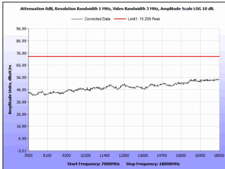
Plot 72. Radiated Spurious Emissions, 5230 MHz, 40 MHz Channel, 7 GHz – 18 GHz, Peak
