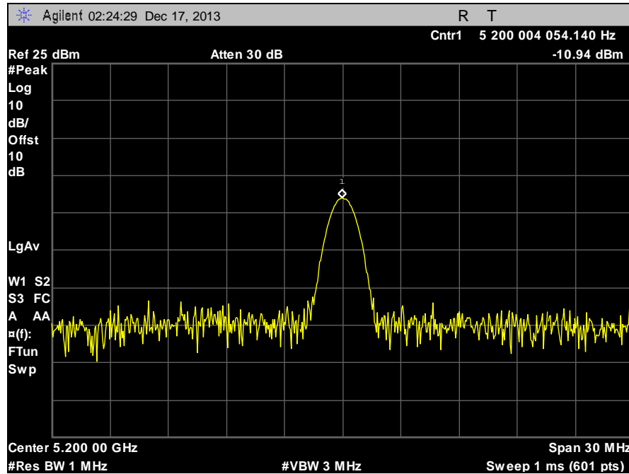
Plot 85. Frequency Stability, 5200 MHz, 20°C, 132 V
