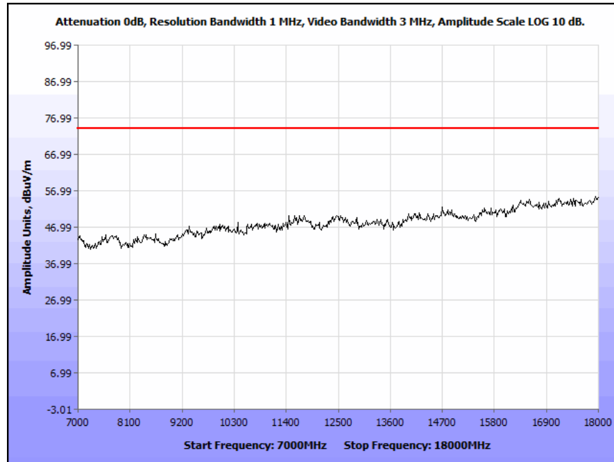
Plot 67. Radiated Spurious Emissions, 5190 MHz, 40 MHz Channel, 7 GHz – 18 GHz, Peak
