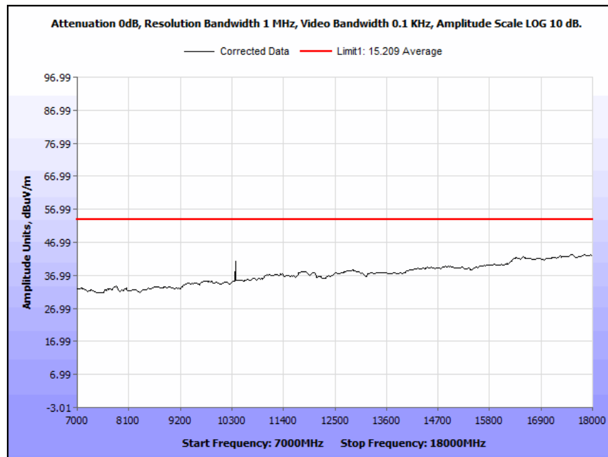
Plot 52. Radiated Spurious Emissions, 5160 MHz, 20 MHz Channel, 7 GHz – 18 GHz, Average
