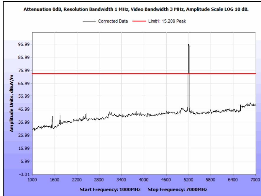
Plot 55. Radiated Spurious Emissions, 5200 MHz, 20 MHz Channel, 1 GHz – 7 GHz, Peak
