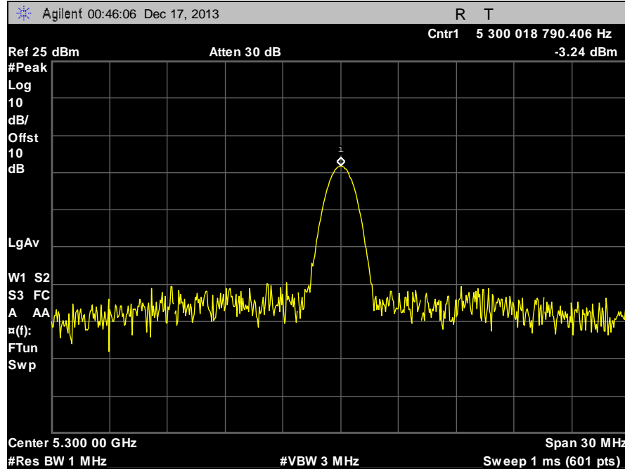
Plot 93. Frequency Stability, 5300 MHz, 10°C, 120 V
