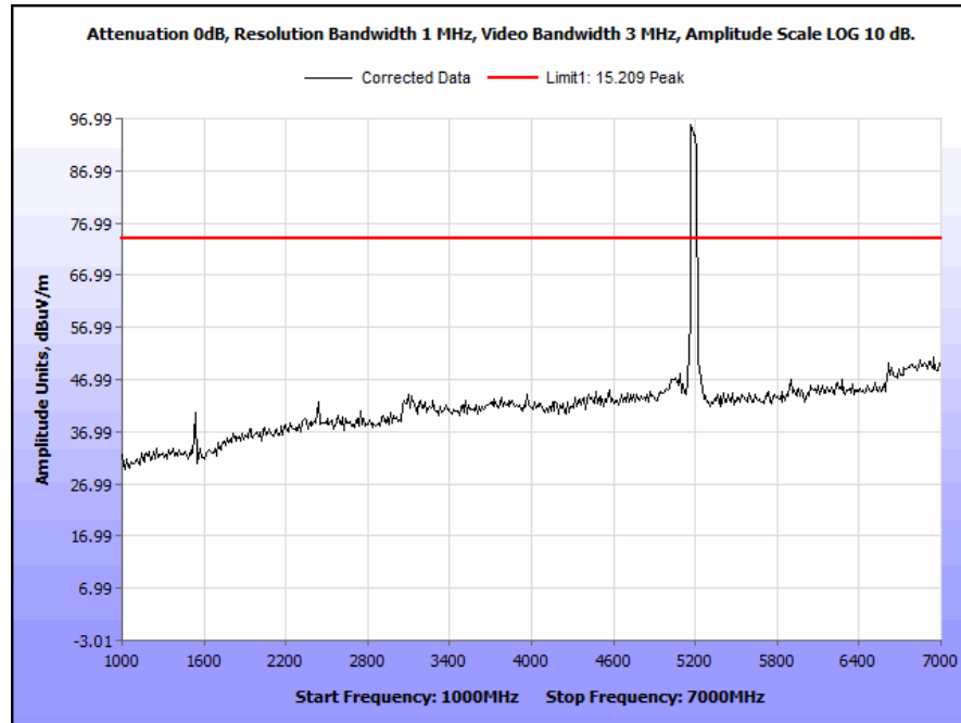
Plot 65. Radiated Spurious Emissions, 5190 MHz, 40 MHz Channel, 1 GHz – 7 GHz, Peak
