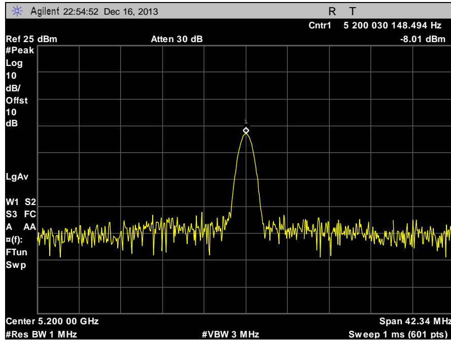
Plot 79. Frequency Stability, 5200 MHz, -20°C, 120 V
