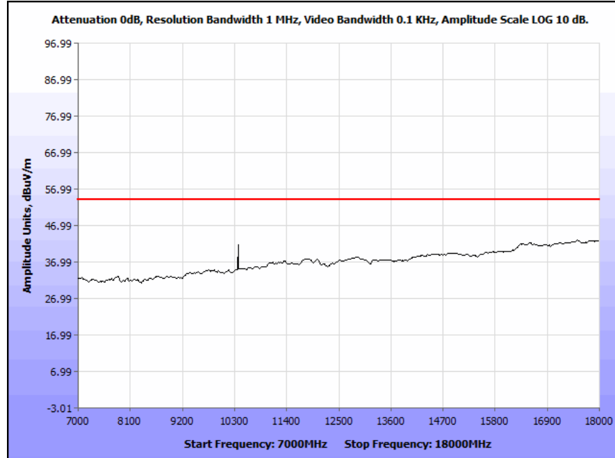
Plot 68. Radiated Spurious Emissions, 5190 MHz, 40 MHz Channel, 7 GHz – 18 GHz, Average
