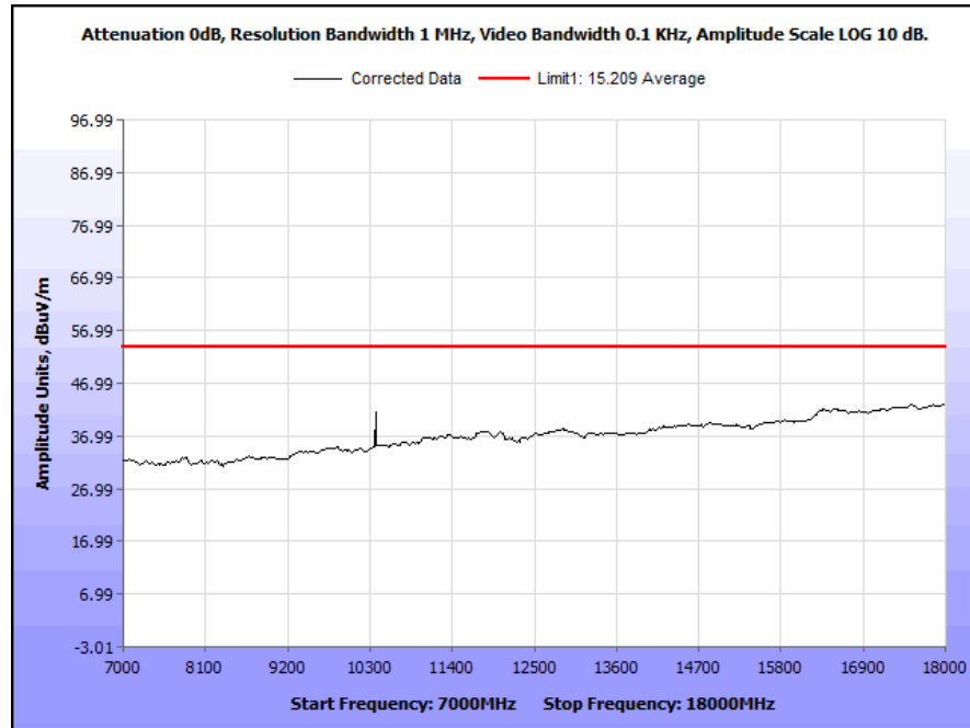
Plot 63. Radiated Spurious Emissions, 5240 MHz, 20 MHz Channel, 7 GHz – 18 GHz, Average
