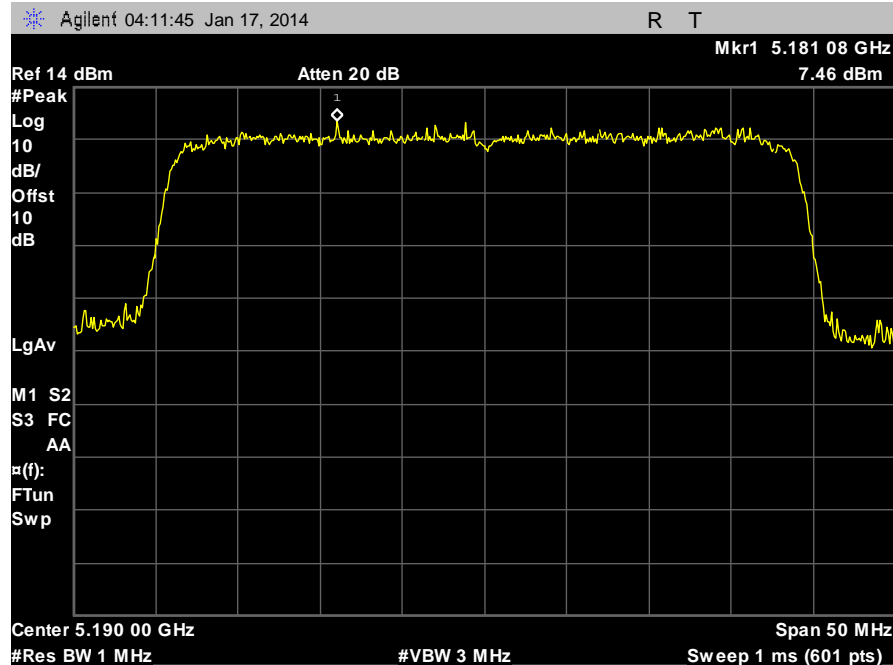
Plot 47. Peak Excursion Ratio, 5190 MHz, 40 MHz
