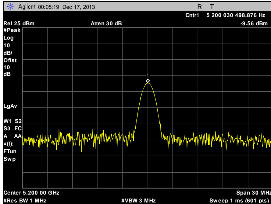
Plot 81. Frequency Stability, 5200 MHz, 0°C, 120 V
