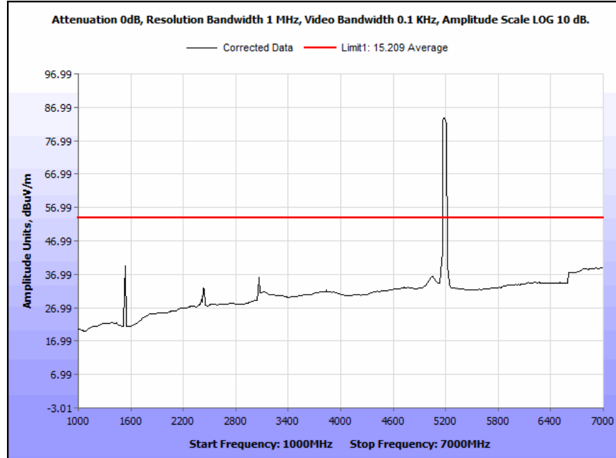
Plot 66. Radiated Spurious Emissions, 5190 MHz, 40 MHz Channel, 1 GHz – 7 GHz, Average
