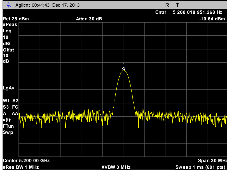
Plot 82. Frequency Stability, 5200 MHz, 10°C, 120 V
