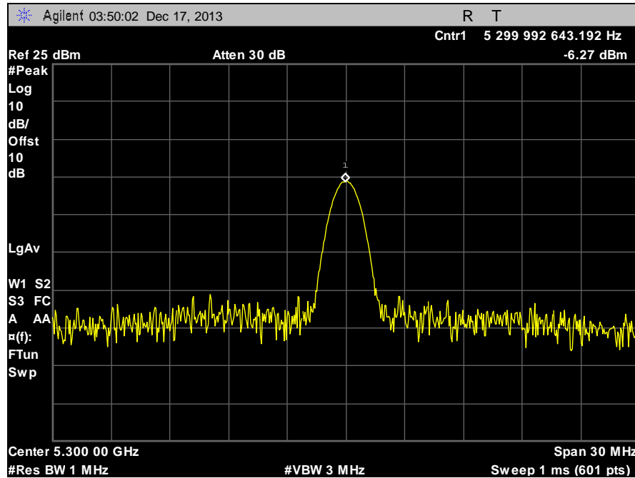
Plot 98. Frequency Stability, 5300 MHz, 40°C, 120 V
