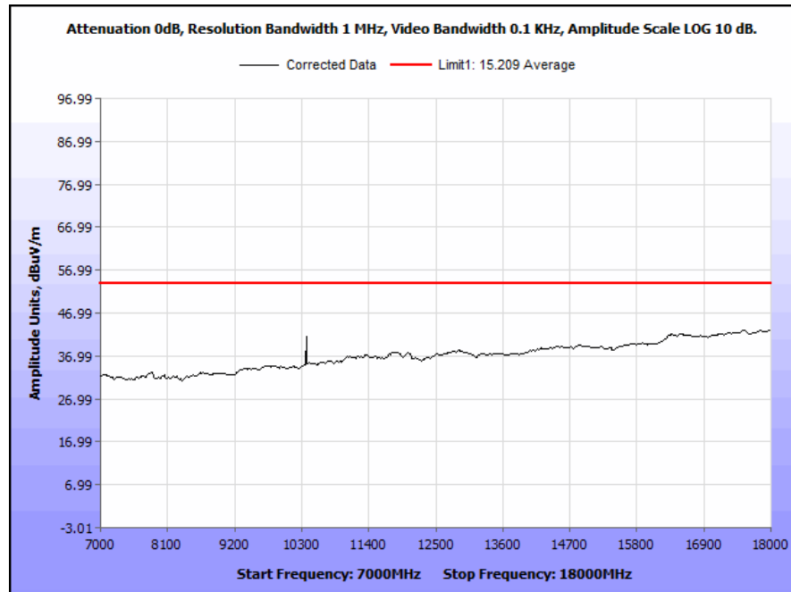
Plot 58. Radiated Spurious Emissions, 5200 MHz, 20 MHz Channel, 7 GHz – 18 GHz, Average
