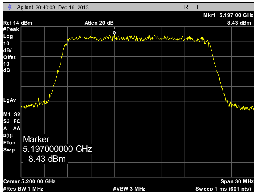
Plot 46. Peak Excursion Ratio, 5200 MHz, 20 MHz
