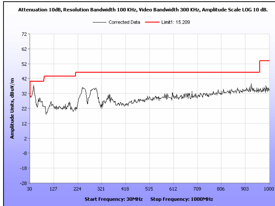
Plot 69. Radiated Spurious Emissions, 5230 MHz, 40 MHz Channel, 30 MHz – 1 GHz
