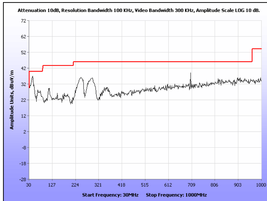
Plot 64. Radiated Spurious Emissions, 5190 MHz, 40 MHz Channel, 30 MHz – 1 GHz
