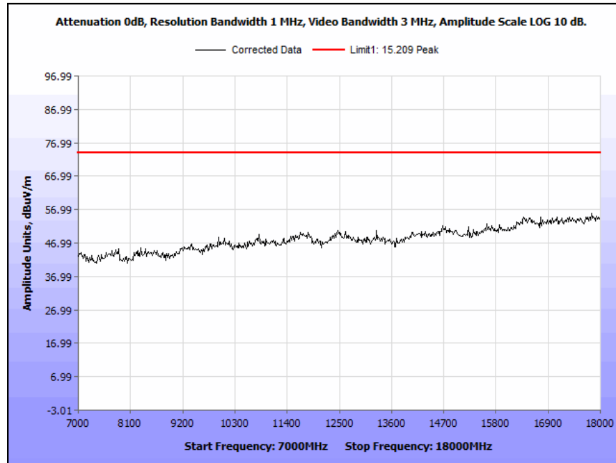
Plot 57. Radiated Spurious Emissions, 5200 MHz, 20 MHz Channel, 7 GHz – 18 GHz, Peak
