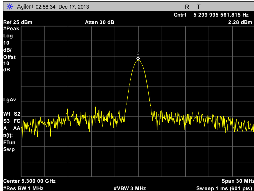
Plot 97. Frequency Stability, 5300 MHz, 30°C, 120 V
