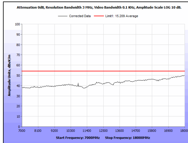
Plot 41. Radiated Spurious Emissions, 40MHz, 7 GHz – 18 GHz, Average
