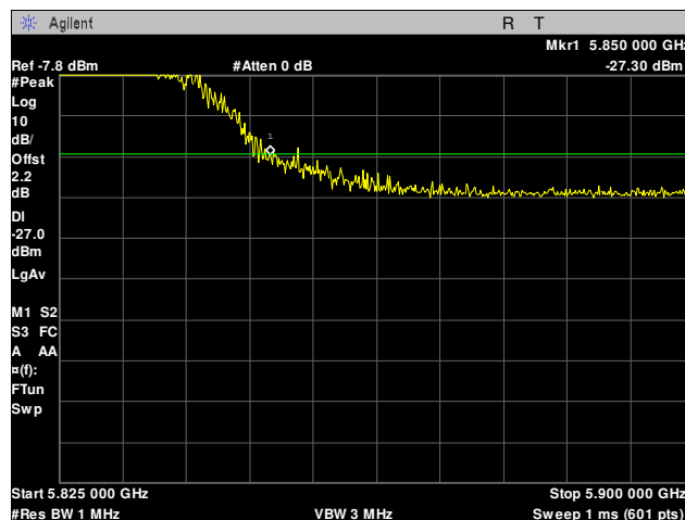
Plot 52. Radiated Band Edge, High Channel, 20 MHz, -27 Peak
