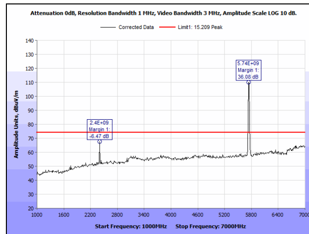
Plot 36. Radiated Spurious Emissions, 5745 MHz, 20 MHz, 1 GHz – 7 GHz, Peak
