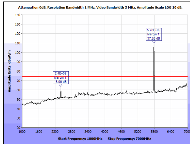
Plot 38. Radiated Spurious Emissions, 5780 MHz, 10 MHz, 1 GHz – 7 GHz, Peak
