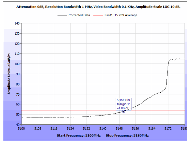
Plot 47. Radiated Band Edge, Low Channel, 20 MHz, Average
