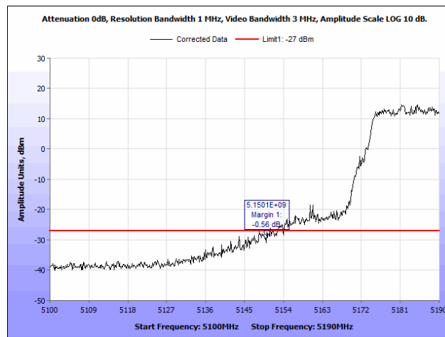
Plot 52. Radiated Band Edge, Low Channel, 40 MHz, Peak
