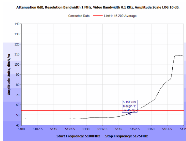
Plot 43. Radiated Band Edge, Low Channel, 10 MHz, Average
