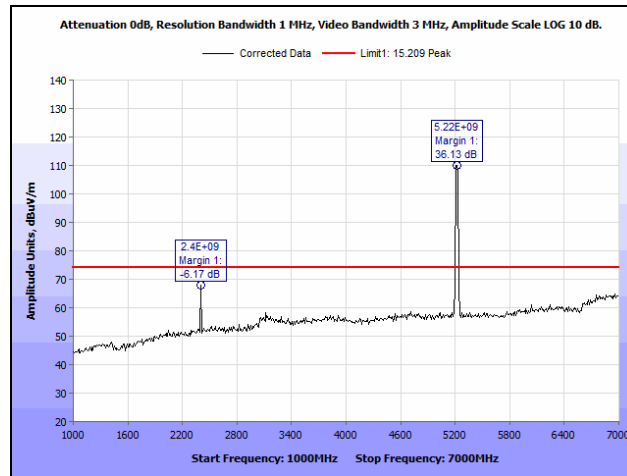
Plot 38. Radiated Spurious Emissions, 5220 MHz, 20 MHz, 1 GHz – 7 GHz, Peak
