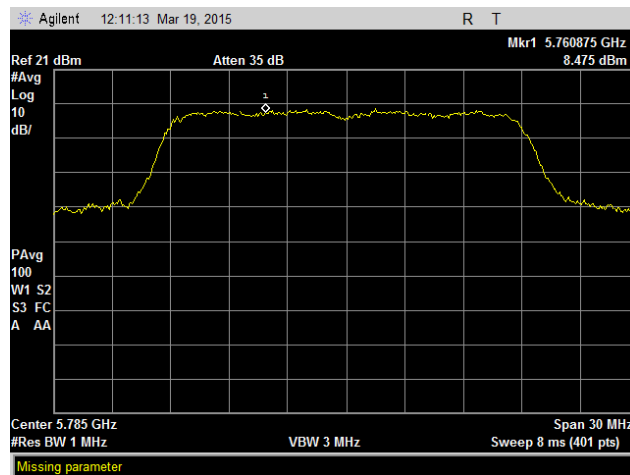
Plot 27. Peak Power Spectral Density, 5785 MHz, Antenna 2
