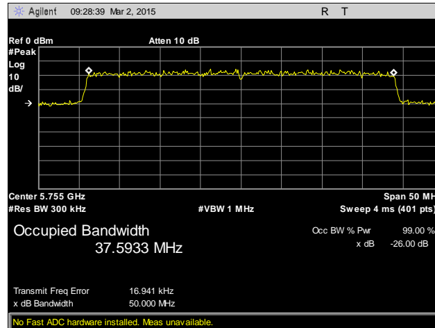
Plot 9. 26 dB Occupied Bandwidth, 5755 MHz, Antenna 2
