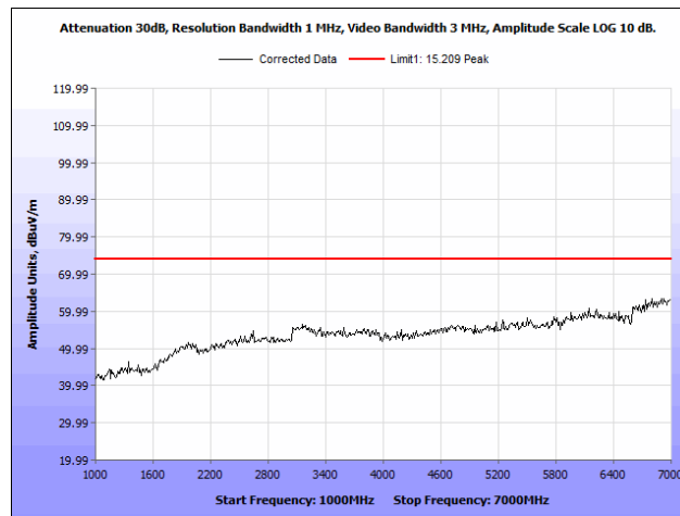
Plot 53. Radiated Spurious Emissions, 5795 MHz, Rubber Ducky Antenna, 1 GHz – 7 GHz, Peak
