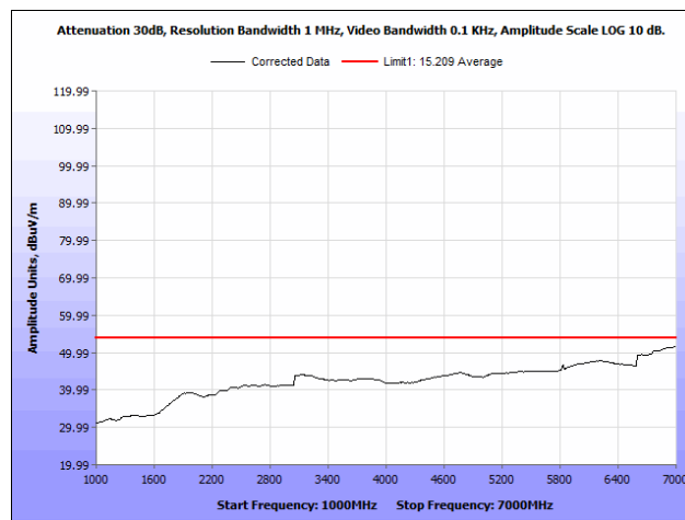
Plot 42. Radiated Spurious Emissions, 5825 MHz, Rubber Ducky Antenna, 1 GHz – 7 GHz, Average
