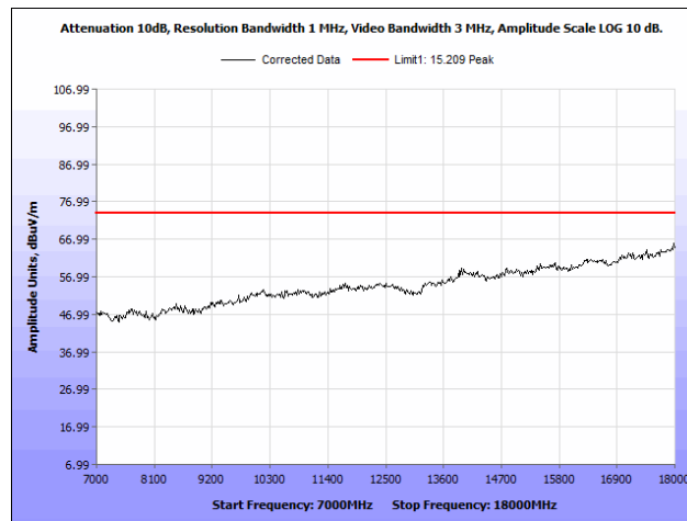
Plot 75. Radiated Spurious Emissions, 5755 MHz, PCB Antenna, 7 GHz – 18 GHz, Peak
