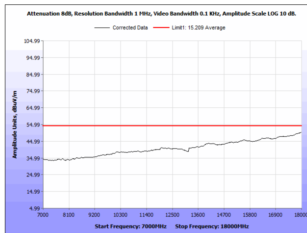
Plot 39. Radiated Spurious Emissions, 5805 MHz, Rubber Ducky Antenna, 7 GHz – 18 GHz, Average
