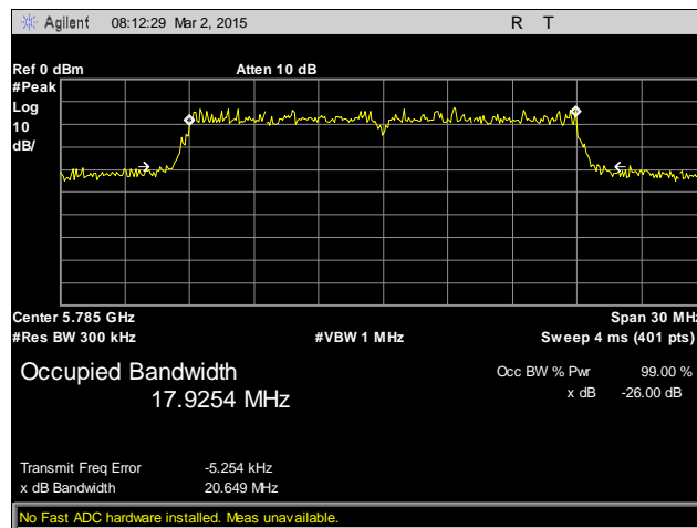
Plot 2. 26 dB Occupied Bandwidth, 5785 MHz, Antenna 1
