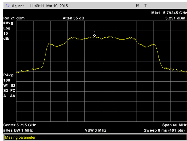
Plot 30. Peak Power Spectral Density, 5795 MHz, Antenna 2
