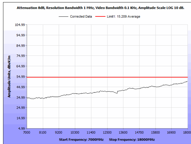
Plot 44. Radiated Spurious Emissions, 5825 MHz, Rubber Ducky Antenna, 7 GHz – 18 GHz, Average
