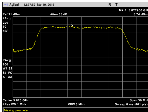
Plot 23. Peak Power Spectral Density, 5825 MHz, Antenna 1
