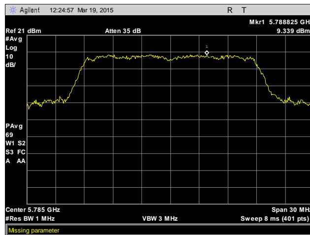
Plot 22. Peak Power Spectral Density, 5785 MHz, Antenna 1
