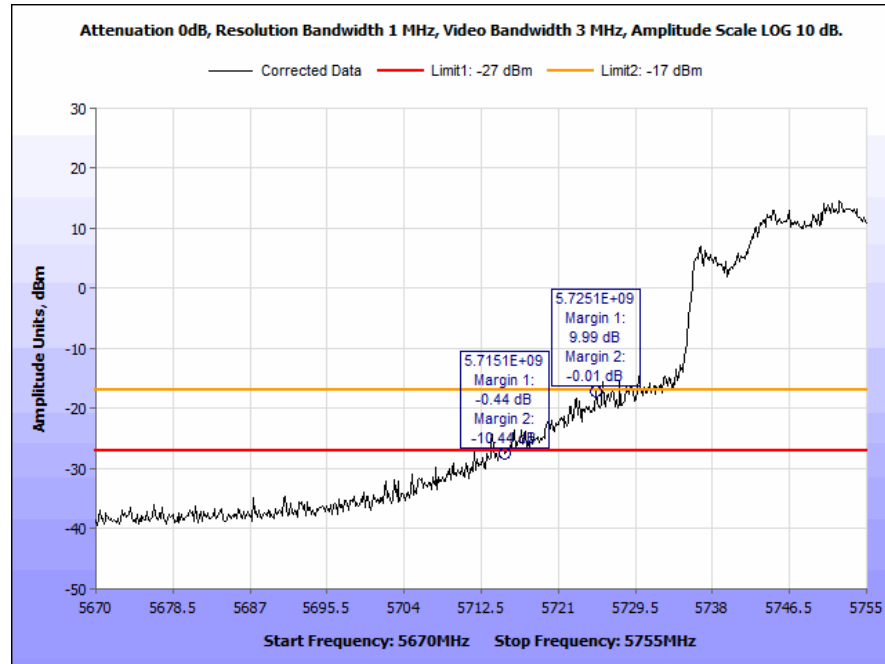
Plot 83. Radiated Band Edge, 5755 MHz @ 5725 MHz, -27 dBm & -17 dBm, Rubber Ducky Antenna
