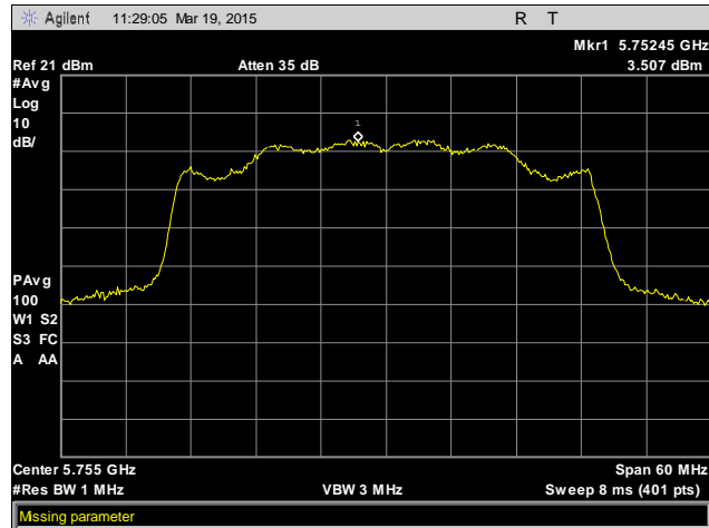
Plot 29. Peak Power Spectral Density, 5755 MHz, Antenna 2
