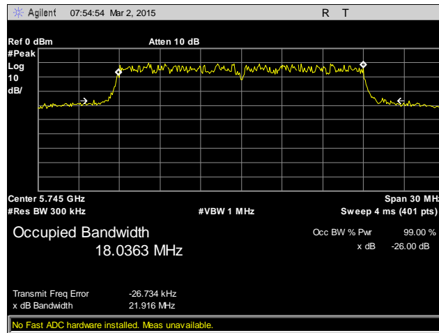
Plot 1. 26 dB Occupied Bandwidth, 5745 MHz, Antenna 1
