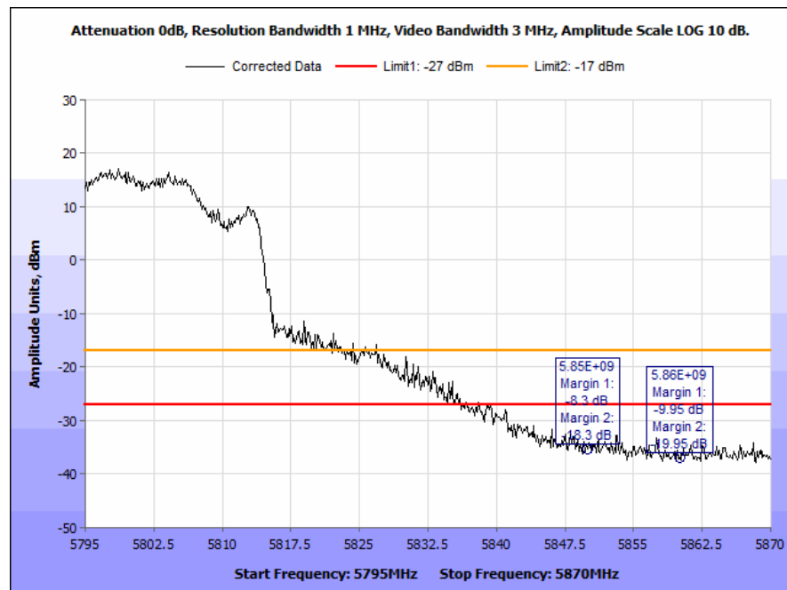
Plot 88. Radiated Band Edge, 5795 MHz @ 5850 MHz, -27 dBm & -17 dBm, PCB Antenna
