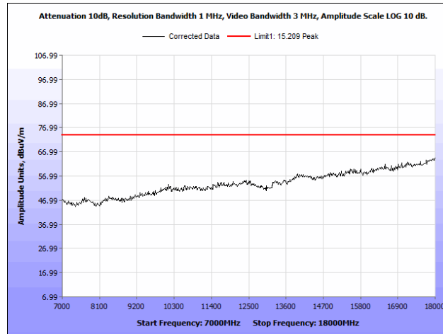
Plot 65. Radiated Spurious Emissions, 5805 MHz, PCB Antenna, 7 GHz – 18 GHz, Peak
