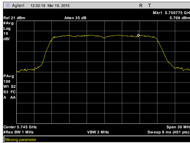
Plot 21. Peak Power Spectral Density, 5745 MHz, Antenna 1
