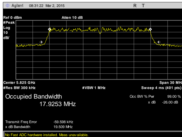
Plot 3. 26 dB Occupied Bandwidth, 5825 MHz, Antenna 1
