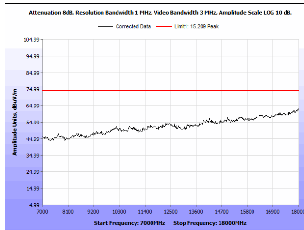
Plot 35. Radiated Spurious Emissions, 5745 MHz, Rubber Ducky Antenna, 7 GHz – 18 GHz, Peak
