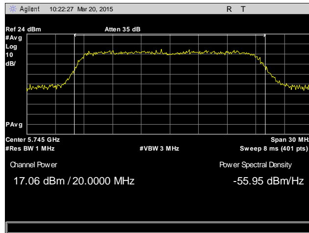
Plot 16. RF Output Power, 5745 MHz, Antenna 2
