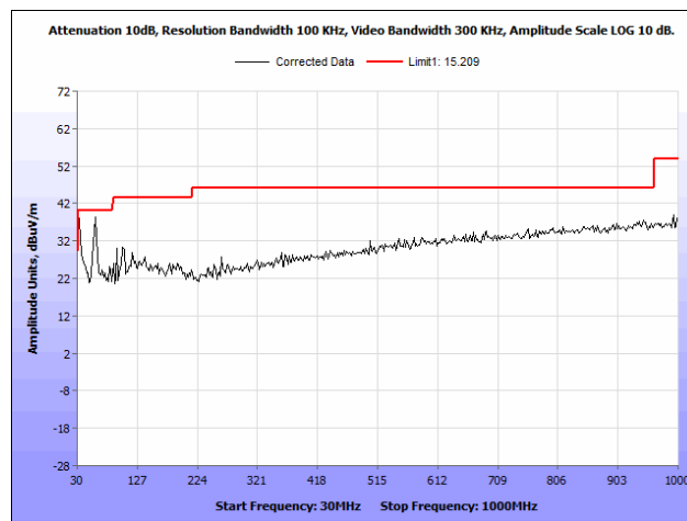
Plot 76. Radiated Spurious Emissions, 5795 MHz, PCB Antenna, 30 MHz – 1 GHz
