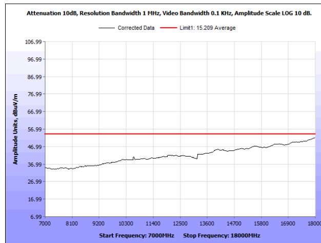
Plot 69. Radiated Spurious Emissions, 5825 MHz, PCB Antenna, 7 GHz – 18 GHz, Average
