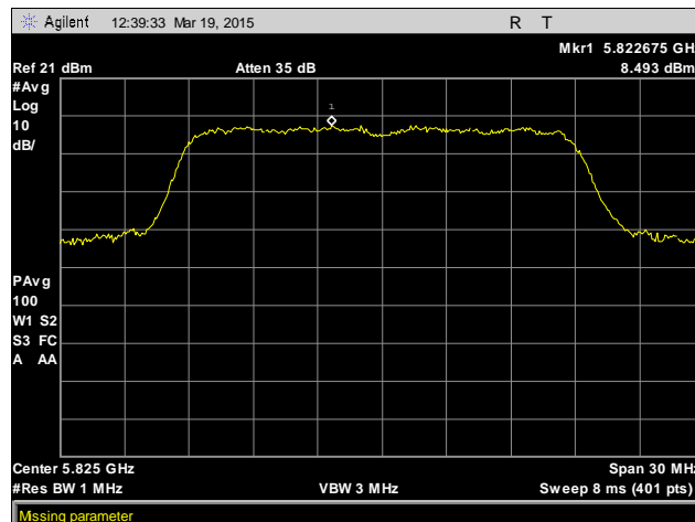
Plot 28. Peak Power Spectral Density, 5825 MHz, Antenna 2
