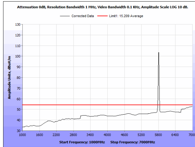
Plot 62. Radiated Spurious Emissions, 5805 MHz, PCB Antenna, 1 GHz – 7 GHz, Average
