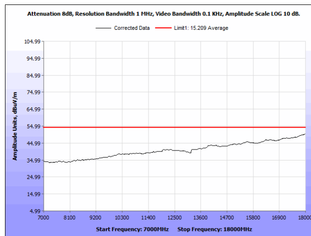
Plot 54. Radiated Spurious Emissions, 5795 MHz, Rubber Ducky Antenna, 7 GHz – 18 GHz, Average
