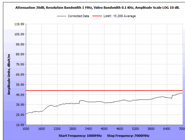
Plot 47. Radiated Spurious Emissions, 5755 MHz, Rubber Ducky Antenna, 1 GHz – 7 GHz, Average
