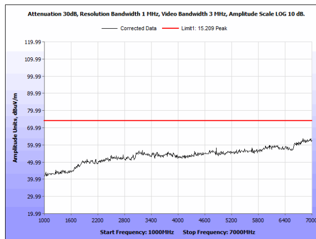
Plot 48. Radiated Spurious Emissions, 5755 MHz, Rubber Ducky Antenna, 1 GHz – 7 GHz, Peak
