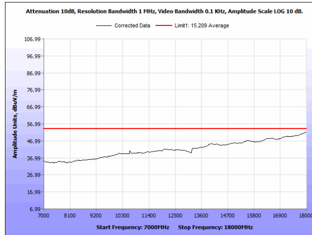
Plot 74. Radiated Spurious Emissions, 5755 MHz, PCB Antenna, 7 GHz – 18 GHz, Average
