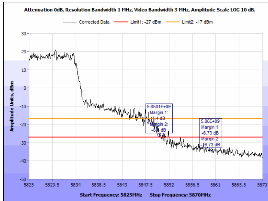
Plot 86. Radiated Band Edge, 5825 MHz @ 5850 MHz, -27 dBm & -17 dBm, PCB Antenna
