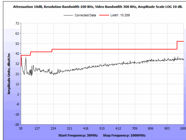
Plot 71. Radiated Spurious Emissions, 5755 MHz, PCB Antenna, 30 MHz – 1 GHz
