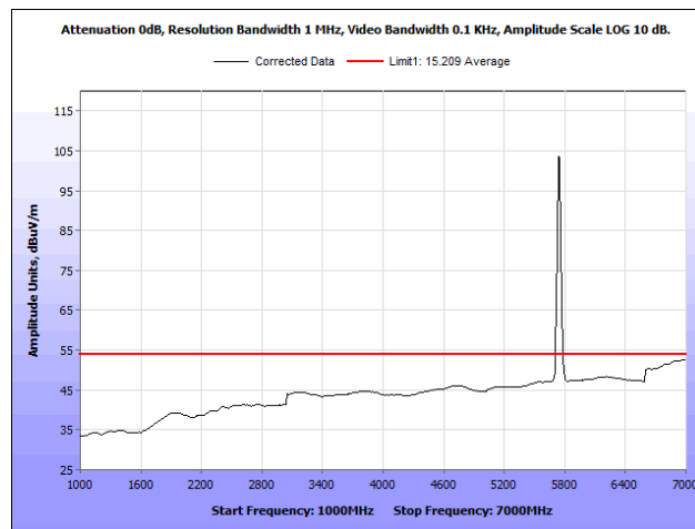
Plot 57. Radiated Spurious Emissions, 5745 MHz, PCB Antenna, 1 GHz – 7 GHz, Average
