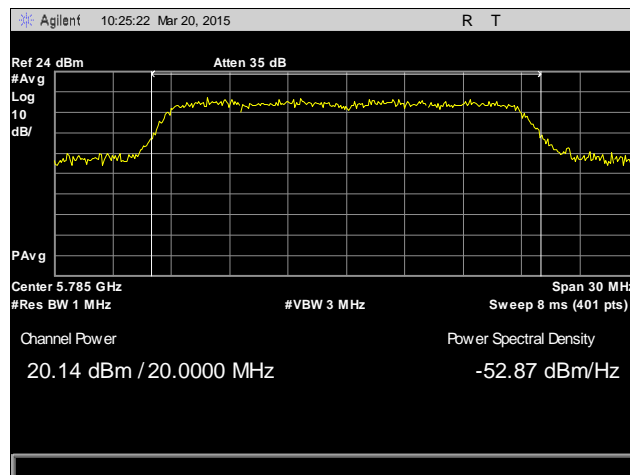
Plot 12. RF Output Power, 5785 MHz, Antenna 1
