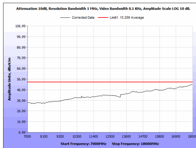
Plot 64. Radiated Spurious Emissions, 5805 MHz, PCB Antenna, 7 GHz – 18 GHz, Average
