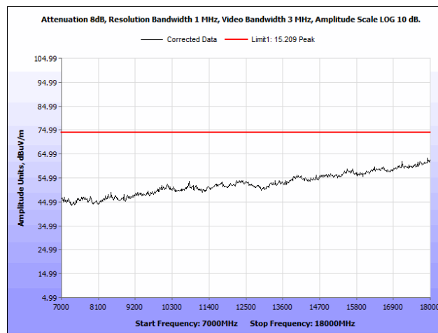
Plot 45. Radiated Spurious Emissions, 5825 MHz, Rubber Ducky Antenna, 7 GHz – 18 GHz, Peak
