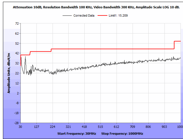
Plot 56. Radiated Spurious Emissions, 5745 MHz, PCB Antenna, 30 MHz – 1 GHz
