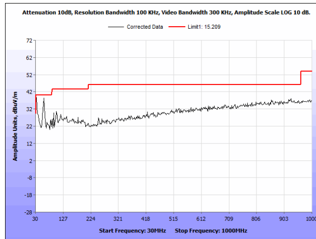
Plot 31. Radiated Spurious Emissions, 5745 MHz, Rubber Ducky Antenna, 30 MHz – 1 GHz
