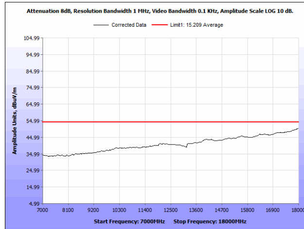
Plot 49. Radiated Spurious Emissions, 5755 MHz, Rubber Ducky Antenna, 7 GHz – 18 GHz, Average
