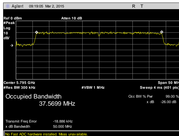
Plot 5. 26 dB Occupied Bandwidth, 5795 MHz, Antenna 1
