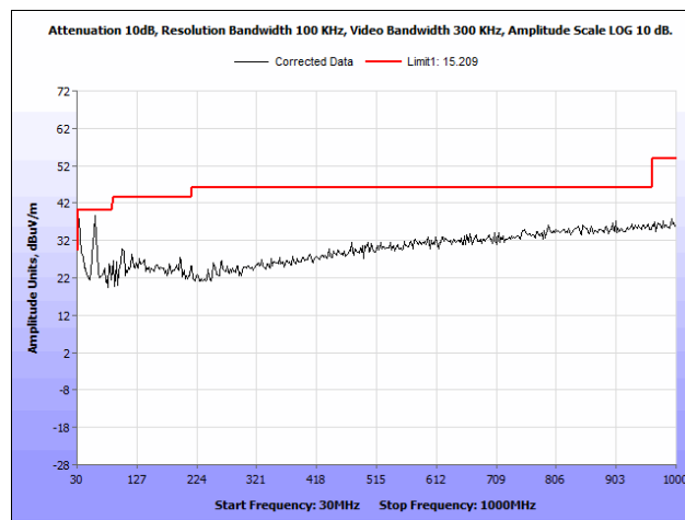
Plot 51. Radiated Spurious Emissions, 5795 MHz, Rubber Ducky Antenna, 30 MHz – 1 GHz
