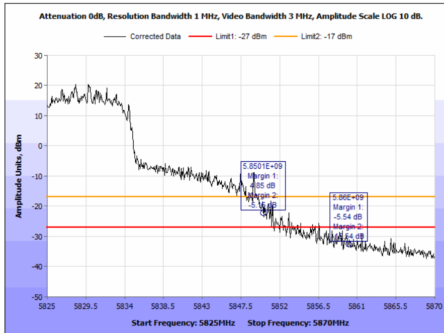
Plot 82. Radiated Band Edge, 5825 MHz @ 5850 MHz, -27 dBm & -17 dBm, Rubber Ducky Antenna
