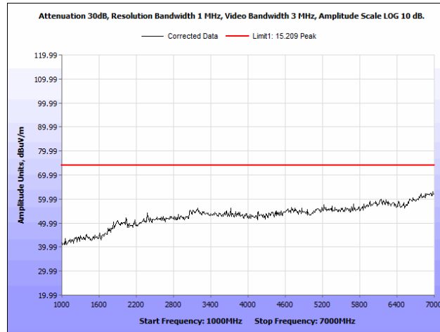
Plot 43. Radiated Spurious Emissions, 5825 MHz, Rubber Ducky Antenna, 1 GHz – 7 GHz, Peak
