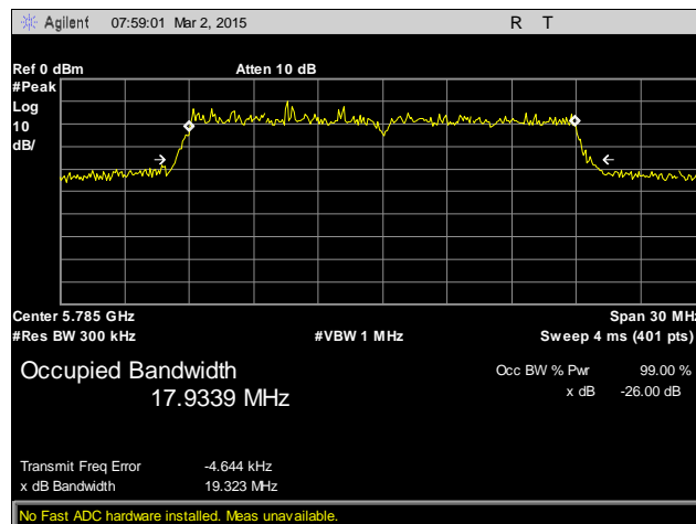
Plot 7. 26 dB Occupied Bandwidth, 5785 MHz, Antenna 2
