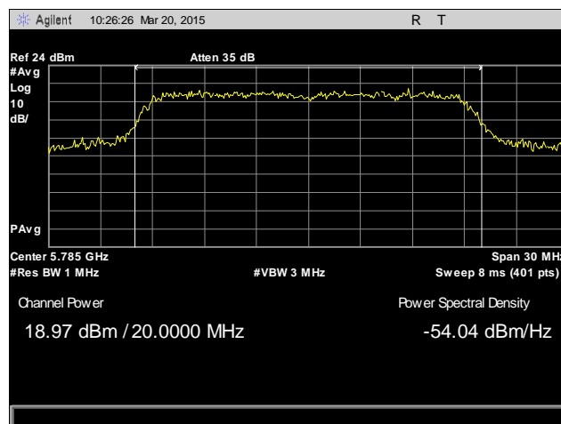
Plot 17. RF Output Power, 5785 MHz, Antenna 2
