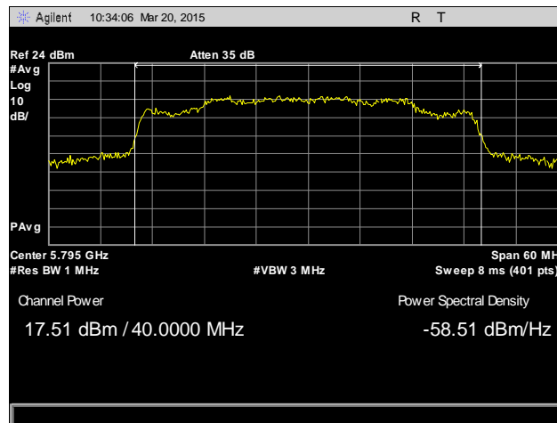
Plot 20. RF Output Power, 5795 MHz, Antenna 2
