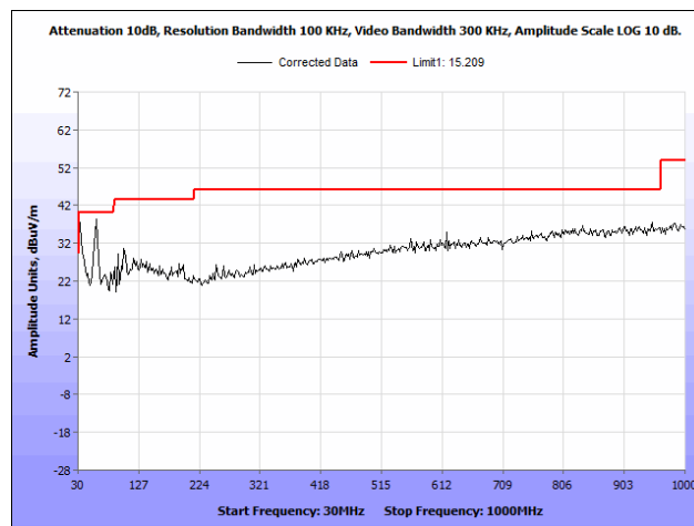
Plot 36. Radiated Spurious Emissions, 5805 MHz, Rubber Ducky Antenna, 30 MHz – 1 GHz
