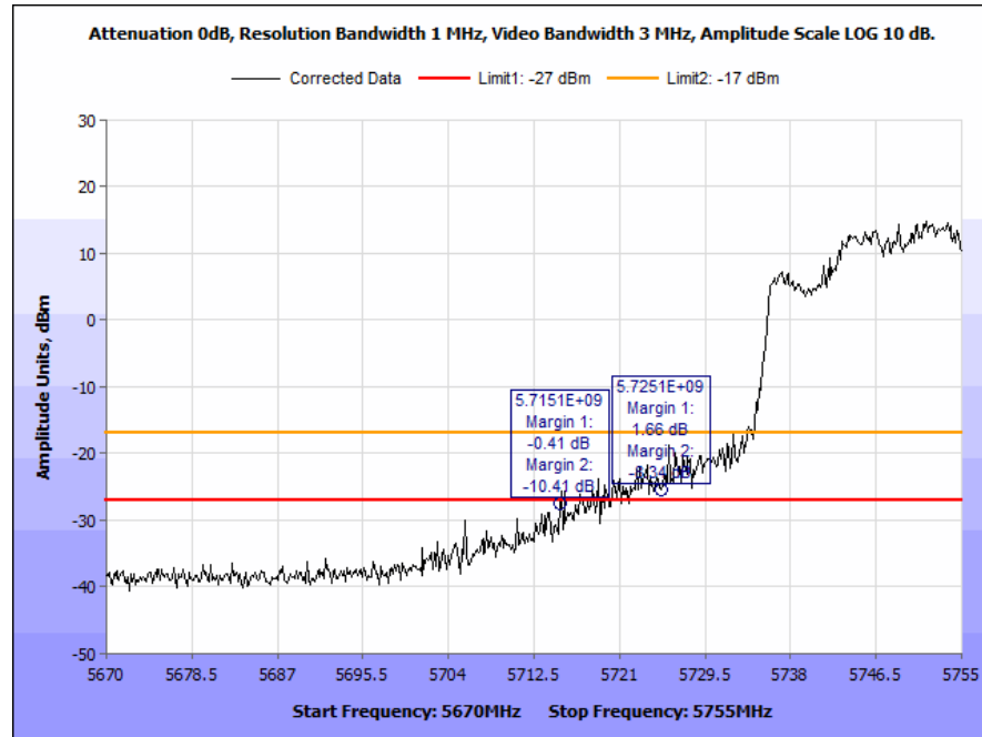
Plot 87. Radiated Band Edge, 5755 MHz @ 5725 MHz, -27 dBm & -17 dBm, PCB Antenna
