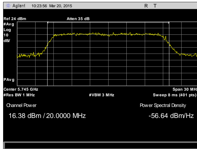
Plot 11. RF Output Power, 5745 MHz, Antenna 1
