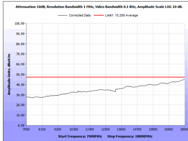
Plot 59. Radiated Spurious Emissions, 5745 MHz, PCB Antenna, 7 GHz – 18 GHz, Average
