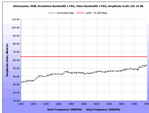
Plot 38. Radiated Spurious Emissions, 5805 MHz, Rubber Ducky Antenna, 1 GHz – 7 GHz, Peak
