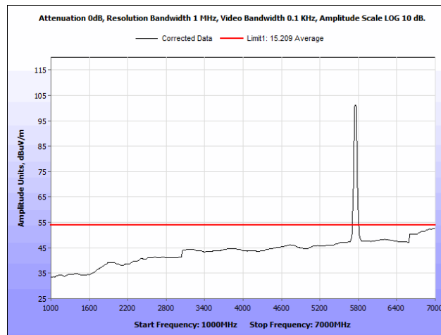
Plot 72. Radiated Spurious Emissions, 5755 MHz, PCB Antenna, 1 GHz – 7 GHz, Average
