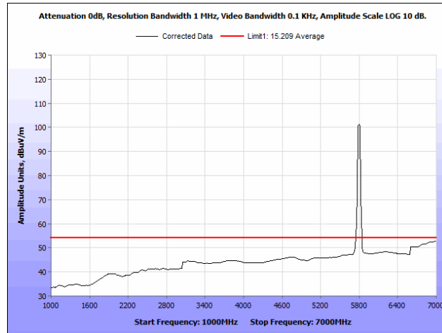
Plot 77. Radiated Spurious Emissions, 5795 MHz, PCB Antenna, 1 GHz – 7 GHz, Average
