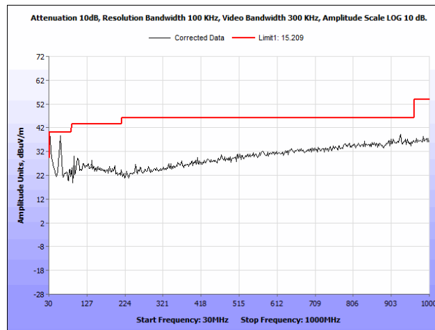
Plot 66. Radiated Spurious Emissions, 5825 MHz, PCB Antenna, 30 MHz – 1 GHz
