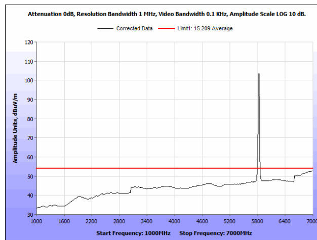
Plot 67. Radiated Spurious Emissions, 5825 MHz, PCB Antenna, 1 GHz – 7 GHz, Average
