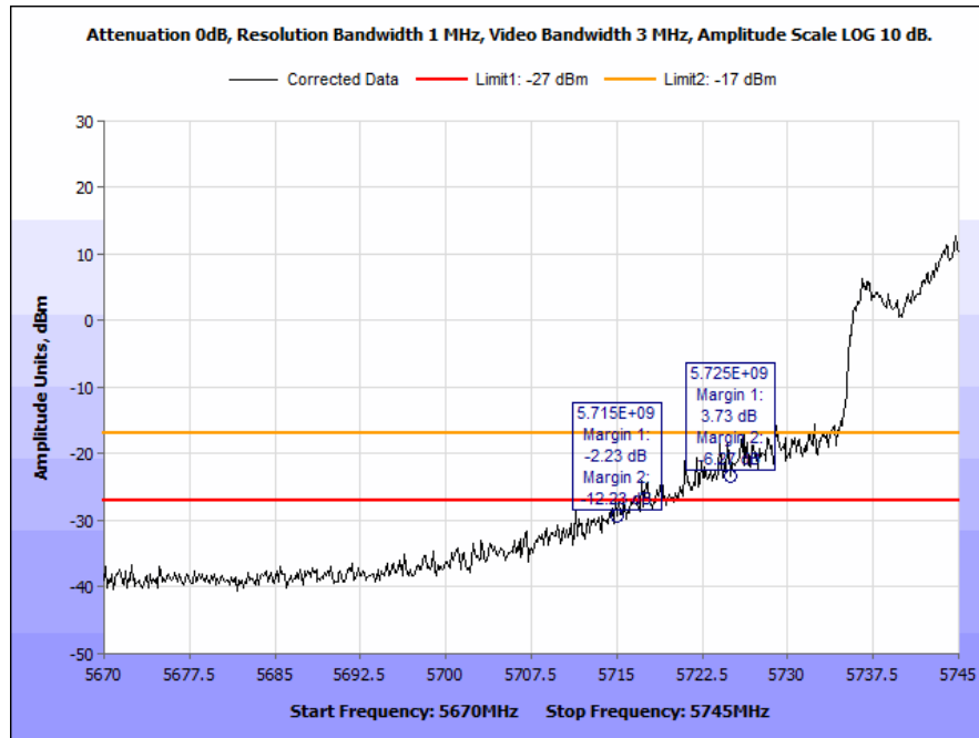
Plot 81. Radiated Band Edge, 5745 MHz @ 5725 MHz, -27 dBm & -17 dBm, Rubber Ducky Antenna
