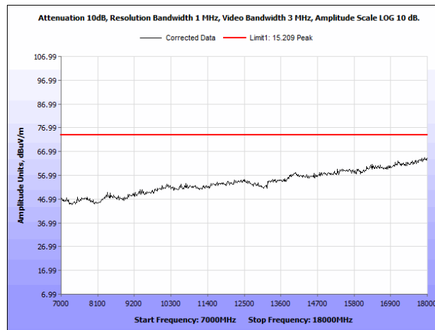
Plot 60. Radiated Spurious Emissions, 5745 MHz, PCB Antenna, 7 GHz – 18 GHz, Peak
