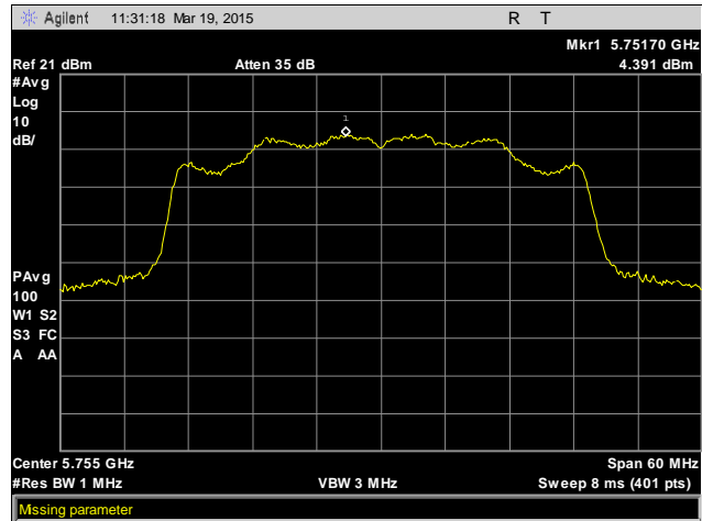
Plot 24. Peak Power Spectral Density, 5755 MHz, Antenna 1
