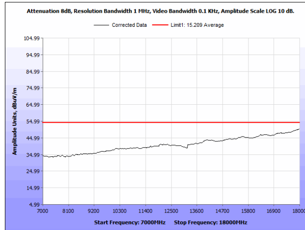
Plot 34. Radiated Spurious Emissions, 5745 MHz, Rubber Ducky Antenna, 7 GHz – 18 GHz, Average
