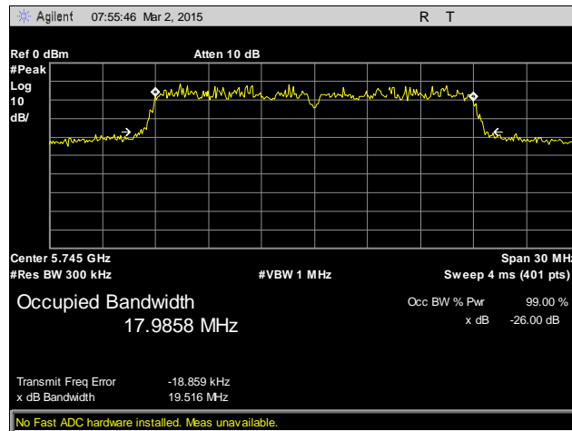
Plot 6. 26 dB Occupied Bandwidth, 5745 MHz, Antenna 2
