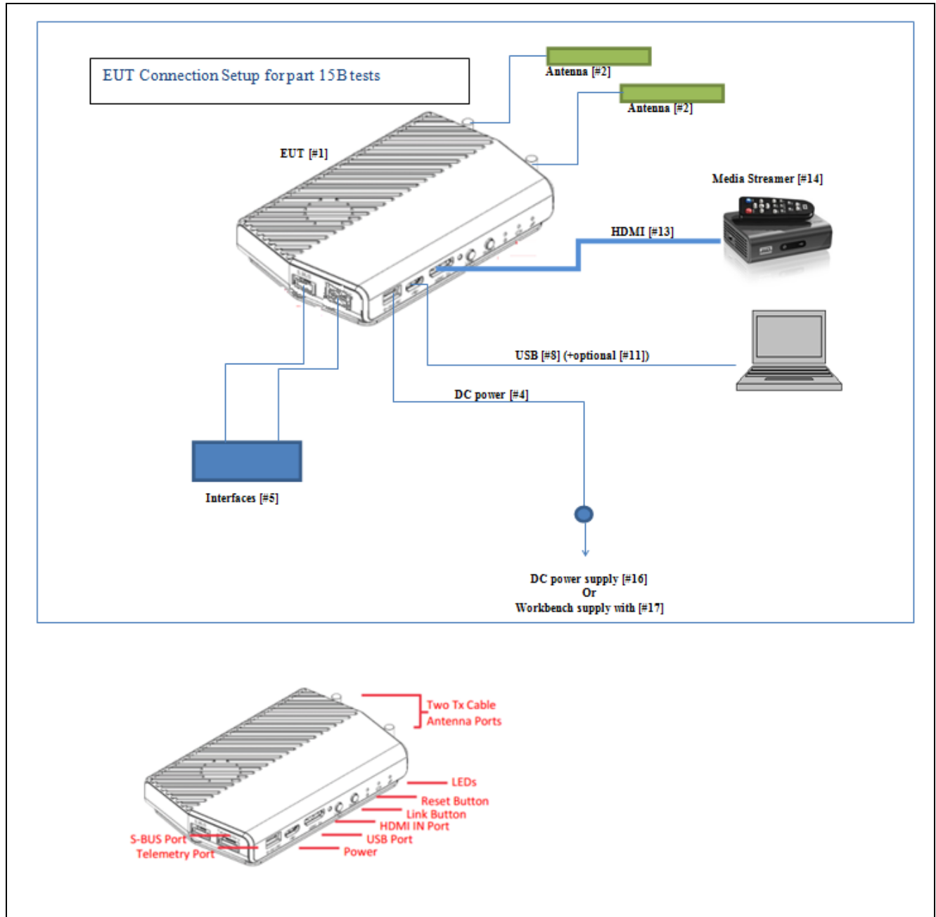
Figure 1. Block Diagram of Test Configuration
