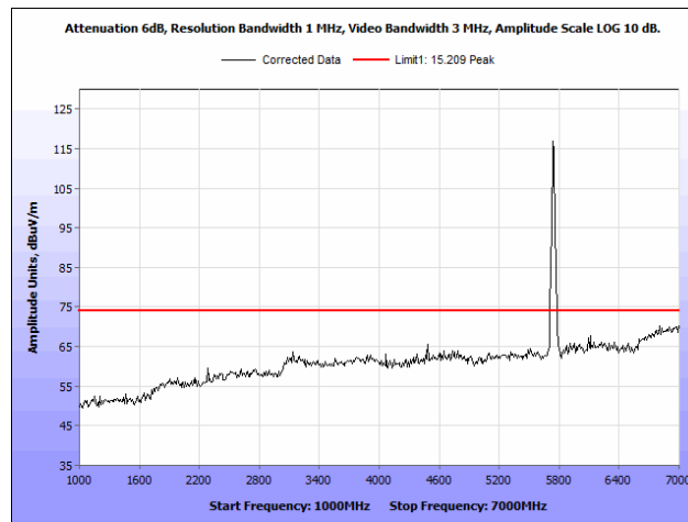
Plot 63. Radiated Spurious Emissions, 5805 MHz, PCB Antenna, 1 GHz – 7 GHz, Peak
