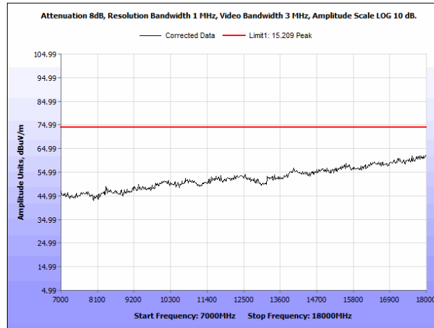
Plot 55. Radiated Spurious Emissions, 5795 MHz, Rubber Ducky Antenna, 7 GHz – 18 GHz, Peak
