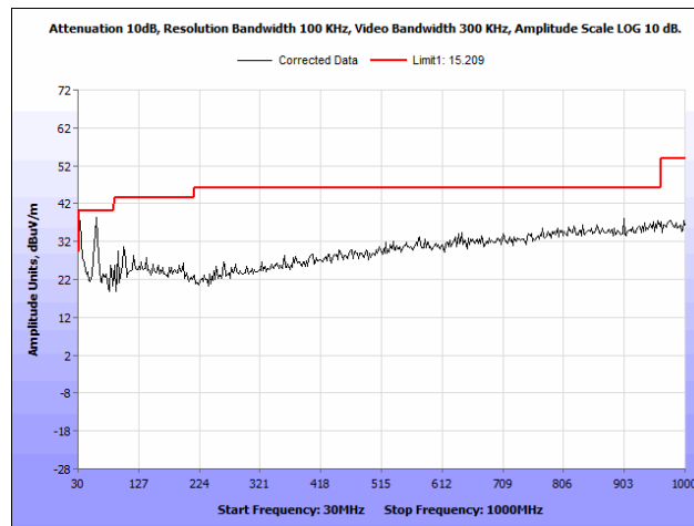
Plot 41. Radiated Spurious Emissions, 5825 MHz, Rubber Ducky Antenna, 30 MHz – 1 GHz
