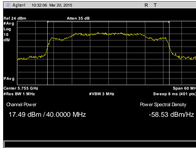
Plot 19. RF Output Power, 5755 MHz, Antenna 2
