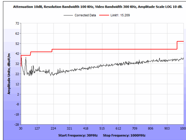
Plot 46. Radiated Spurious Emissions, 5755 MHz, Rubber Ducky Antenna, 30 MHz – 1 GHz
