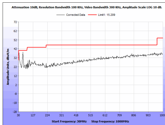
Plot 61. Radiated Spurious Emissions, 5805 MHz, PCB Antenna, 30 MHz – 1 GHz
