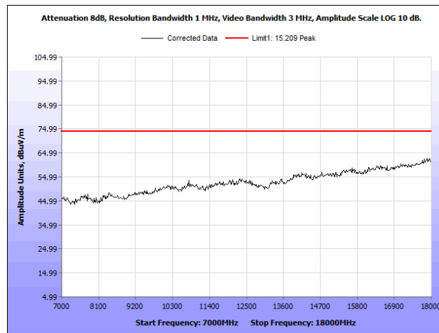
Plot 50. Radiated Spurious Emissions, 5755 MHz, Rubber Ducky Antenna, 7 GHz – 18 GHz, Peak
