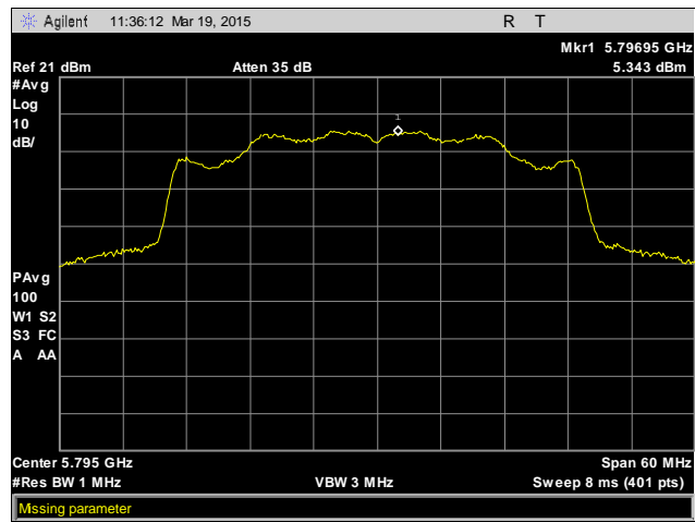
Plot 25. Peak Power Spectral Density, 5795 MHz, Antenna 1
