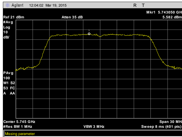
Plot 26. Peak Power Spectral Density, 5745 MHz, Antenna 2
