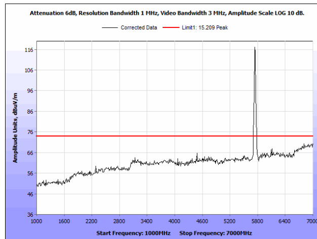
Plot 58. Radiated Spurious Emissions, 5745 MHz, PCB Antenna, 1 GHz – 7 GHz, Peak
