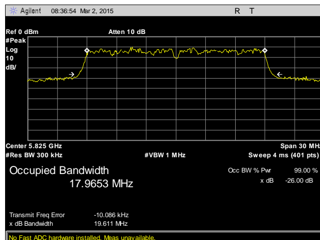
Plot 8. 26 dB Occupied Bandwidth, 5825 MHz, Antenna 2
