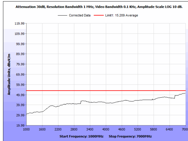
Plot 37. Radiated Spurious Emissions, 5805 MHz, Rubber Ducky Antenna, 1 GHz – 7 GHz, Average
