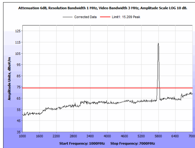
Plot 78. Radiated Spurious Emissions, 5795 MHz, PCB Antenna, 1 GHz – 7 GHz, Peak
