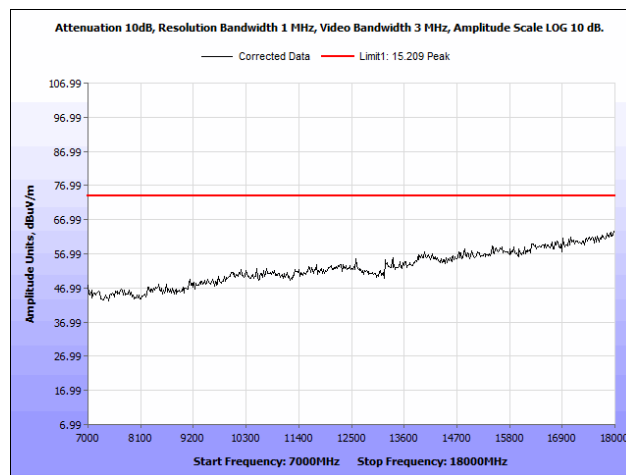
Plot 70. Radiated Spurious Emissions, 5825 MHz, PCB Antenna, 7 GHz – 18 GHz, Peak
