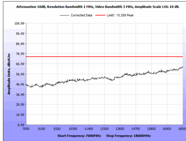
Plot 80. Radiated Spurious Emissions, 5795 MHz, PCB Antenna, 7 GHz – 18 GHz, Peak
