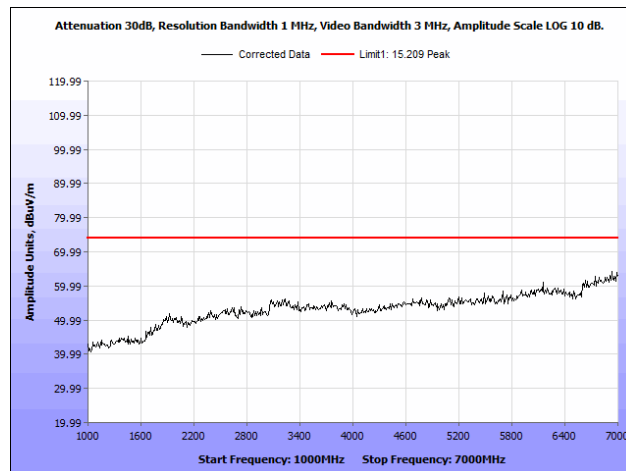
Plot 33. Radiated Spurious Emissions, 5745 MHz, Rubber Ducky Antenna, 1 GHz – 7 GHz, Peak
