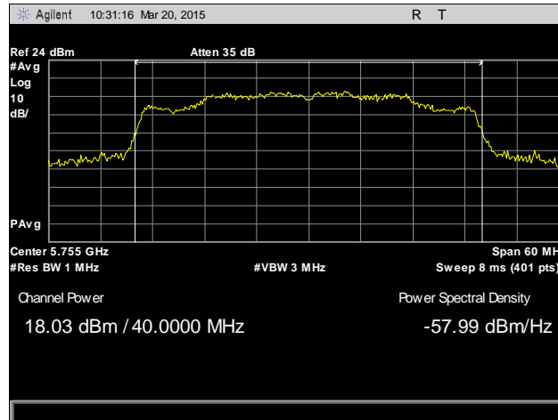
Plot 14. RF Output Power, 5755 MHz, Antenna 1
