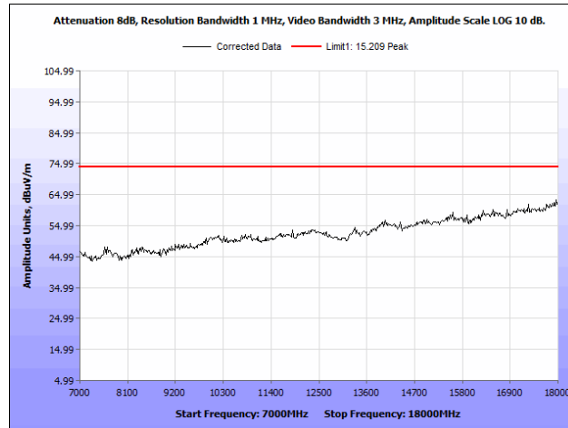
Plot 40. Radiated Spurious Emissions, 5805 MHz, Rubber Ducky Antenna, 7 GHz – 18 GHz, Peak
