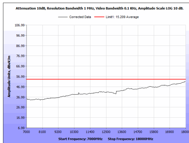
Plot 79. Radiated Spurious Emissions, 5795 MHz, PCB Antenna, 7 GHz – 18 GHz, Average
