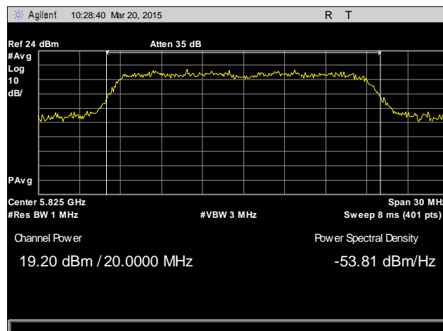
Plot 13. RF Output Power, 5825 MHz, Antenna 1
