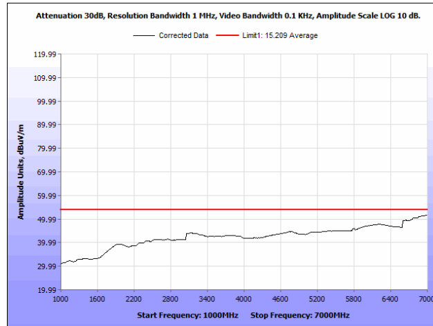
Plot 52. Radiated Spurious Emissions, 5795 MHz, Rubber Ducky Antenna, 1 GHz – 7 GHz, Average
