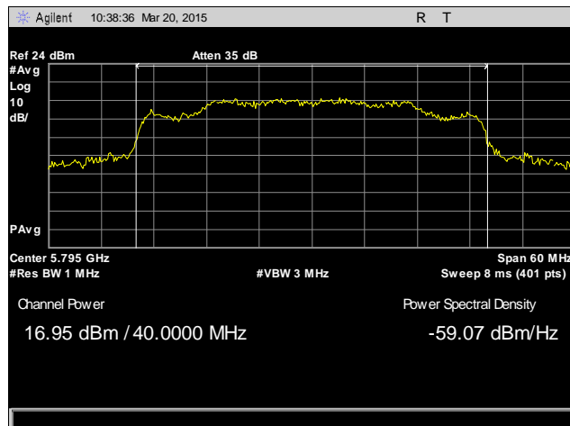
Plot 15. RF Output Power, 5795 MHz, Antenna 1
