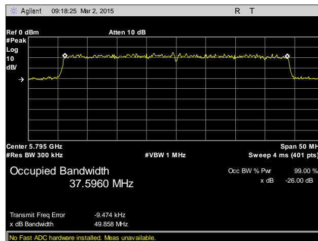
Plot 10. 26 dB Occupied Bandwidth, 5795 MHz, Antenna 2
