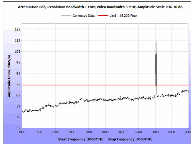
Plot 68. Radiated Spurious Emissions, 5825 MHz, PCB Antenna, 1 GHz – 7 GHz, Peak
