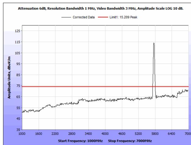
Plot 73. Radiated Spurious Emissions, 5755 MHz, PCB Antenna, 1 GHz – 7 GHz, Peak
