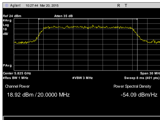
Plot 18. RF Output Power, 5825 MHz, Antenna 2
