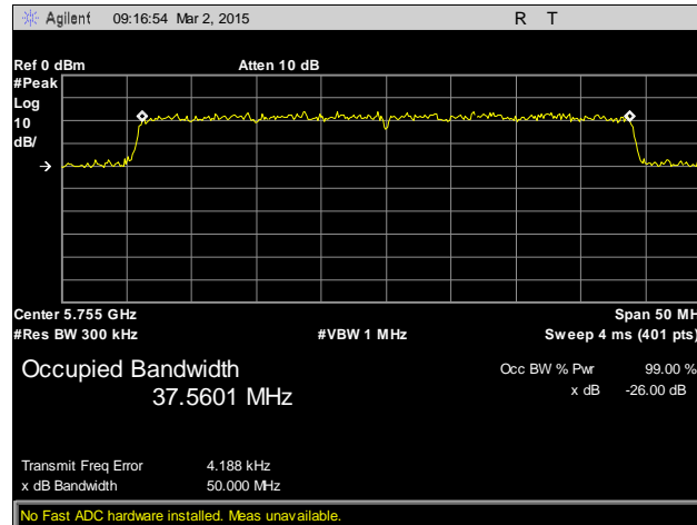
Plot 4. 26 dB Occupied Bandwidth, 5755 MHz, Antenna 1
