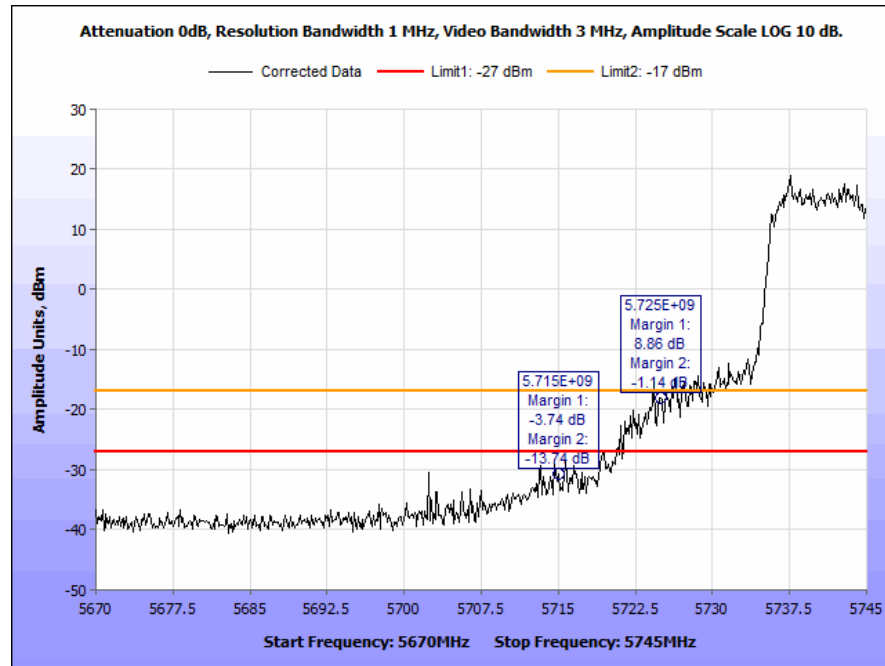
Plot 85. Radiated Band Edge, 5745 MHz @ 5725 MHz, -27 dBm & -17 dBm, PCB Antenna
