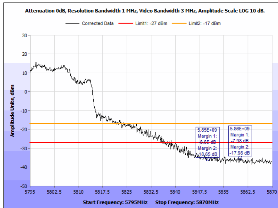
Plot 84. Radiated Band Edge, 5795 MHz @ 5850 MHz, -27 dBm & -17 dBm, Rubber Ducky Antenna
