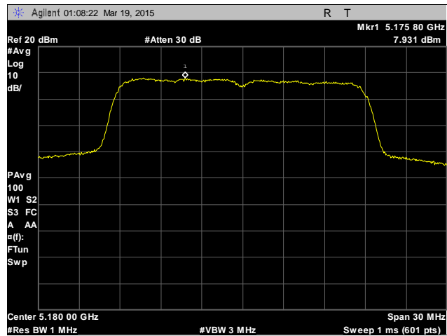
Plot 26. Peak Power Spectral Density, 5180 MHz, Antenna 2
