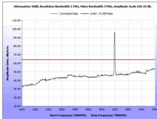
Plot 38. Radiated Spurious Emissions, 5200 MHz, Rubber Ducky Antenna, 1 GHz – 7 GHz, Peak
