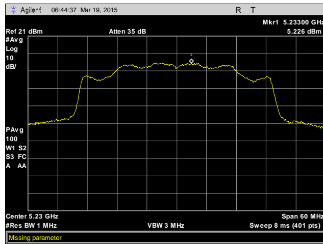
Plot 30. Peak Power Spectral Density, 5230 MHz, Antenna 2
