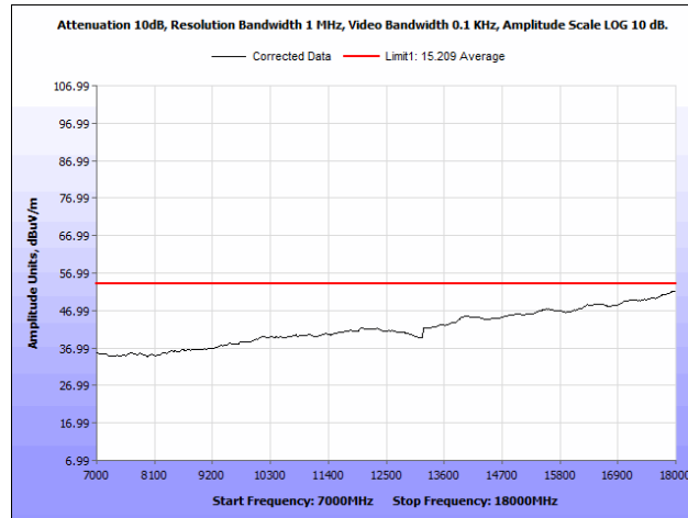
Plot 59. Radiated Spurious Emissions, 5180 MHz, PCB Antenna, 7 GHz – 18 GHz, Average
