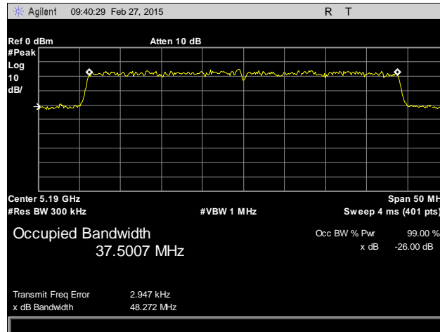
Plot 9. 26 dB Occupied Bandwidth, 5190 MHz, Antenna 2
