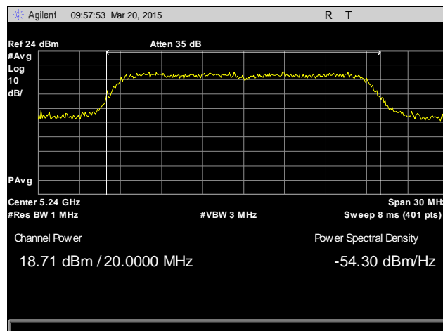
Plot 18. Peak Power Output, 5240 MHz, Antenna 2
