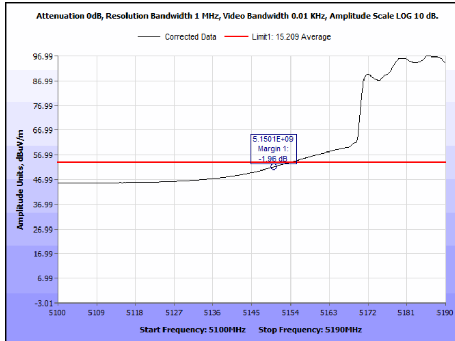
Plot 83. Radiated Band Edge, 5190 MHz @ 5150 MHz, Average, Rubber Ducky Antenna
