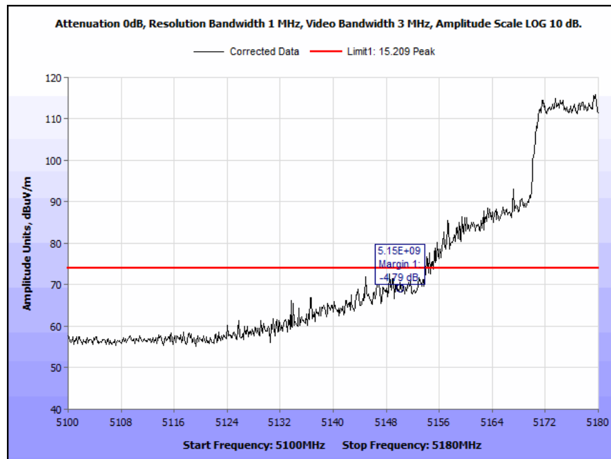
Plot 82. Radiated Band Edge, 5180 MHz @ 5150 MHz, Peak, Rubber Ducky Antenna
