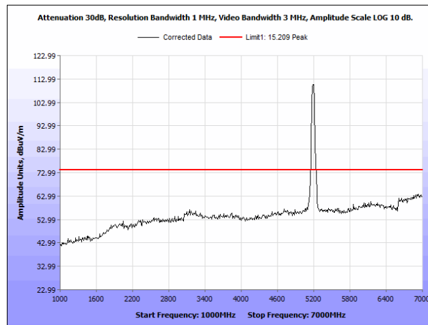
Plot 78. Radiated Spurious Emissions, 5230 MHz, PCB Antenna, 1 GHz – 7 GHz, Peak
