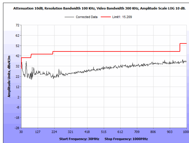
Plot 61. Radiated Spurious Emissions, 5200 MHz, PCB Antenna, 30 MHz – 1 GHz
