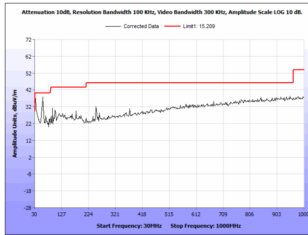
Plot 31. Radiated Spurious Emissions, 5180 MHz, Rubber Ducky Antenna, 30 MHz – 1 GHz
