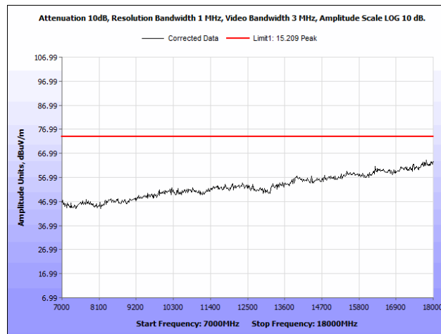
Plot 50. Radiated Spurious Emissions, 5190 MHz, Rubber Ducky Antenna, 7 GHz – 18 GHz, Peak
