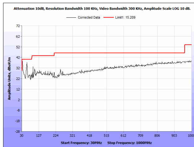
Plot 36. Radiated Spurious Emissions, 5200 MHz, Rubber Ducky Antenna, 30 MHz – 1 GHz
