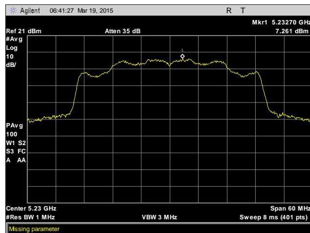
Plot 25. Peak Power Spectral Density, 5230 MHz, Antenna 1
