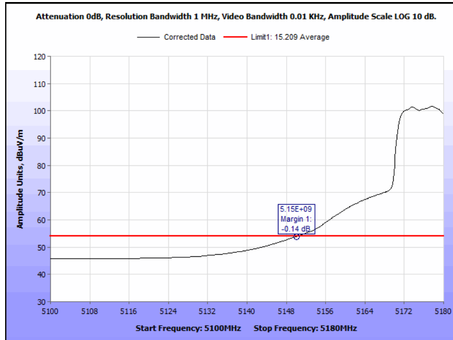
Plot 81. Radiated Band Edge, 5180 MHz @ 5150 MHz, Average, Rubber Ducky Antenna
