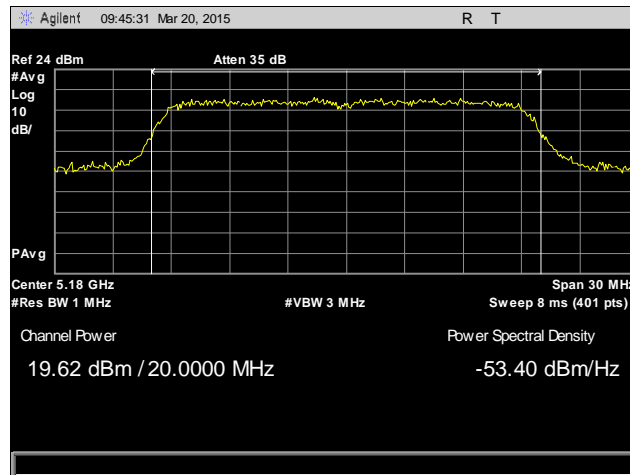
Plot 11. Peak Power Output, 5180 MHz, Antenna 1
