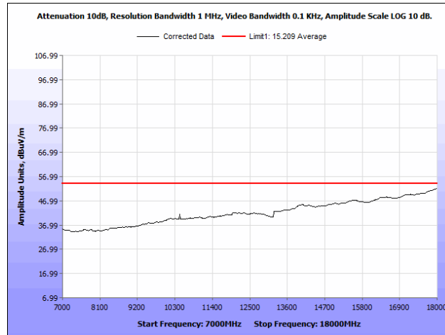
Plot 34. Radiated Spurious Emissions, 5180 MHz, Rubber Ducky Antenna, 7 GHz – 18 GHz, Average
