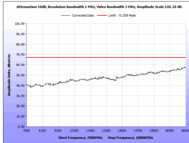
Plot 55. Radiated Spurious Emissions, 5230 MHz, Rubber Ducky Antenna, 7 GHz – 18 GHz, Peak
