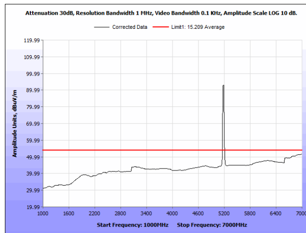
Plot 32. Radiated Spurious Emissions, 5180 MHz, Rubber Ducky Antenna, 1 GHz – 7 GHz, Average
