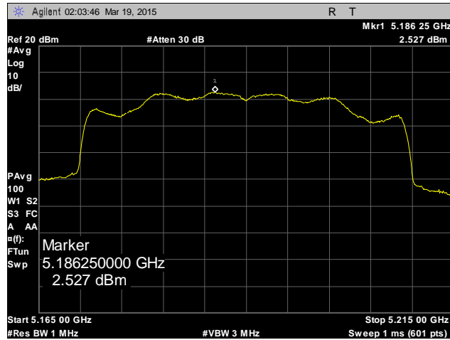
Plot 29. Peak Power Spectral Density, 5190 MHz, Antenna 2
