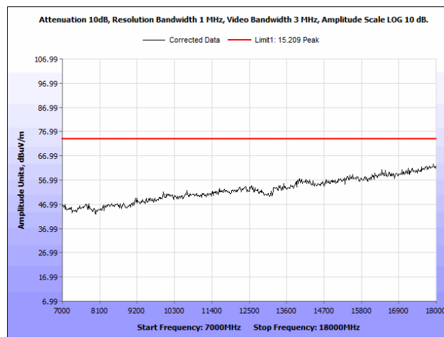
Plot 70. Radiated Spurious Emissions, 5220 MHz, PCB Antenna, 7 GHz – 18 GHz, Peak
