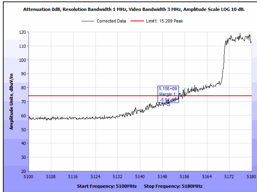
Plot 86. Radiated Band Edge, 5180 MHz @ 5150 MHz, Peak, PCB Antenna
