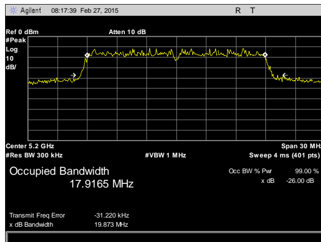
Plot 2. 26 dB Occupied Bandwidth, 5200 MHz, Antenna 1
