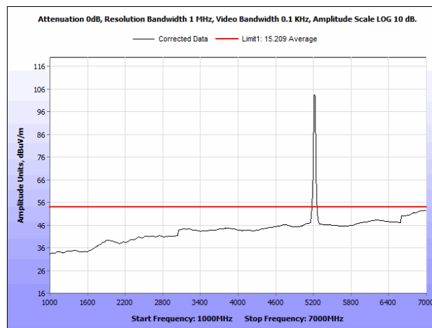
Plot 67. Radiated Spurious Emissions, 5220 MHz, PCB Antenna, 1 GHz – 7 GHz, Average
