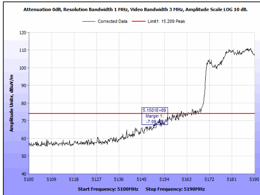
Plot 88. Radiated Band Edge, 5190 MHz @ 5150 MHz, Peak, PCB Antenna
