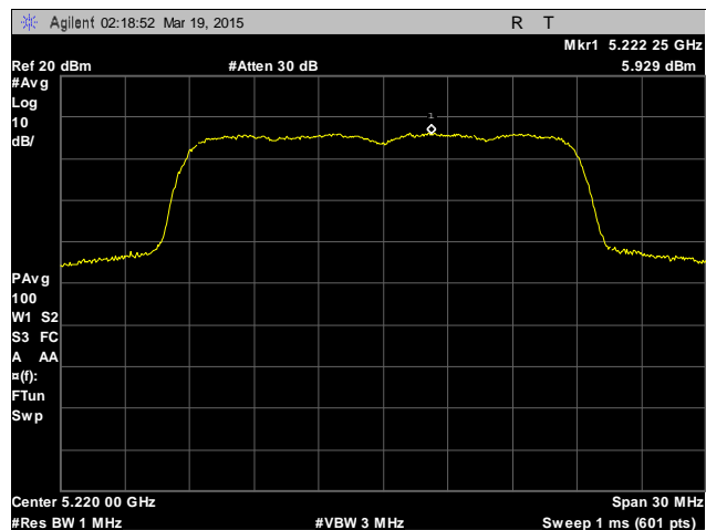
Plot 27. Peak Power Spectral Density, 5220 MHz, Antenna 2
