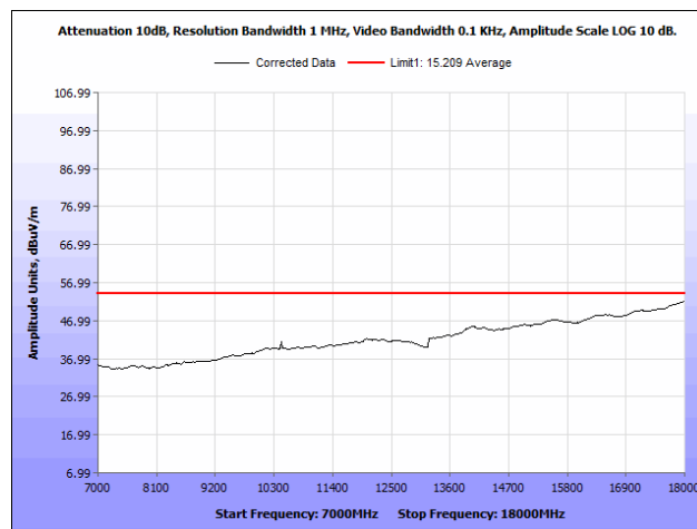
Plot 39. Radiated Spurious Emissions, 5200 MHz, Rubber Ducky Antenna, 7 GHz – 18 GHz, Average
