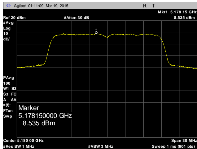
Plot 21. Peak Power Spectral Density, 5180 MHz, Antenna 1
