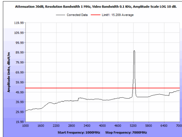
Plot 52. Radiated Spurious Emissions, 5230 MHz, Rubber Ducky Antenna, 1 GHz – 7 GHz, Average
