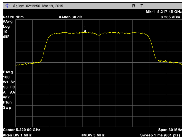
Plot 22. Peak Power Spectral Density, 5220 MHz, Antenna 1
