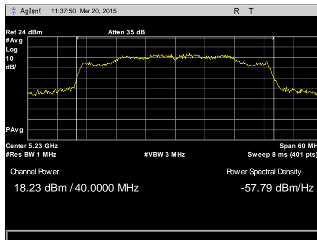
Plot 15. Peak Power Output, 5230 MHz, Antenna 1
