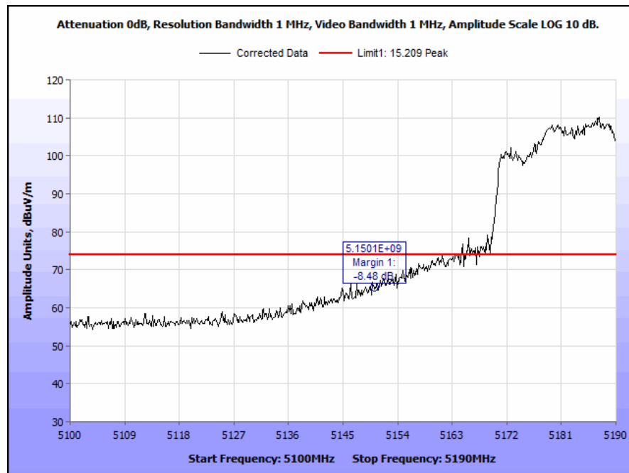
Plot 84. Radiated Band Edge, 5190 MHz @ 5150 MHz, Peak, Rubber Ducky Antenna
