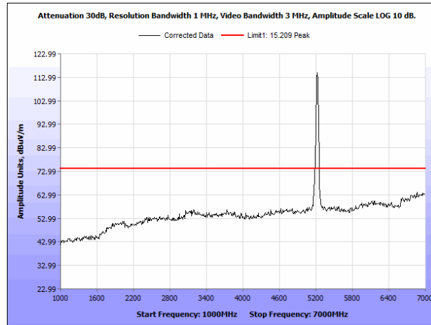
Plot 68. Radiated Spurious Emissions, 5220 MHz, PCB Antenna, 1 GHz – 7 GHz, Peak
