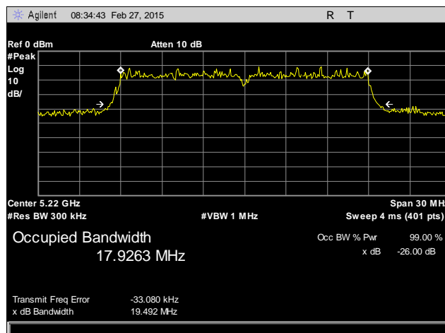
Plot 3. 26 dB Occupied Bandwidth, 5220 MHz, Antenna 1
