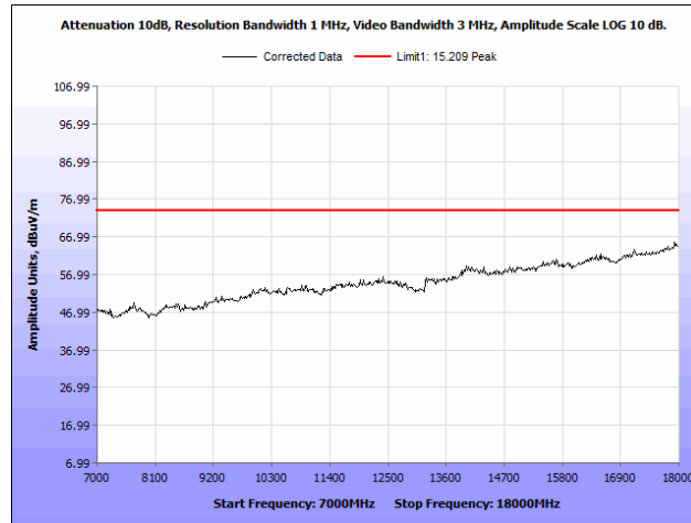
Plot 80. Radiated Spurious Emissions, 5230 MHz, PCB Antenna, 7 GHz – 18 GHz, Peak
