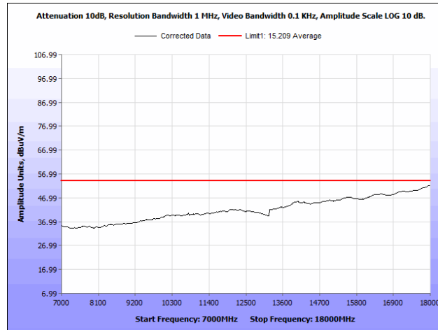
Plot 74. Radiated Spurious Emissions, 5190 MHz, PCB Antenna, 7 GHz – 18 GHz, Average
