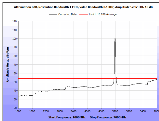
Plot 72. Radiated Spurious Emissions, 5190 MHz, PCB Antenna, 1 GHz – 7 GHz, Average
