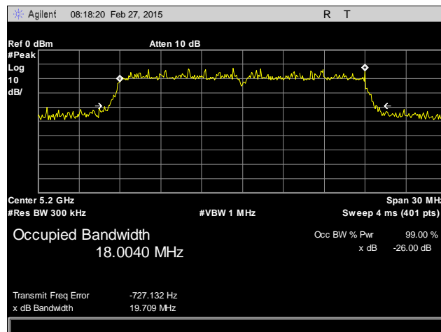
Plot 7. 26 dB Occupied Bandwidth, 5200 MHz, Antenna 2
