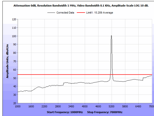
Plot 77. Radiated Spurious Emissions, 5230 MHz, PCB Antenna, 1 GHz – 7 GHz, Average
