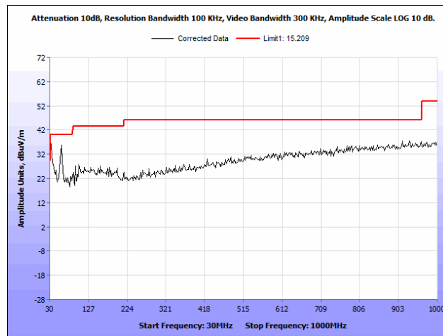
Plot 41. Radiated Spurious Emissions, 5200 MHz, Rubber Ducky Antenna, 30 MHz – 1 GHz
