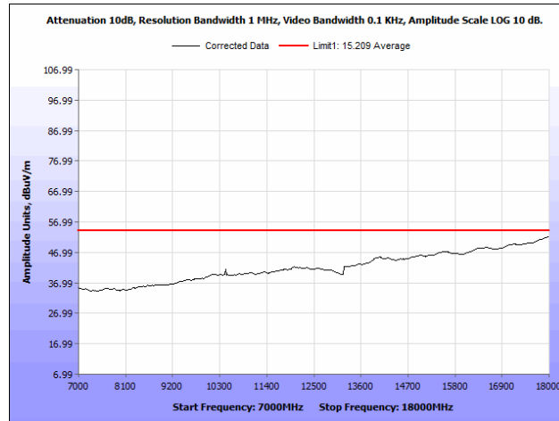
Plot 49. Radiated Spurious Emissions, 5190 MHz, Rubber Ducky Antenna, 7 GHz – 18 GHz, Average
