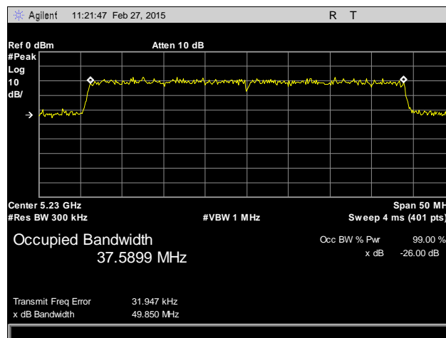
Plot 10. 26 dB Occupied Bandwidth, 5230 MHz, Antenna 2
