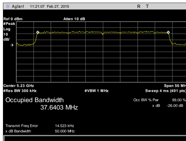
Plot 5. 26 dB Occupied Bandwidth, 5230 MHz, Antenna 1
