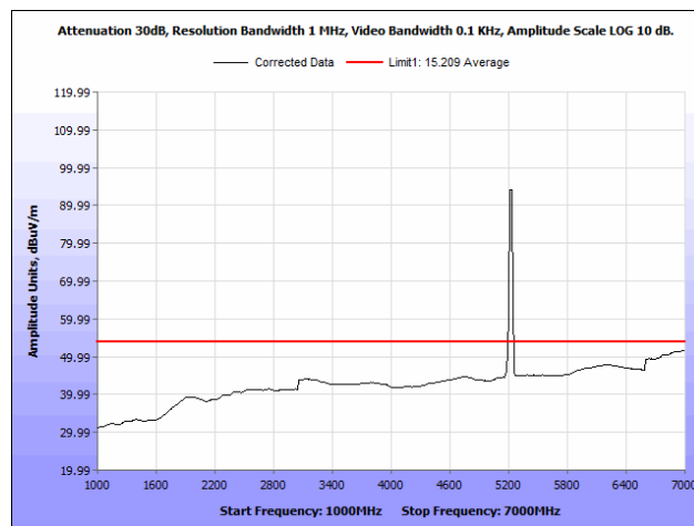
Plot 42. Radiated Spurious Emissions, 5200 MHz, Rubber Ducky Antenna, 1 GHz – 7 GHz, Average
