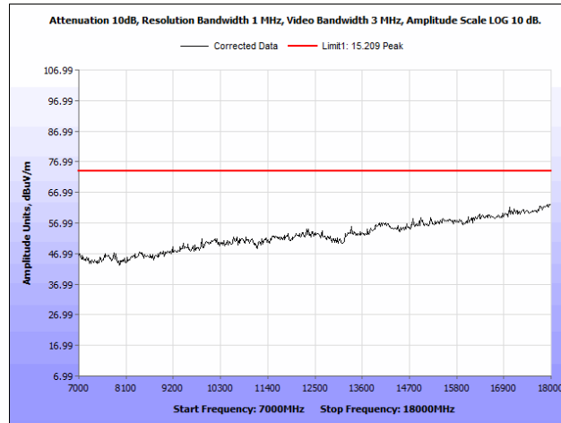
Plot 65. Radiated Spurious Emissions, 5200 MHz, PCB Antenna, 7 GHz – 18 GHz, Peak
