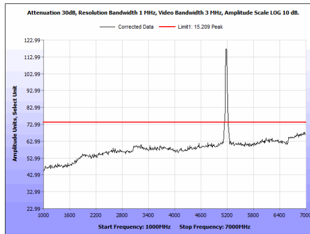
Plot 58. Radiated Spurious Emissions, 5180 MHz, PCB Antenna, 1 GHz – 7 GHz, Peak
