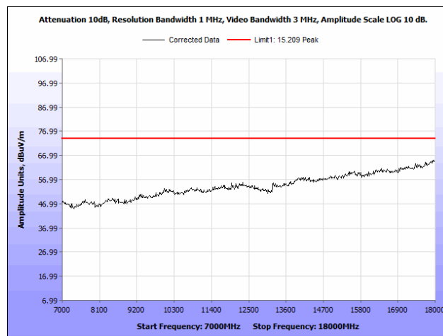
Plot 45. Radiated Spurious Emissions, 5220 MHz, Rubber Ducky Antenna, 7 GHz – 18 GHz, Peak
