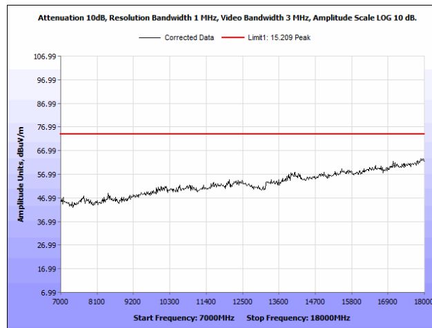
Plot 60. Radiated Spurious Emissions, 5180 MHz, PCB Antenna, 7 GHz – 18 GHz, Peak
