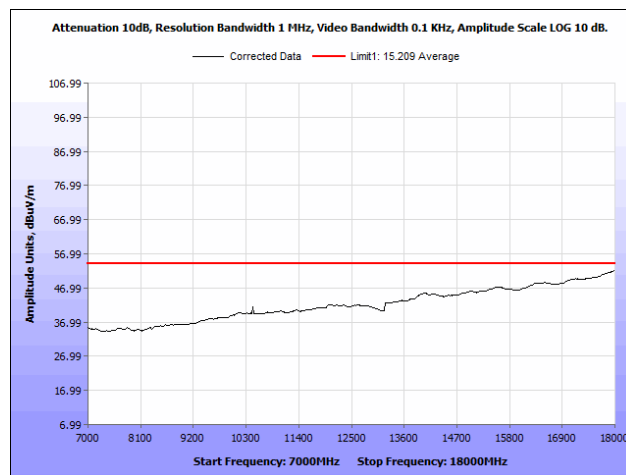
Plot 54. Radiated Spurious Emissions, 5230 MHz, Rubber Ducky Antenna, 7 GHz – 18 GHz, Average
