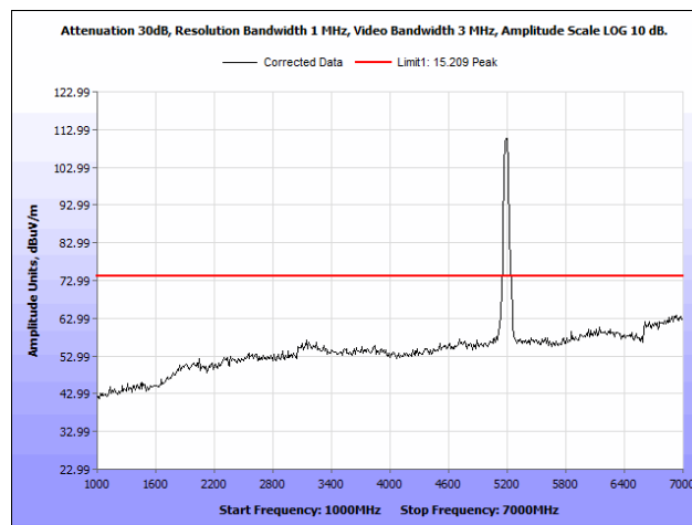
Plot 73. Radiated Spurious Emissions, 5190 MHz, PCB Antenna, 1 GHz – 7 GHz, Peak
