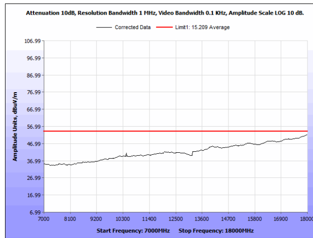
Plot 44. Radiated Spurious Emissions, 5220 MHz, Rubber Ducky Antenna, 7 GHz – 18 GHz, Average
