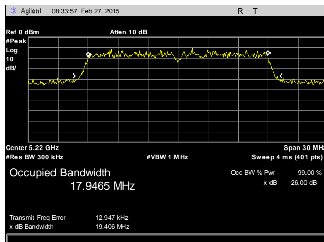
Plot 8. 26 dB Occupied Bandwidth, 5220 MHz, Antenna 2
