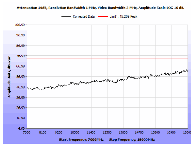
Plot 75. Radiated Spurious Emissions, 5190 MHz, PCB Antenna, 7 GHz – 18 GHz, Peak
