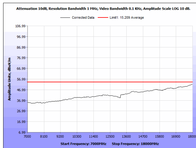
Plot 79. Radiated Spurious Emissions, 5230 MHz, PCB Antenna, 7 GHz – 18 GHz, Average
