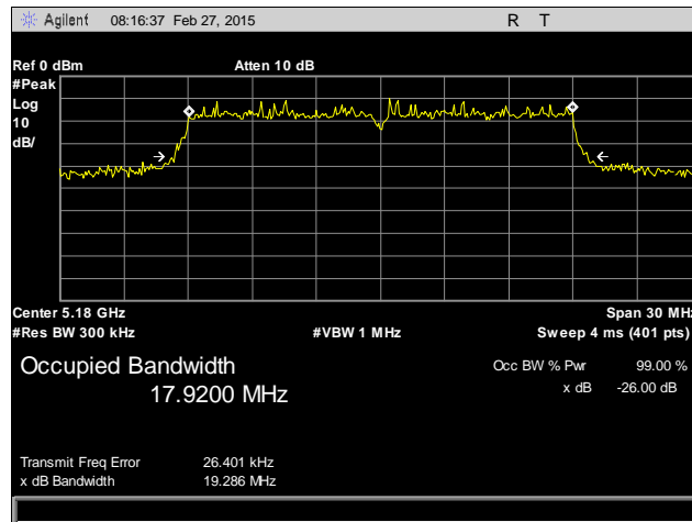
Plot 1. 26 dB Occupied Bandwidth, 5180 MHz, Antenna 1
