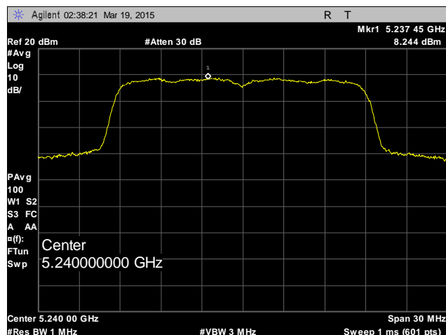
Plot 23. Peak Power Spectral Density, 5240 MHz, Antenna 1
