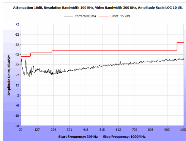
Plot 66. Radiated Spurious Emissions, 5220 MHz, PCB Antenna, 30 MHz – 1 GHz
