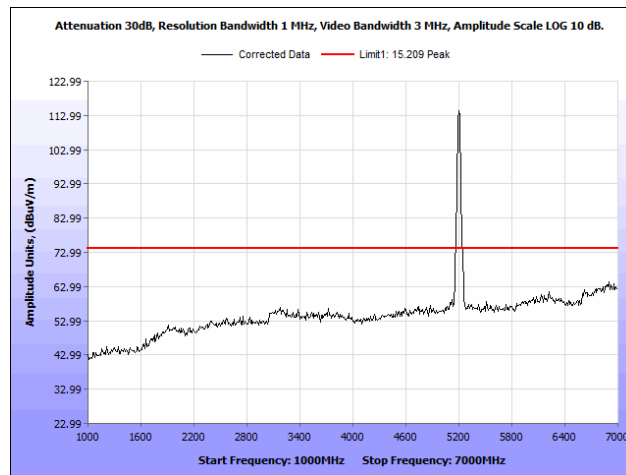
Plot 63. Radiated Spurious Emissions, 5200 MHz, PCB Antenna, 1 GHz – 7 GHz, Peak
