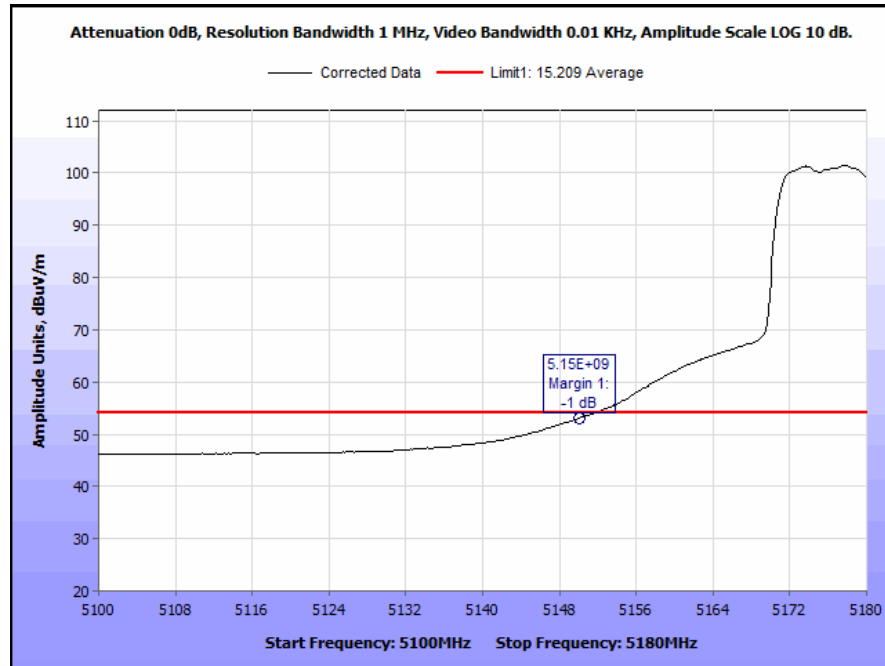
Plot 85. Radiated Band Edge, 5180 MHz @ 5150 MHz, Average, PCB Antenna
