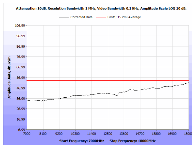
Plot 64. Radiated Spurious Emissions, 5200 MHz, PCB Antenna, 7 GHz – 18 GHz, Average
