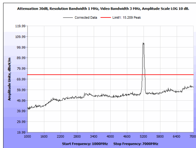
Plot 48. Radiated Spurious Emissions, 5190 MHz, Rubber Ducky Antenna, 1 GHz – 7 GHz, Peak
