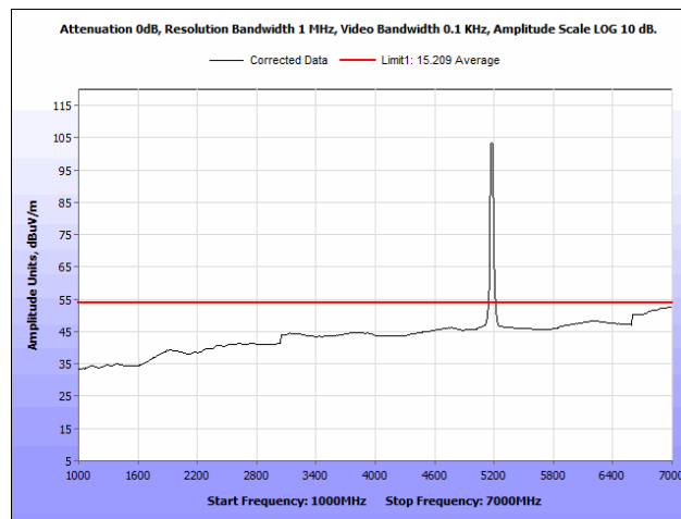
Plot 57. Radiated Spurious Emissions, 5180 MHz, PCB Antenna, 1 GHz – 7 GHz, Average
