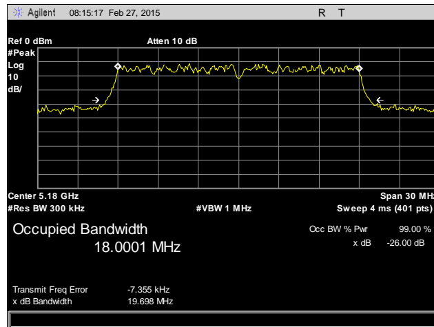
Plot 6. 26 dB Occupied Bandwidth, 5180 MHz, Antenna 2
