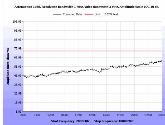
Plot 35. Radiated Spurious Emissions, 5180 MHz, Rubber Ducky Antenna, 7 GHz – 18 GHz, Peak
