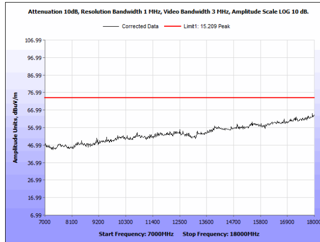
Plot 40. Radiated Spurious Emissions, 5200 MHz, Rubber Ducky Antenna, 7 GHz – 18 GHz, Peak
