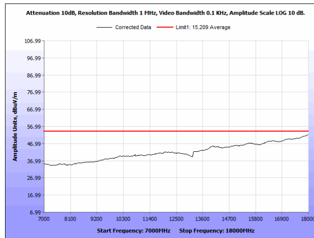
Plot 69. Radiated Spurious Emissions, 5220 MHz, PCB Antenna, 7 GHz – 18 GHz, Average
