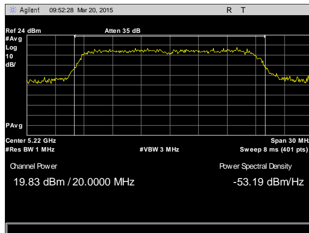
Plot 12. Peak Power Output, 5220 MHz, Antenna 1
