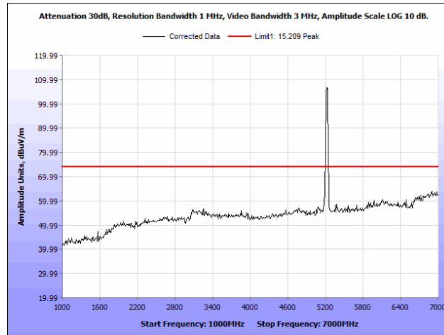
Plot 43. Radiated Spurious Emissions, 5220 MHz, Rubber Ducky Antenna, 1 GHz – 7 GHz, Peak
