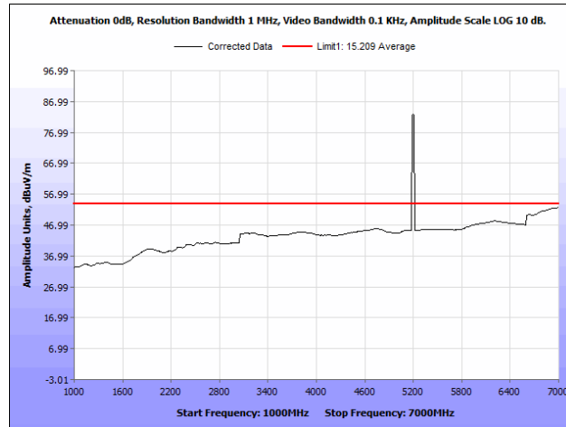
Plot 62. Radiated Spurious Emissions, 5200 MHz, PCB Antenna, 1 GHz – 7 GHz, Average
