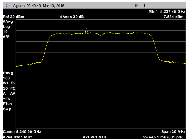
Plot 28. Peak Power Spectral Density, 5240 MHz, Antenna 2
