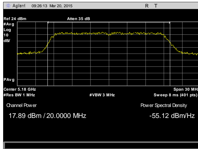
Plot 16. Peak Power Output, 5180 MHz, Antenna 2
