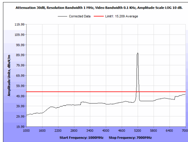
Plot 47. Radiated Spurious Emissions, 5190 MHz, Rubber Ducky Antenna, 1 GHz – 7 GHz, Average
