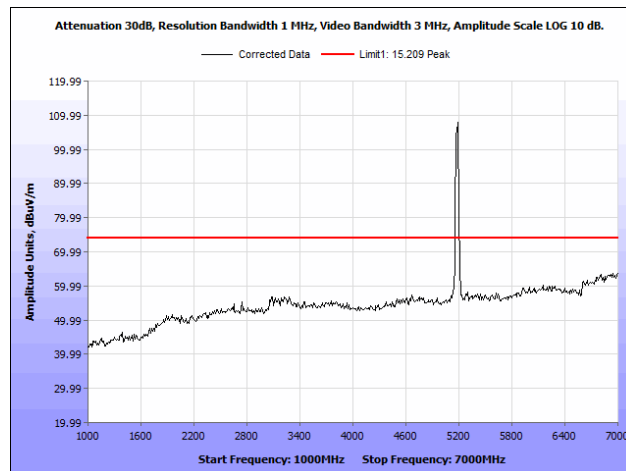
Plot 33. Radiated Spurious Emissions, 5180 MHz, Rubber Ducky Antenna, 1 GHz – 7 GHz, Peak
