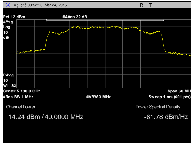
Plot 19. Peak Power Output, 5190 MHz, Antenna 2
