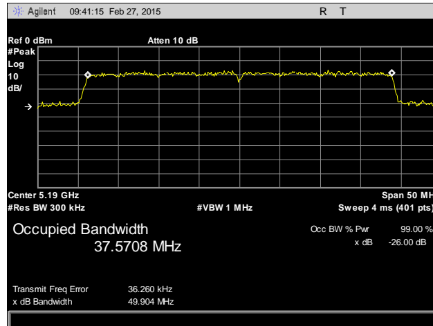
Plot 4. 26 dB Occupied Bandwidth, 5190 MHz, Antenna 1
