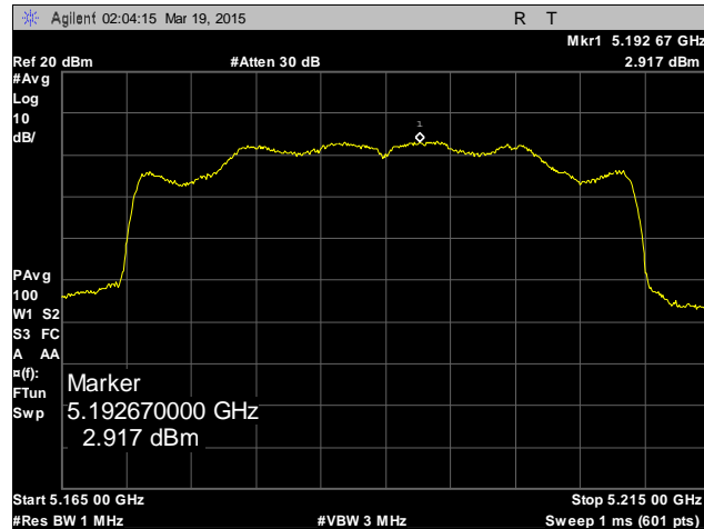
Plot 24. Peak Power Spectral Density, 5190 MHz, Antenna 1
