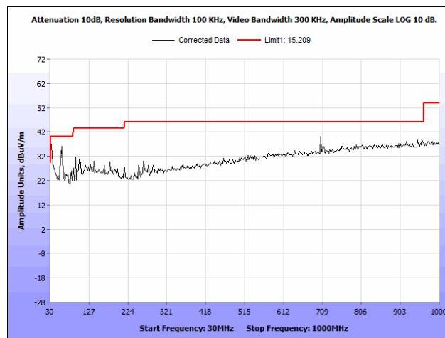
Plot 51. Radiated Spurious Emissions, 5230 MHz, Rubber Ducky Antenna, 30 MHz – 1 GHz
