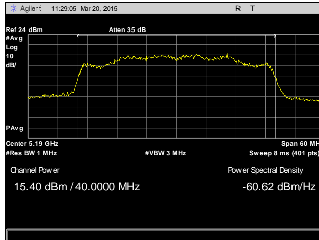
Plot 14. Peak Power Output, 5190 MHz, Antenna 1
