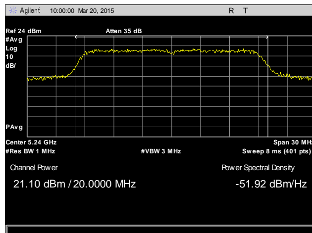
Plot 13. Peak Power Output, 5240 MHz, Antenna 1
