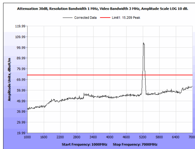
Plot 53. Radiated Spurious Emissions, 5230 MHz, Rubber Ducky Antenna, 1 GHz – 7 GHz, Peak
