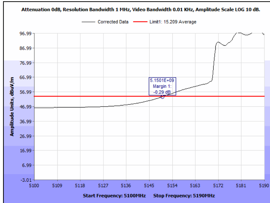
Plot 87. Radiated Band Edge, 5190 MHz @ 5150 MHz, Average, PCB Antenna
