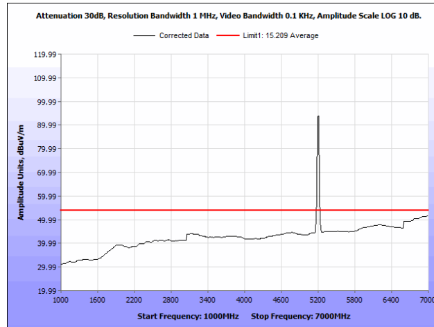
Plot 37. Radiated Spurious Emissions, 5200 MHz, Rubber Ducky Antenna, 1 GHz – 7 GHz, Average
