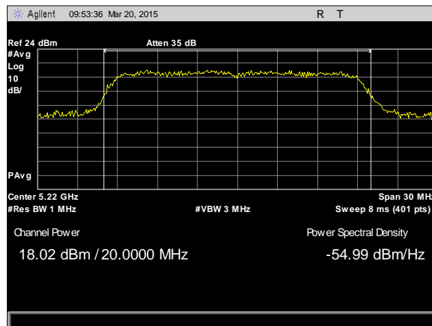
Plot 17. Peak Power Output, 5220 MHz, Antenna 2
