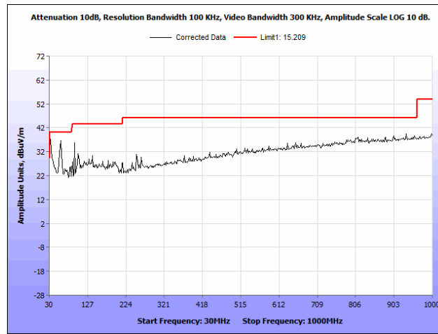
Plot 56. Radiated Spurious Emissions, 5180 MHz, PCB Antenna, 30 MHz – 1 GHz
