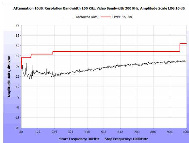
Plot 76. Radiated Spurious Emissions, 5230 MHz, PCB Antenna, 30 MHz – 1 GHz
