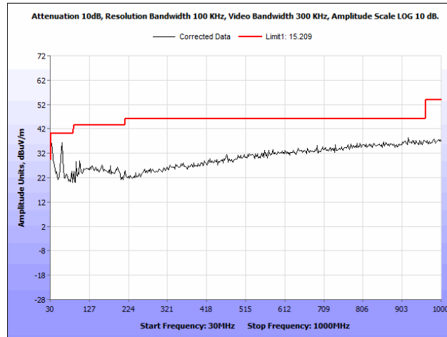
Plot 46. Radiated Spurious Emissions, 5190 MHz, Rubber Ducky Antenna, 30 MHz – 1 GHz
