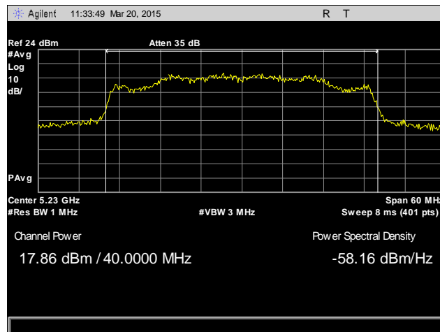
Plot 20. Peak Power Output, 5230 MHz, Antenna 2
