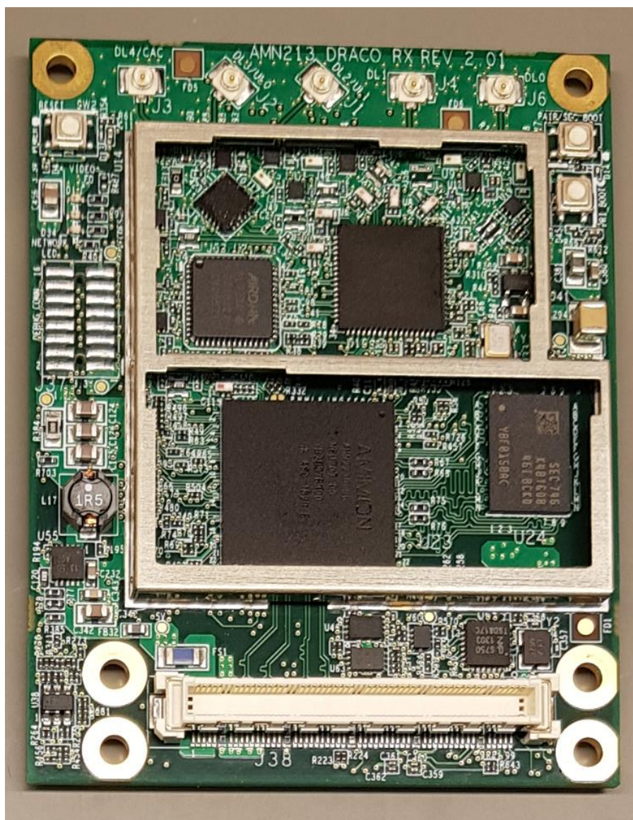
Figure 1- AMN42012 – Top View without shields
