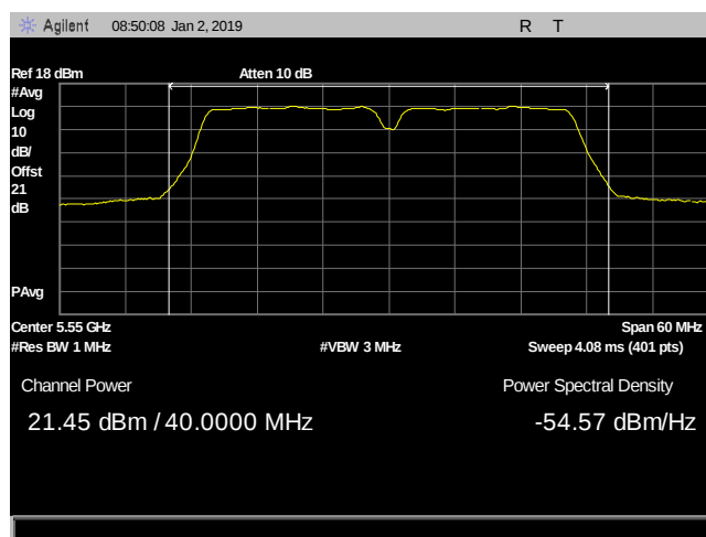
Plot 17. Output Power, UNII 2C, 2 dBi configuration, CF 5550 MHz
