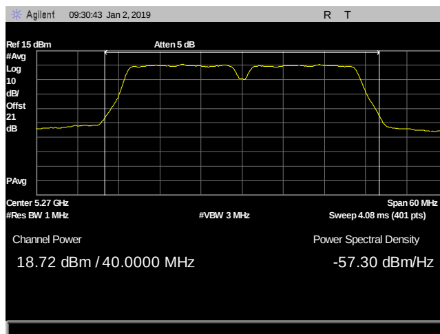
Plot 8. Output Power, UNII 2A, 11 dBi configuration, CF 5270 MHz
