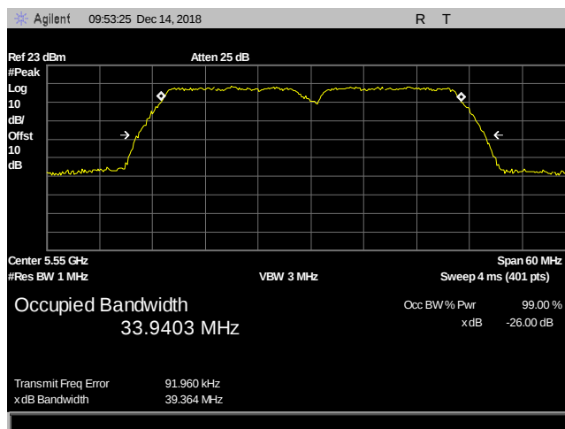
Plot 4. 26 dB Occupied Bandwidth, UNII 2C, 40 MHz, 5550 MHz, J2
