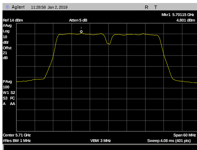
Plot 27. Power Spectral Density, UNII 2C, 11 dBi configuration, CF 5710 MHz
