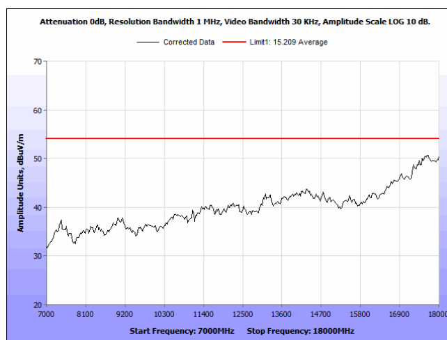
Plot 63. Unwanted Emissions, 2 dBi, Average, CF 5550 MHz, 7 – 18 GHz
