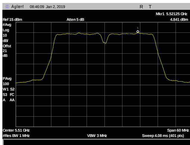
Plot 28. Power Spectral Density, UNII 2C, 2 dBi configuration, CF 5510 MHz
