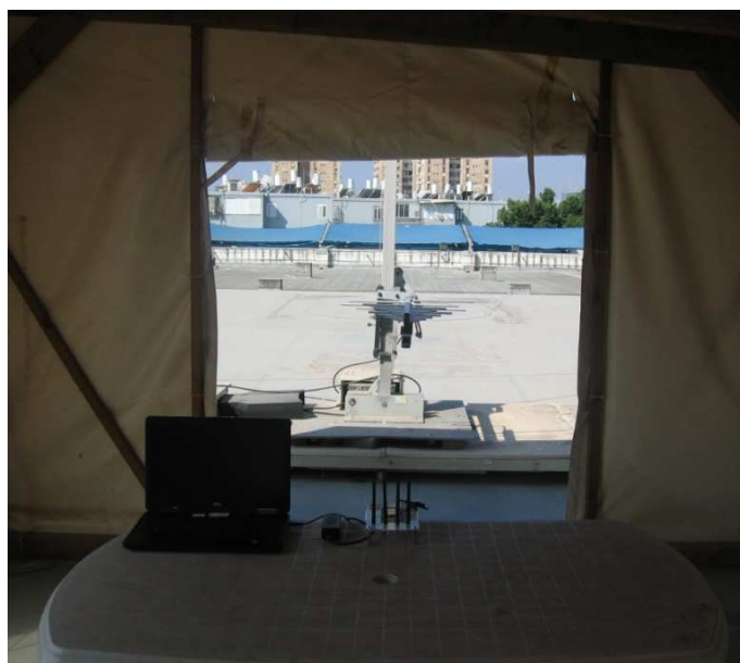
Figure 5: RE 200MHz – 1GHz - Test Setup
