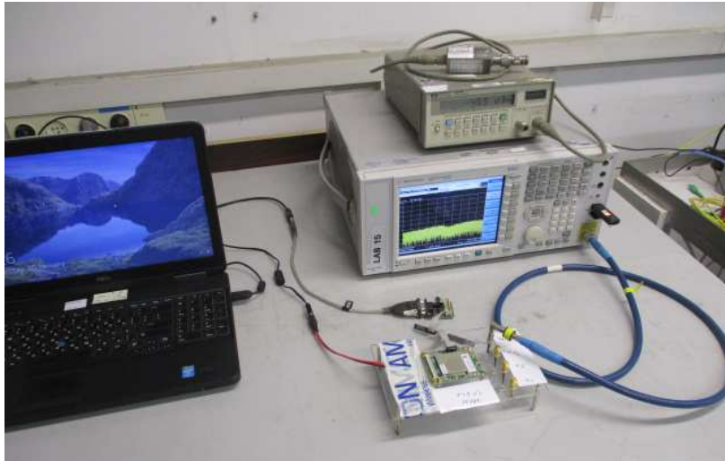
Figure 1: Conducted Measurements- Test Setup
