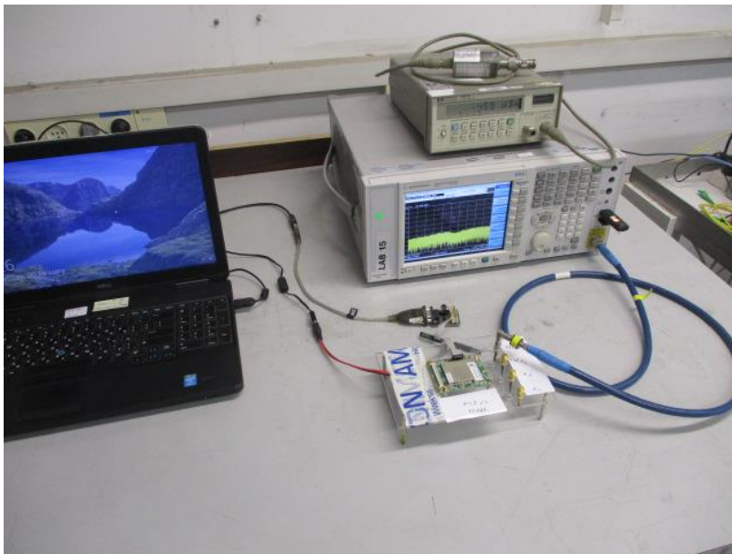
Figure 2. Conducted Emission Test (with Spectrum Analyzer)
