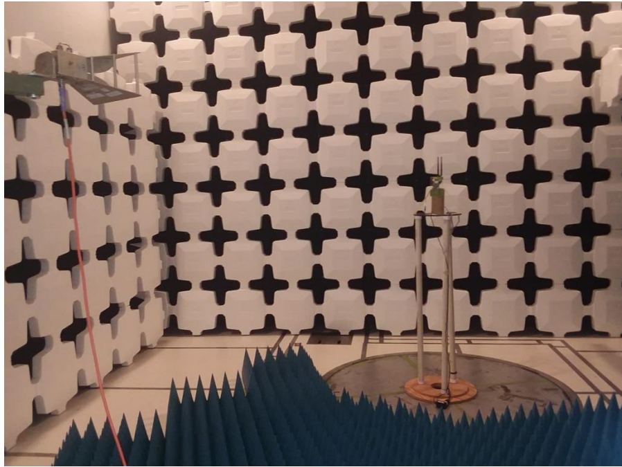
Photograph 3. Radiated Emissions, 2x2 Test Setup Above 1GHz
