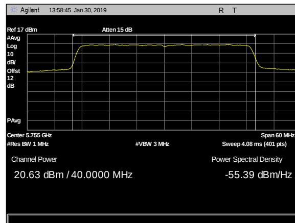
Plot 9. Output Power, 2dBi & 5dBi 4x4, 5755MHz, c2
