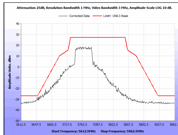
Plot 56. Radiated Band Edge, UNII3-mask, 5725, BW40M, CF5755MHz, 2x2, 5dBi
