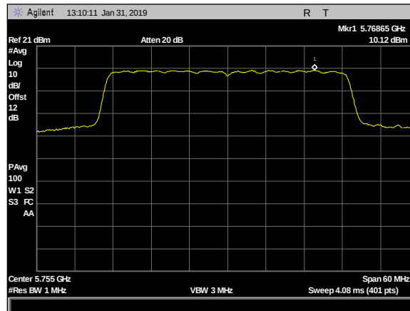
Plot 19. Power Spectral Density, 2dBi & 5dBi- 2x2, 5755MHz, c2
