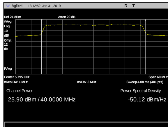
Plot 6. Output Power, 2dBi & 5dBi- 2x2, 5795MHz, c1
