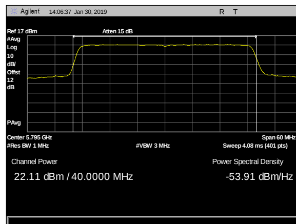
Plot 14. Output Power, 2dBi & 5dBi 4x4, 5795MHz, c3
