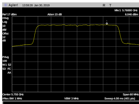
Plot 21. Power Spectral Density, 2dBi & 5dBi- 4x4, 5755MHz, c2
