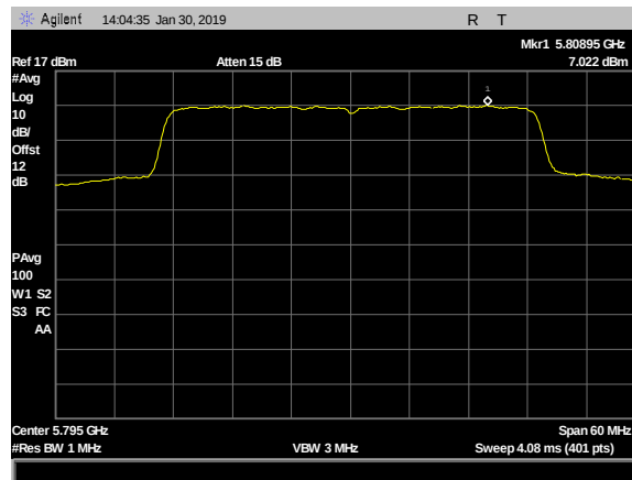
Plot 25. Power Spectral Density, 2dBi & 5dBi- 4x4, 5795MHz, c2
