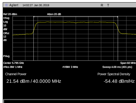
Plot 12. Output Power, 2dBi & 5dBi 4x4, 5795MHz, c1
