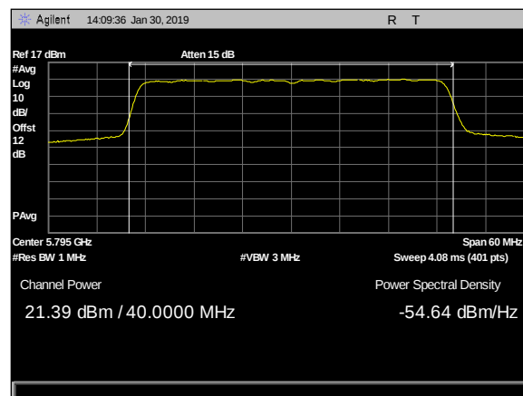
Plot 15. Output Power, 2dBi & 5dBi 4x4, 5795MHz, c4
