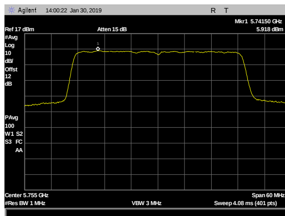
Plot 20. Power Spectral Density, 2dBi & 5dBi- 4x4, 5755MHz, c1
