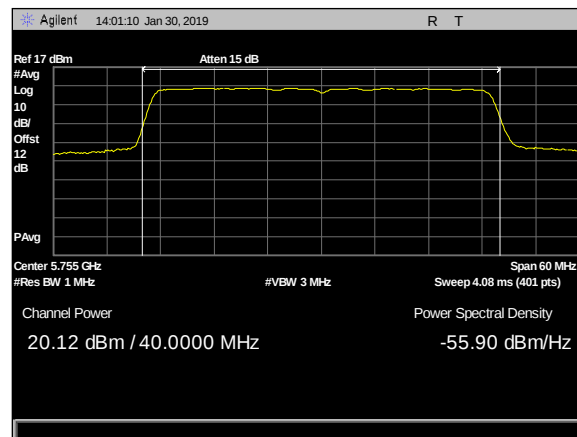
Plot 8. Output Power, 2dBi & 5dBi 4x4, 5755MHz, c1
