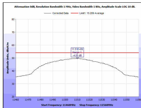
Plot 42. Undesirable Emissions, Average, 4x4, 5dBi, 5755, 7-18GHz, 11.51GHz spur
