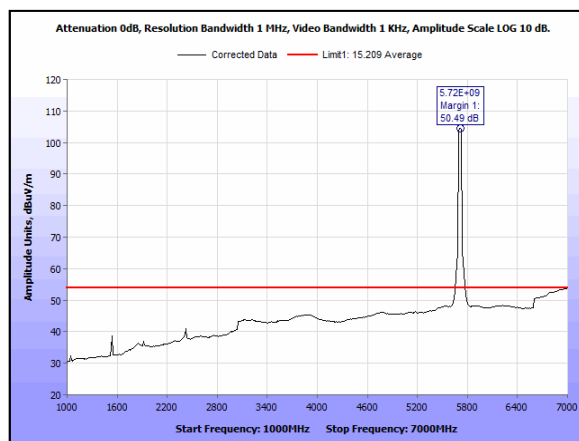
Plot 190. Radiated Emissions, Average, 4x4, 5dBi, 5710, 1-7GHz
