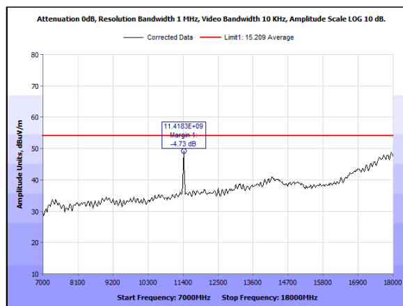
Plot 191. Radiated Emissions, Average, 4x4, 5dBi, 5710, 7-18GHz
