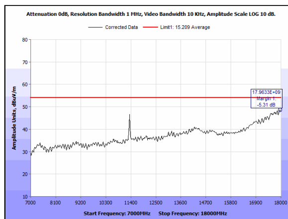
Plot 189. Radiated Emissions, Average, 4x4, 5dBi, 5670, 7-18GHz
