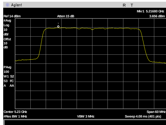
Plot 34. Power Spectral Density, 5dBi - 2x2 - 5230MHz - c1
