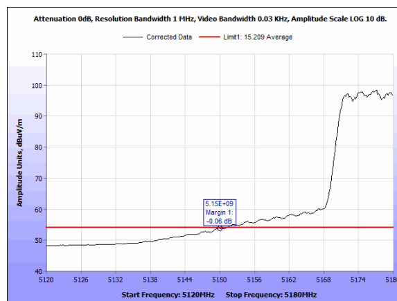
Plot 78. Radiated Bandedge, Average, 5150, BW40M, CF5190MHz, 2x2, 5dBi
