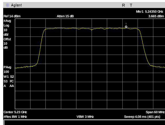
Plot 35. Power Spectral Density, 5dBi - 2x2 - 5230MHz - c2
