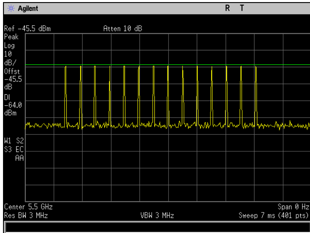
Plot 5. DFS Radar Waveform Calibration, 5500 MHz, Radar Type 4
