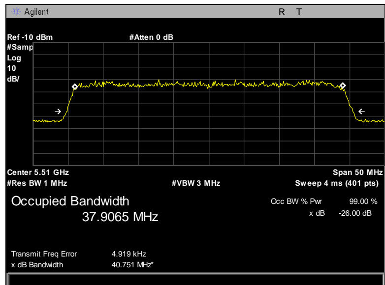
Plot 9. 99% Bandwidth, 40 MHz
