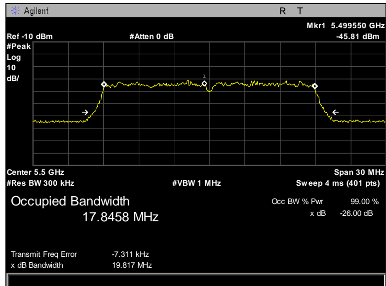
Plot 8. 99% Bandwidth, 20 MHz
