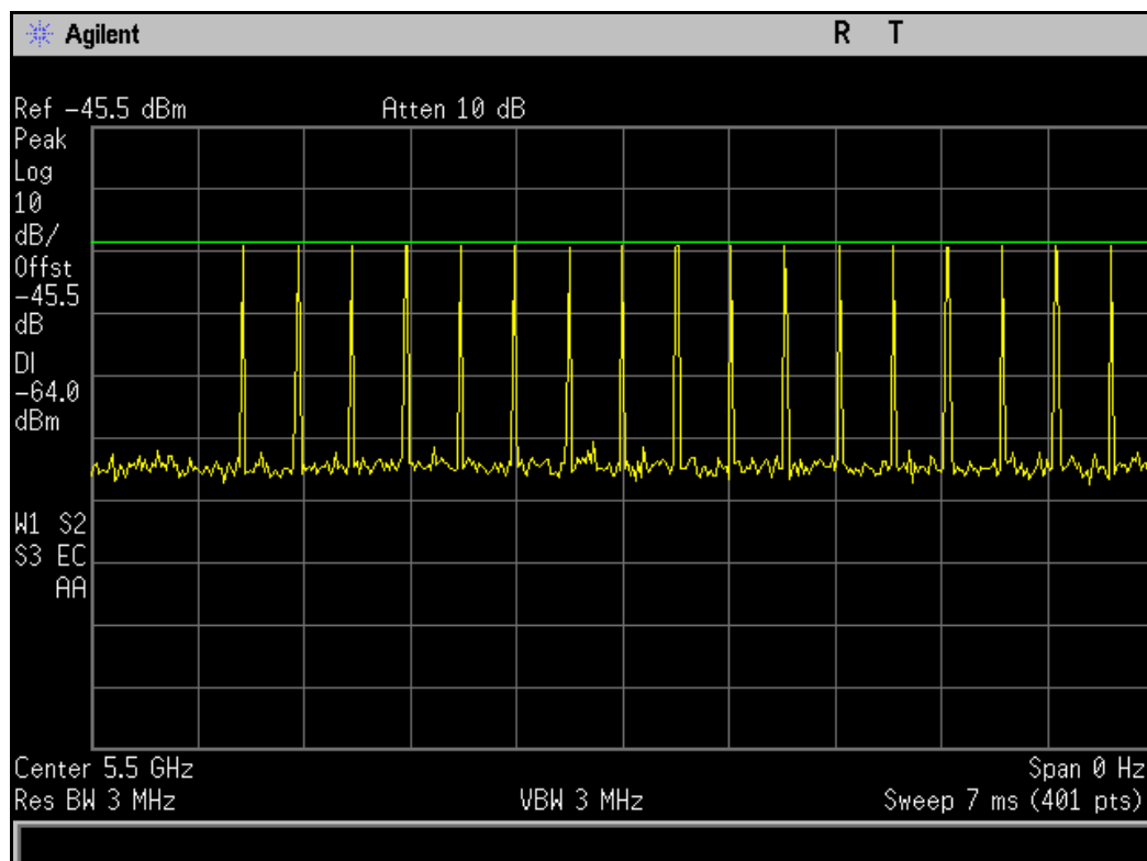
Plot 4. DFS Radar Waveform Calibration, 5500 MHz, Radar Type 3
