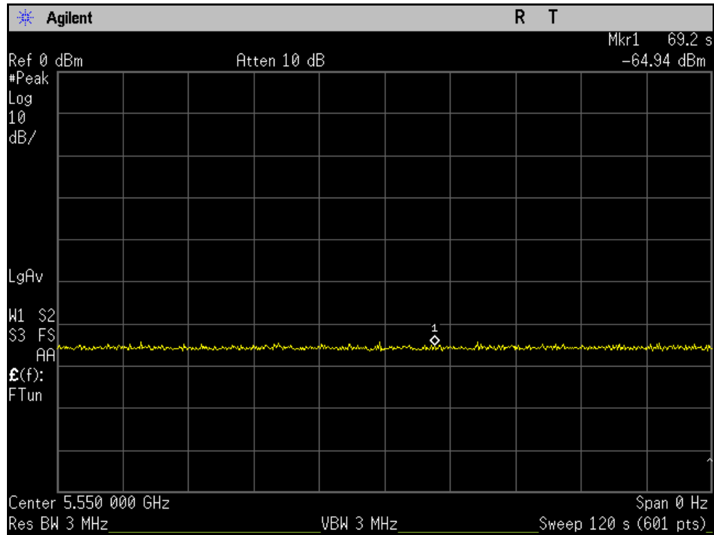
Plot 12. Channel Availability Check, Radar at End
