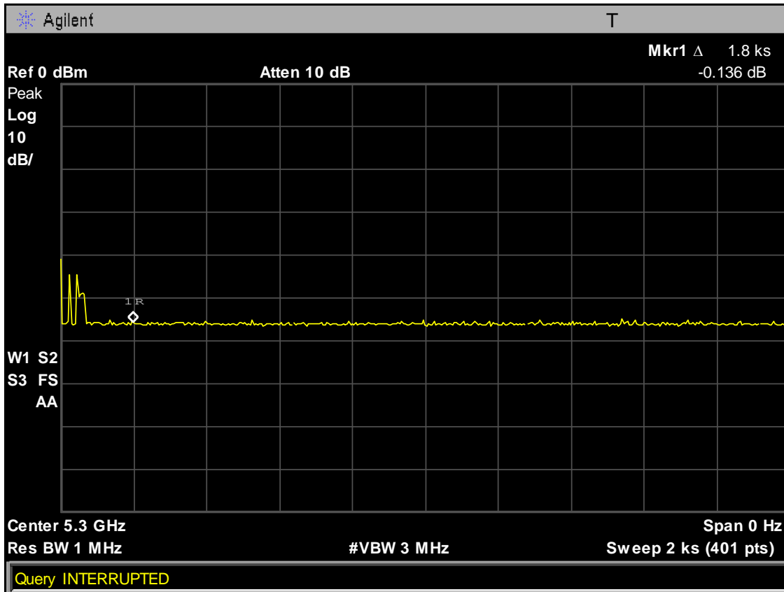
Plot 15. In-Service Monitoring for Non-Occupancy Period
