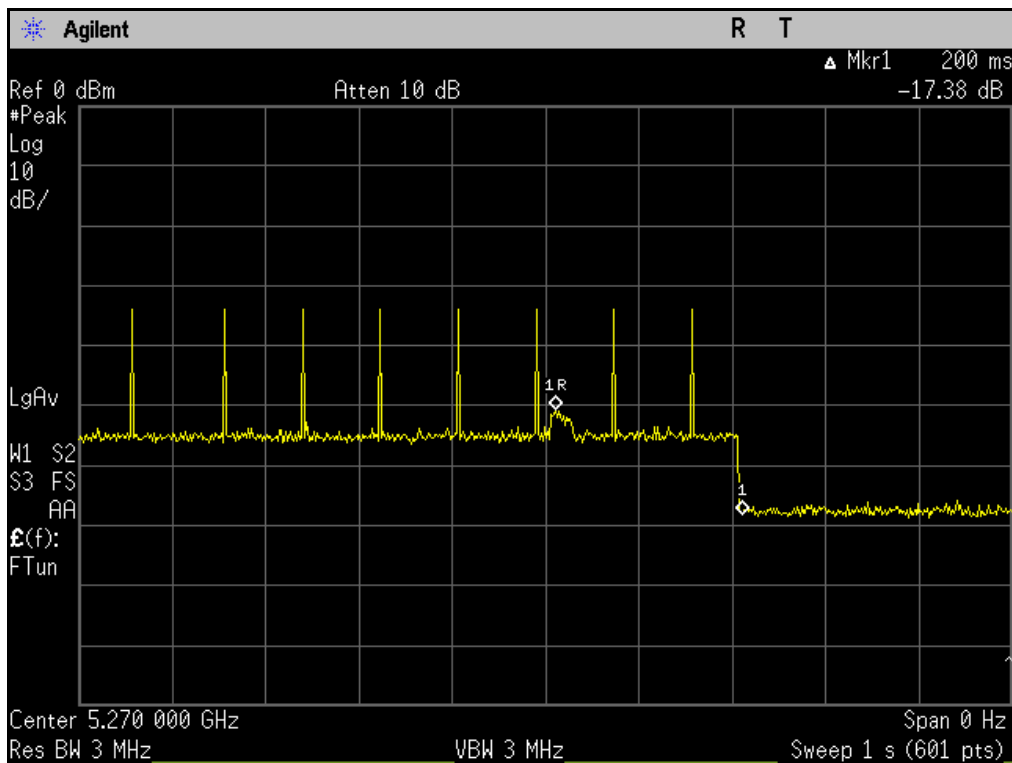
Plot 14. In-Service Monitoring for Channel Closing Transmission Time
