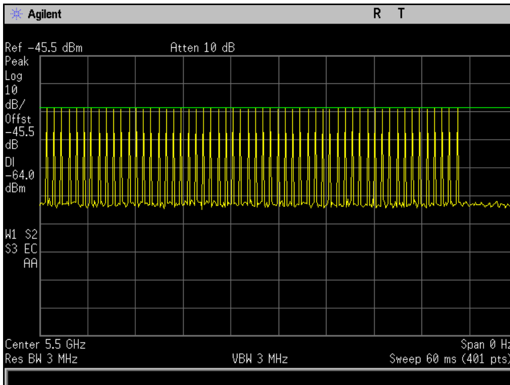
Plot 2. DFS Radar Waveform Calibration, 5500 MHz, Radar Type 1
