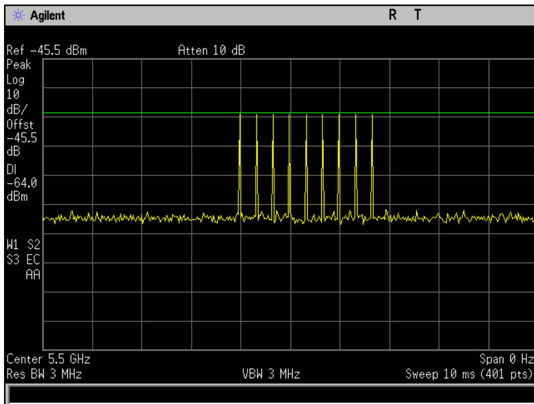
Plot 7. DFS Radar Waveform Calibration, 5500 MHz, Radar Type 6
