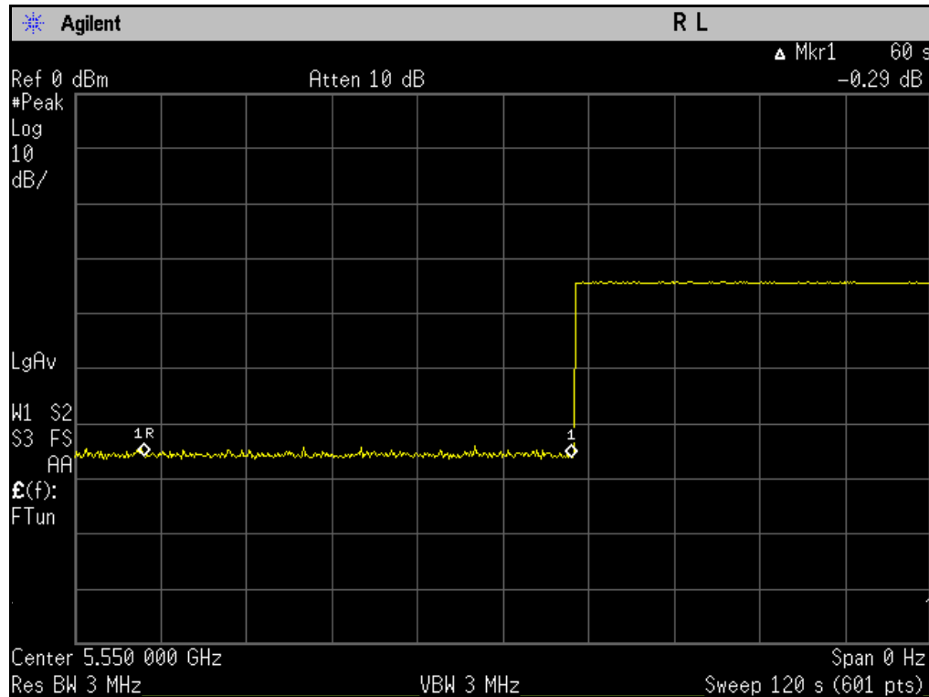
Plot 10. Channel Availability Check Time
