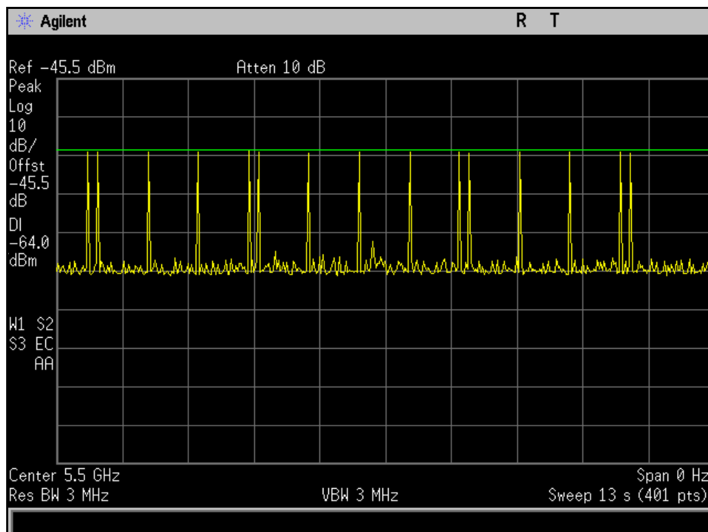
Plot 6. DFS Radar Waveform Calibration, 5500 MHz, Radar Type 5
