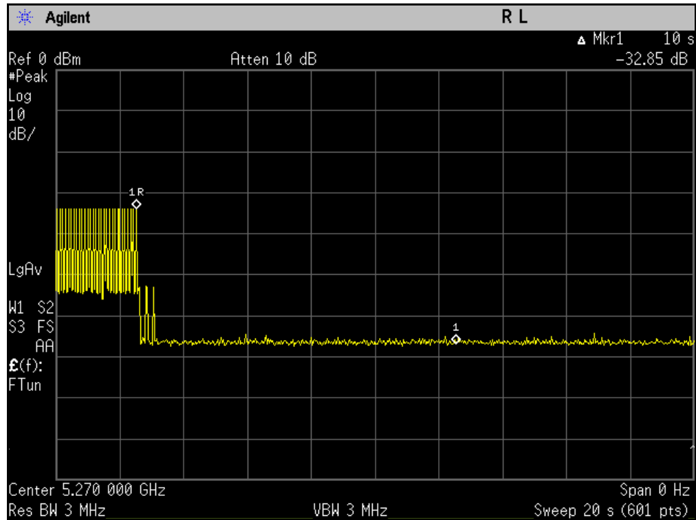
Plot 13. In-Service Monitoring for Channel Move Time
