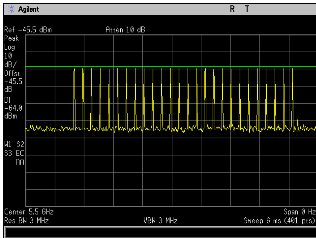
Plot 3. DFS Radar Waveform Calibration, 5500 MHz, Radar Type 2
