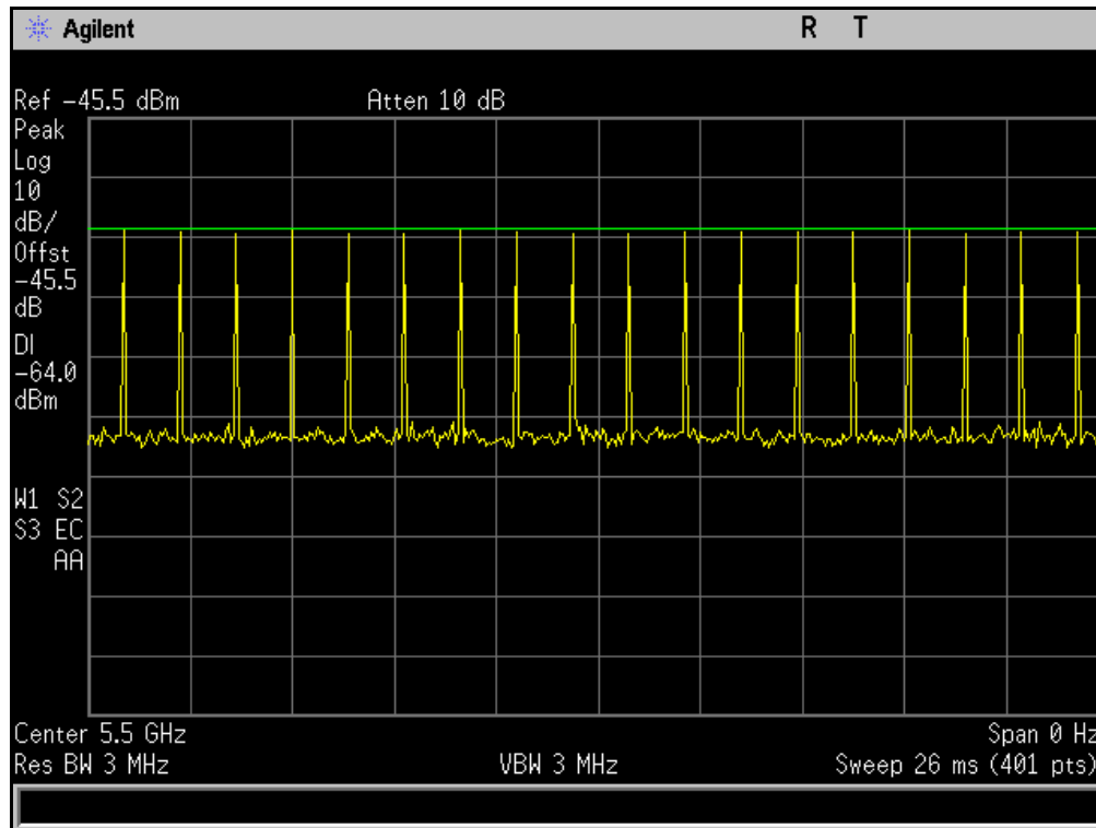
Plot 1. DFS Radar Waveform Calibration, 5500 MHz, Radar Type 0
