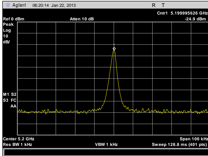
Plot 52. Frequency Stability, 5200 MHz, -10°C, 120 V
