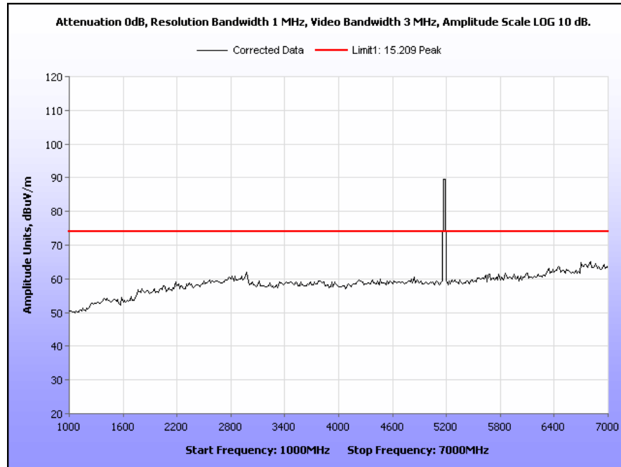
Plot 28. Radiated Spurious Emissions, 5180 MHz, 20 MHz Channel, 1 GHz – 7 GHz, Peak
