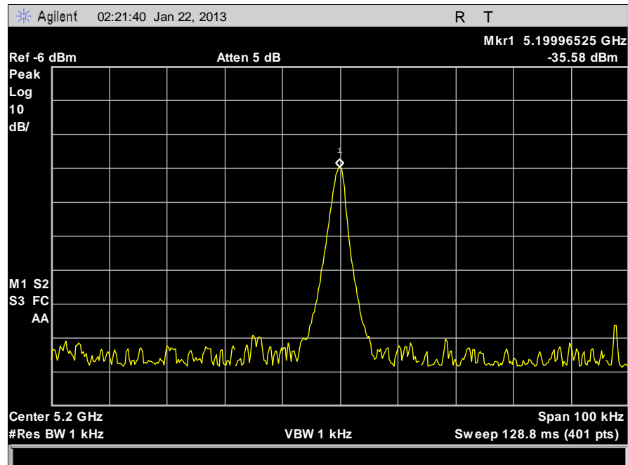
Plot 57. Frequency Stability, 5200 MHz, 20°C, 132 V
