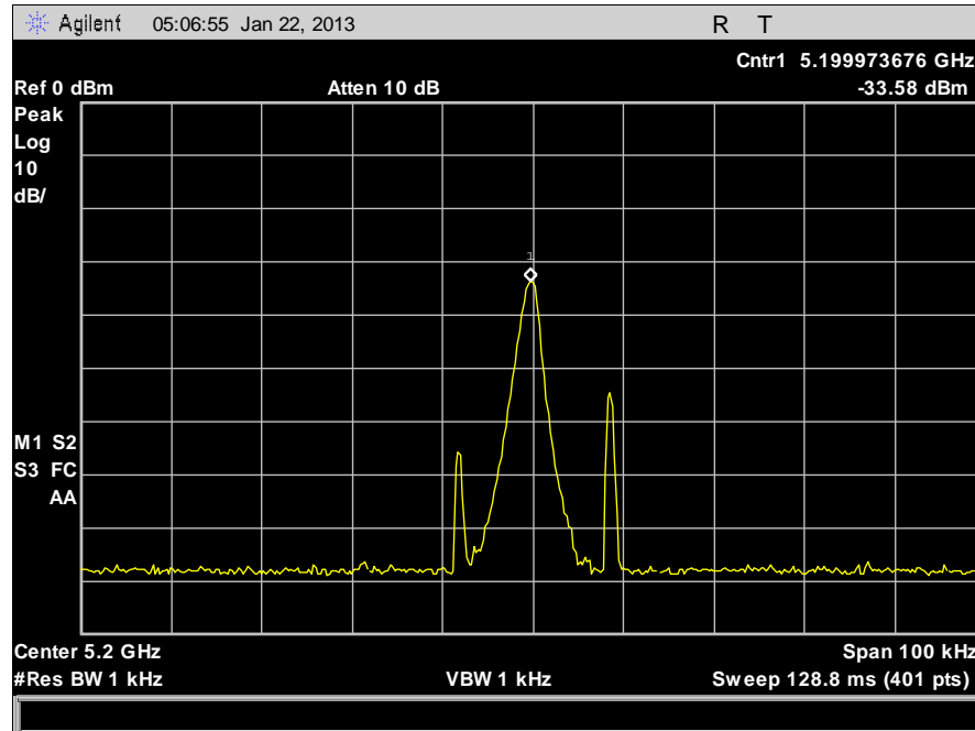
Plot 54. Frequency Stability, 5200 MHz, 10°C, 120 V
