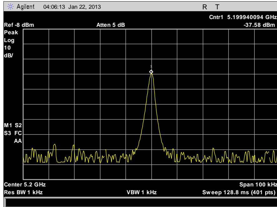
Plot 60. Frequency Stability, 5200 MHz, 50°C, 120 V
