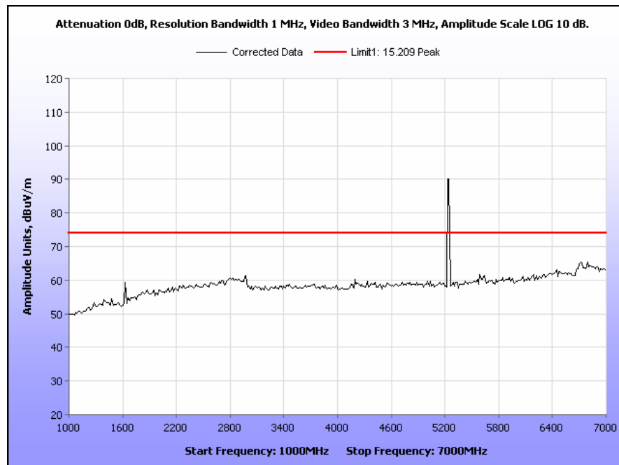
Plot 37. Radiated Spurious Emissions, 5240 MHz, 20 MHz Channel, 1 GHz – 7 GHz, Peak
