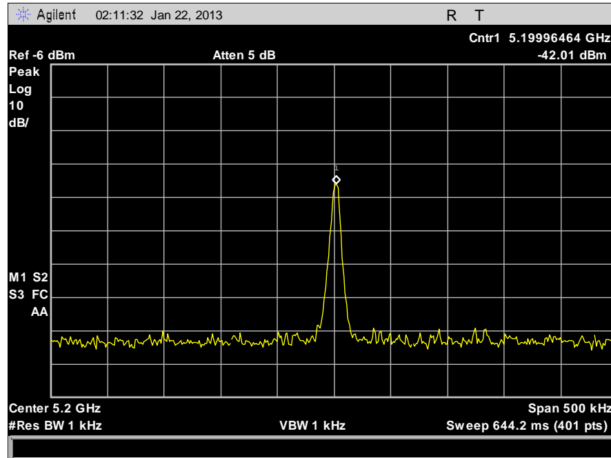
Plot 56. Frequency Stability, 5200 MHz, 20°C, 120 V
