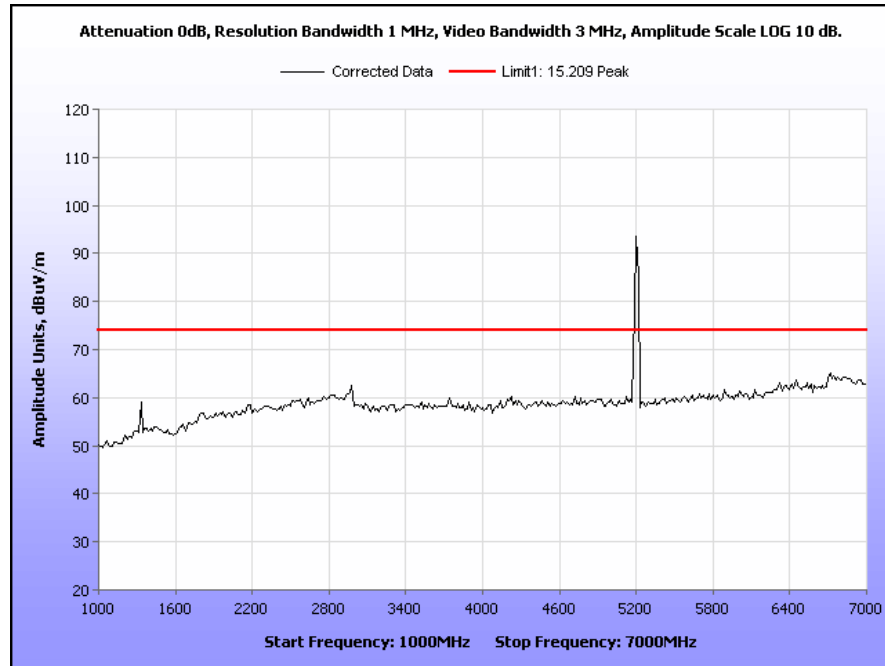
Plot 32. Radiated Spurious Emissions, 5200 MHz, 20 MHz Channel, 1 GHz – 7 GHz, Peak
