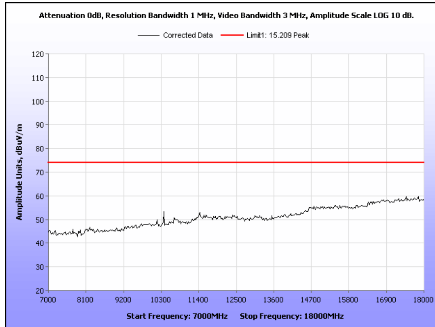
Plot 34. Radiated Spurious Emissions, 5200 MHz, 20 MHz Channel, 7 GHz – 18 GHz, Peak
