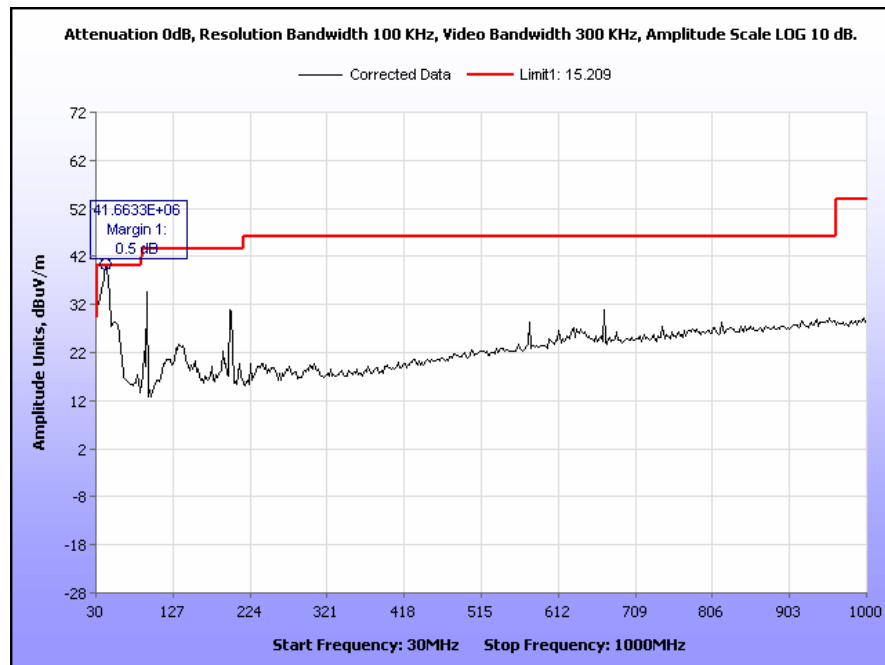
Plot 35. Radiated Spurious Emissions, 5240 MHz, 20 MHz Channel, Tx Power 13, 30 MHz – 1 GHz
