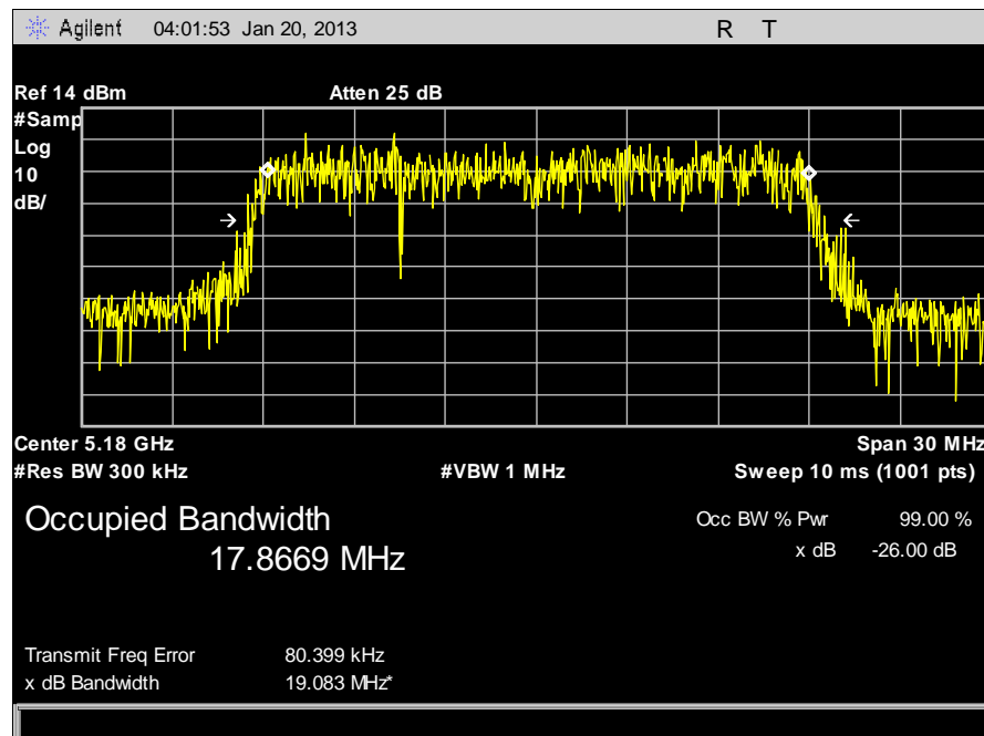
Plot 9. Occupied Bandwidth, 5180 MHz, 99%
