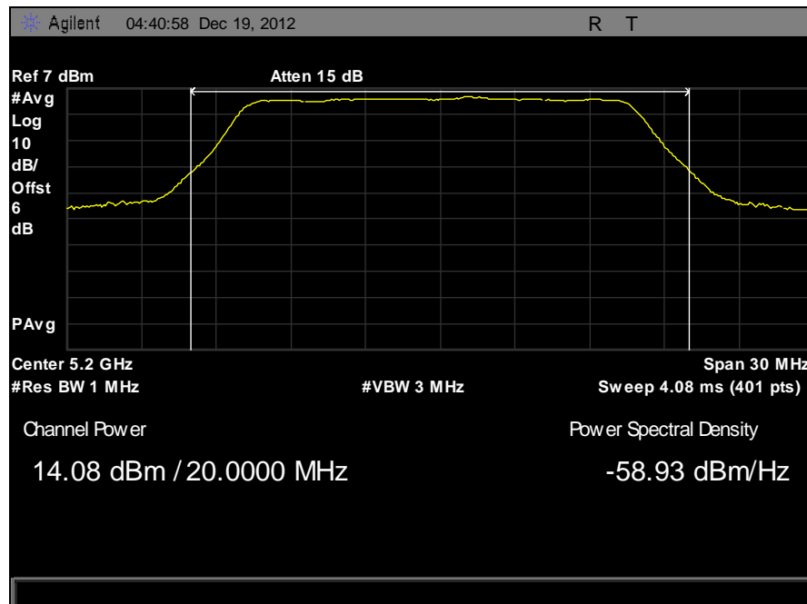
Plot 15. Peak Output Power, 5200 MHz 20 MHz
