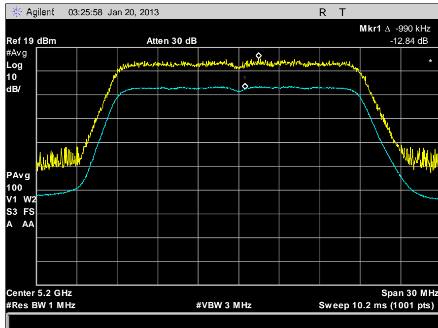
Plot 24. Peak Excursion Ratio, 5200 MHz, PX
