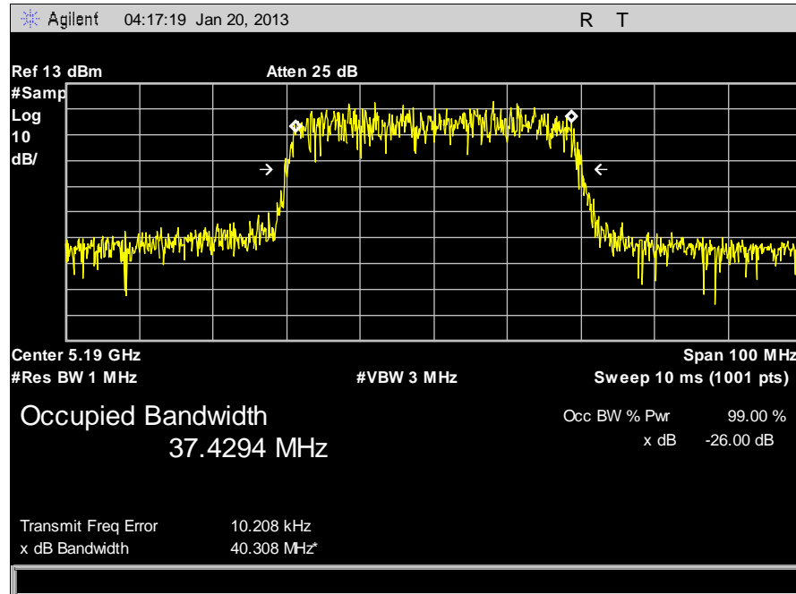
Plot 10. Occupied Bandwidth, 5190 MHz, 99%
