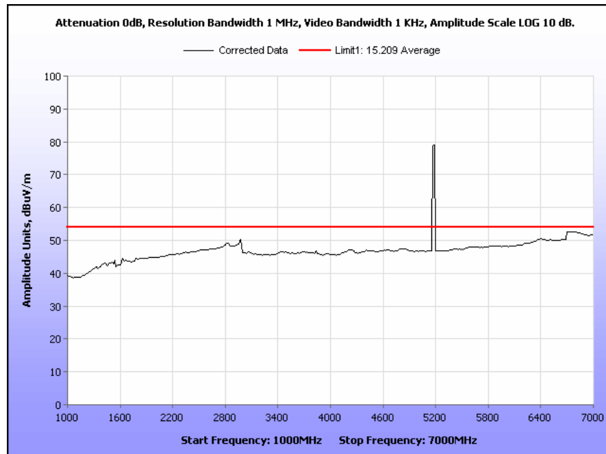
Plot 27. Radiated Spurious Emissions, 5180 MHz, 20 MHz Channel, 1 GHz – 7 GHz, Average
