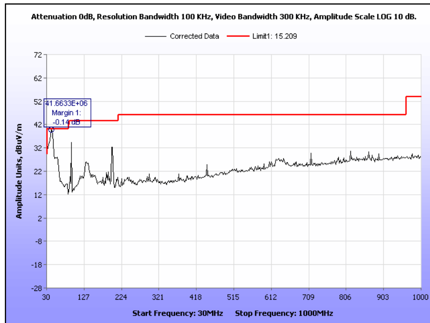
Plot 45. Radiated Spurious Emissions, 5230 MHz, 40 MHz Channel, Tx Power 14, 30 MHz – 1 GHz
