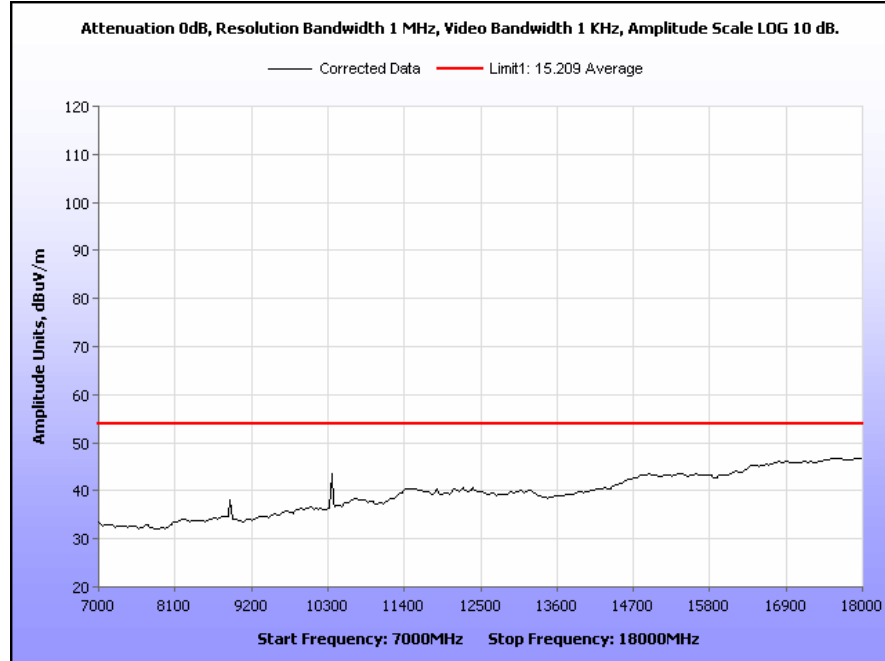
Plot 33. Radiated Spurious Emissions, 5200 MHz, 20 MHz Channel, 7 GHz – 18 GHz, Average
