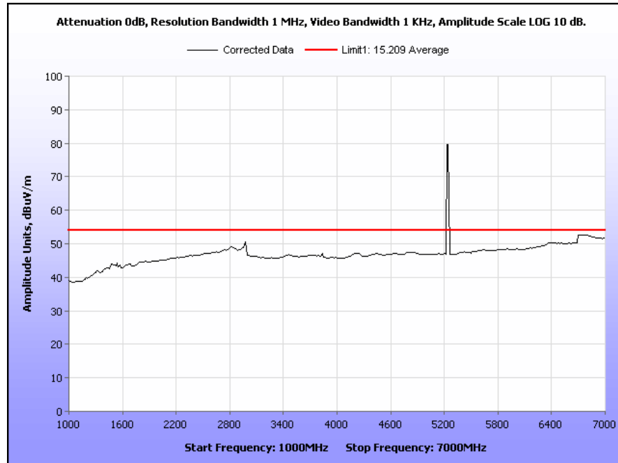
Plot 36. Radiated Spurious Emissions, 5240 MHz, 20 MHz Channel, 1 GHz – 7 GHz, Average
