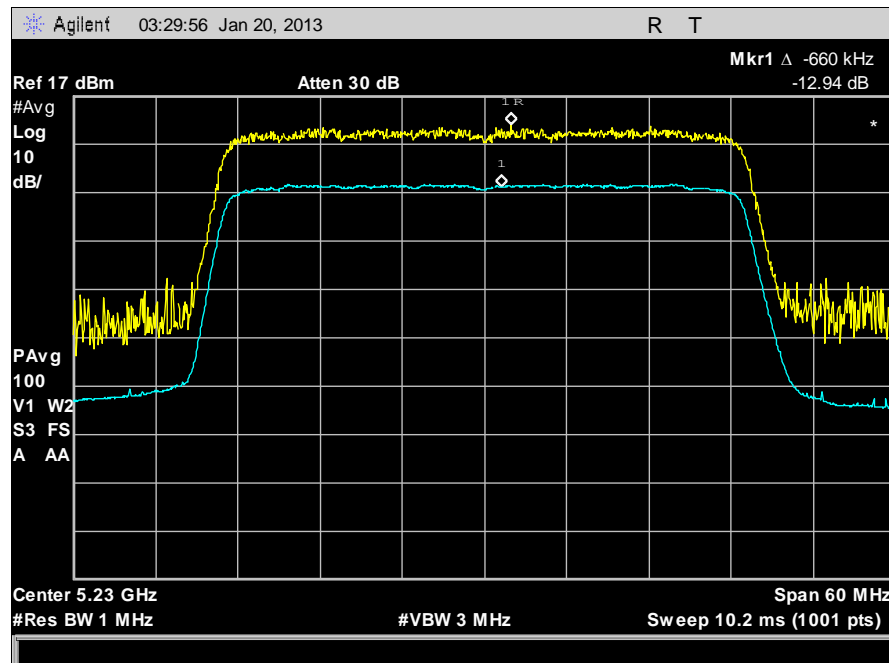
Plot 25. Peak Excursion Ratio, 5230 MHz, PX
