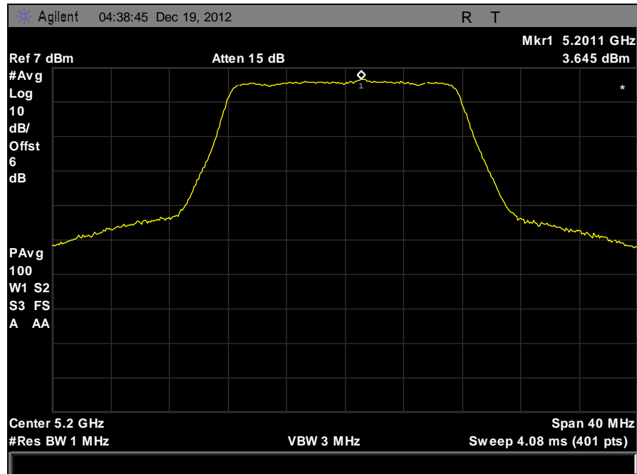
Plot 20. Peak Power Spectral Density, 5200 MHz 20 MHz
