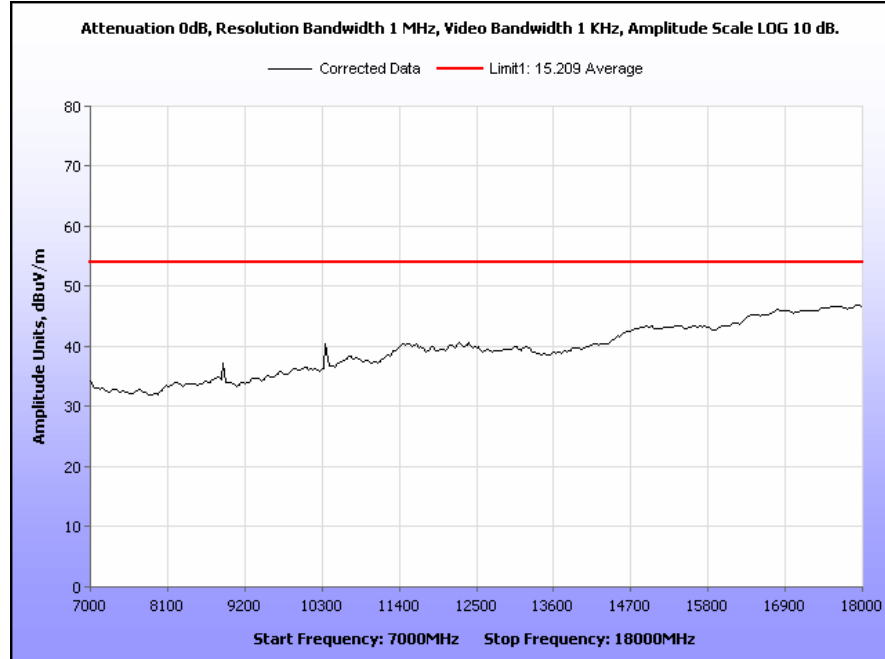
Plot 29. Radiated Spurious Emissions, 5180 MHz, 20 MHz Channel, 7 GHz – 18 GHz, Average
