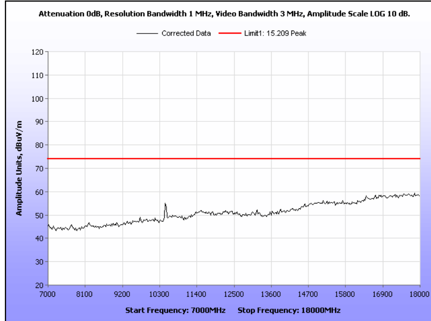
Plot 49. Radiated Spurious Emissions, 5230 MHz, 40 MHz Channel, 7 GHz – 18 GHz, Peak
