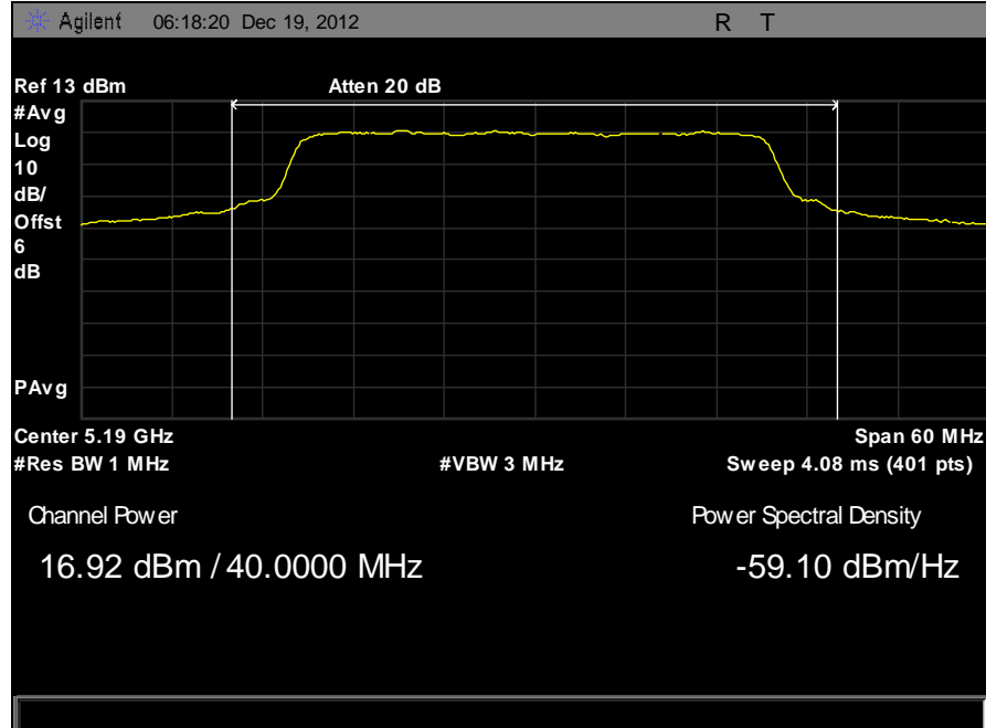
Plot 17. Peak Output Power, 5190 MHz 40 MHz
