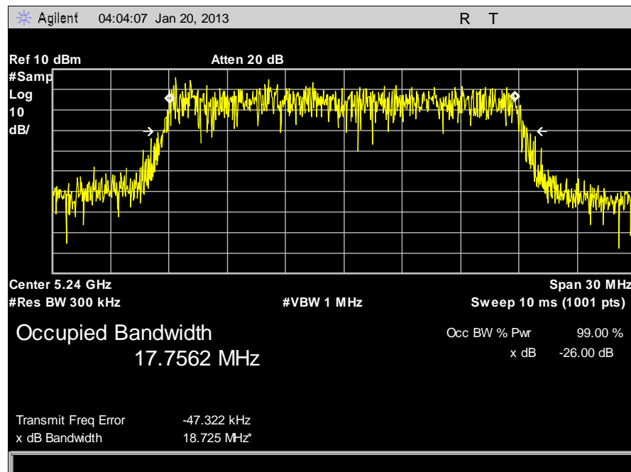
Plot 13. Occupied Bandwidth, 5240 MHz, 99%
