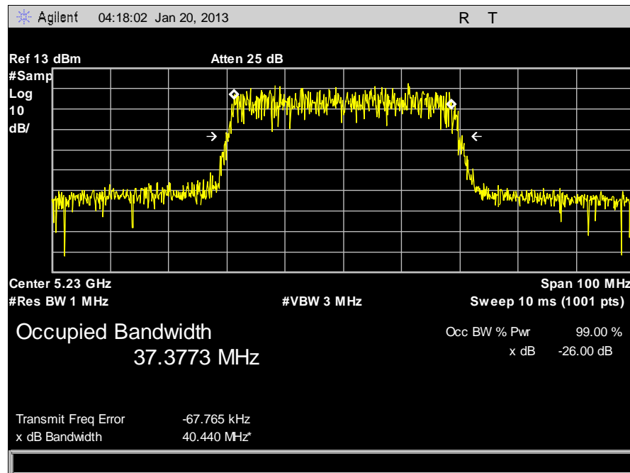
Plot 12. Occupied Bandwidth, 5230 MHz, 99%
