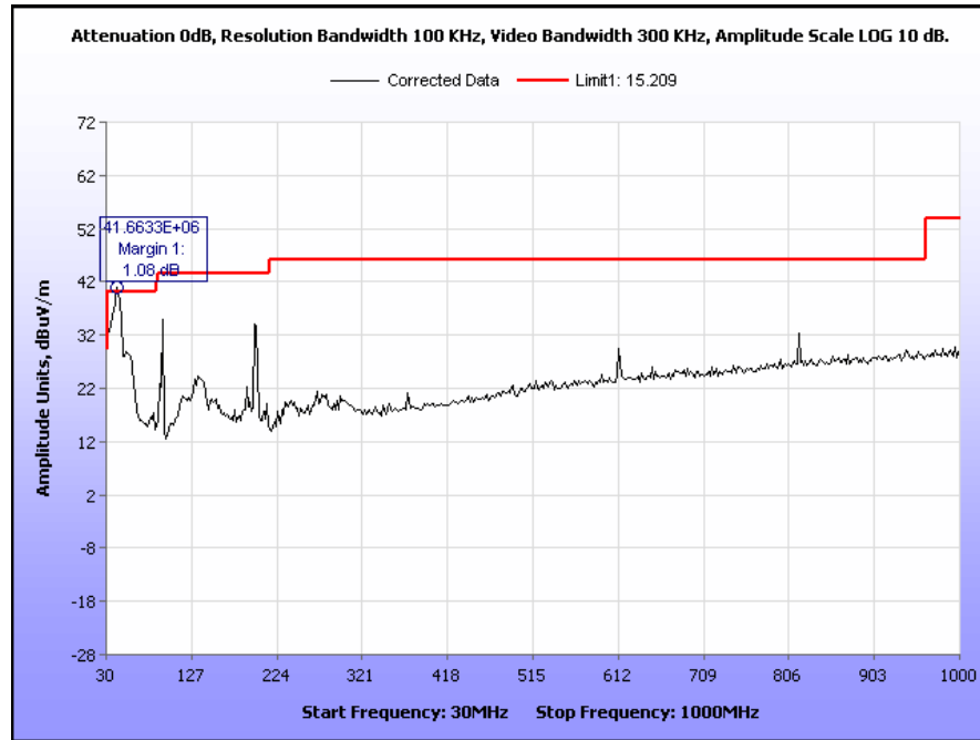
Plot 26. Radiated Spurious Emissions, 5180 MHz, 20 MHz Channel, Tx Power 13, 30 MHz – 1 GHz
