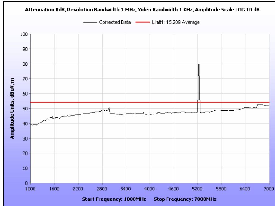
Plot 46. Radiated Spurious Emissions, 5230 MHz, 40 MHz Channel, 1 GHz – 7 GHz, Average
