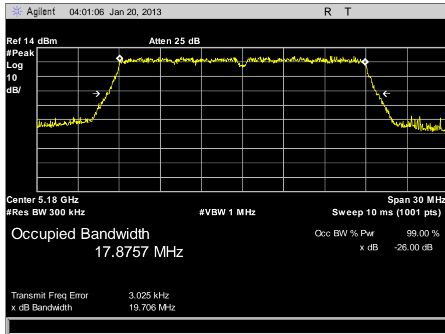
Plot 6. Occupied Bandwidth, 5180 MHz, 26 dB
