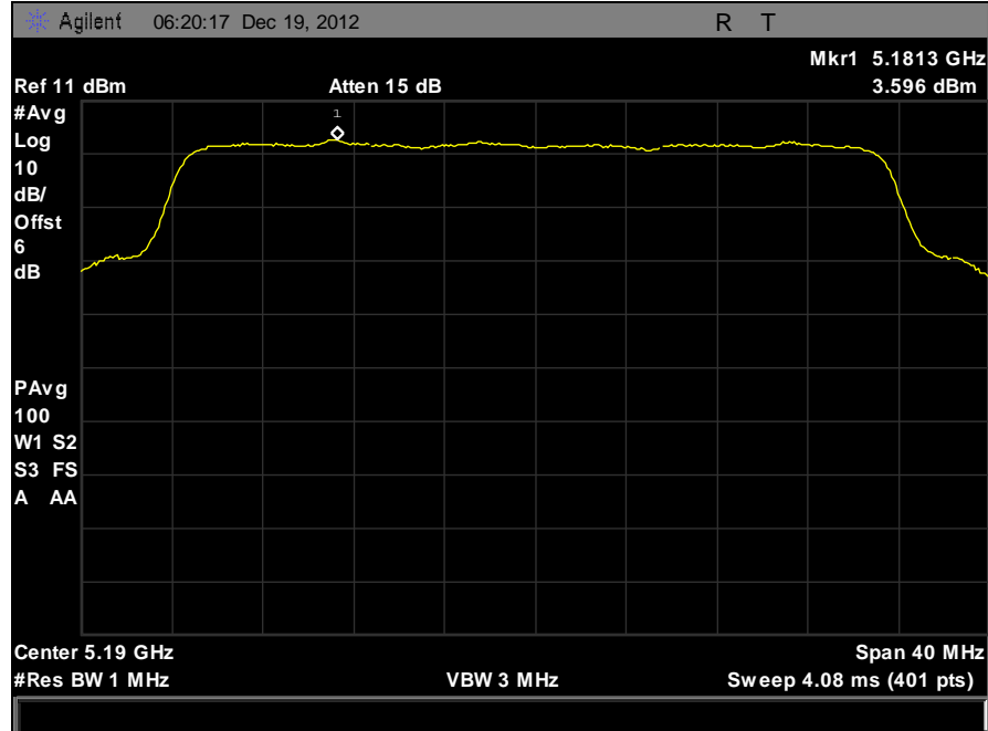
Plot 22. Peak Power Spectral Density, 5190 MHz 40 MHz
