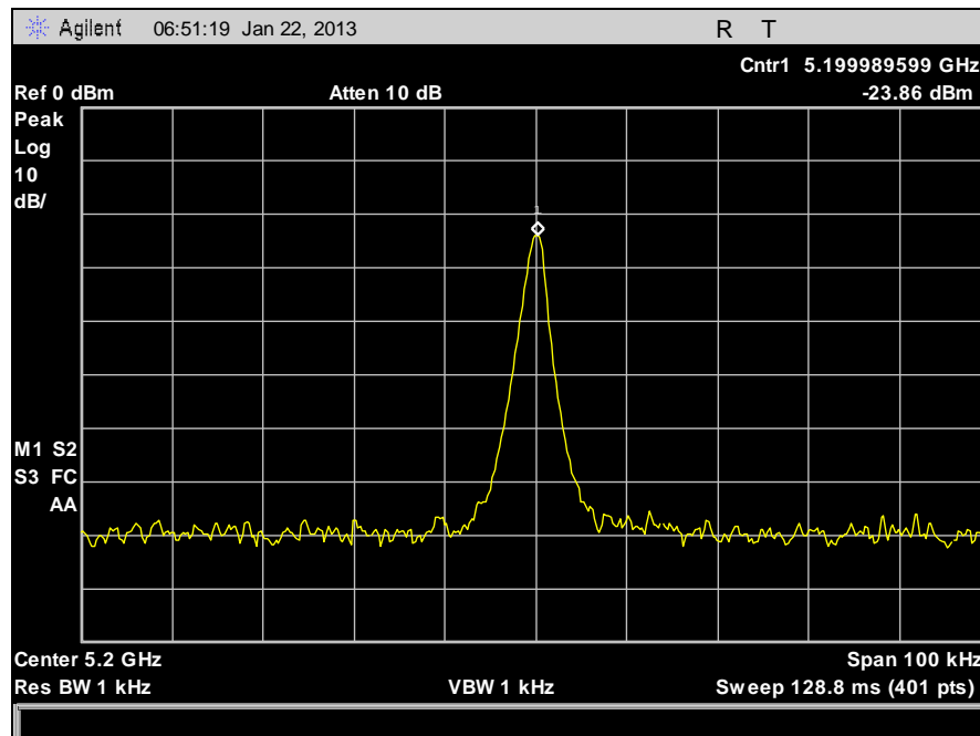
Plot 51. Frequency Stability, 5200 MHz, -20°C, 120 V
