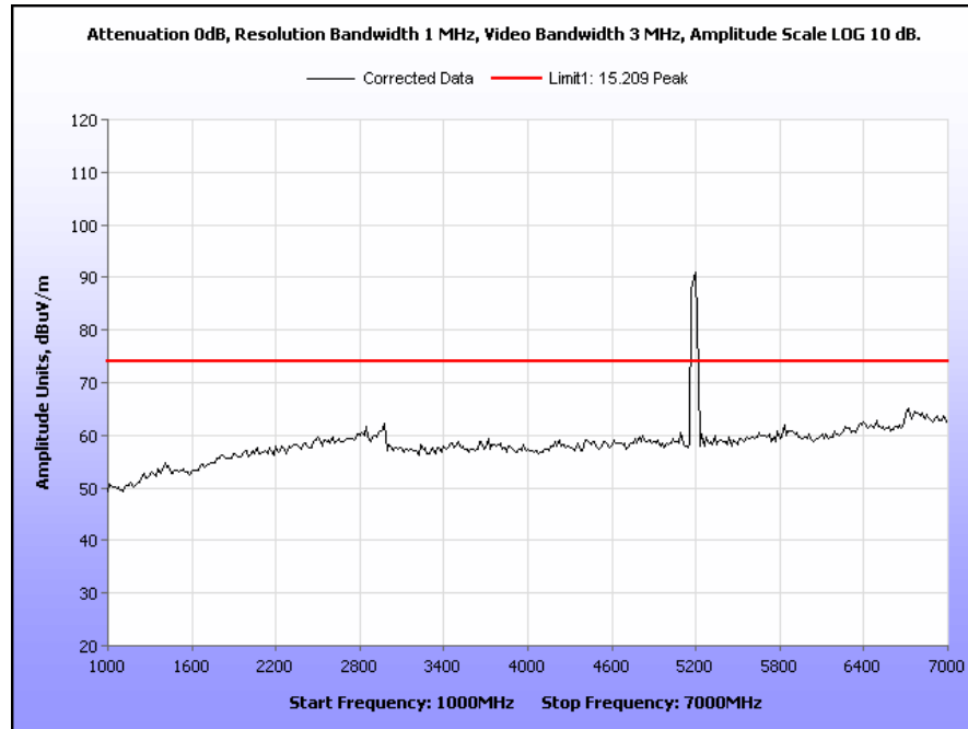
Plot 42. Radiated Spurious Emissions, 5190 MHz, 40 MHz Channel, 1 GHz – 7 GHz, Peak
