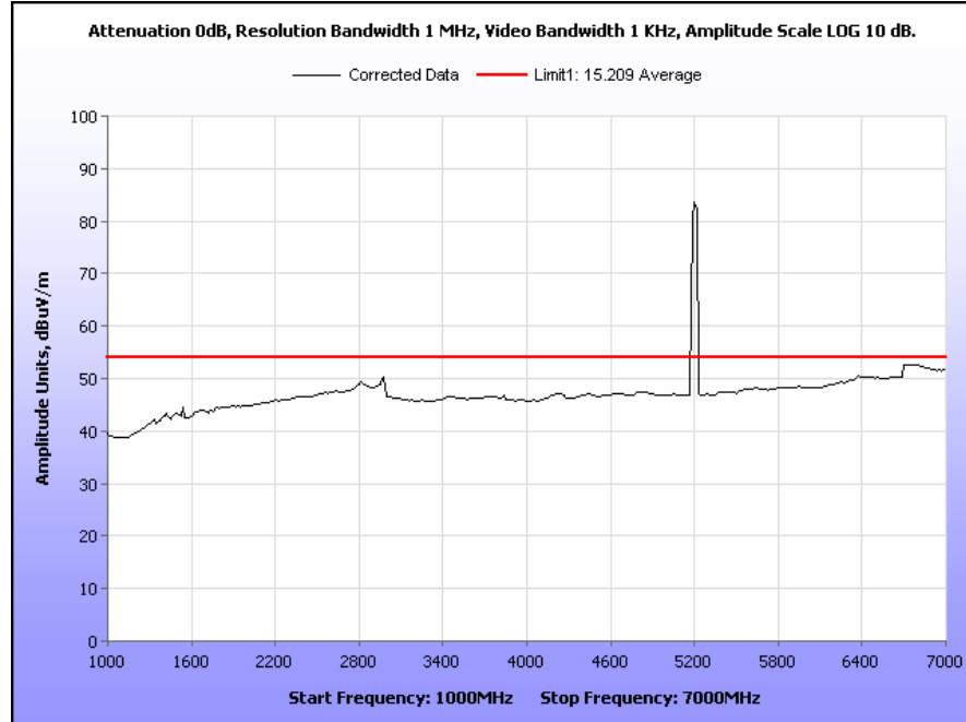
Plot 31. Radiated Spurious Emissions, 5200 MHz, 20 MHz Channel, 1 GHz – 7 GHz, Average
