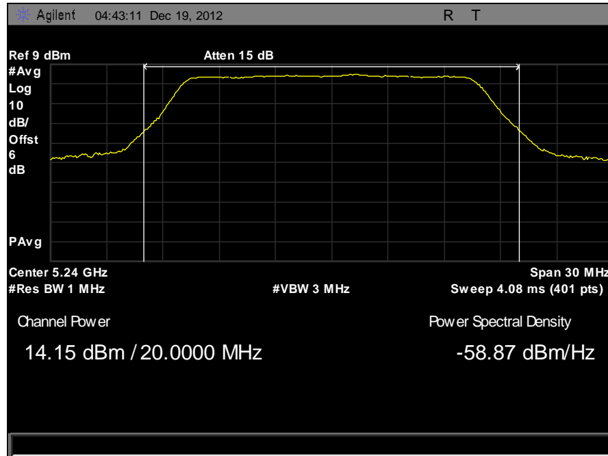
Plot 16. Peak Output Power, 5240 MHz 20 MHz
