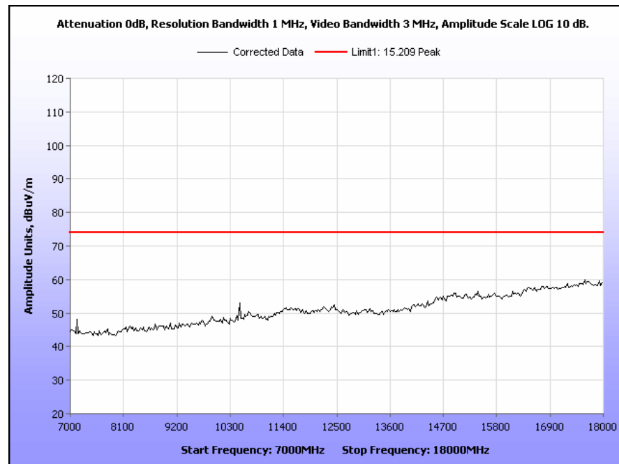
Plot 39. Radiated Spurious Emissions, 5240 MHz, 20 MHz Channel, 7 GHz – 18 GHz, Peak
