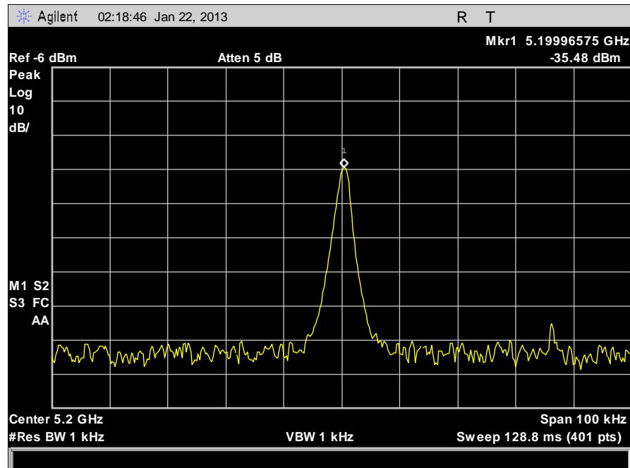
Plot 55. Frequency Stability, 5200 MHz, 20°C, 108V
