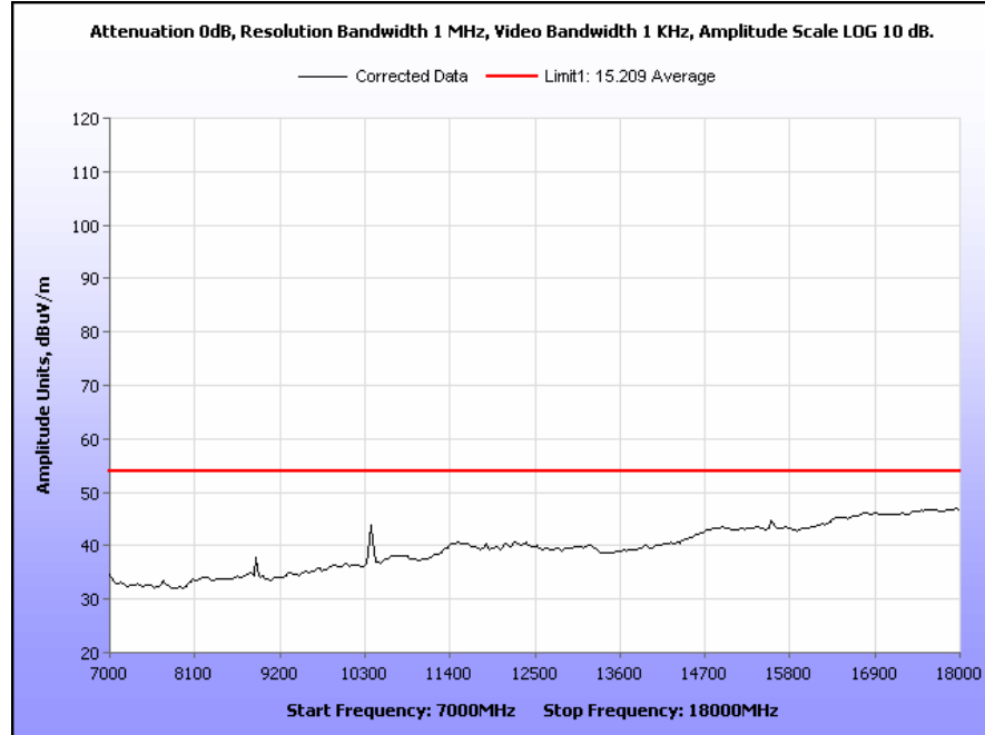
Plot 43. Radiated Spurious Emissions, 5190 MHz, 40 MHz Channel, 7 GHz – 18 GHz, Average
