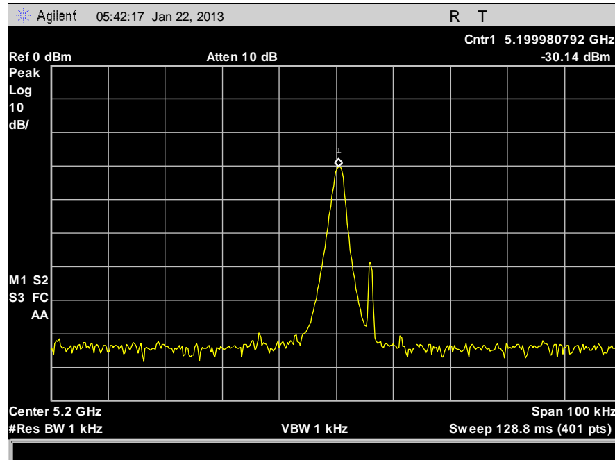
Plot 53. Frequency Stability, 5200 MHz, 0°C, 120 V
