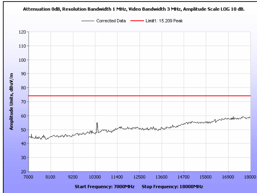
Plot 44. Radiated Spurious Emissions, 5190 MHz, 40 MHz Channel, 7 GHz – 18 GHz, Peak
