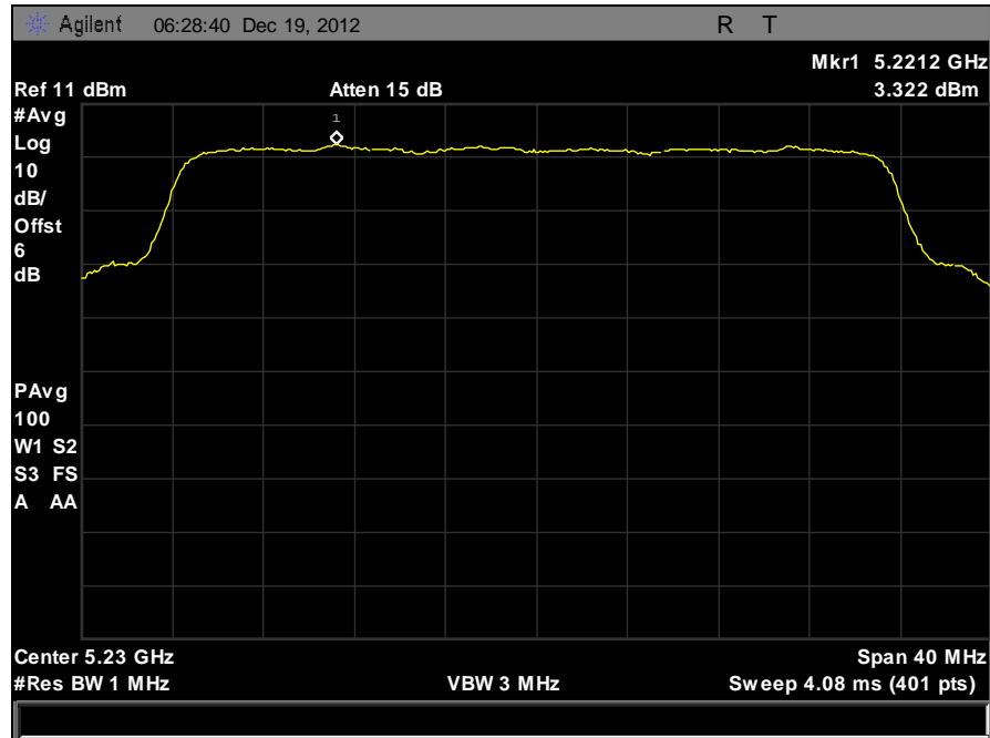
Plot 23. Peak Power Spectral Density, 5230 MHz 40 MHz
