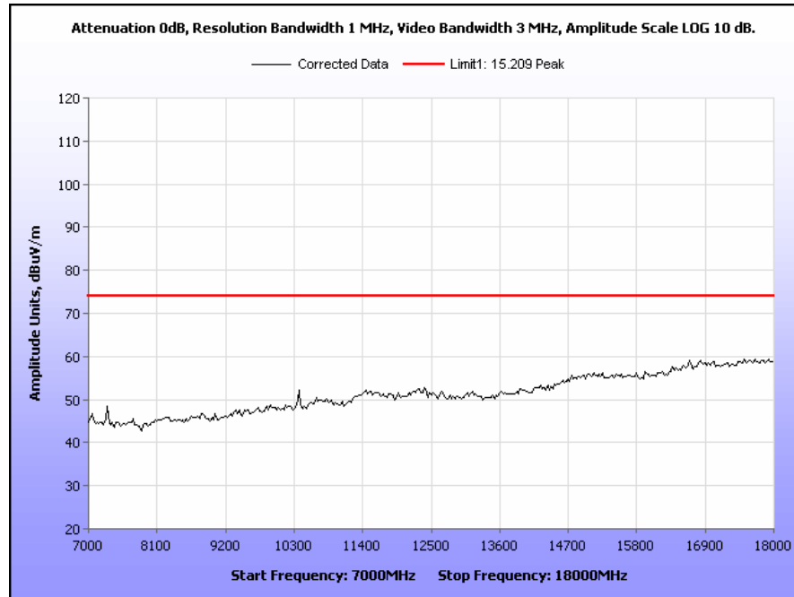
Plot 30. Radiated Spurious Emissions, 5180 MHz, 20 MHz Channel, 7 GHz – 18 GHz, Peak
