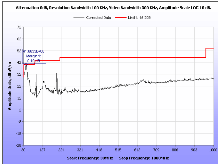
Plot 40. Radiated Spurious Emissions, 5190 MHz, 40 MHz Channel, Tx Power 14.5, 30 MHz – 1 GHz
