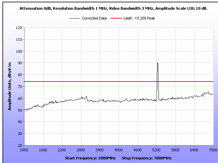
Plot 47. Radiated Spurious Emissions, 5230 MHz, 40 MHz Channel, 1 GHz – 7 GHz, Peak
