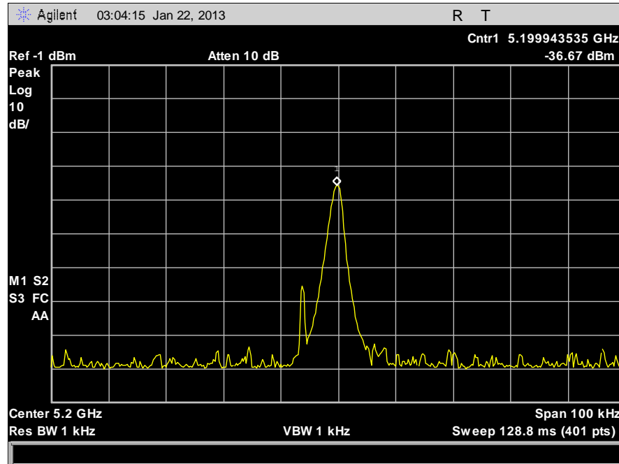
Plot 58. Frequency Stability, 5200 MHz, 30°C, 120 V
