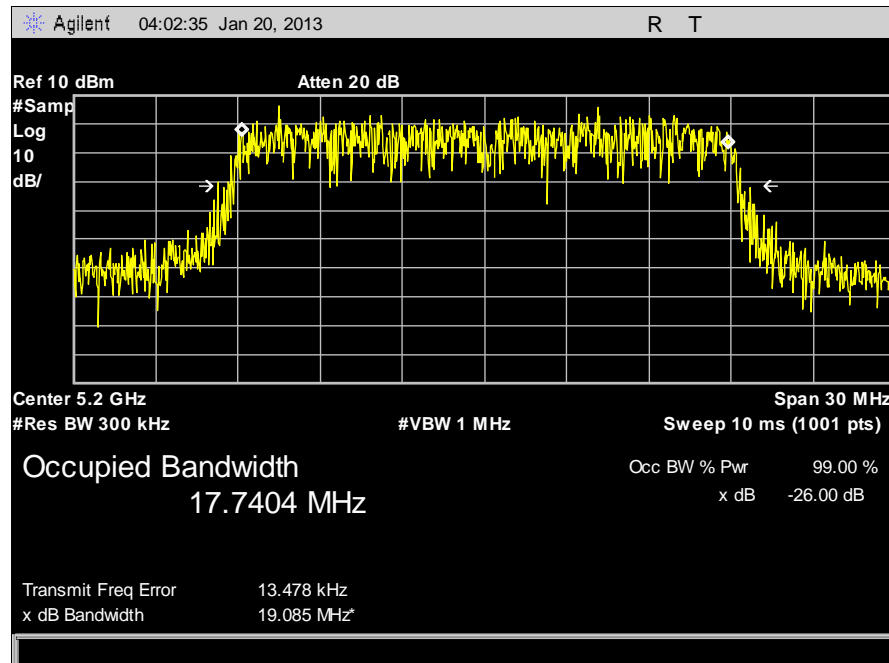
Plot 11. Occupied Bandwidth, 5200 MHz, 99%
