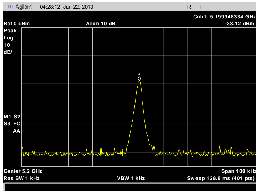
Plot 61. Frequency Stability, 5200 MHz, 55°C, 120 V
