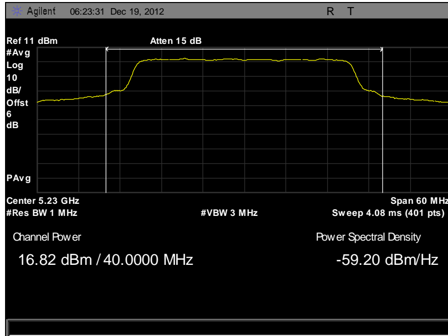
Plot 18. Peak Output Power, 5230 MHz 40 MHz
