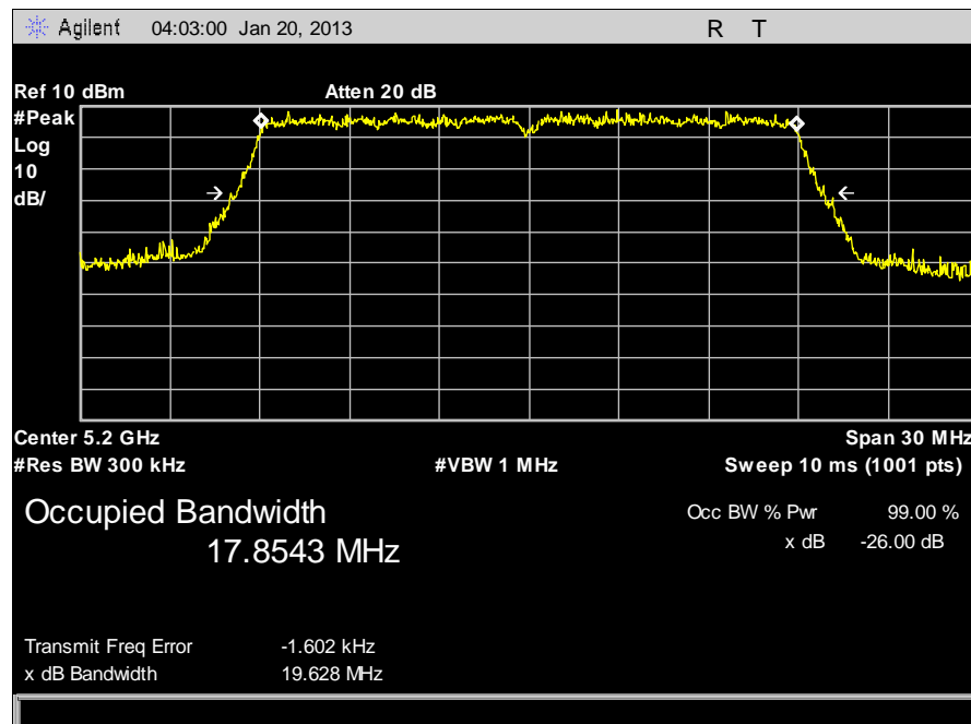
Plot 7. Occupied Bandwidth, 5200 MHz, 26 dB
