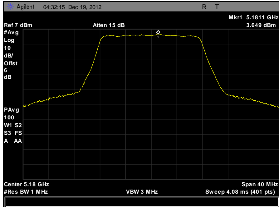
Plot 19. Peak Power Spectral Density, 5180 MHz 20 MHz
