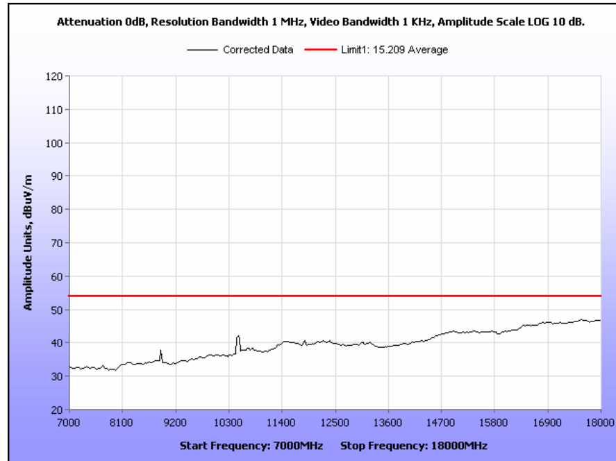
Plot 38. Radiated Spurious Emissions, 5240 MHz, 20 MHz Channel, 7 GHz – 18 GHz, Average
