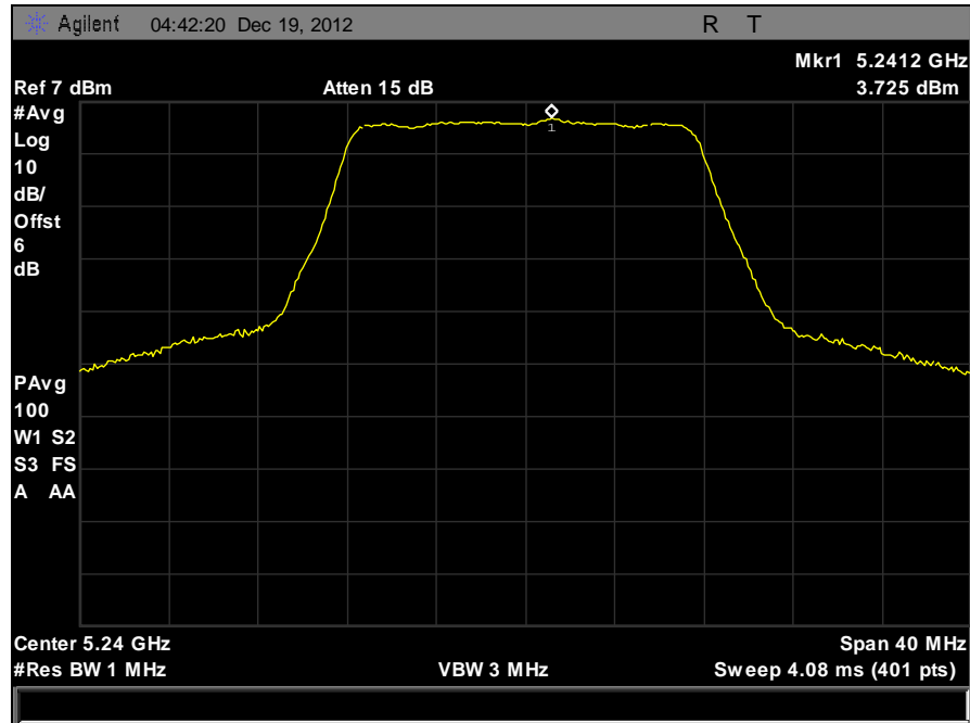
Plot 21. Peak Power Spectral Density, 5240 MHz 20 MHz
