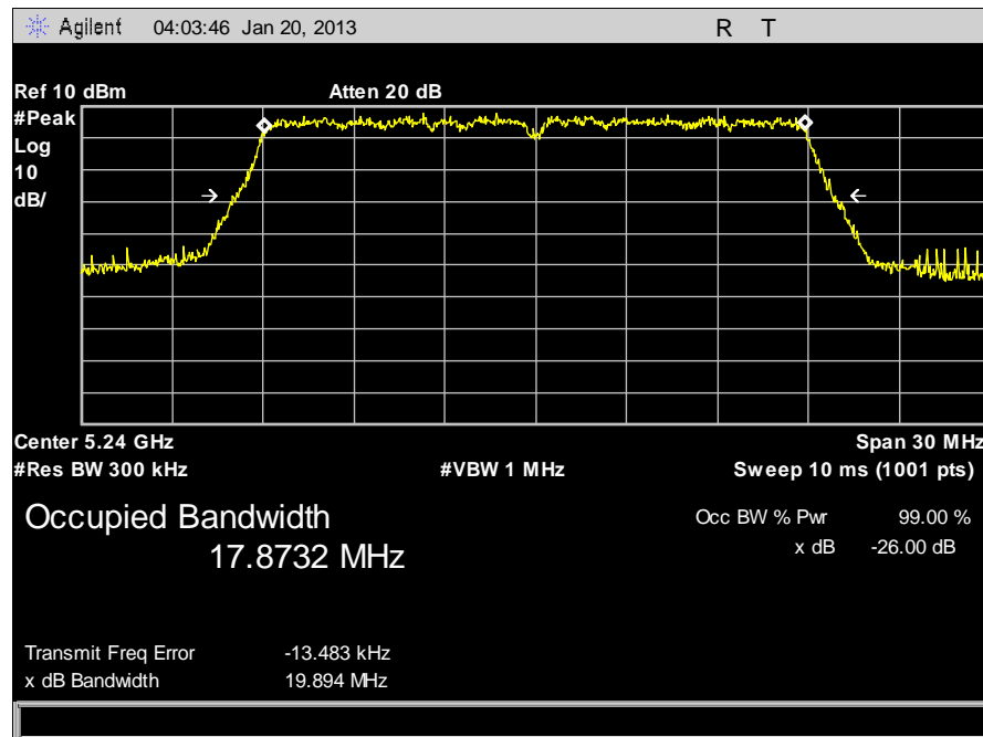
Plot 8. Occupied Bandwidth, 5240 MHz, 26 dB
