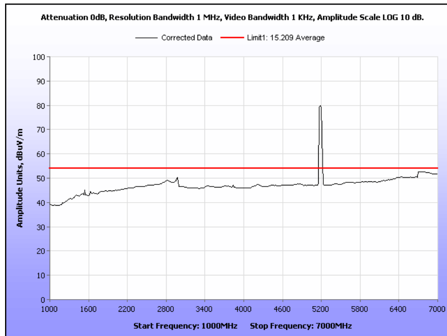
Plot 41. Radiated Spurious Emissions, 5190 MHz, 40 MHz Channel, 1 GHz – 7 GHz, Average
