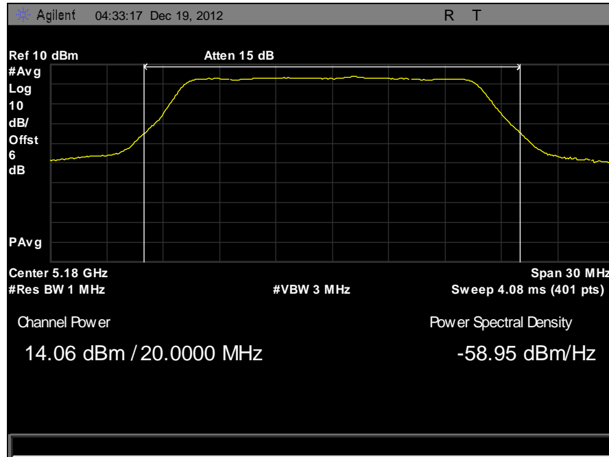
Plot 14. Peak Output Power, 5180 MHz 20 MHz
