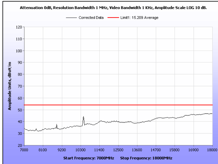
Plot 48. Radiated Spurious Emissions, 5230 MHz, 40 MHz Channel, 7 GHz – 18 GHz, Average
