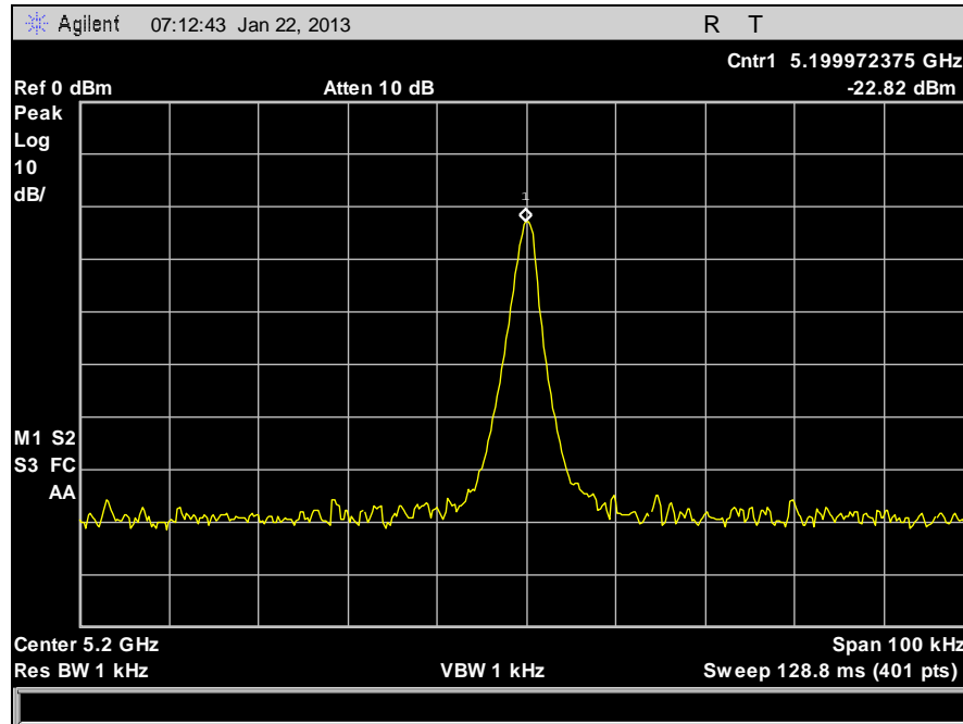
Plot 50. Frequency Stability, 5200 MHz, -30°C, 120 V
