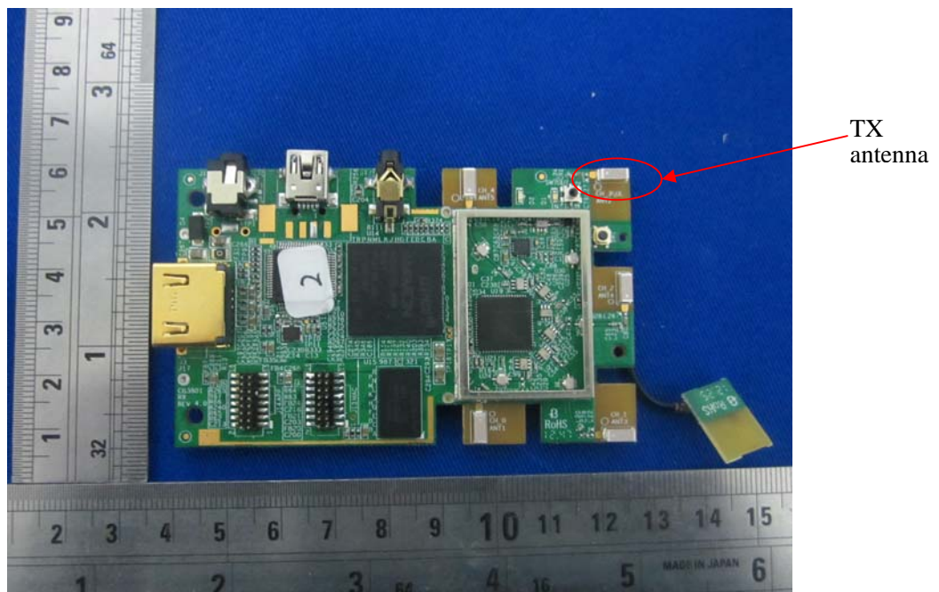
EUT – Bottom Cover Off View
