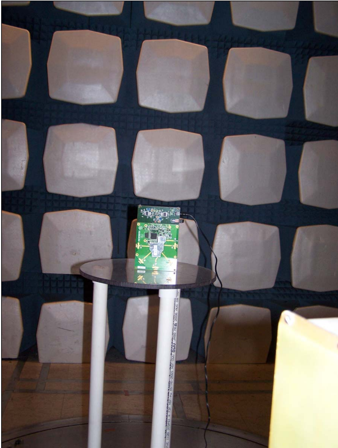
Radiated Spurious Emissions Setup
