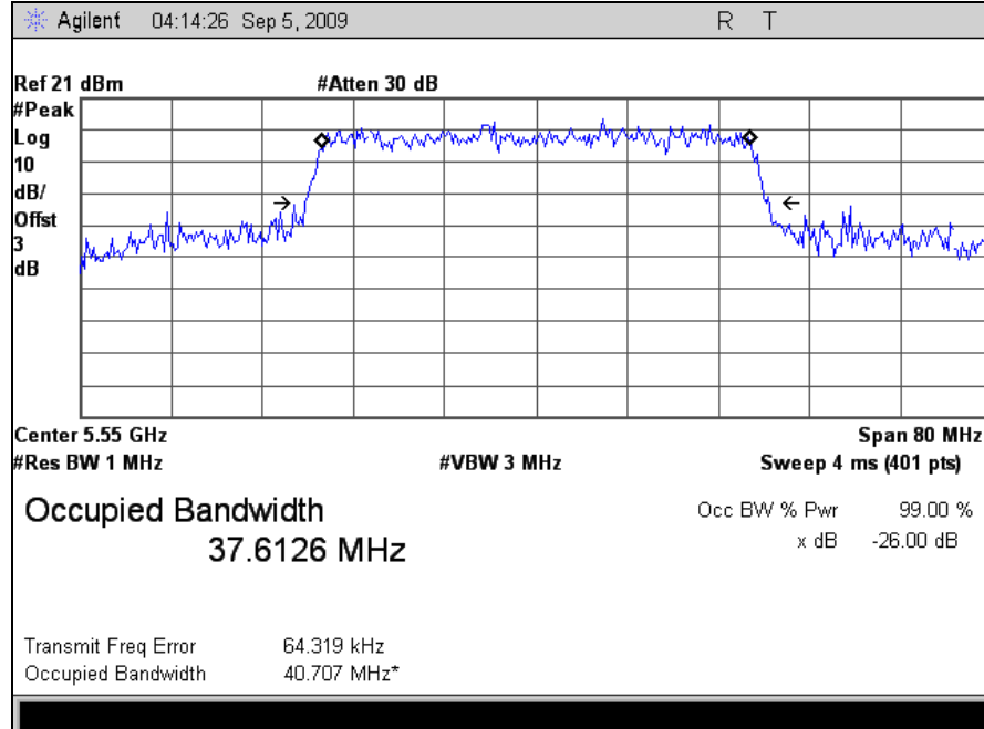
Plot 13. Occupied Bandwidth, Antenna Port 0, 5550 MHz
