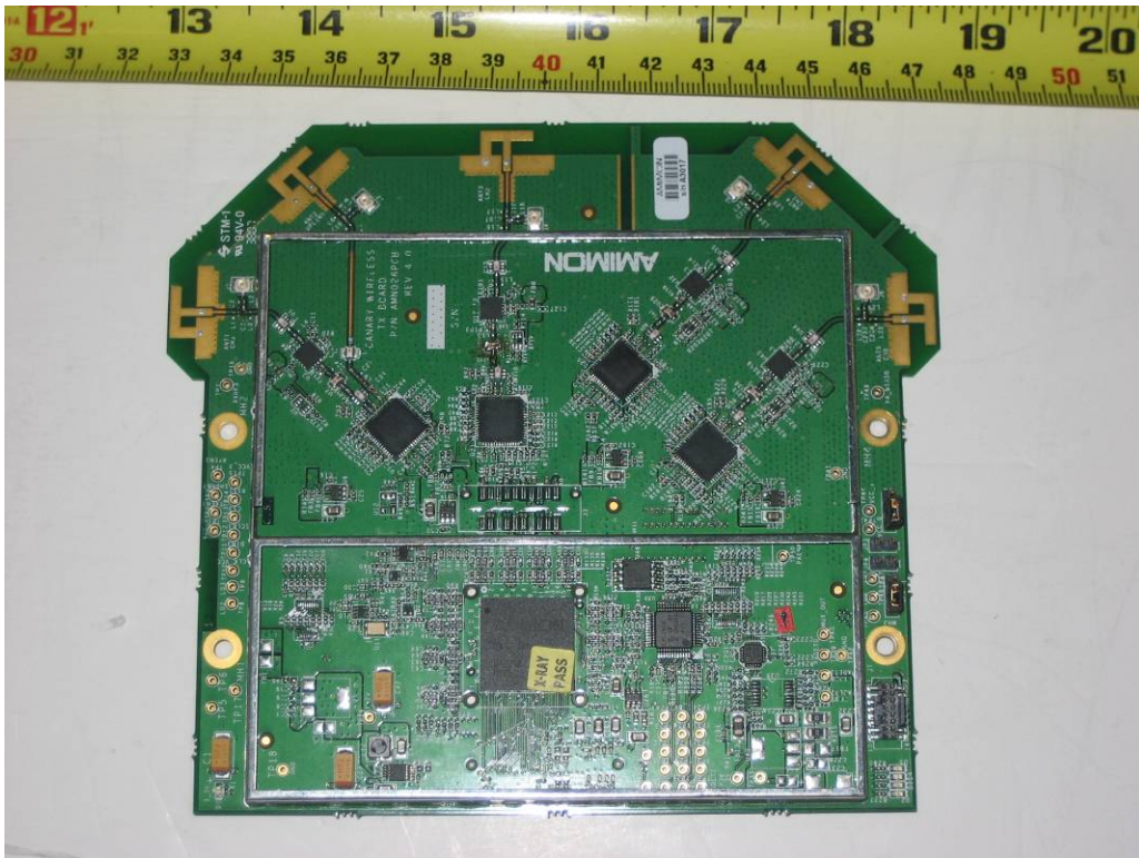
Module Top View
