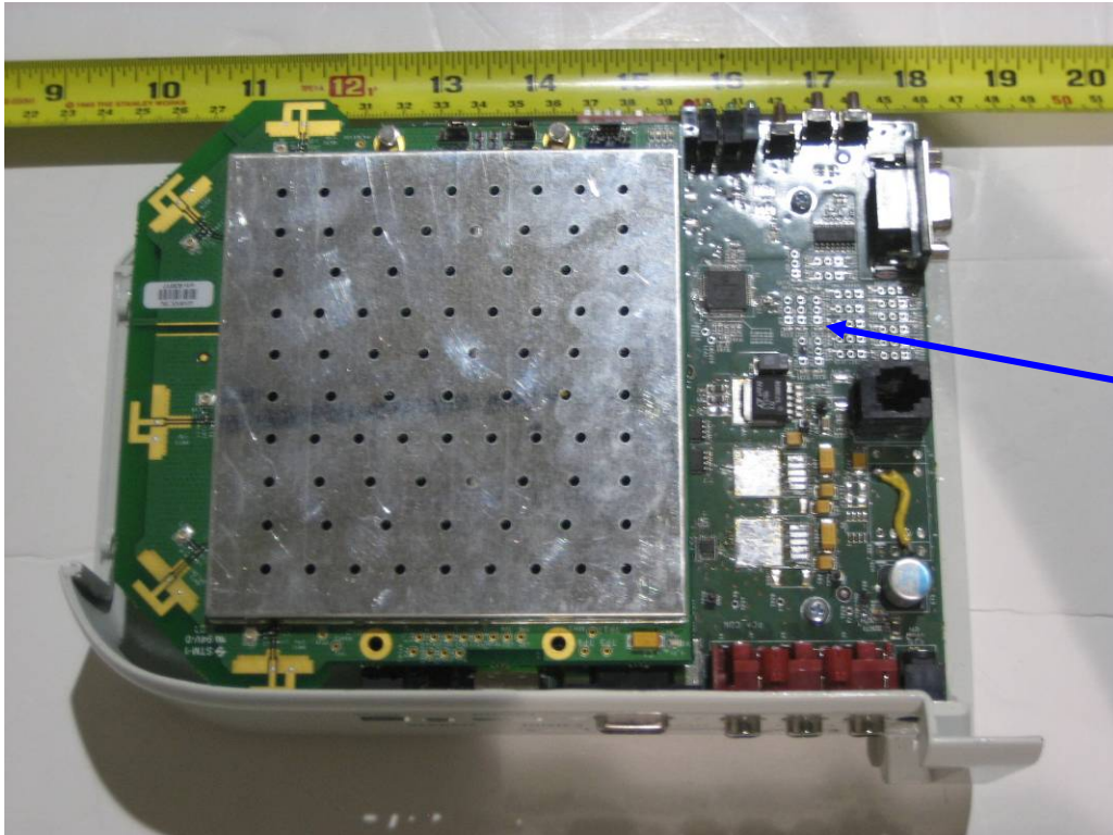
Module in supporting board
