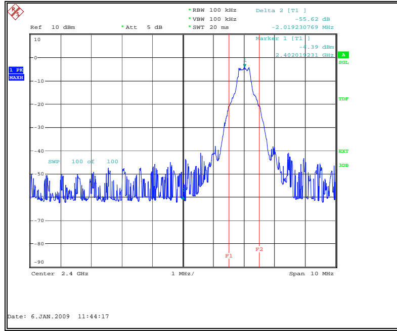
Fig. 1 Frequency Band Edges: Channel 0, Hopping Off
