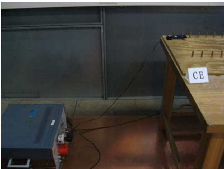
Photo of AC Powerline Conducted Emission Test
