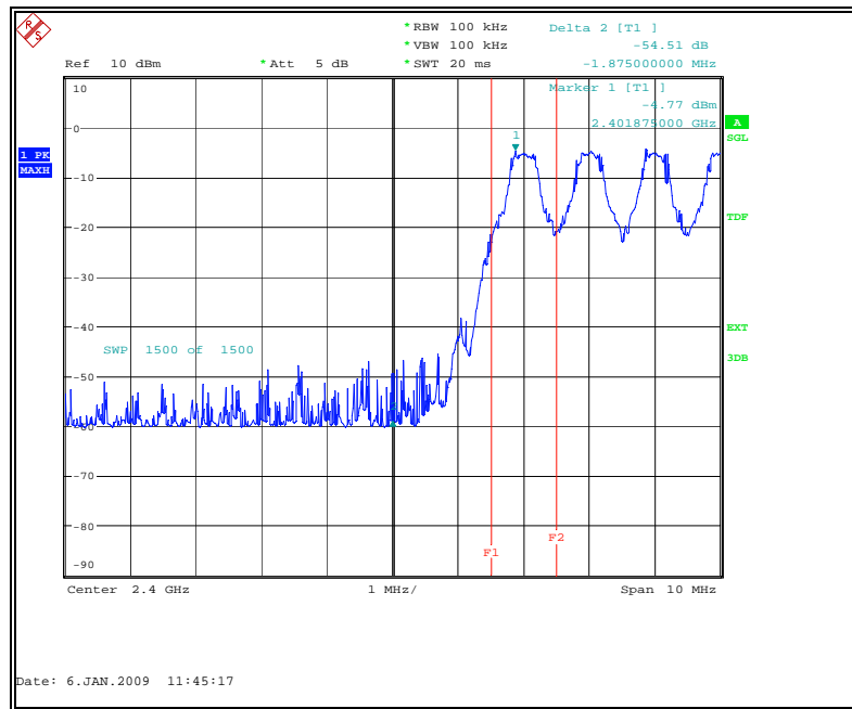
Fig. 2 Frequency Band Edges: Channel 0, Hopping On
