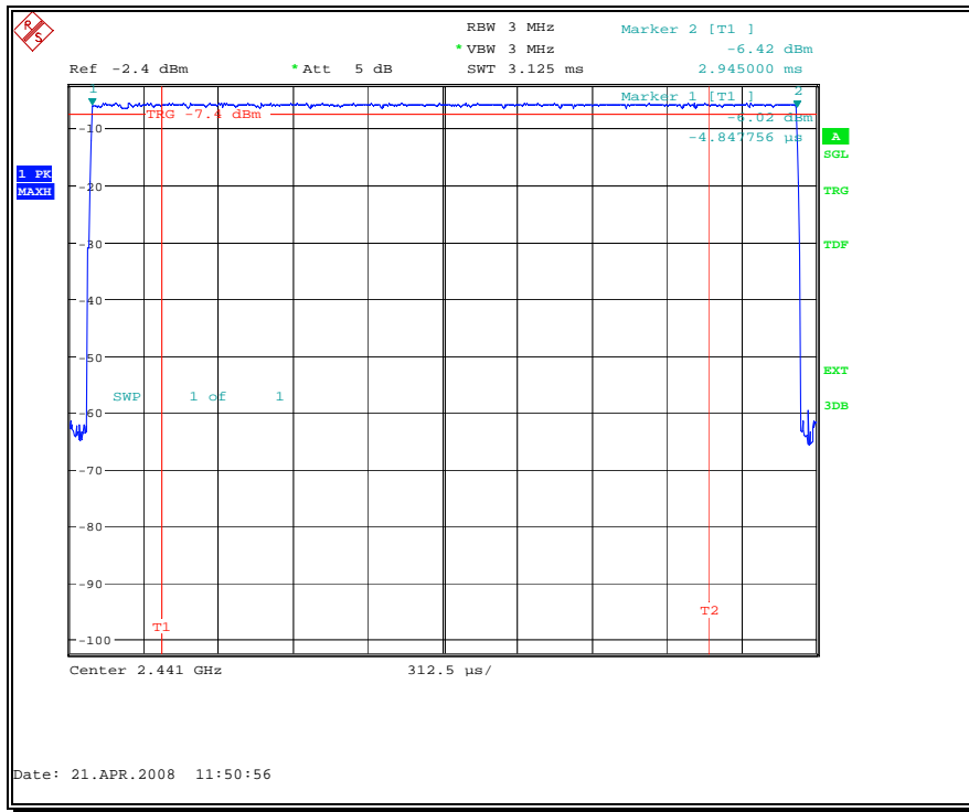
Fig. 25 Time of occupancy (Dwell Time): Channel 39
