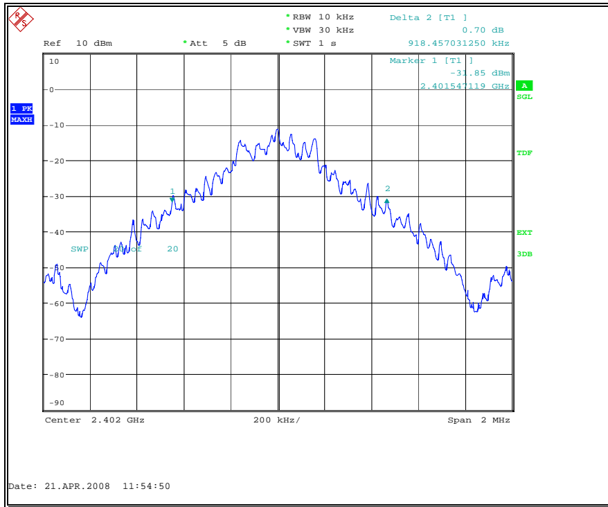
Fig. 26 20dB Bandwidth: Channel 0
