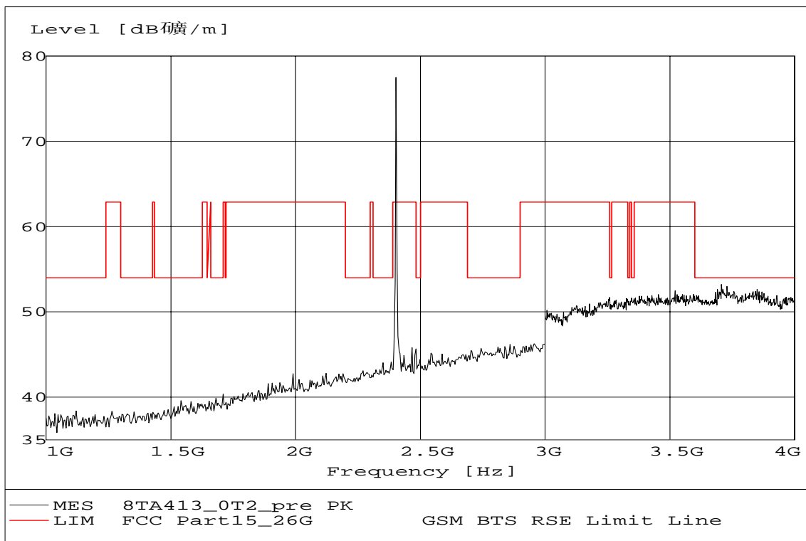
Fig. 16 Radiated emission: Channel 0, 1 GHz ~ 4 GHz
