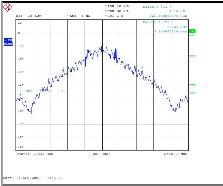
Fig. 27 20dB Bandwidth: Channel 39
