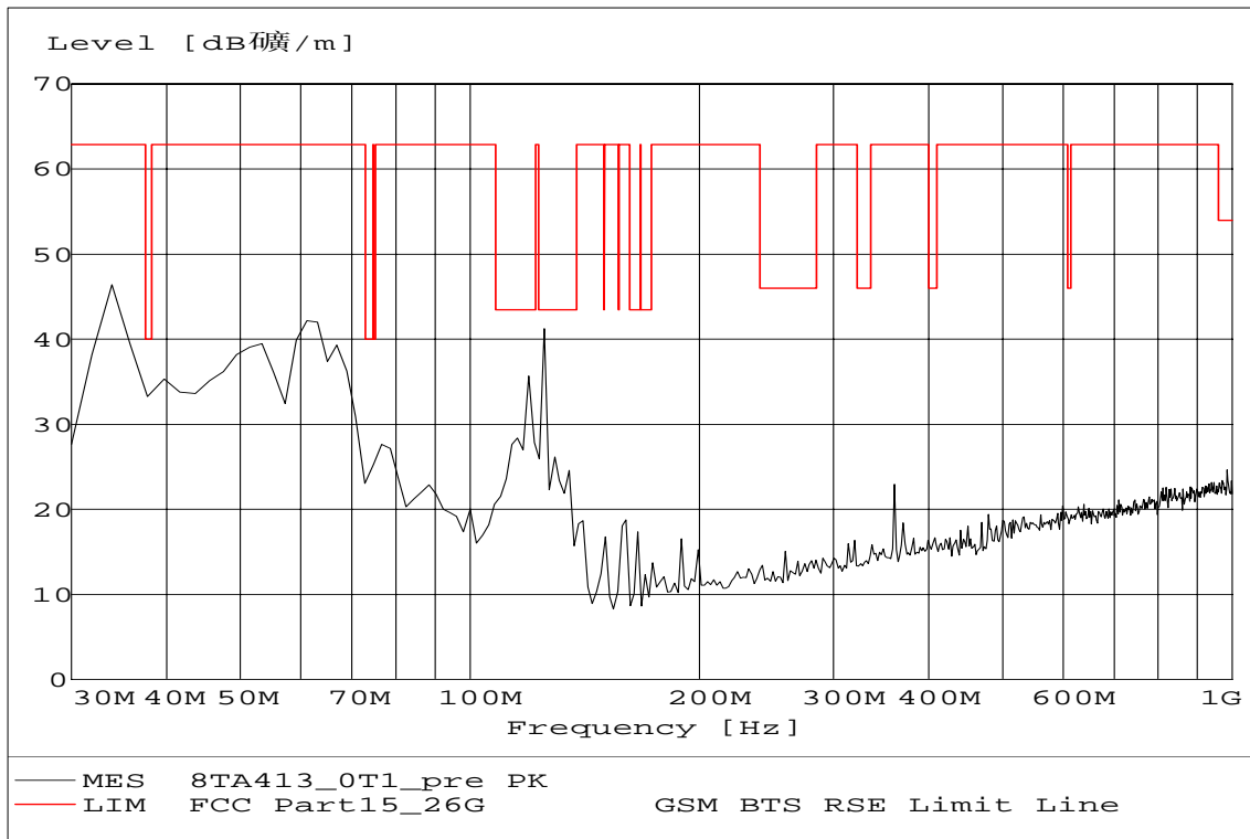
Fig. 15 Radiated emission: Channel 0, 30 MHz ~ 1 GHz
