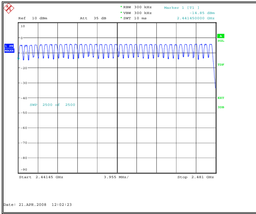
Fig. 31 Number of hopping frequencies: Channel 40 - 78
