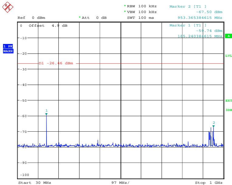
Fig. 11 Conducted spurious emission: Channel 78, 2480MHz
