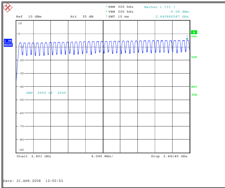
Fig. 30 Number of hopping frequencies: Channel 0 – 39
