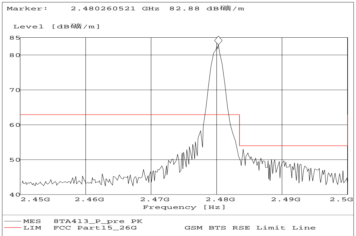
Fig. 14 Radiated emission: 2.45GHz ~ 2.5GHz
