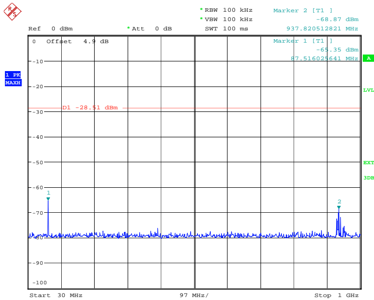
Fig. 5 Conducted spurious emission: Channel 0,2402MHz
