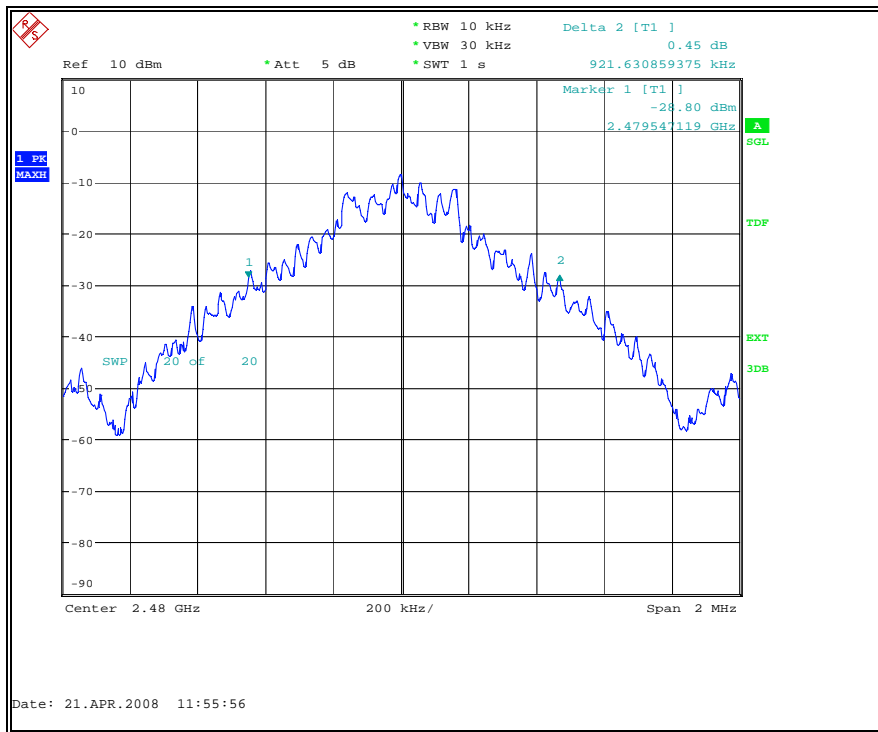
Fig. 28 20dB Bandwidth: Channel 78
