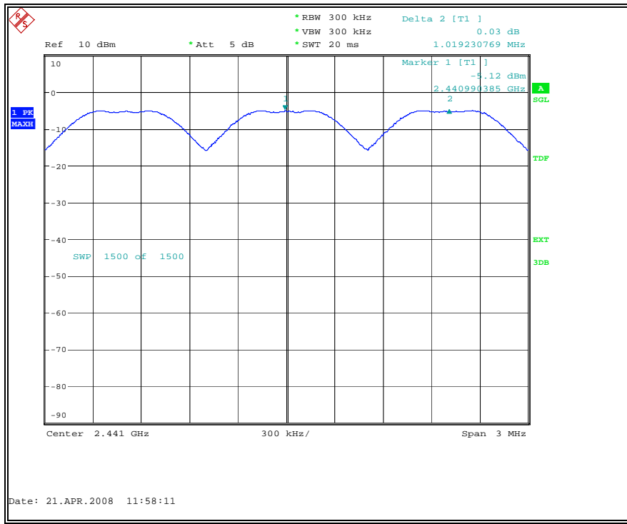
Fig. 29 Carrier frequency separation measurement: Channel 39
