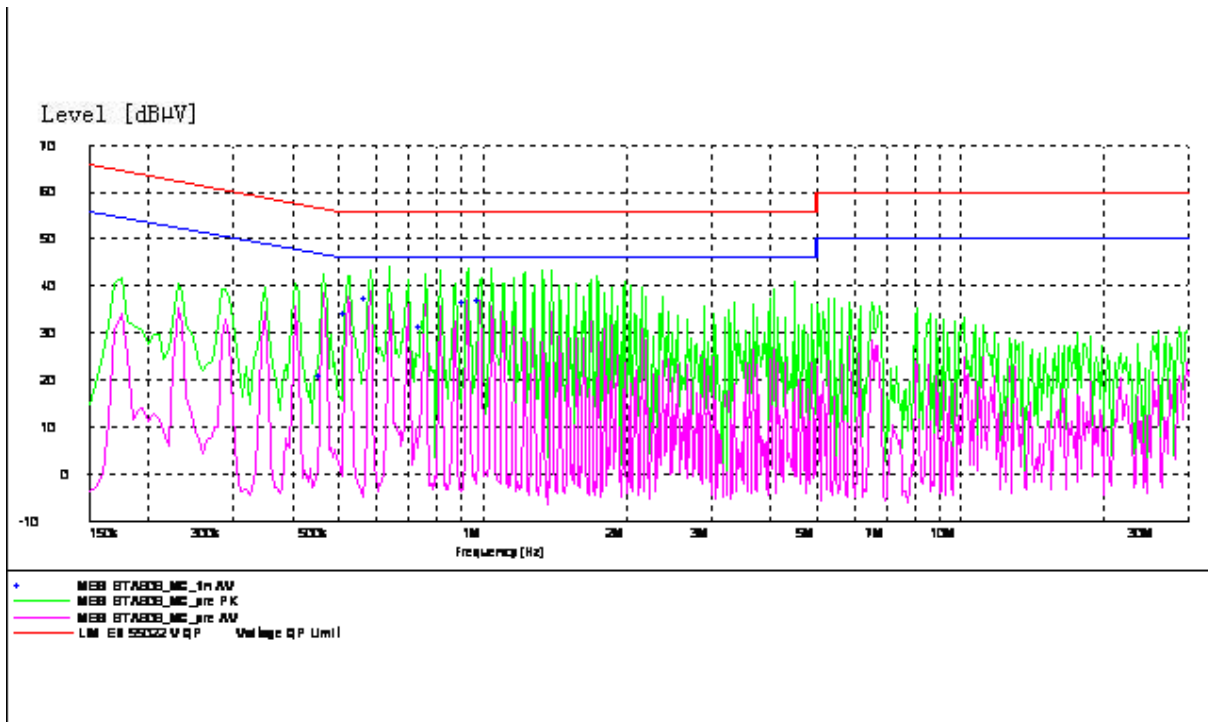
Figure B.5 Conducted Emission
