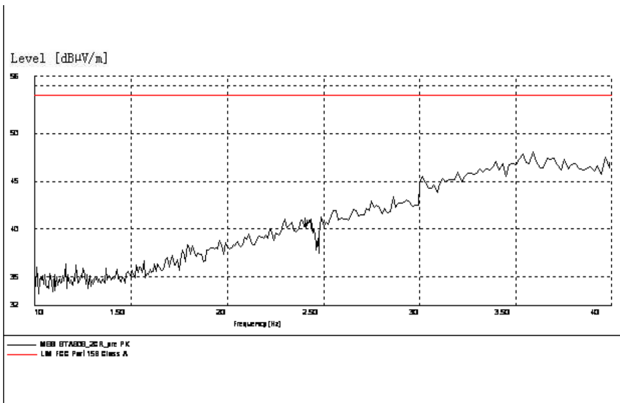
Figure B.2 Radiated Emission from 1GHz to 4GHz
