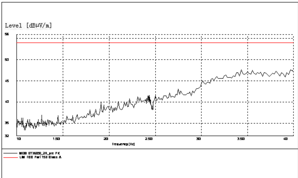
Figure B.4 Radiated Emission from 1GHz to 4GHz
