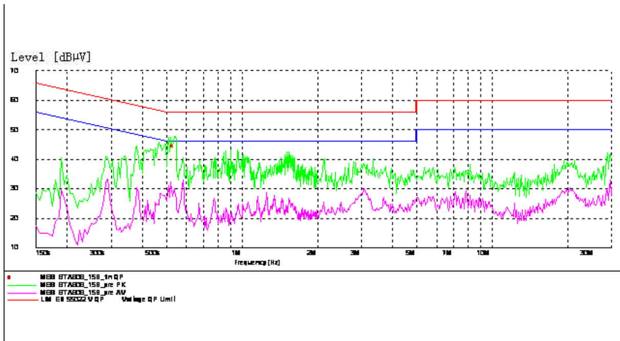
Figure B.6 Conducted Emission
