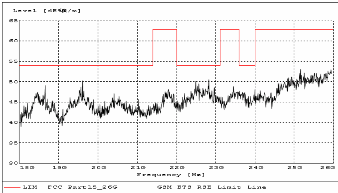
Fig. 24 Radiated emission: 18 GHz ~ 26 GHz
