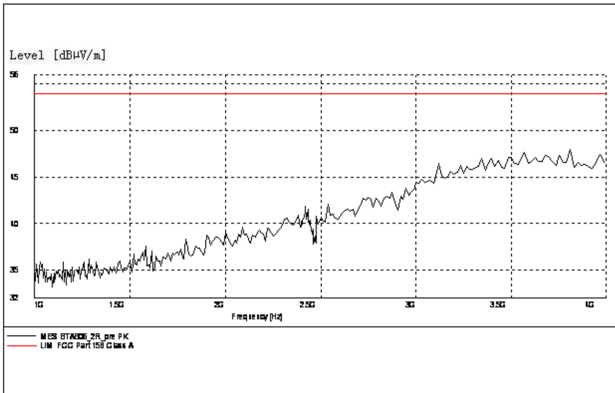
Figure B.4 Radiated Emission from 1GHz to 4GHz
