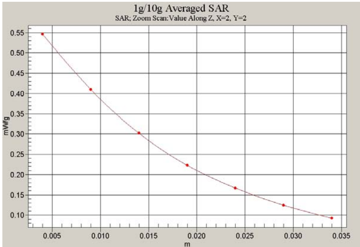
Fig. 40 Z-Scan at power reference point (850 MHz CH251)
