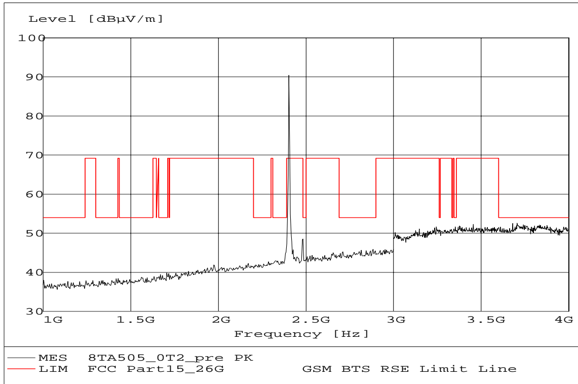
Fig. 15 Radiated emission: Channel 0, 1 GHz ~ 4 GHz
