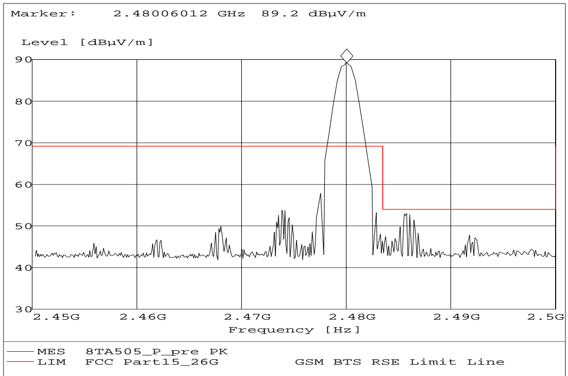
Fig. 23 Radiated emission (Power): 2.45GHz ~ 2.5GHz
