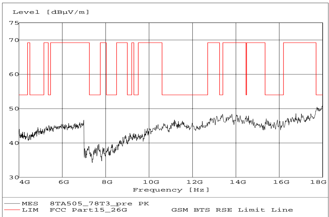
Fig. 16 Radiated emission: Channel 0, 4 GHz ~ 18 GHz
