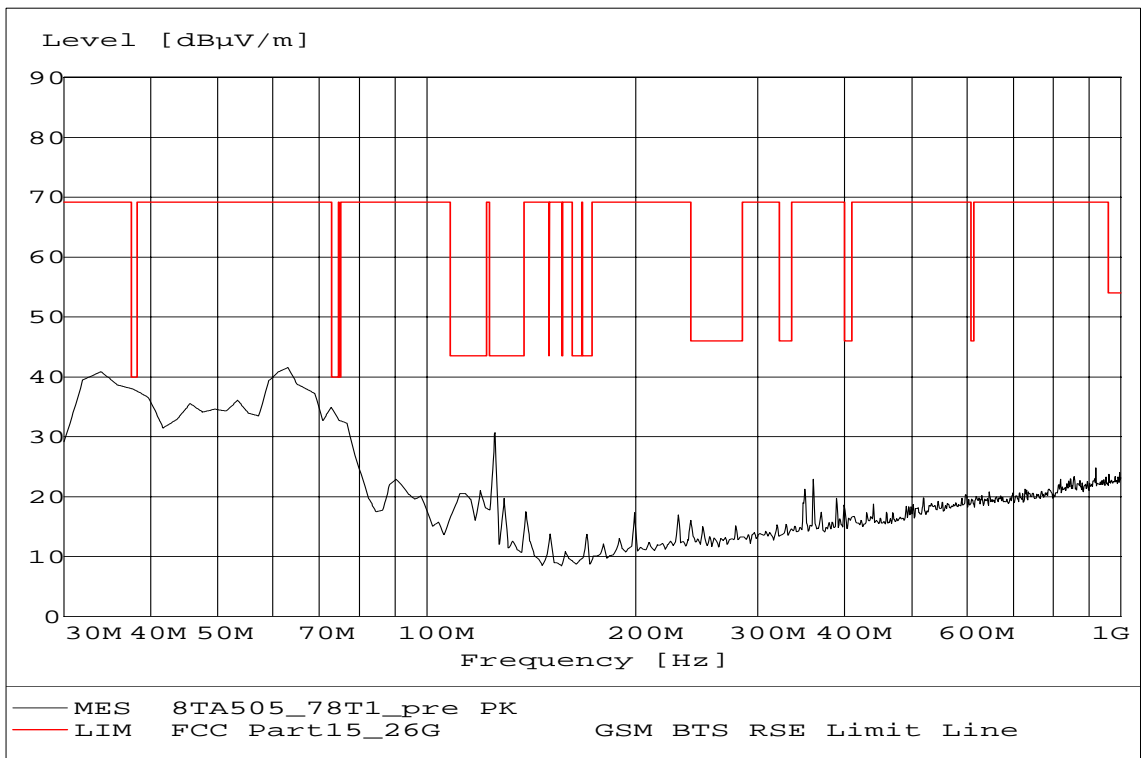
Fig. 20 Radiated emission: Channel 78, 30 MHz ~ 1 GHz
