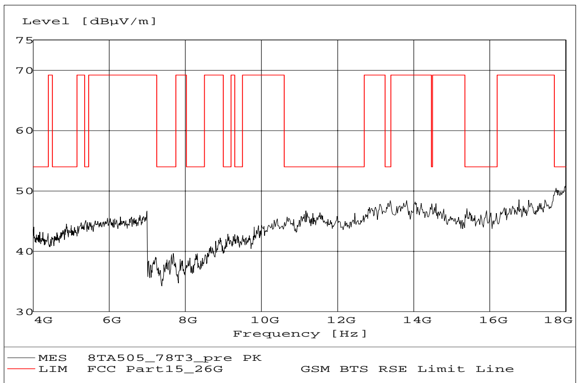
Fig. 22 Radiated emission: Channel 78, 4 GHz ~ 18 GHz
