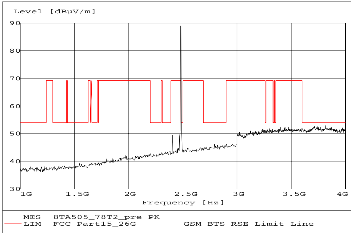
Fig. 21 Radiated emission: Channel 78, 1 GHz ~ 4 GHz
