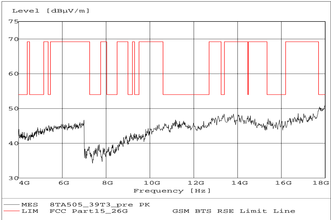
Fig. 19 Radiated emission: Channel 39, 4 GHz ~ 18 GHz
