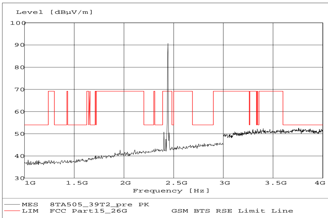
Fig. 18 Radiated emission: Channel 39, 1 GHz ~ 4 GHz
