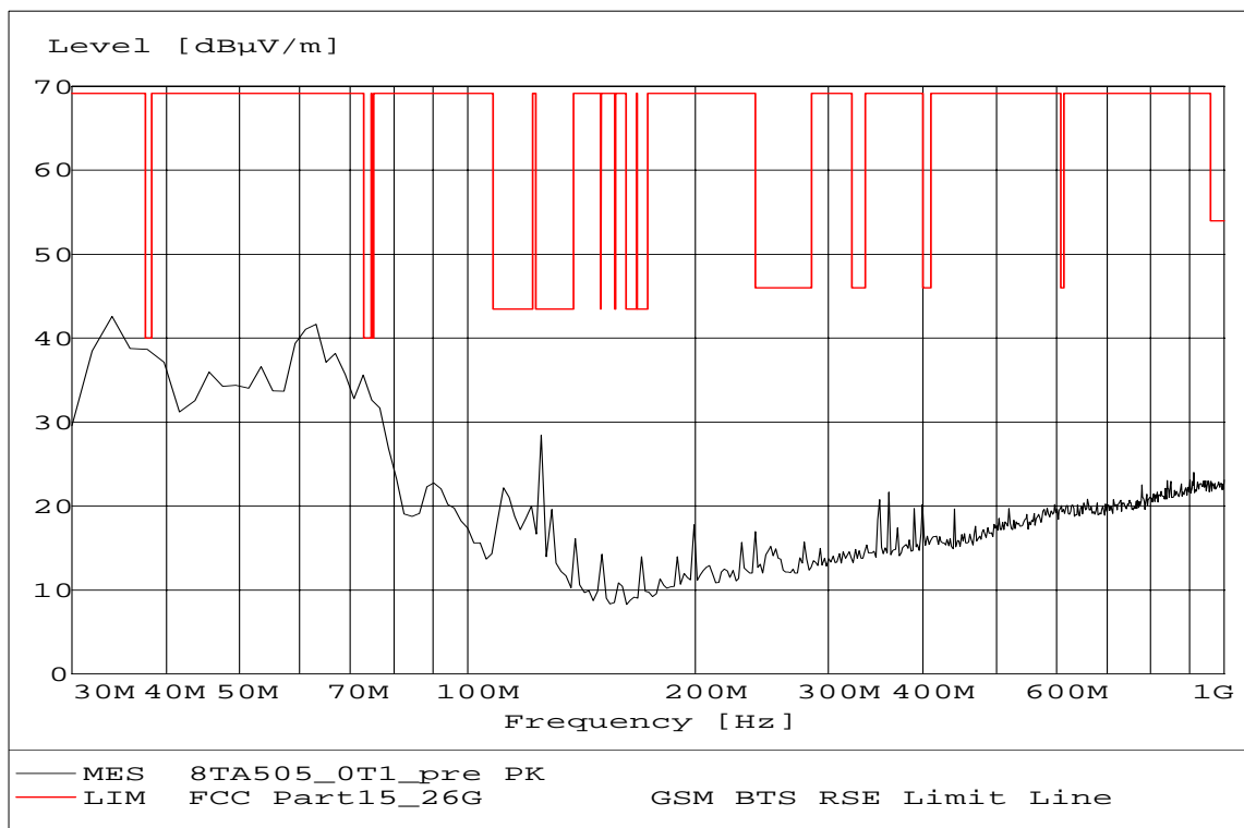
Fig. 14 Radiated emission: Channel 0, 30 MHz ~ 1 GHz
