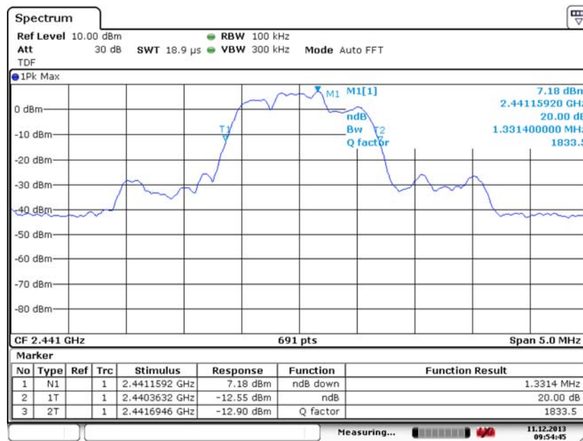
Fig. 76 Occupied 20dB Bandwidth (8DPSK, Ch 39)
