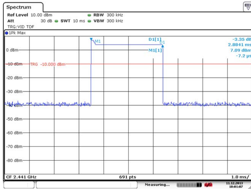
Fig. 80 Time of Occupancy(Dwell Time) ( \pi/4 DQPSK, Ch39)
