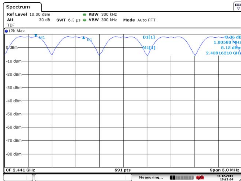
Fig. 90 Carrier Frequency Separation (GFSK, Ch39)
