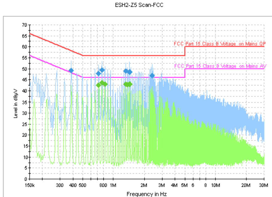
Fig. 93 AC Power line Conducted Emission (Traffic, AE2)
