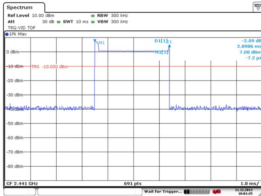
Fig. 82 Time of Occupancy(Dwell Time) (8DPSK, Ch39)
