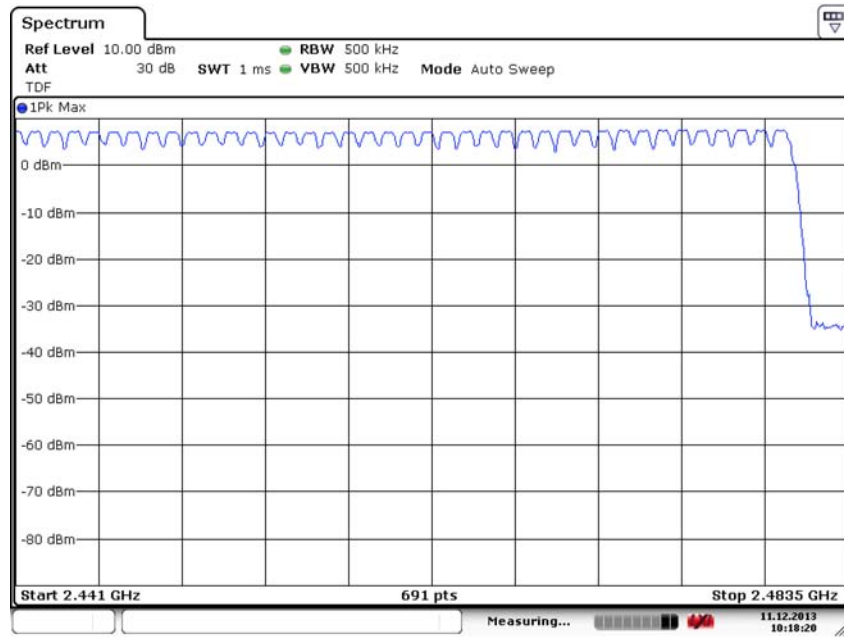
Fig. 87 Hopping channel ch39~78 ( \pi/4 DQPSK, Ch39)
