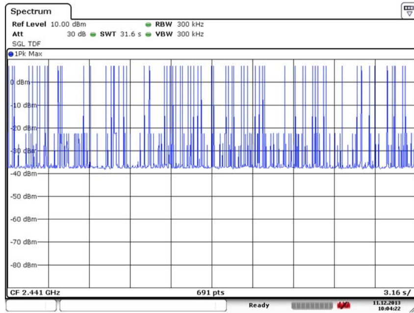
Fig. 83 Number of Transmissions (8DPSK, Ch39)
