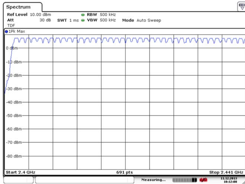
Fig. 88 Hopping channel ch0~39 (8DPSK, Ch39)
