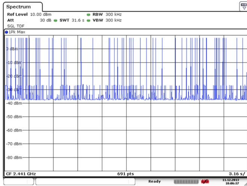
Fig. 79 Number of Transmissions (GFSK, Ch39)
