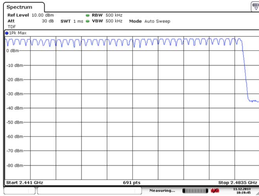
Fig. 85 Hopping channel ch39~78 (GFSK, Ch39)
