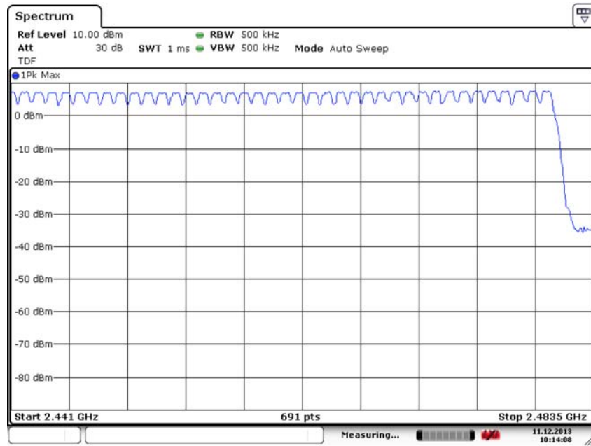
Fig. 89 Hopping channel ch39~78 (8DPSK, Ch39)
