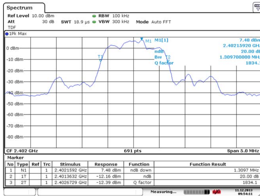
Fig. 75 Occupied 20dB Bandwidth (8DPSK, Ch 0)
