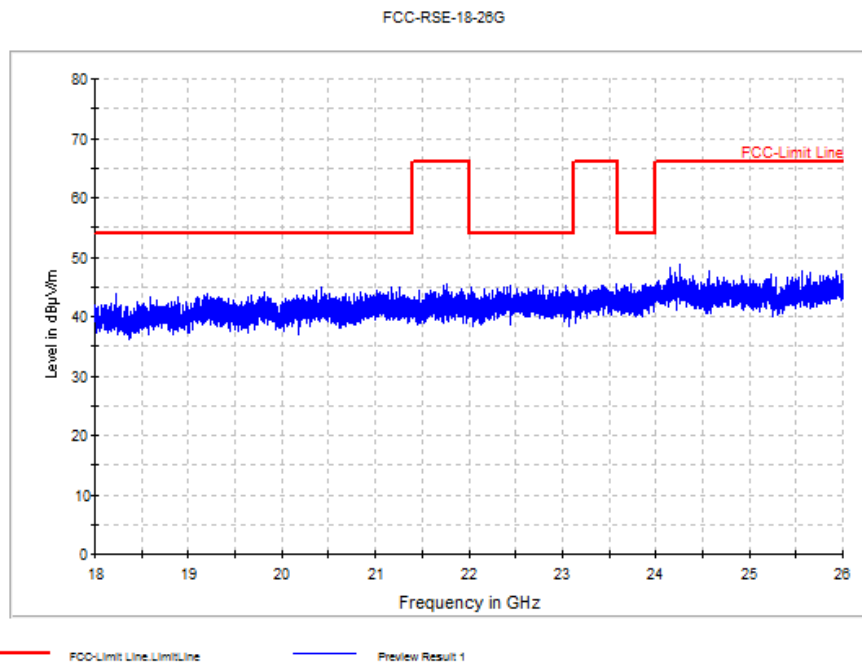
Fig. 68 Radiated Spurious Emission (All channel, 18 GHz ~26 GHz)
