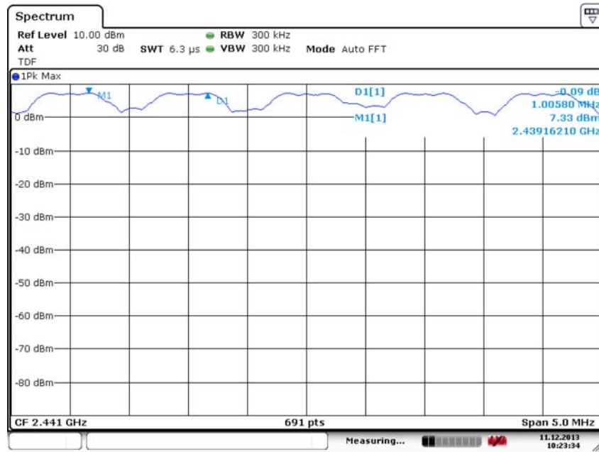
Fig. 91 Carrier Frequency Separation ( \pi/4 DQPSK, Ch39)
