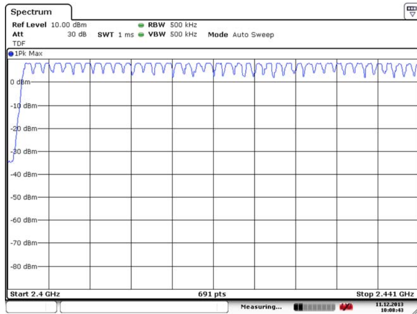
Fig. 84 Hopping channel ch0~39 (GFSK, Ch39)
