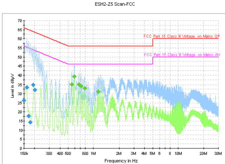
Fig. 95 AC Power line Conducted Emission (Traffic, AE3)
