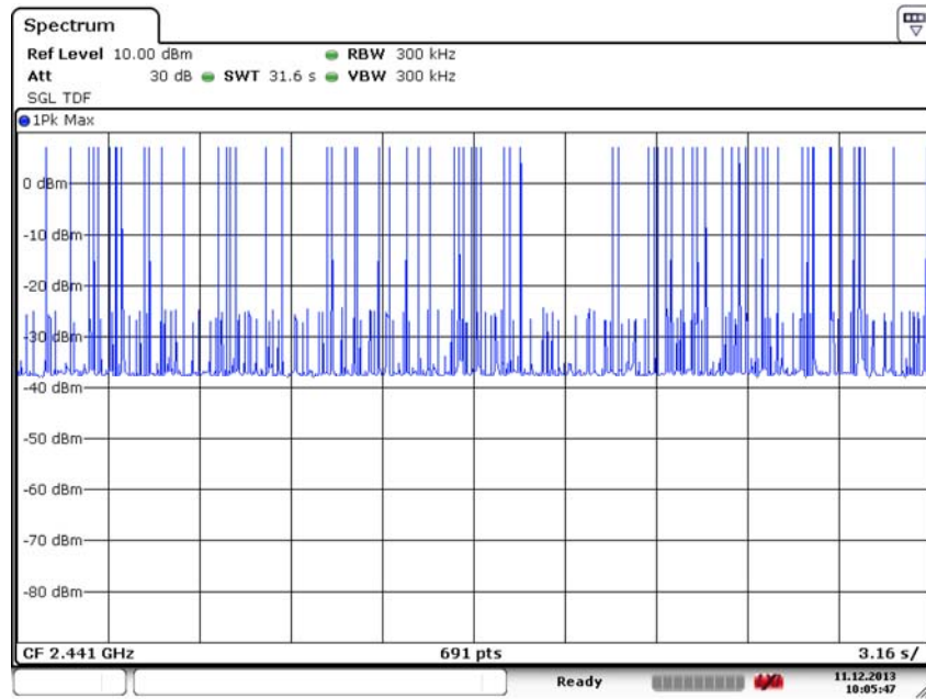
Fig. 81 Number of Transmissions ( \pi/4 DQPSK, Ch39)
