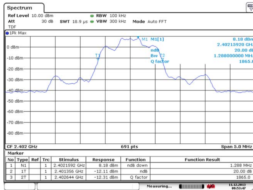
Fig. 72 Occupied 20dB Bandwidth ( \pi/4 DQPSK, Ch 0)
