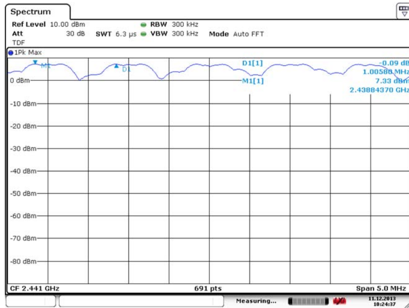
Fig. 92 Carrier Frequency Separation (8DPSK, Ch39)
