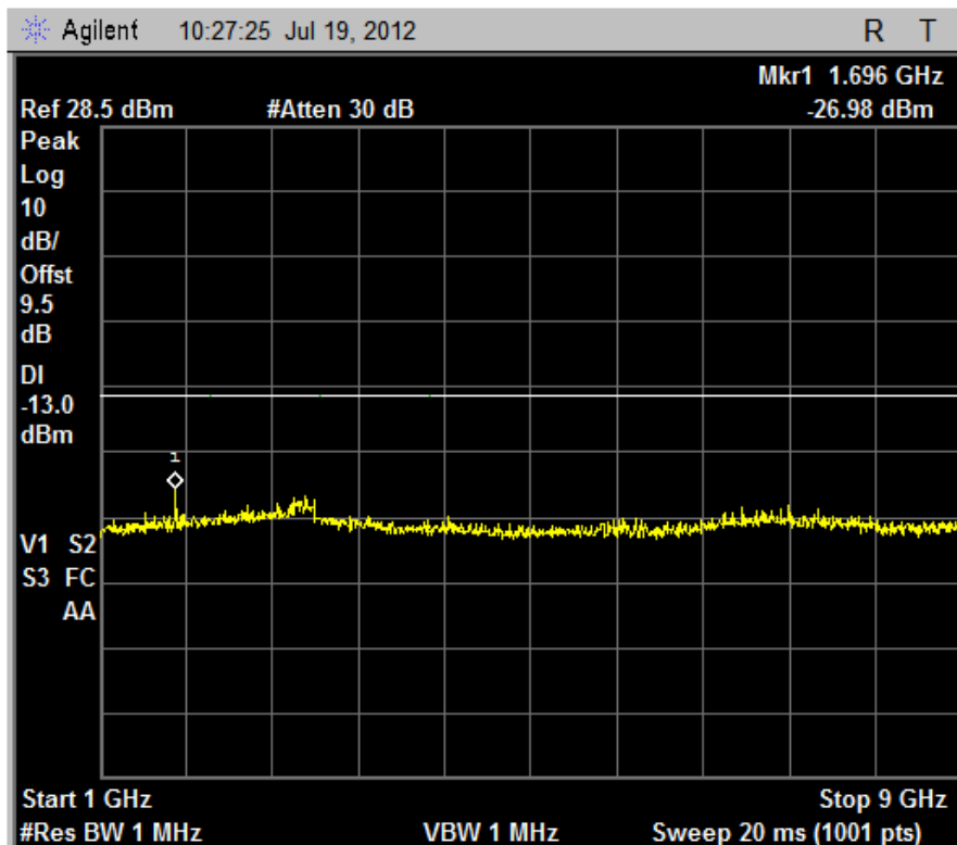
(Plot C3.1: EDGE 850MHz Channel = 251, 1GHz to 9GHz)
