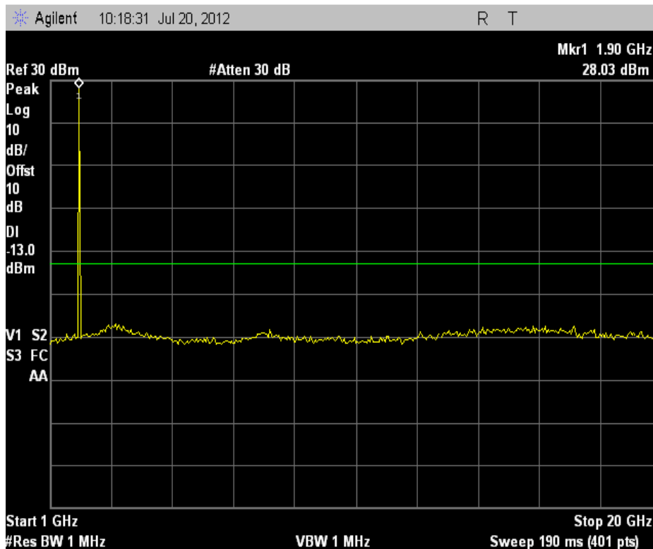
(Plot B2.1: GSM 1900MHz Channel = 661, 1GHz to 20GHz)
