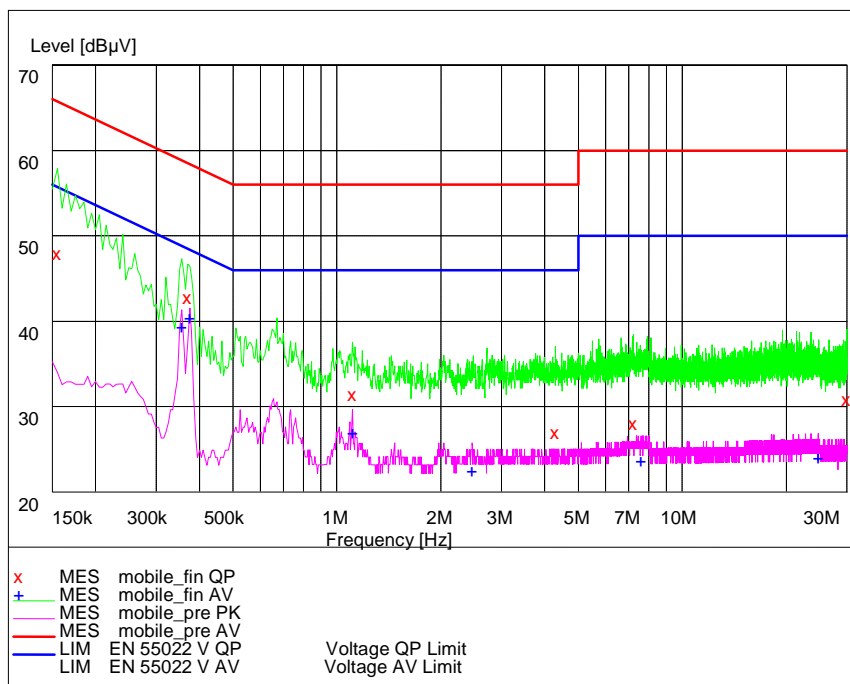
Pic2. Conducted emission L +N Line
