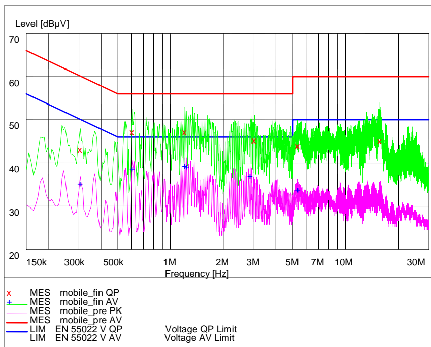
Pic4. Conducted emission L+N Line
