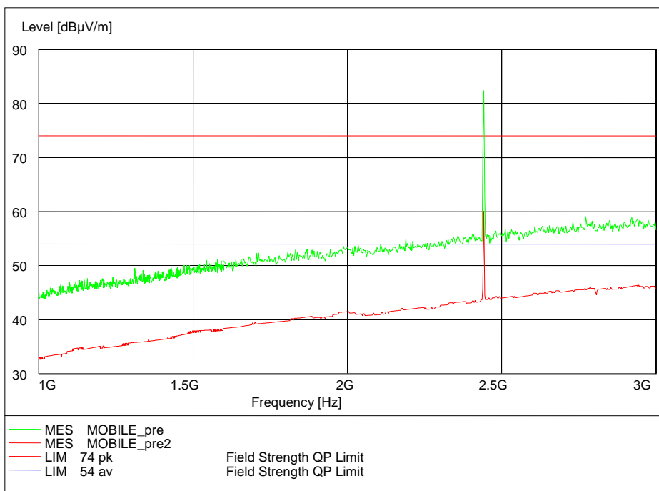
Frequency Range: 1GHz-3GHz Detector: Av mode and PK mode Modulation type: GFSK (LE)
