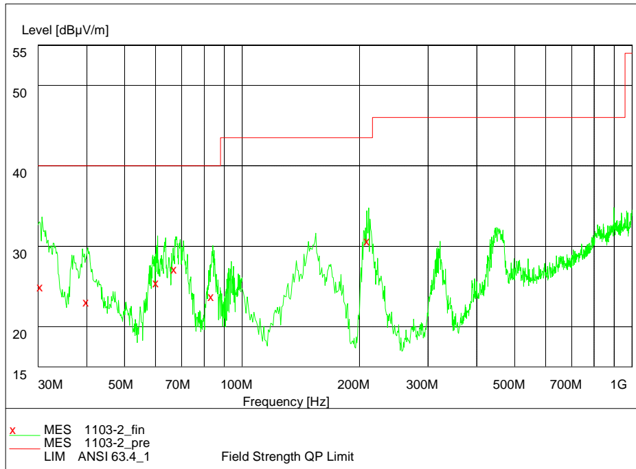
Pic12. Radiated emission (30MHz – 1GHz)
