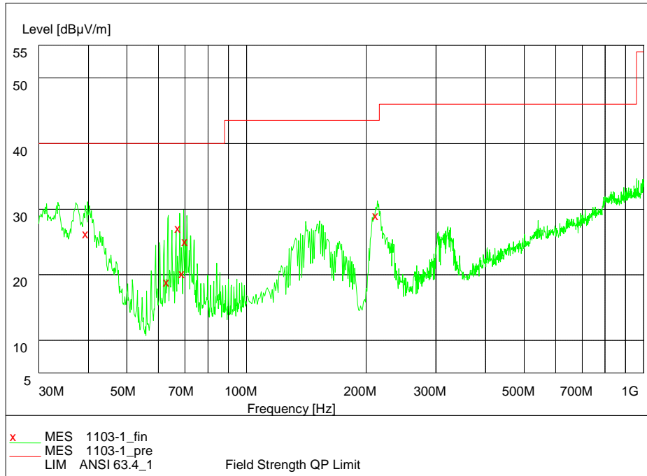
Pic10. Radiated emission (30MHz – 1GHz)
