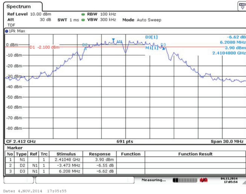
Fig. 97 Occupied 6dB Bandwidth (802.11b, Ch 1)
