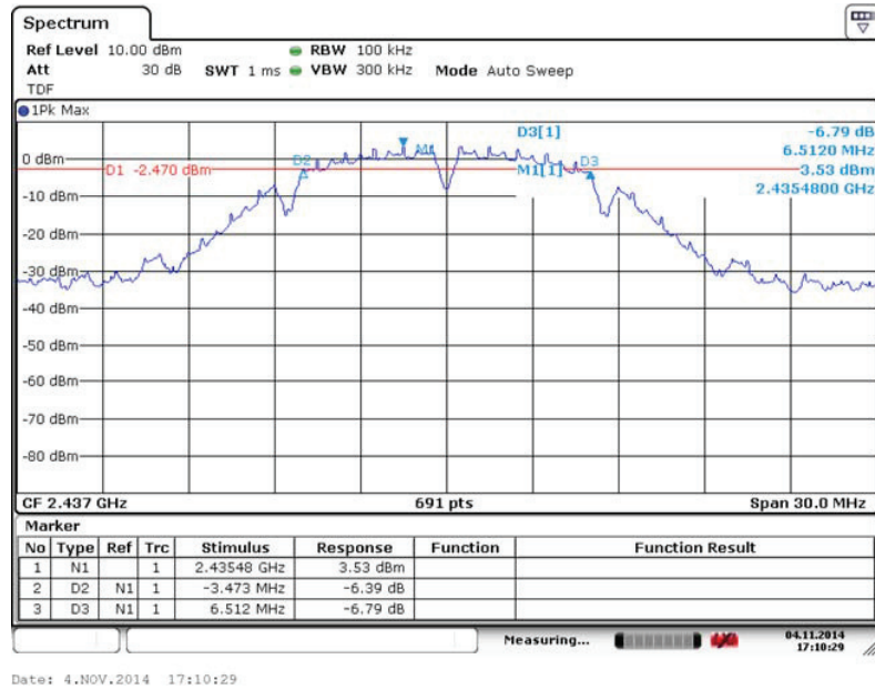
Fig. 98 Occupied 6dB Bandwidth (802.11b, Ch 6)
