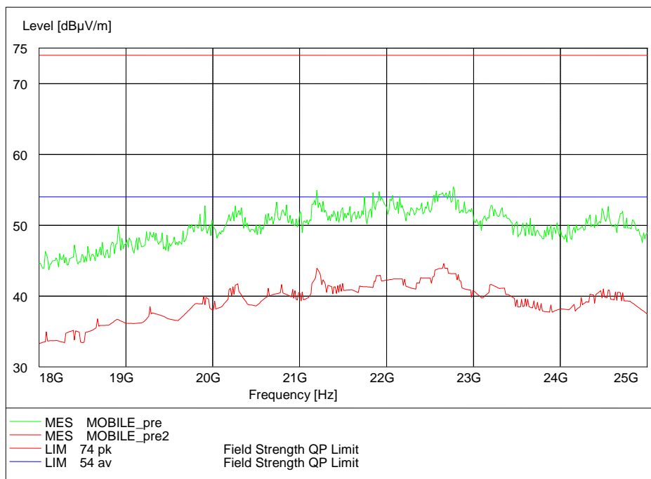
Frequency Range: 18GHz-25GHz Detector: Av mode and PK mode Modulation type: GFSK
