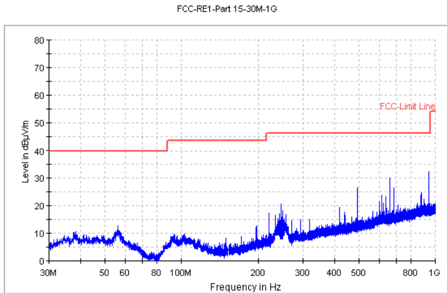
Fig. 50 Radiated Spurious Emission (GFSK, Ch0, 30 MHz ~1 GHz)
