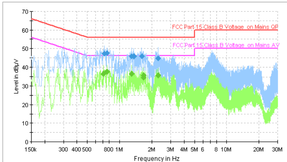
ESH2-Z5 Scan-FCC
