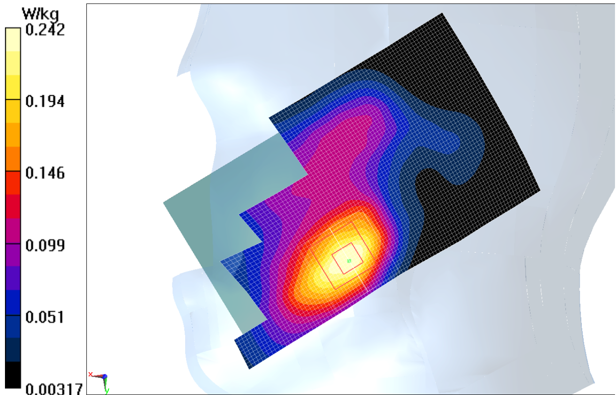
Fig.3 1900 MHz CH512
