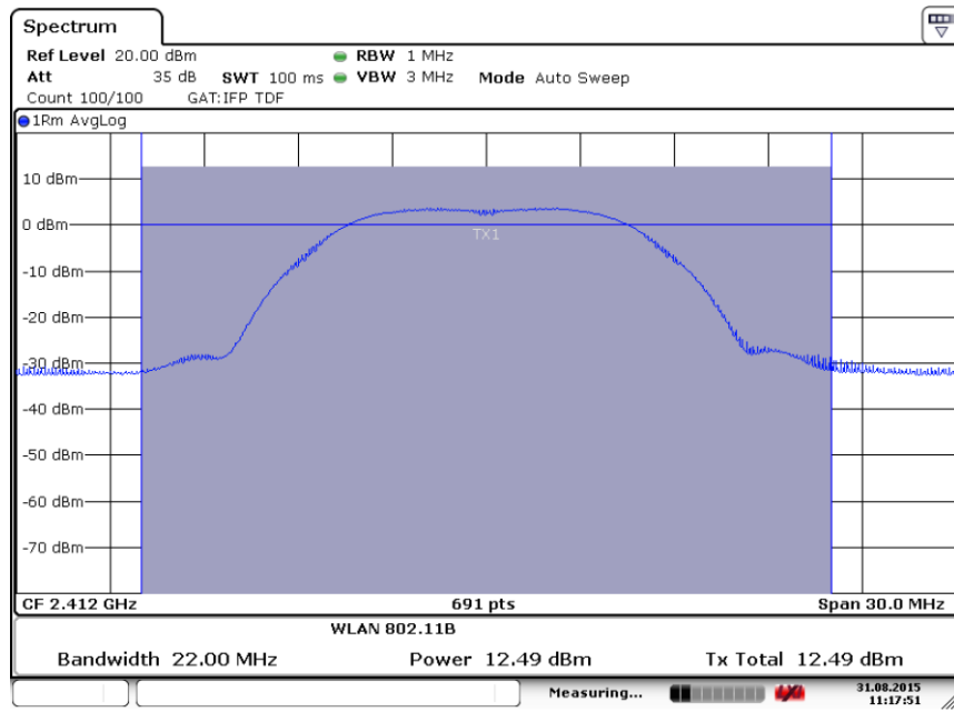
Fig.7 Maximum Average Output Power (802.11b, Ch 1,5Mbps)
