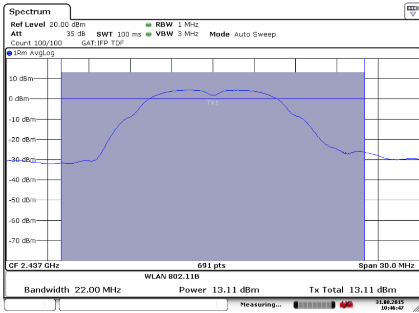
Fig.5 Maximum Average Output Power (802.11b, Ch 6,2Mbps)
